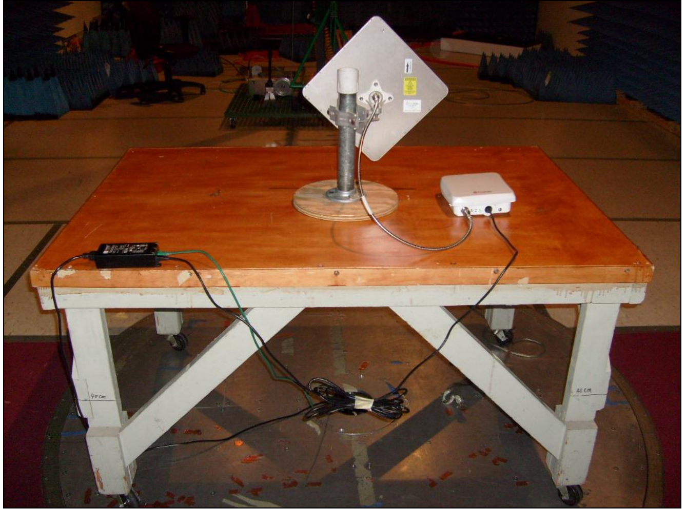
Photograph 9. Radiated Emissions, 23 dBi Panel, Rear View, Test Setup
