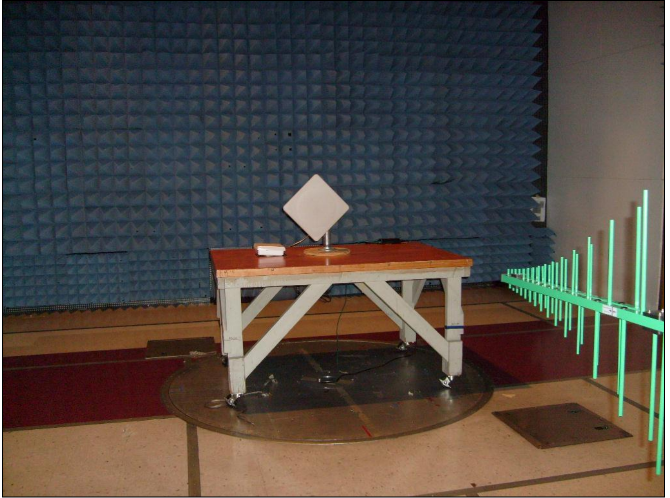
Photograph 10. Radiated Emissions, 30 MHz – 1 GHz
