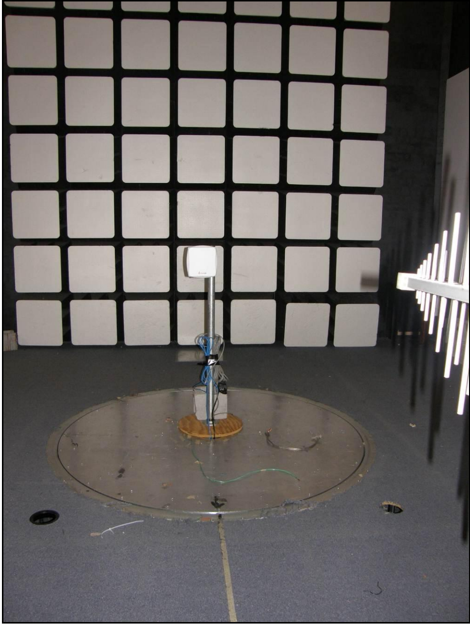
Photograph 4. Radiated Emission, Test Setup, 30 MHz – 1 GHz
