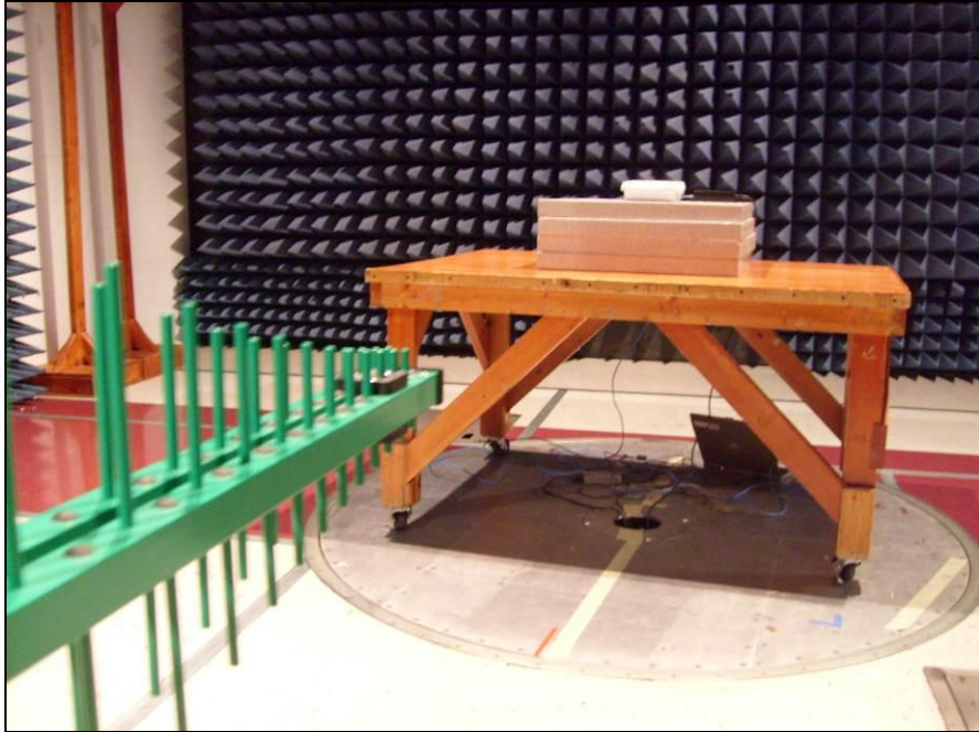
Photograph 1. Radiated Emission Spurious Test Setup, 30 MHz – 1 GHz
