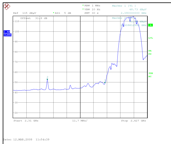
Plot 29. 802.11/b radiated restricted band 2310- 2390 MHz Avg., 2.4 GHz
