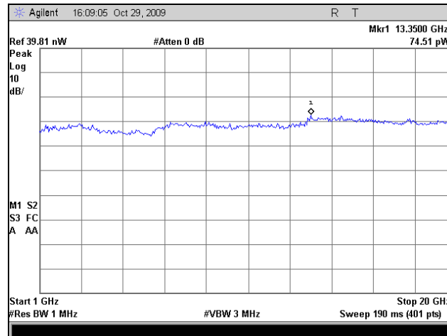
Plot 77. Conducted Spurious Emissions, 1 GHz – 20 GHz
