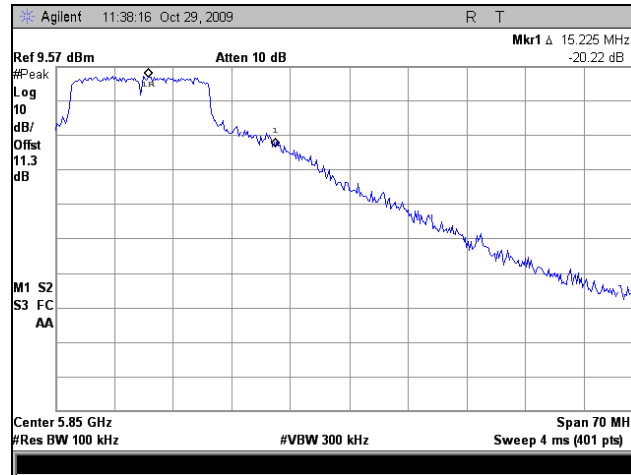
Plot 71. Upper Conducted Band Edge, High Channel, 5 GHz
