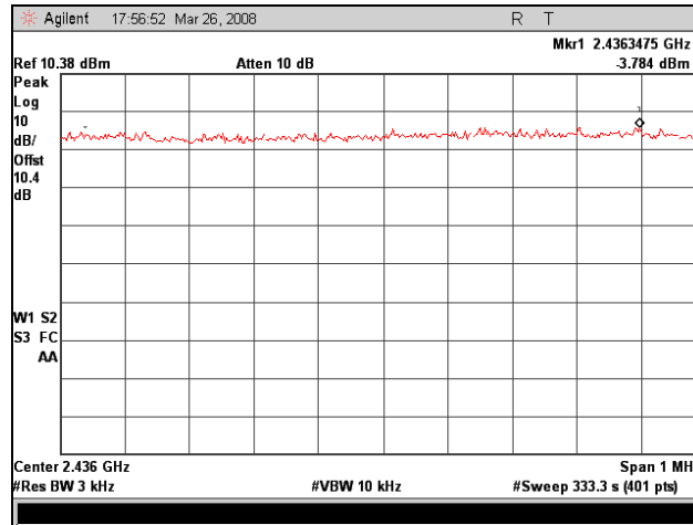
Plot 79. 802.11/b – Mid Ch Peak Power Spectral Density, 2.4 GHz
