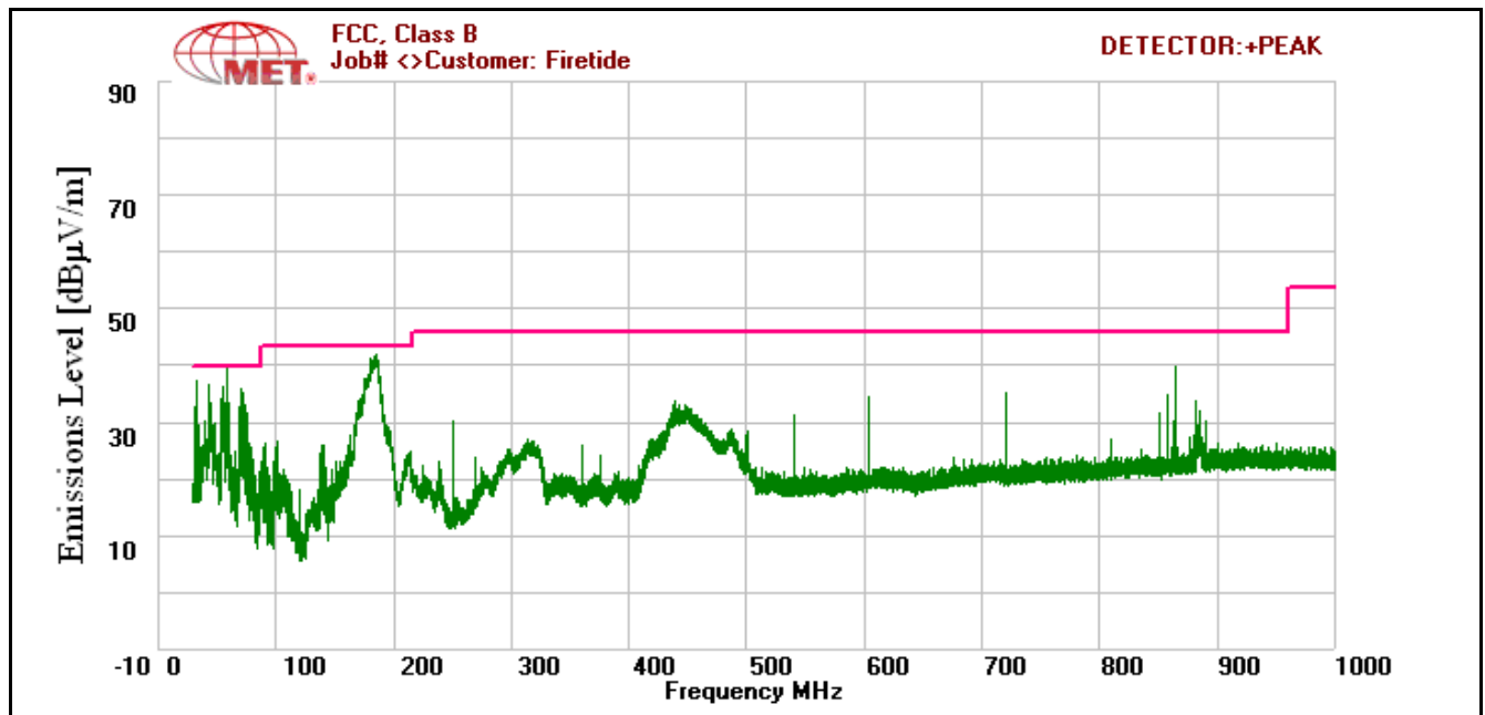
Plot 3. Radiated Emissions, FCC Limits, 30 MHz – 1 GHz
