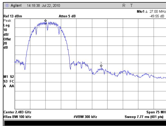
Plot 74. Upper Conducted Band Edge, High Channel, 2.4 GHz, 802.11b
