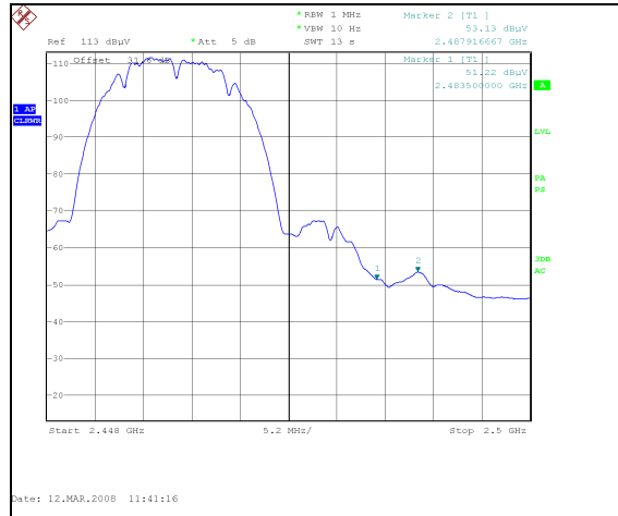
Plot 31. 802.11/b radiated restricted band 2483.5 – 2500MHz Avg., 2.4 GHz
