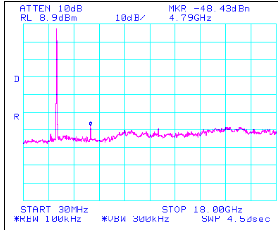
Plot 50. 802.11/b – Low Channel Conducted Emissions 30MHz - 18GHz, 2.4 GHz
