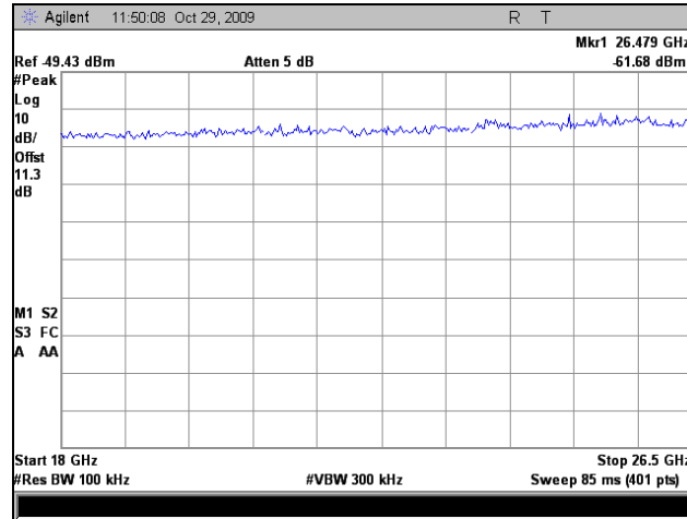
Plot 64. Conducted Emissions, Mid Channel 802.11a, 18 GHz – 26 GHz
