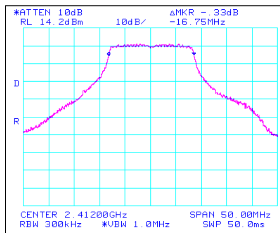
Plot 14. 802.11/g Low Ch Occupied Band Width, 2.4 GHz
