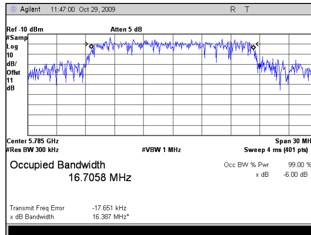
Plot 23. Occupied Band Width, Mid Channel, 802.11a, 20 MHz, IC Limits
