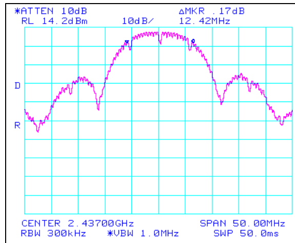
Plot 10. 802.11/b Mid Ch Occupied Band Width, 2.4 GHz
