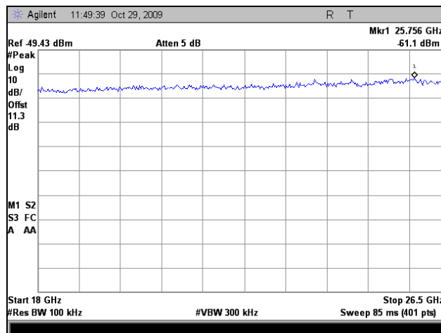
Plot 60. Conducted Emissions, Low Channel 802.11a, 18 GHz – 26 GHz
