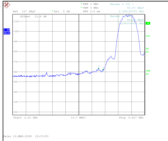
Plot 36. 802.11/b radiated restricted band 2310- 2390 MHz Peak, 2.4 GHz
