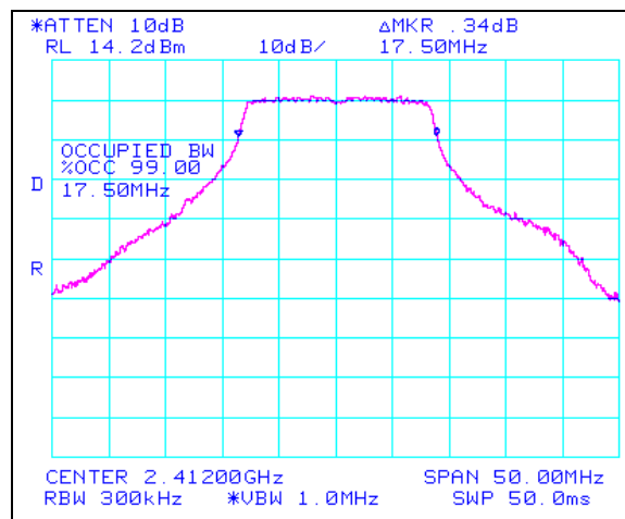
Plot 13. 802.11/g Low Ch Occupied Band Width 99%, 2.4 GHz
