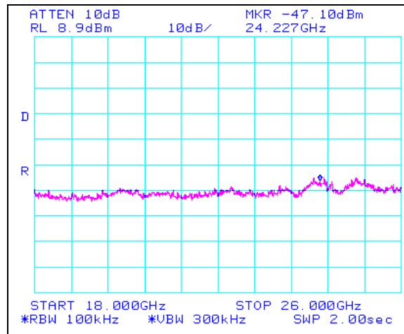
Plot 57. 802.11/g – High Channel Conducted Emissions 18-26GHz, 2.4 GHz
