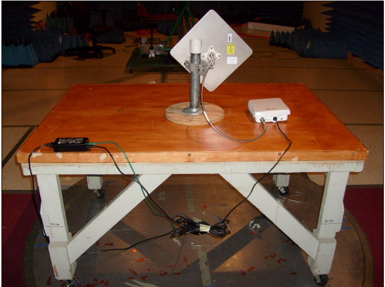
Photograph 7. Radiated Emissions, 23 dBi Panel, Rear View, Test Setup
