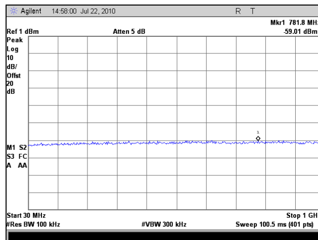
Plot 66. Conducted Emissions, High Channel, 802.11a, 30 MHz – 1 GHz
