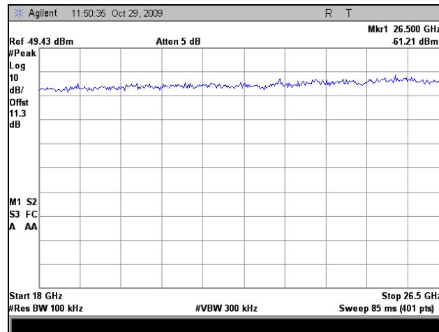
Plot 68. Conducted Emissions, High Channel 802.11a, 18 GHz – 26 GHz
