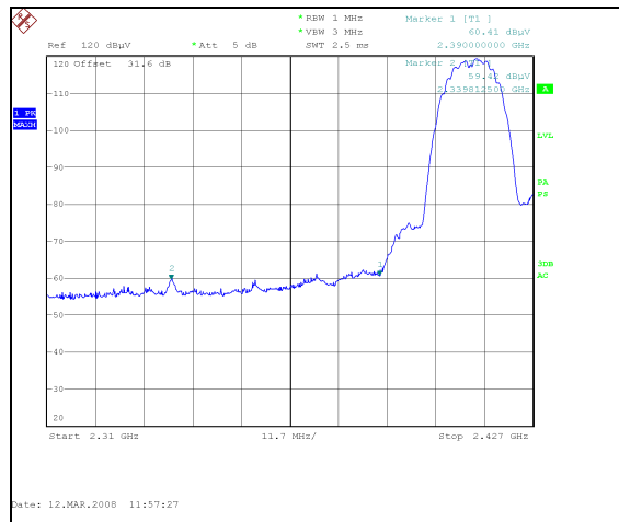
Plot 28. 802.11/b radiated restricted band 2310- 2390 MHz Peak, 2.4 GHz
