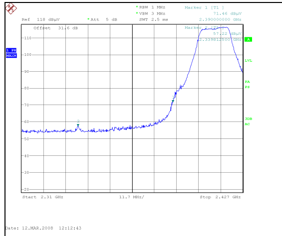
Plot 40. 802.11/g radiated restricted band 2310- 2390 MHz Peak, 2.4 GHz
