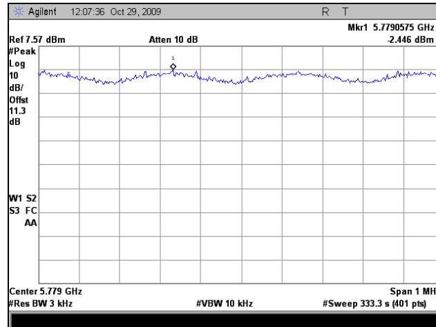
Plot 87. Peak Power Spectral Density, Mid Channel
