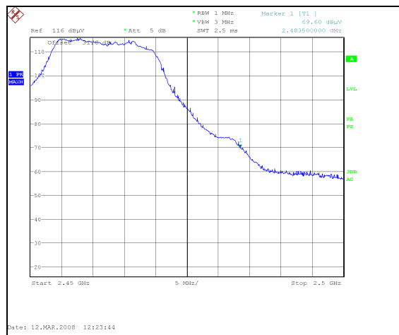
Plot 42. 802.11/g radiated restricted band 2483.5 – 2500MHz Peak, 2.4 GHz
