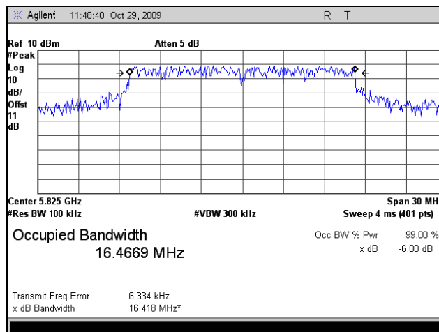
Plot 21. Occupied Band Width, High Channel, 802.11a, 20 MHz, FCC Limits
