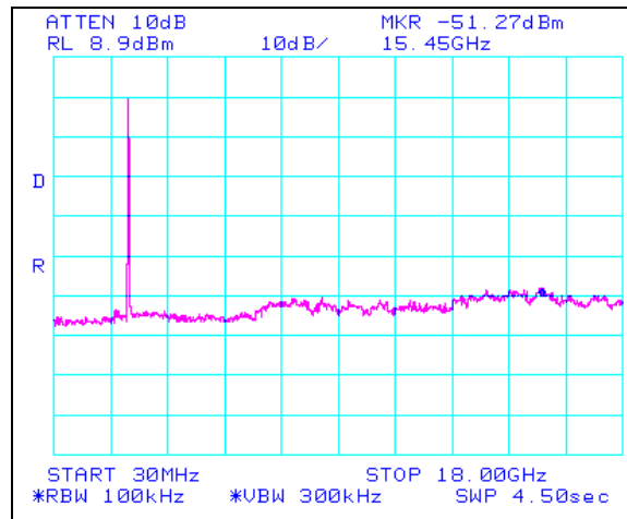
Plot 54. 802.11/g – Low Channel Conducted Emissions 30MHz- 18GHz, 2.4 GHz
