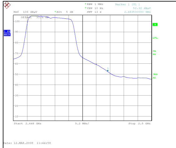
Plot 35. 802.11/g radiated restricted band 2483.5 – 2500MHz Avg., 2.4 GHz
