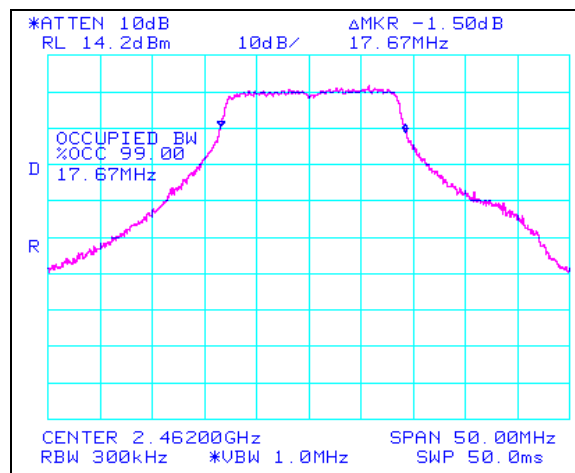
Plot 17. 802.11/g High Ch Occupied Band Width 99%, 2.4 GHz
