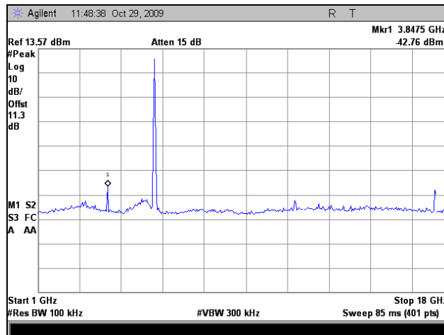
Plot 59. Conducted Emissions, Low Channel, 802.11a, 1 GHz – 18 GHz
