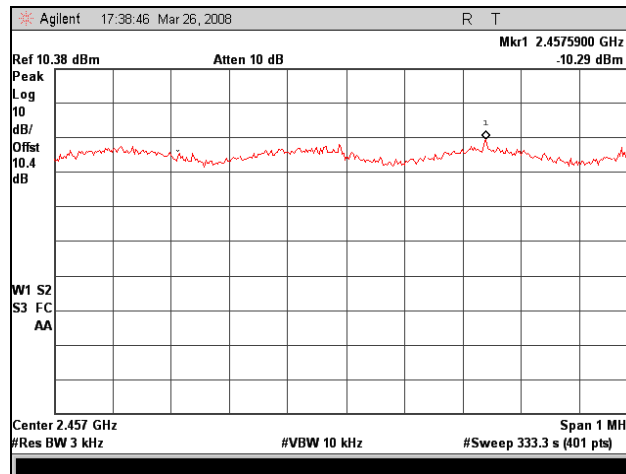
Plot 83. 802.11/g – High Ch Peak Power Spectral Density, 2.4 GHz
