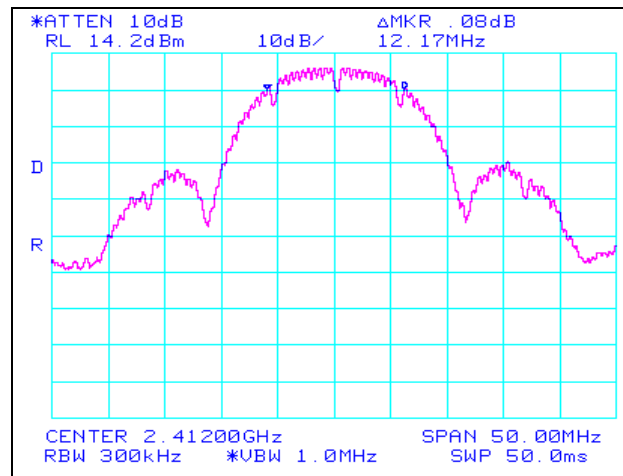
Plot 8. 802.11/b Low Ch Occupied Band Width, , 2.4 GHz
