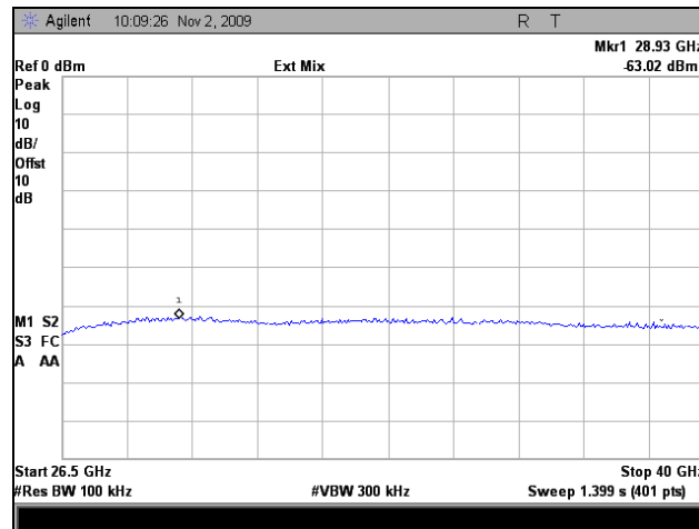
Plot 65. Conducted Emissions, Mid Channel, 802.11a, 26 GHz – 40 GHz
