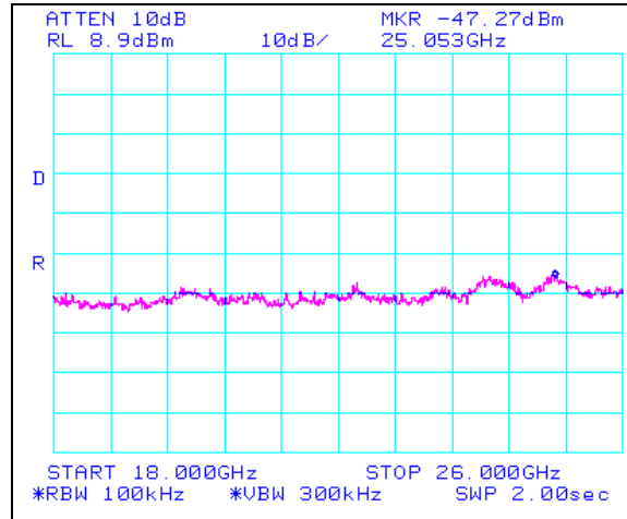
Plot 53. 802.11/b – High Channel Conducted Emissions 18-26GHz, 2.4 GHz
