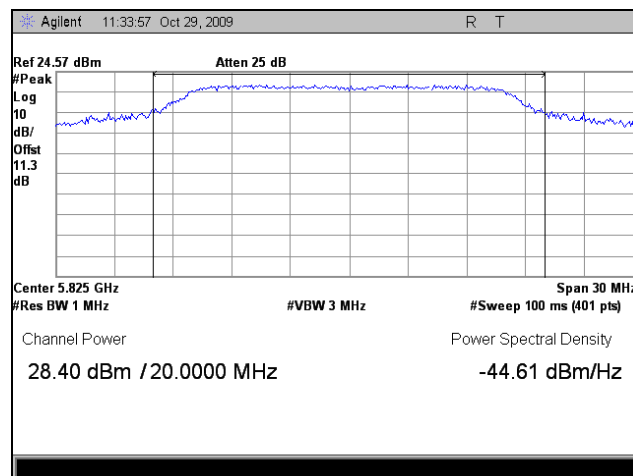
Plot 27. Peak Output Power, High Channel
