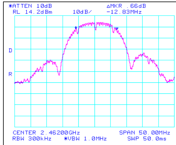
Plot 12. 802.11/b High Ch Occupied Band Width, 2.4 GHz
