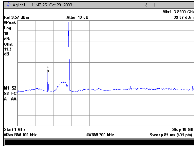
Plot 67. Conducted Emissions, High Channel, 802.11a, 1 GHz – 18 GHz
