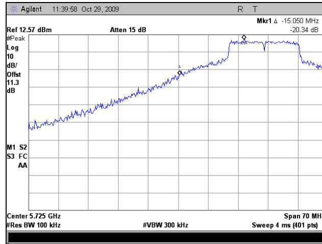
Plot 70. Lower Conducted Band Edge, Low Channel, 5 GHz
