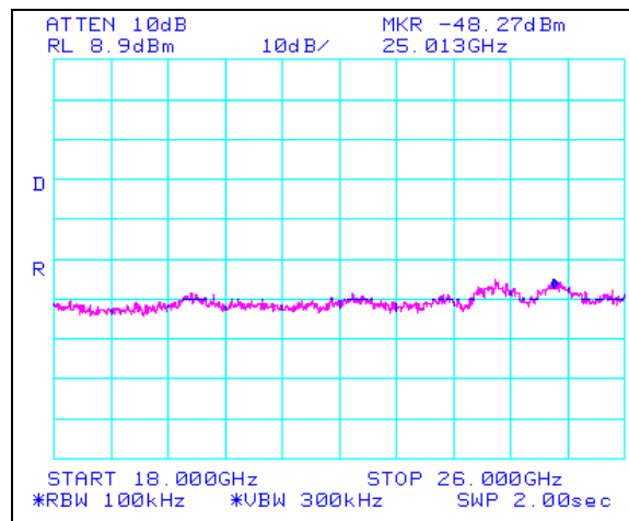
Plot 55. 802.11/g – Low Channel Conducted Emissions 18-26GHz, 2.4 GHz
