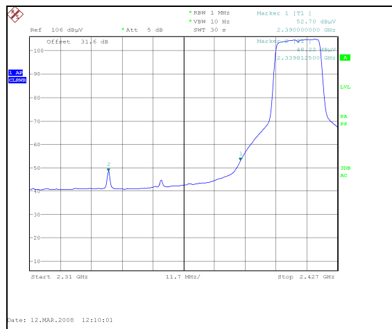
Plot 41. 802.11/g radiated restricted band 2310- 2390 MHz Avg., 2.4 GHz
