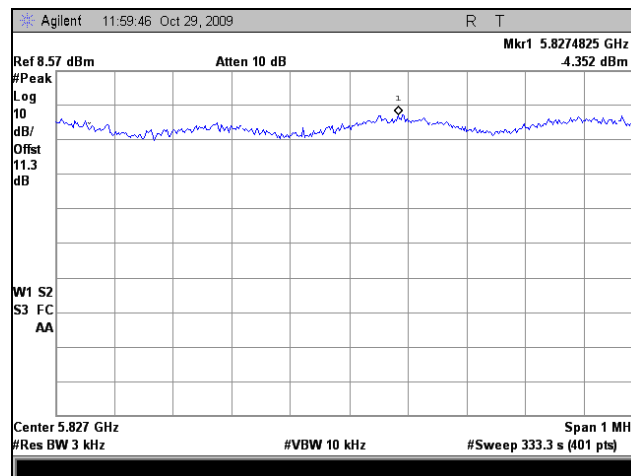
Plot 89. Peak Power Spectral Density, High Channel
