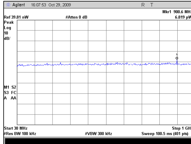
Plot 76. Conducted Spurious Emissions, 30 MHz – 1 GHz
