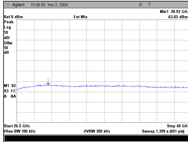
Plot 61. Conducted Emissions, Low Channel, 802.11a, 26 GHz – 40 GHz
