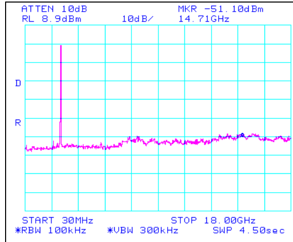
Plot 56. 802.11/g – High Channel Conducted Emissions 30MHz – 18GHz, 2.4 GHz
