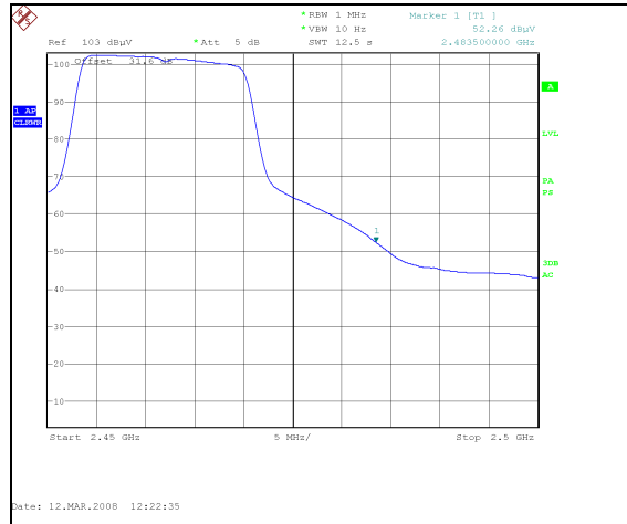
Plot 43. 802.11/g radiated restricted band 2483.5 – 2500MHz Avg., 2.4 GHz
