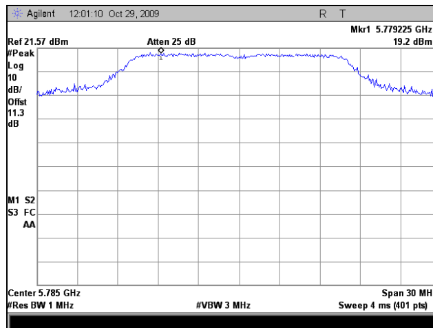
Plot 86. Peak Power Spectral Density, Mid Channel, Determination
