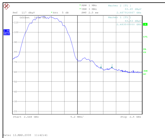
Plot 30. 802.11/b radiated restricted band 2483.5 – 2500MHz Peak, 2.4 GHz
