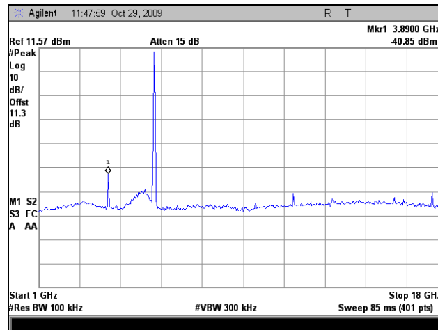
Plot 63. Conducted Emissions, Mid Channel, 802.11a, 1 GHz – 18 GHz
