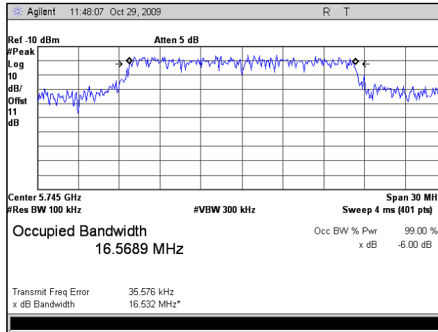
Plot 19. Occupied Band Width, Low Channel, 802.11a, 20 MHz, FCC Limits
