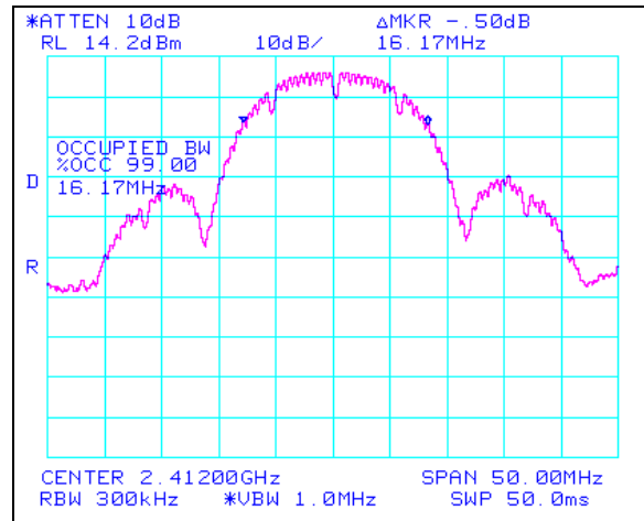
Plot 7. 802.11/b Low Ch Occupied Band Width 99%, 2.4 GHz
