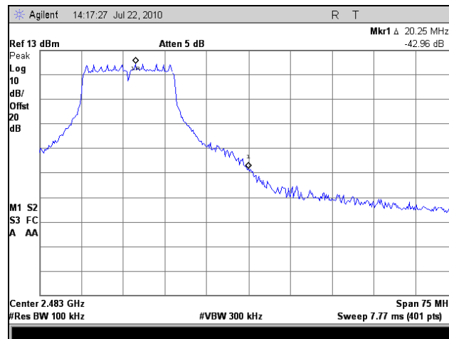
Plot 75. Upper Conducted Band Edge, High Channel, 2.4 GHz, 802.11g
