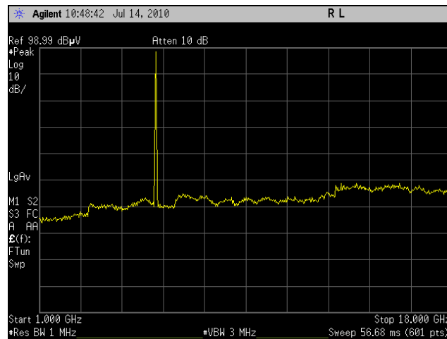
Plot 48. Radiated Spurious Emissions, Mid Channel, 802.11a, 1 GHz – 18 GHz, 23 dBi Panel
