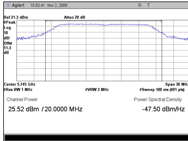
Plot 25. Peak Output Power, Low Channel
