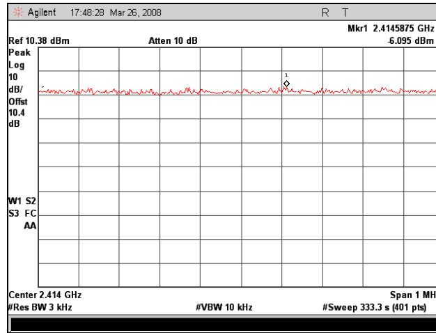
Plot 78. 802.11/b – Low Ch Peak Power Spectral Density, 2.4 GHz
