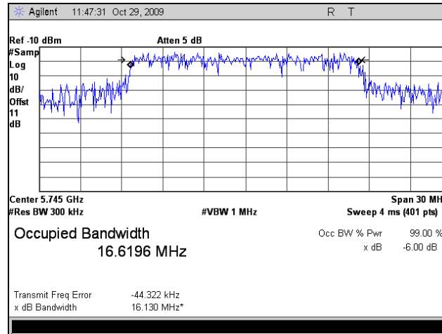
Plot 22. Occupied Band Width, Low Channel, 802.11a, 20 MHz, IC Limits
