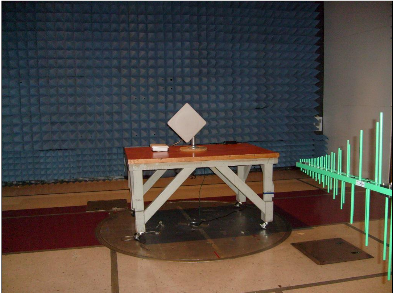
Photograph 8. Radiated Emissions, 30 MHz – 1 GHz
