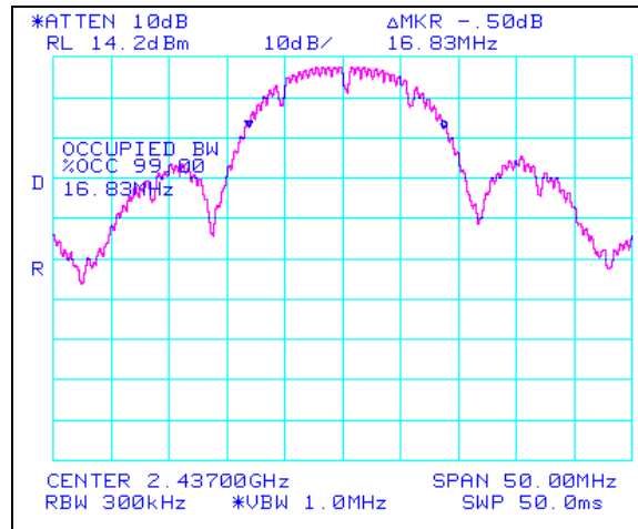
Plot 9. 802.11/b Mid Ch Occupied Band Width 99%, 2.4 GHz
