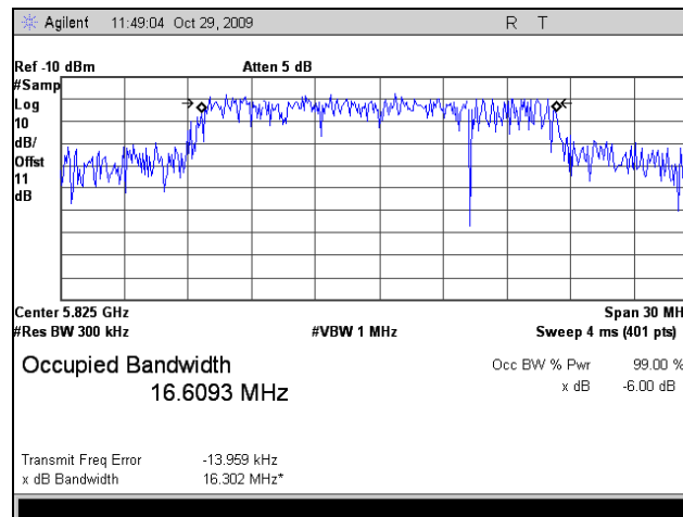
Plot 24. Occupied Band Width, High Channel, 802.11a, 20 MHz, IC Limits
