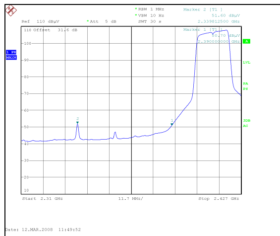
Plot 33. 802.11/g radiated restricted band 2310- 2390 MHz Avg., 2.4 GHz
