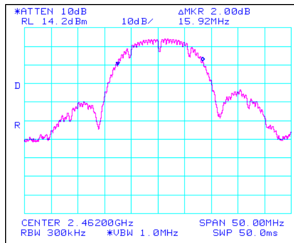
Plot 11. 802.11/b High Ch Occupied Band Width 99%, 2.4 GHz
