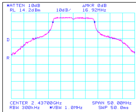
Plot 16. 802.11/g Mid Ch Occupied Band Width, 2.4 GHz
