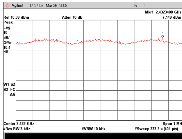
Plot 82. 802.11/g – Mid Ch Peak Power Spectral Density, 2.4 GHz
