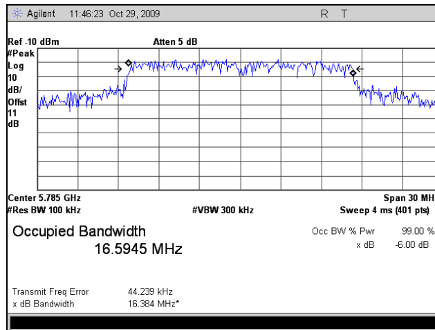
Plot 20. Occupied Band Width, Mid Channel, 802.11a, 20 MHz, FCC Limits
