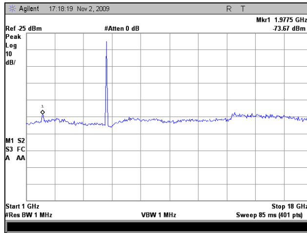
Plot 44. Radiated Spurious Emissions, Low Channel, 802.11a, 1 GHz – 18 GHz
