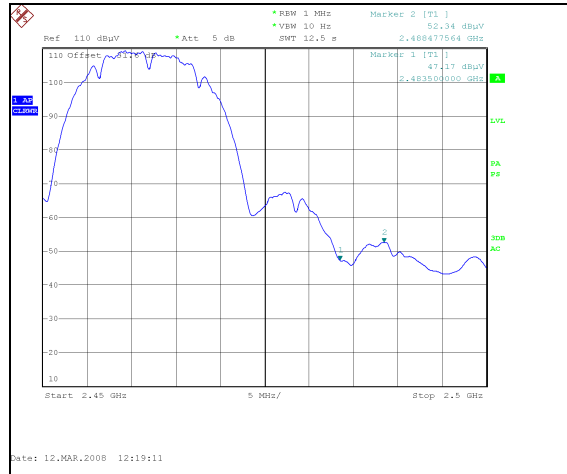
Plot 39. 802.11/b radiated restricted band 2483.5 – 2500MHz Avg., 2.4 GHz
