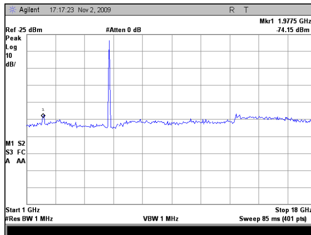
Plot 46. Radiated Spurious Emissions, High Channel, 802.11a, 1 GHz – 18 GHz
