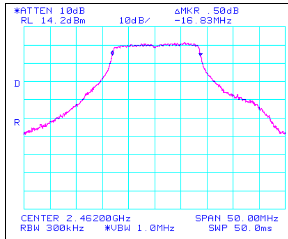
Plot 18. 802.11/g High Ch Occupied Band Width, 2.4 GHz
