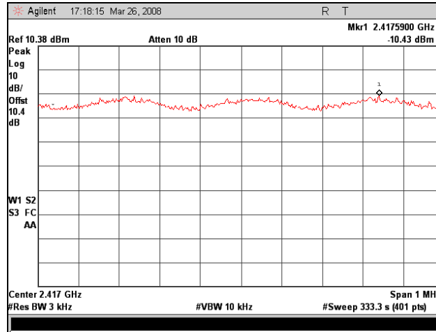
Plot 81. 802.11/g – Low Ch Peak Power Spectral Density, 2.4 GHz
