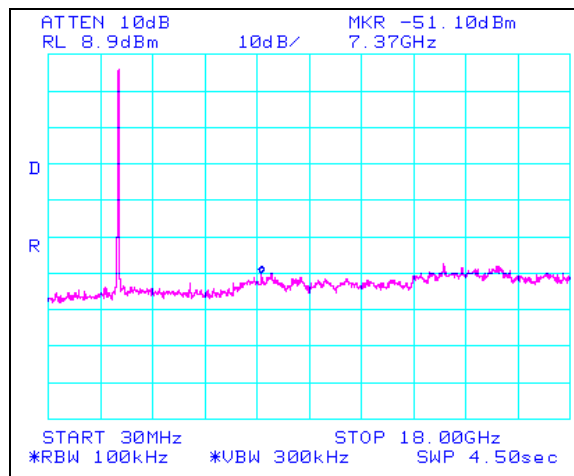
Plot 52. 802.11/b – High Channel Conducted Emissions 30MHz- 18GHz, 2.4 GHz
