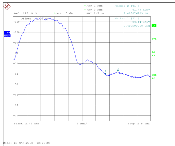
Plot 38. 802.11/b radiated restricted band 2483.5 – 2500MHz Peak, 2.4 GHz
