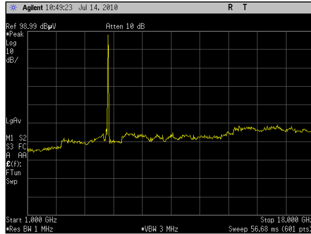
Plot 47. Radiated Spurious Emissions, Low Channel, 802.11a, 1 GHz – 18 GHz, 23 dBi Panel
