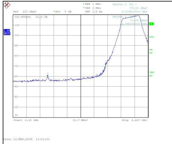
Plot 32. 802.11/g radiated restricted band 2310- 2390 MHz Peak, 2.4 GHz
