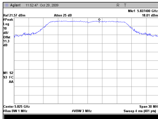
Plot 88. Peak Power Spectral Density, High Channel, Determination
