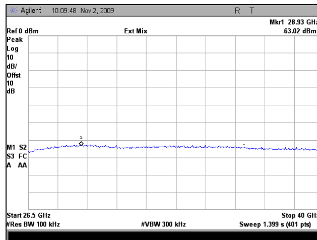
Plot 69. Conducted Emissions, High Channel, 802.11a, 26 GHz – 40 GHz
