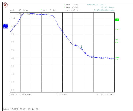
Plot 34. 802.11/g radiated restricted band 2483.5 – 2500MHz Peak, 2.4 GHz
