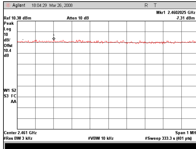
Plot 80. 802.11/b – High Ch Peak Power Spectral Density, 2.4 GHz
