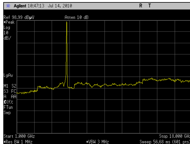
Plot 49. Radiated Spurious Emissions, High Channel, 802.11a, 1 GHz – 18 GHz, 23 dBi Panel
