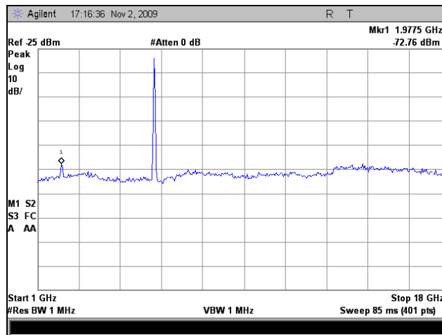
Plot 45. Radiated Spurious Emissions, Mid Channel, 802.11a, 1 GHz – 18 GHz
