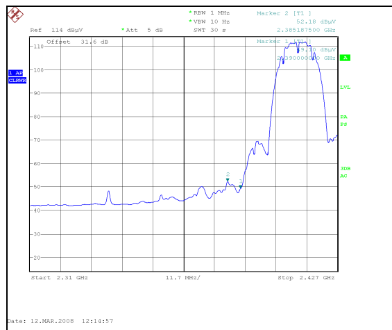
Plot 37. 802.11/b radiated restricted band 2310- 2390 MHz Avg., 2.4 GHz
