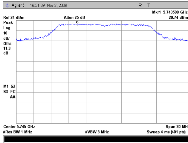
Plot 84. Peak Power Spectral Density, Low Channel, Determination
