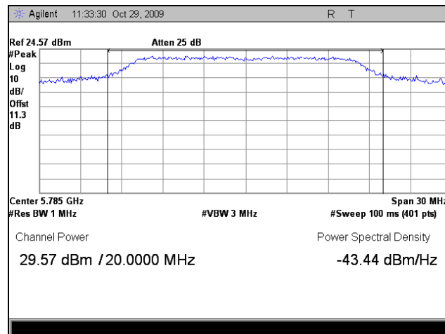
Plot 26. Peak Output Power, Mid Channel
