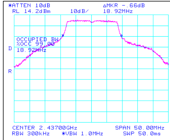
Plot 15. 802.11/g Mid Ch Occupied Band Width 99%, 2.4 GHz
