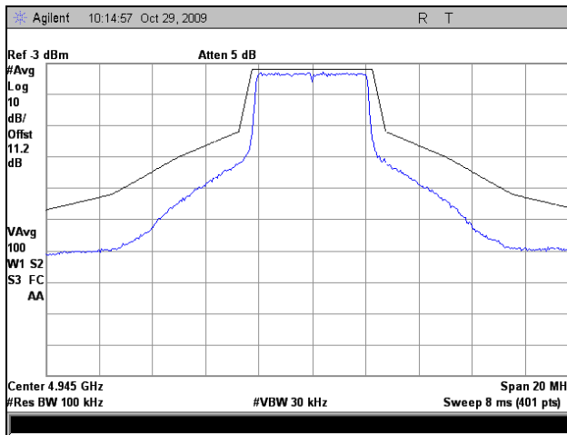
Plot 17. Emission Mask, 802.11a, Low Channel, 5 MHz
