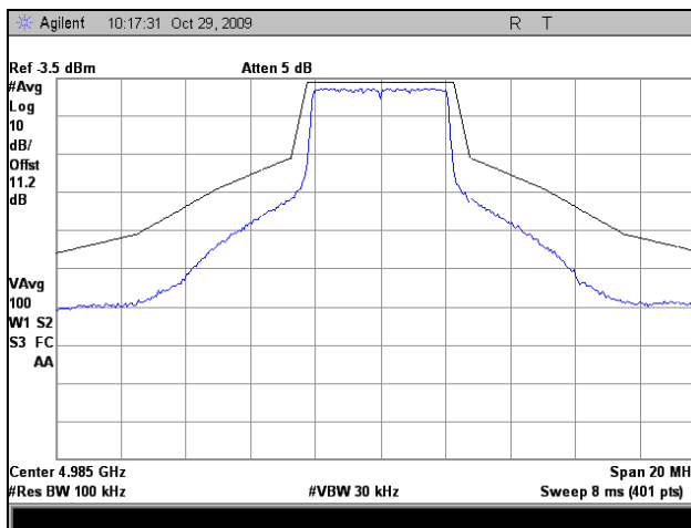
Plot 19. Emission Mask, 802.11a, High Channel, 5 MHz
