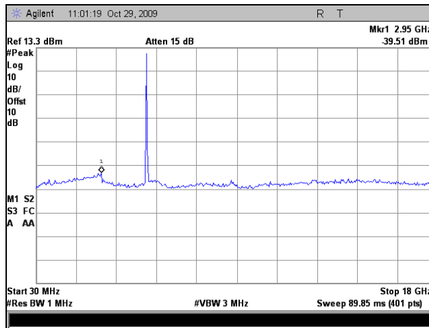
Plot 36. Conducted Spurious Emissions, Mid Channel, 5 MHz (30 MHz - 18GHz)
