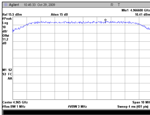
Plot 13. Peak Spectral Density, 802.11a, Mid Channel, 10 MHz
