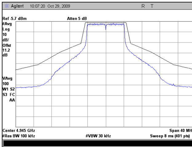
Plot 20. Emission Mask, 802.11a, Low Channel, 10 MHz
