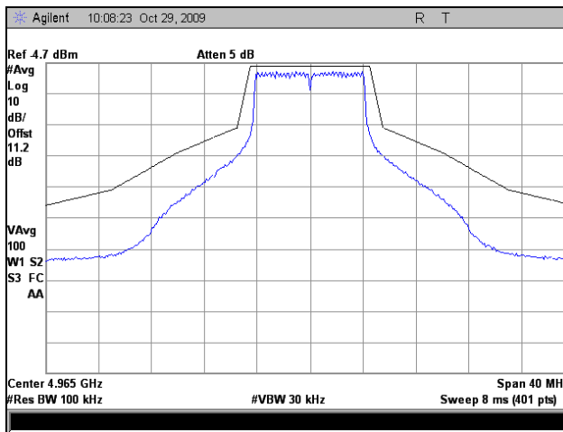
Plot 21. Emission Mask, 802.11a, Mid Channel, 10 MHz
