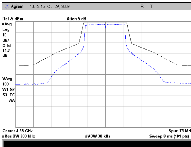
Plot 24. Emission Mask, 802.11a, High Channel, 20 MHz
