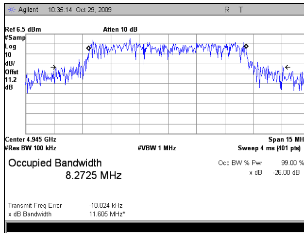
Plot 28. Occupied Bandwidth, 802.11a, Low Channel, 10 MHz
