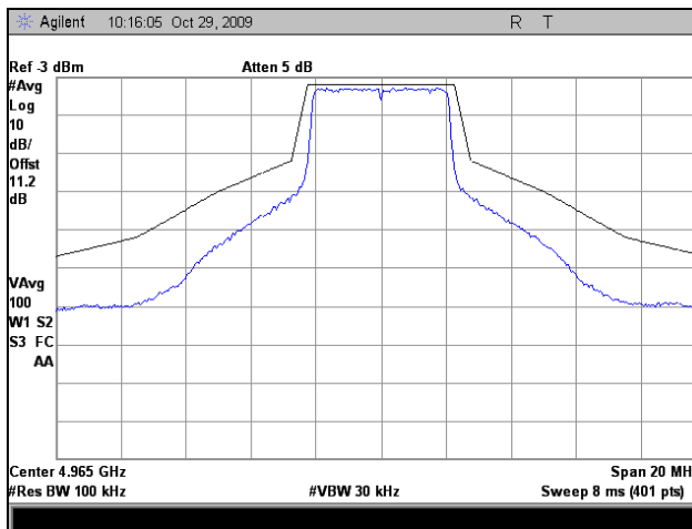
Plot 18. Emission Mask, 802.11a, Mid Channel, 5 MHz
