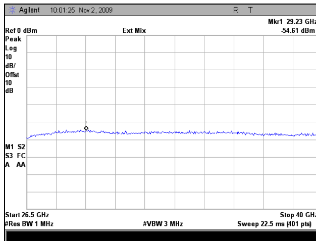
Plot 56. Conducted Spurious Emissions, High Channel, 20 MHz (26 GHz – 40 GHz)
