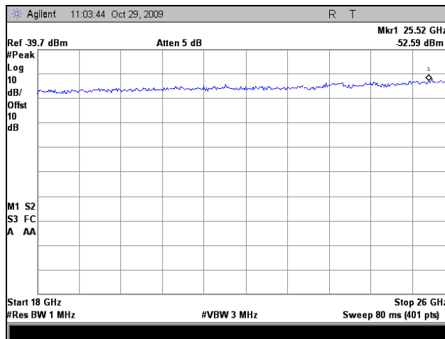
Plot 37. Conducted Spurious Emissions, Mid Channel, 5 MHz (18 GHz – 26 GHz)
