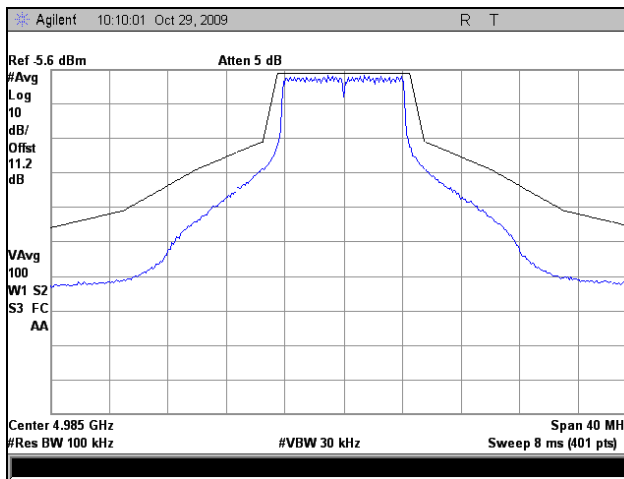
Plot 22. Emission Mask, 802.11a, High Channel, 10 MHz
