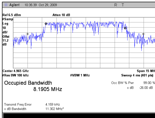
Plot 29. Occupied Bandwidth, 802.11a, Mid Channel, 10 MHz
