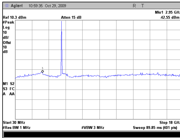
Plot 45. Conducted Spurious Emissions, Mid Channel, 10 MHz (30 MHz - 18GHz)
