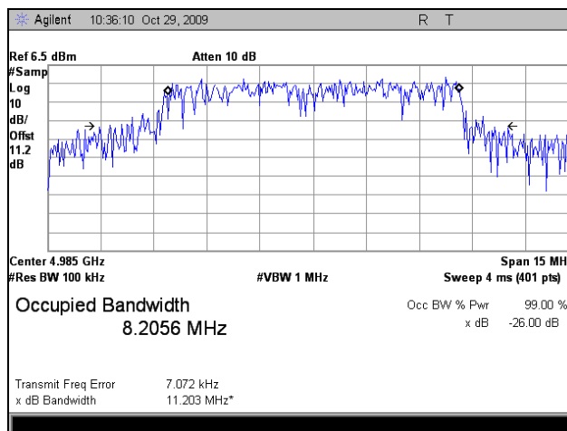
Plot 30. Occupied Bandwidth, 802.11a, High Channel, 10 MHz
