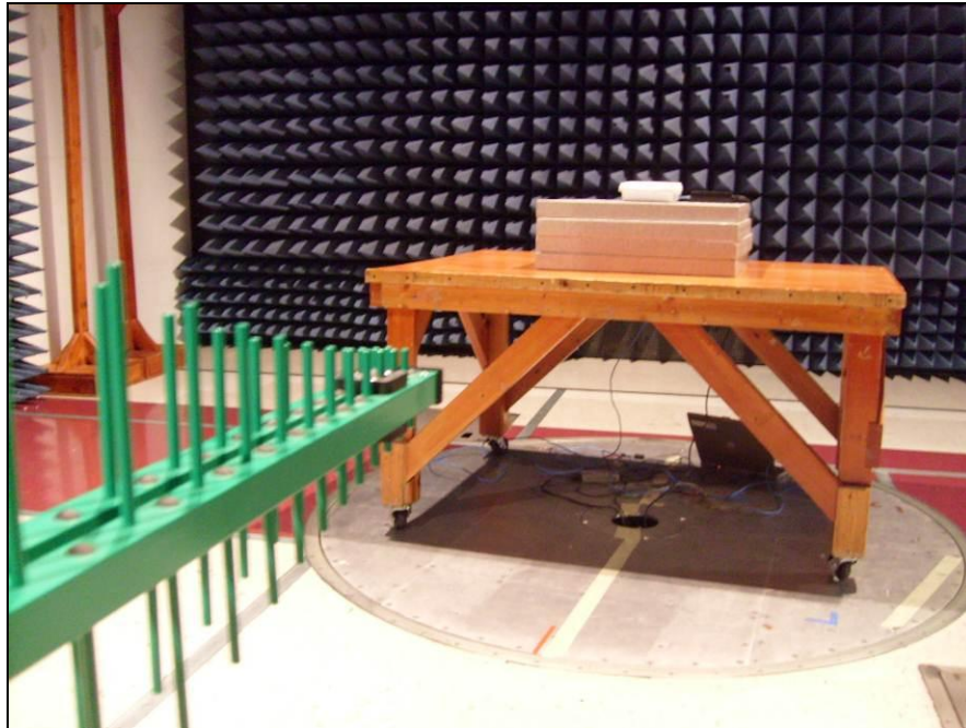
Photograph 2. Radiated Emission Spurious Test Setup, 30 MHz – 1 GHz
