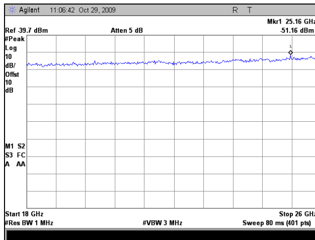
Plot 55. Conducted Spurious Emissions, High Channel, 20 MHz (18 GHz – 26 GHz)
