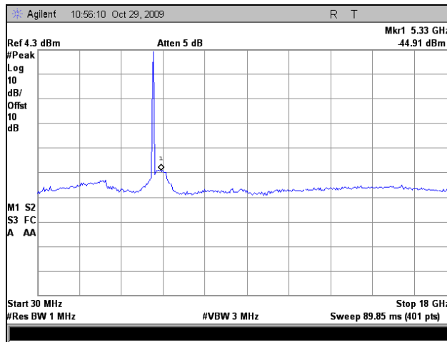
Plot 54. Conducted Spurious Emissions, High Channel, 20 MHz (30 MHz - 18GHz)
