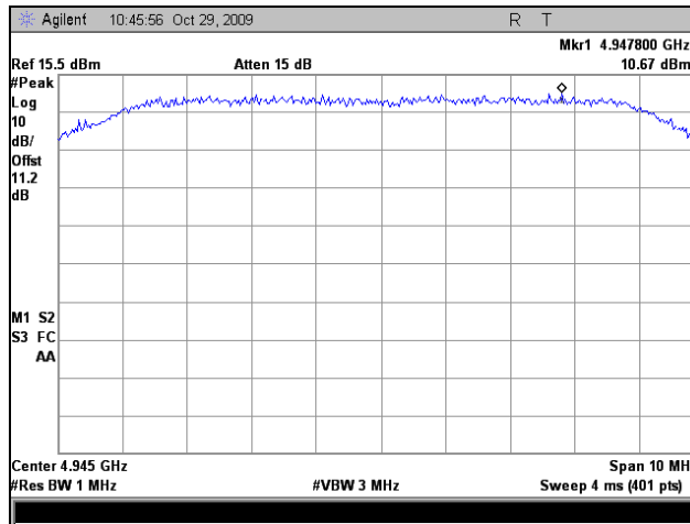
Plot 12. Peak Spectral Density, 802.11a, Low Channel, 10 MHz
