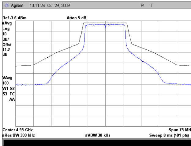
Plot 23. Emission Mask, 802.11a, Low Channel, 20 MHz
