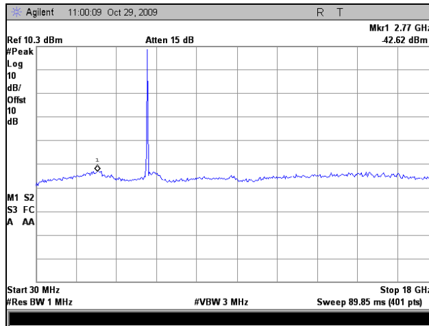
Plot 48. Conducted Spurious Emissions, High Channel, 10 MHz (30 MHz - 18GHz)
