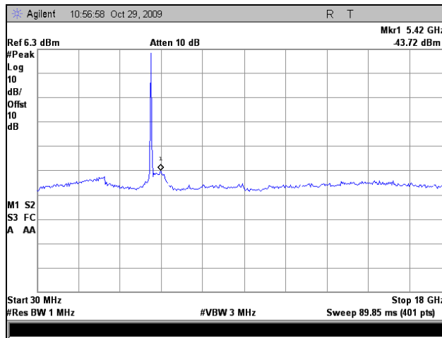
Plot 51. Conducted Spurious Emissions, Low Channel, 20 MHz (30 MHz - 18GHz)
