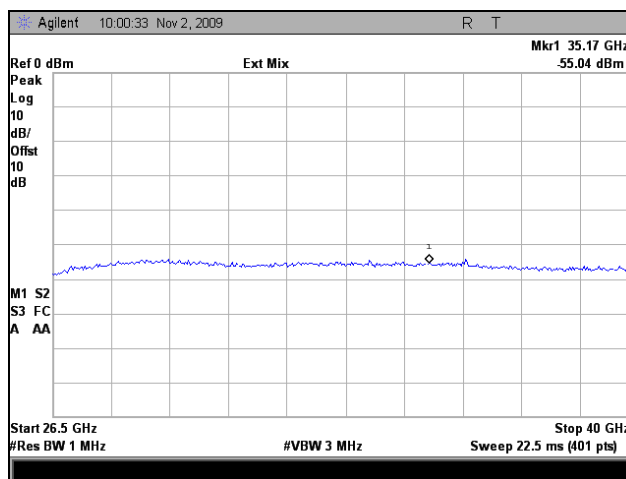
Plot 53. Conducted Spurious Emissions, Low Channel, 20 MHz (26 GHz – 40 GHz)
