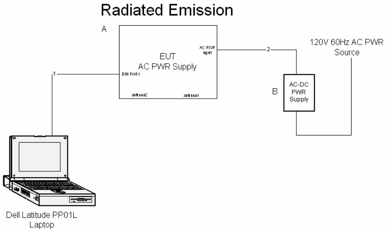
Figure 2. Block Diagram of Test Configuration (Radiated Emissions)
