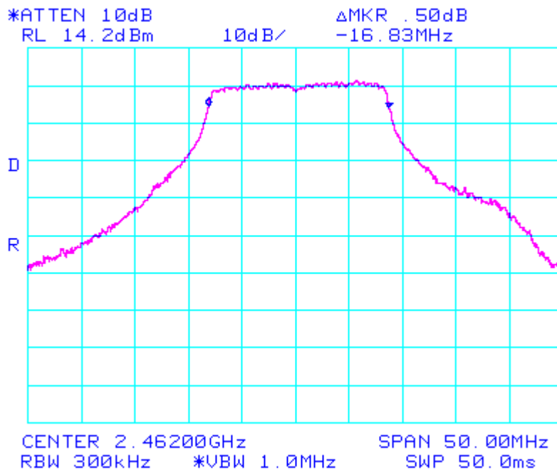
802.11/g High Ch Occupied Band Width
