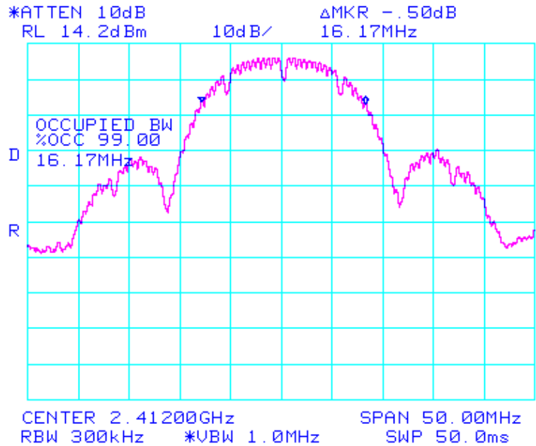
802.11/b Low Ch Occupied Band Width 99%.
