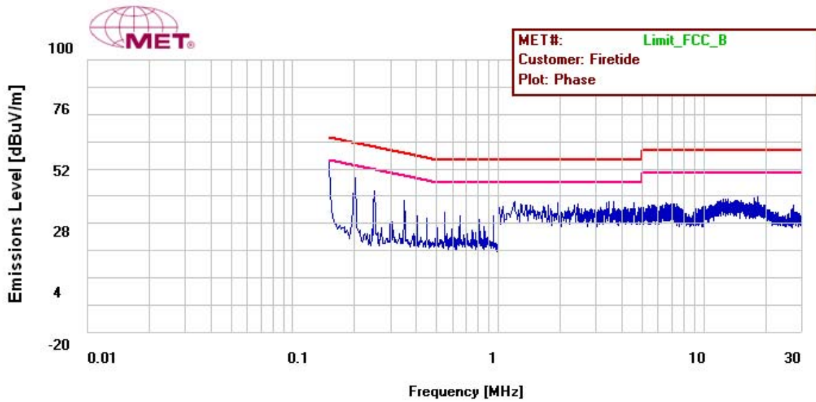
Plot 1. Conducted Emissions, Phase Line Plot
