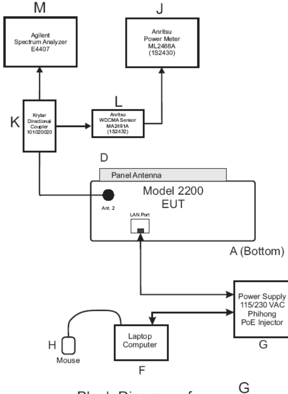
Block Diagram of Test Configuration (Conducted Emissions)
