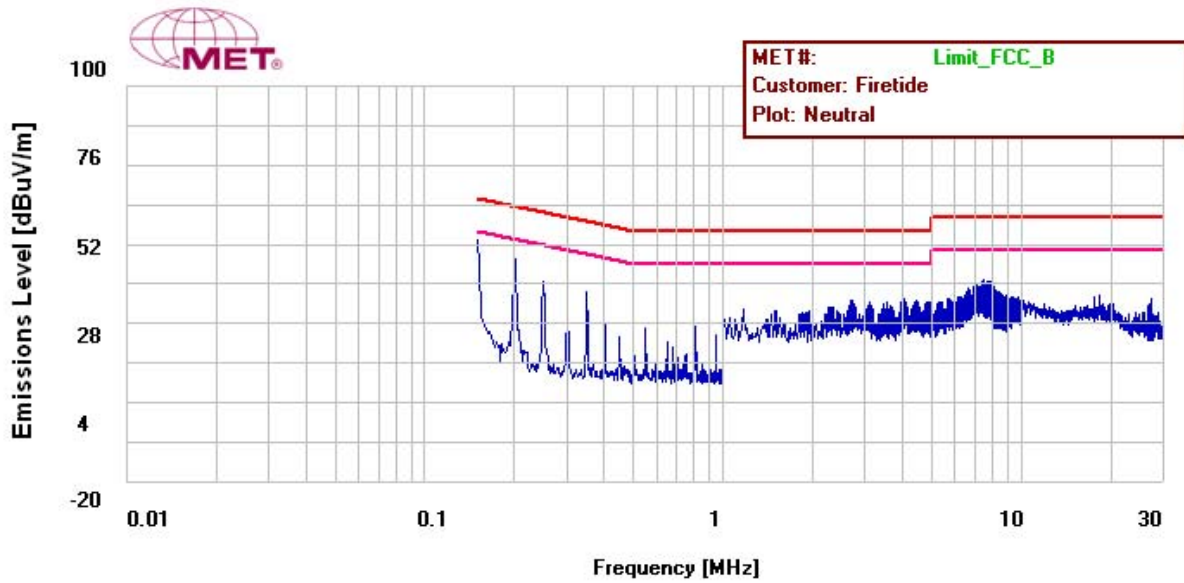
Plot 2. Conducted Emissions, Neutral Line Plot
