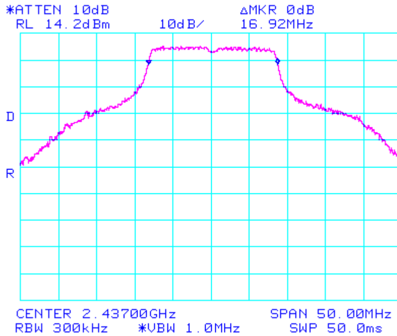
802.11/g Mid Ch Occupied Band Width
