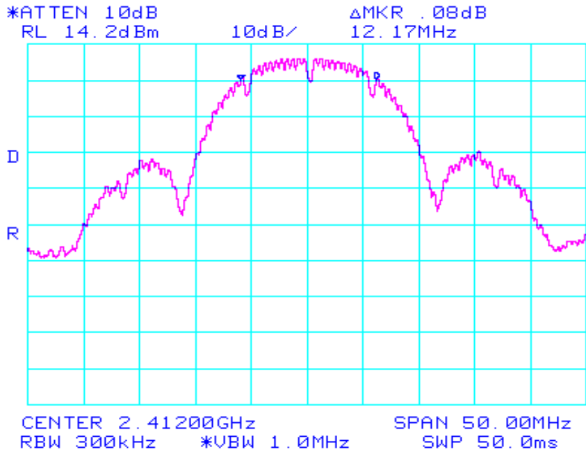
802.11/b Low Ch Occupied Band Width.
