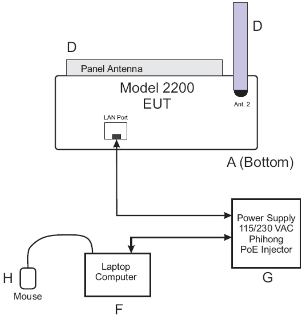
Block Diagram of Test Configuration (Radiated Emissions)
