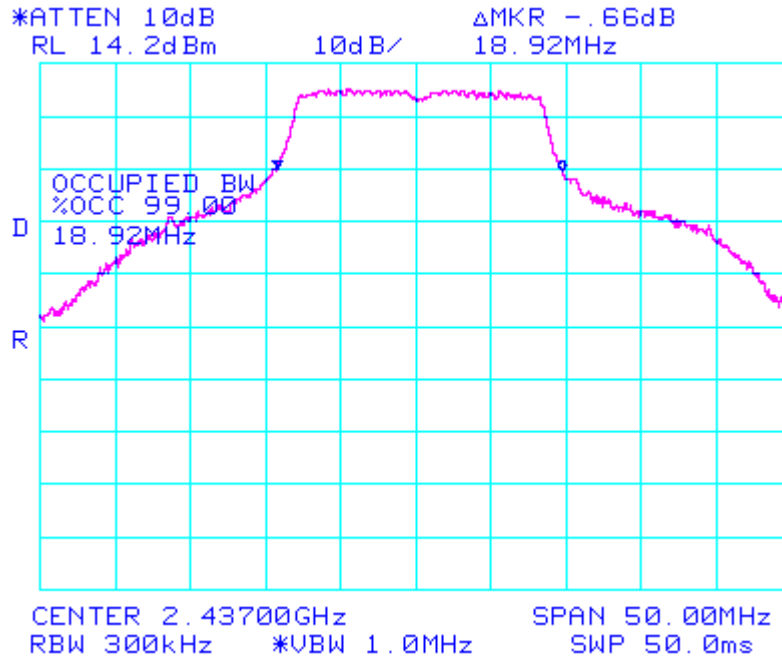
802.11/g Mid Ch Occupied Band Width 99%
