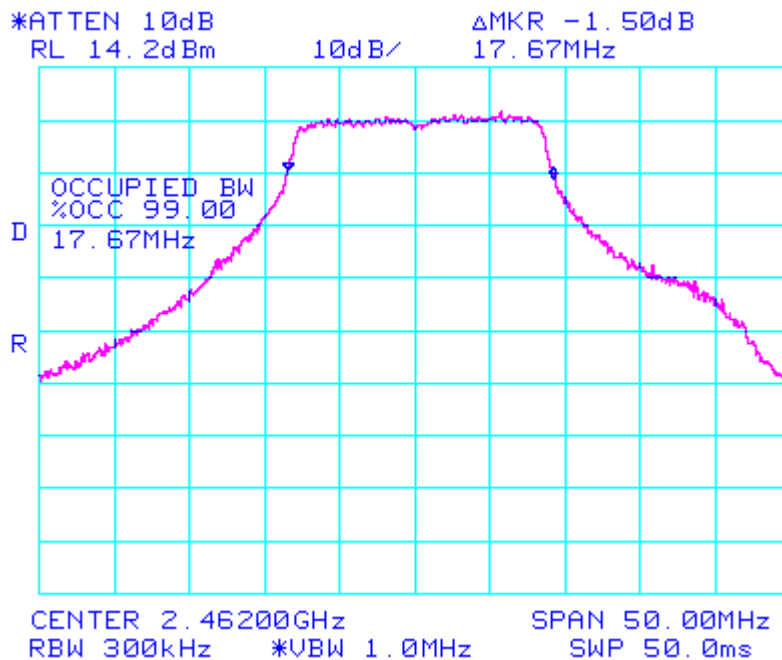
802.11/g High Ch Occupied Band Width 99%
