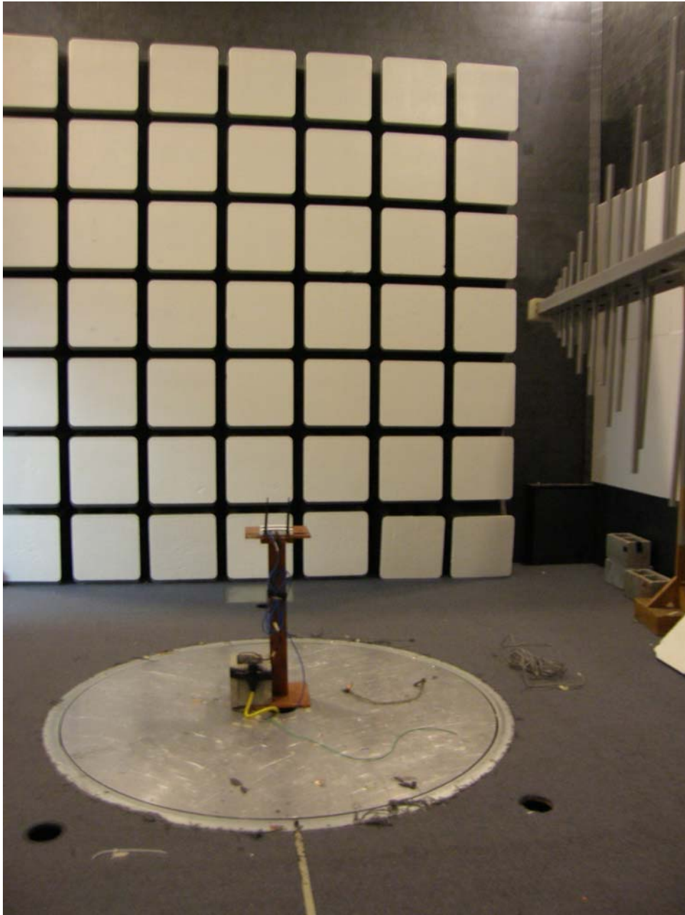
Radiated Emission Test Setup 30 MHz - 1 GHz
