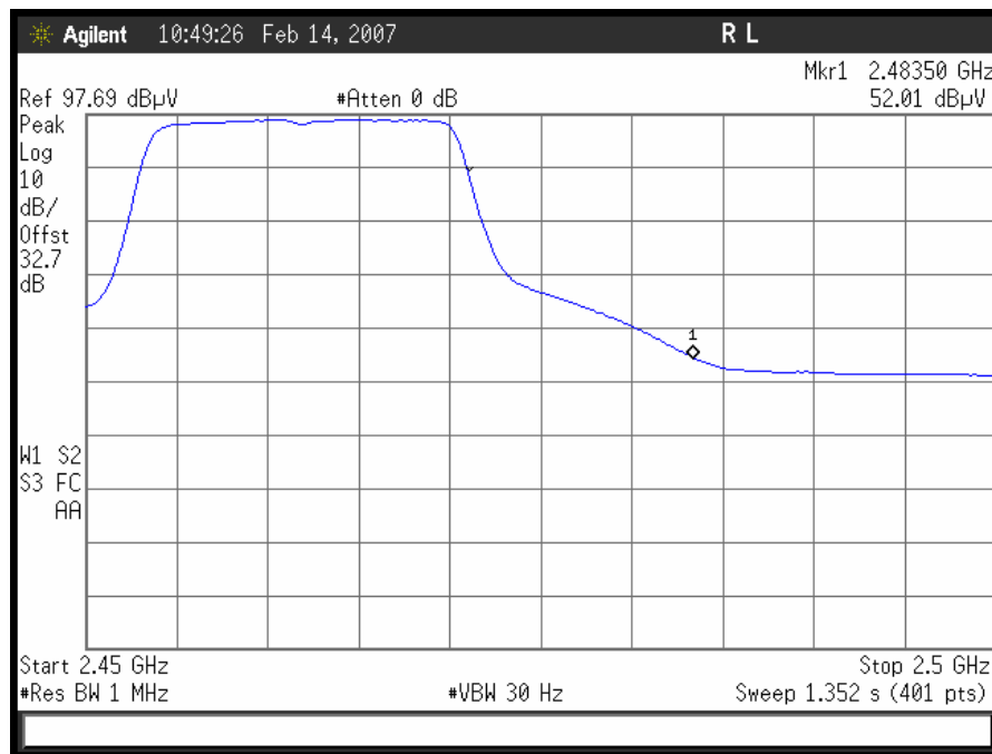
802.11/g radiated restricted band 2483.5 – 2500MHz Avg
