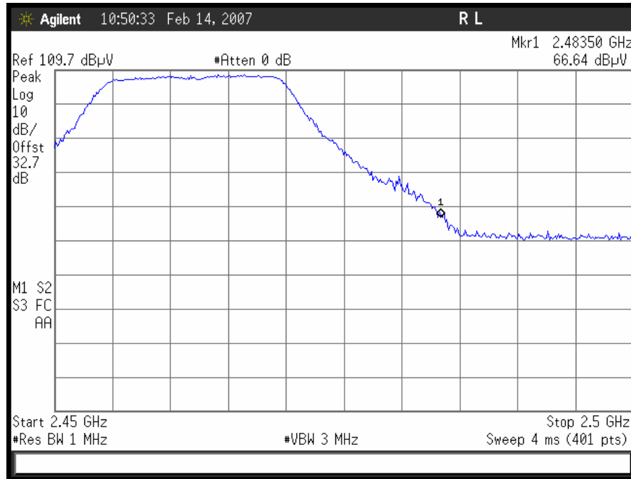
802.11/g radiated restricted band 2483.5 – 2500MHz Peak
