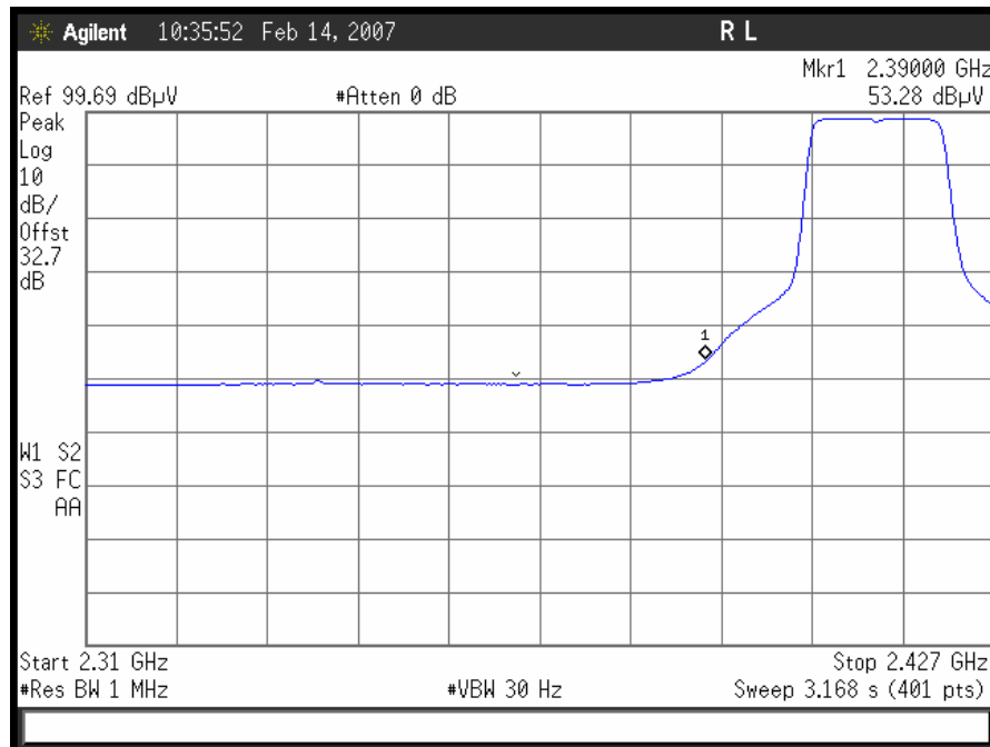
802.11/g radiated restricted band 2310- 2390 MHz Avg
