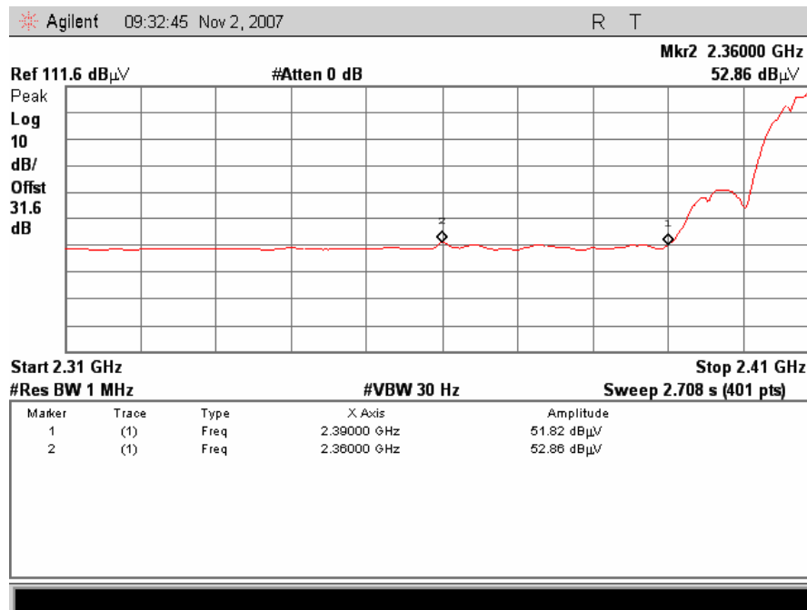
802.11/b radiated restricted band 2310- 2390 MHz Avg
