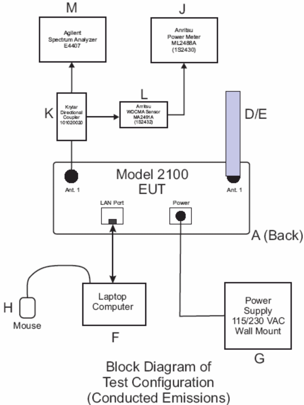
Figure 2. Block Diagram of Test Configuration (Conducted Emissions)
