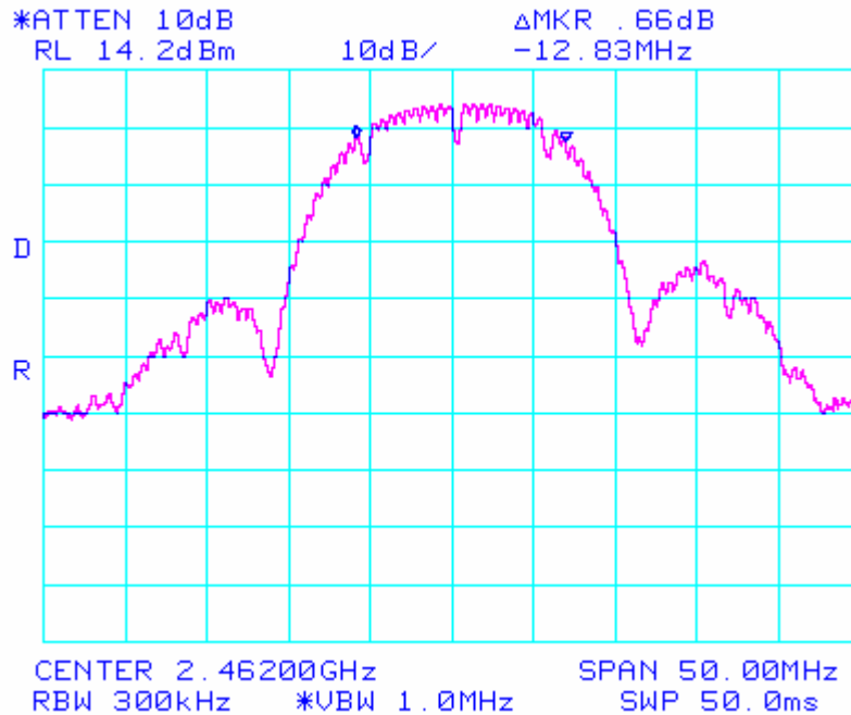
802.11/b High Ch Occupied Band Width
