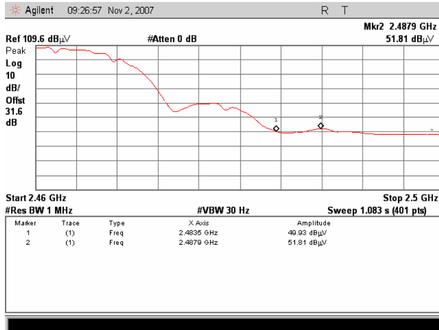
802.11/b radiated restricted band 2483.5 – 2500MHz Avg
