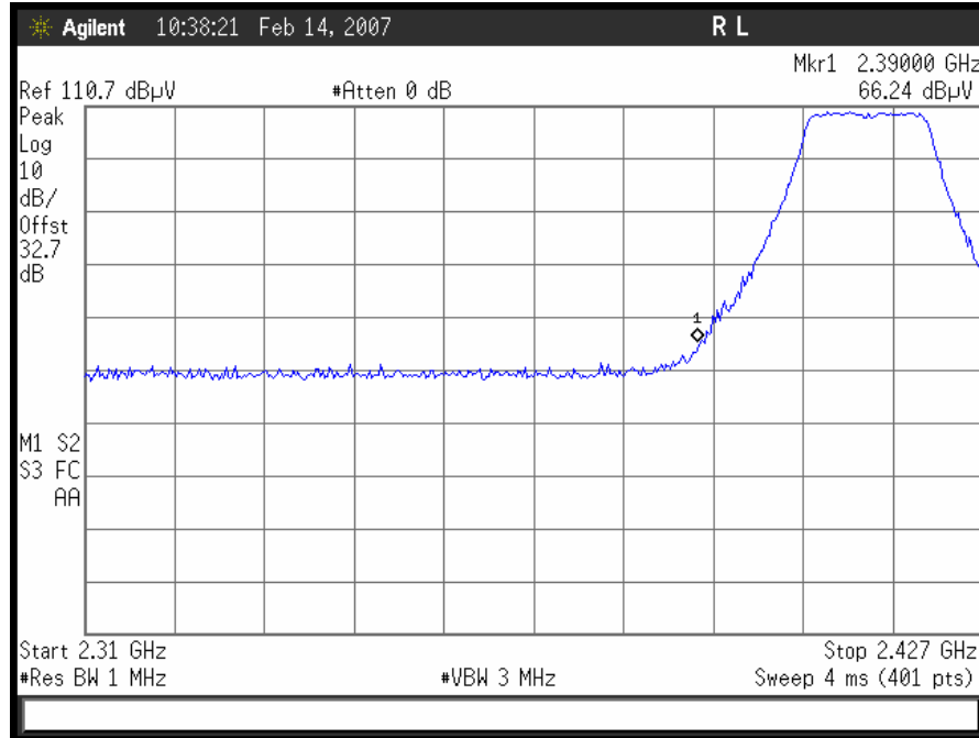
802.11/g radiated restricted band 2310- 2390 MHz Peak
