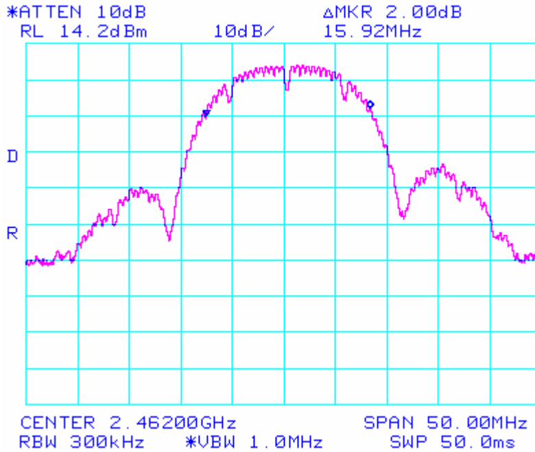
802.11/b High Ch Occupied Band Width 99%
