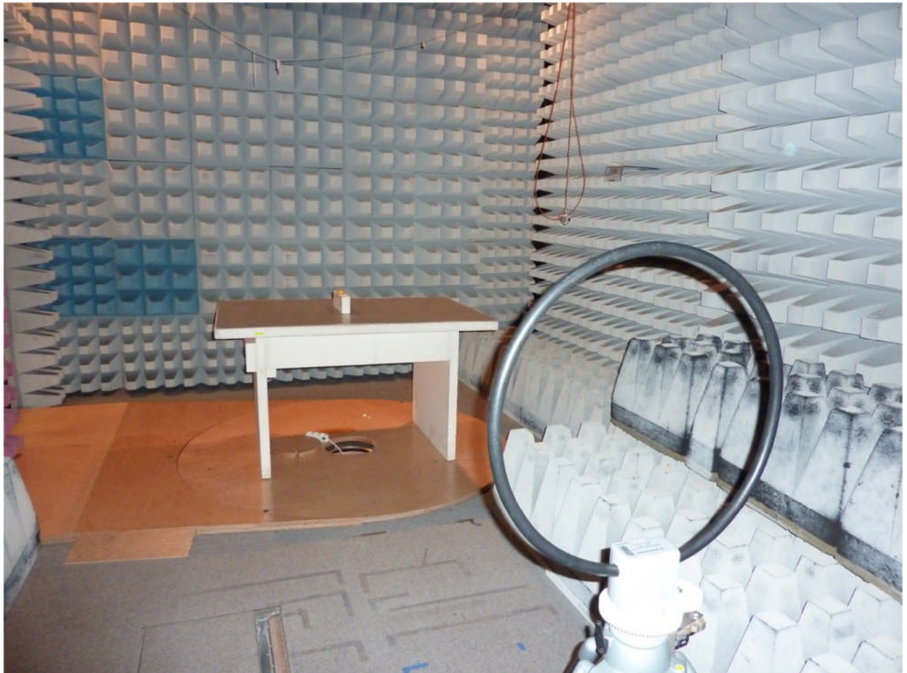
113539emi1.JPG: Test set-up preliminary radiated emission (H-Field)
