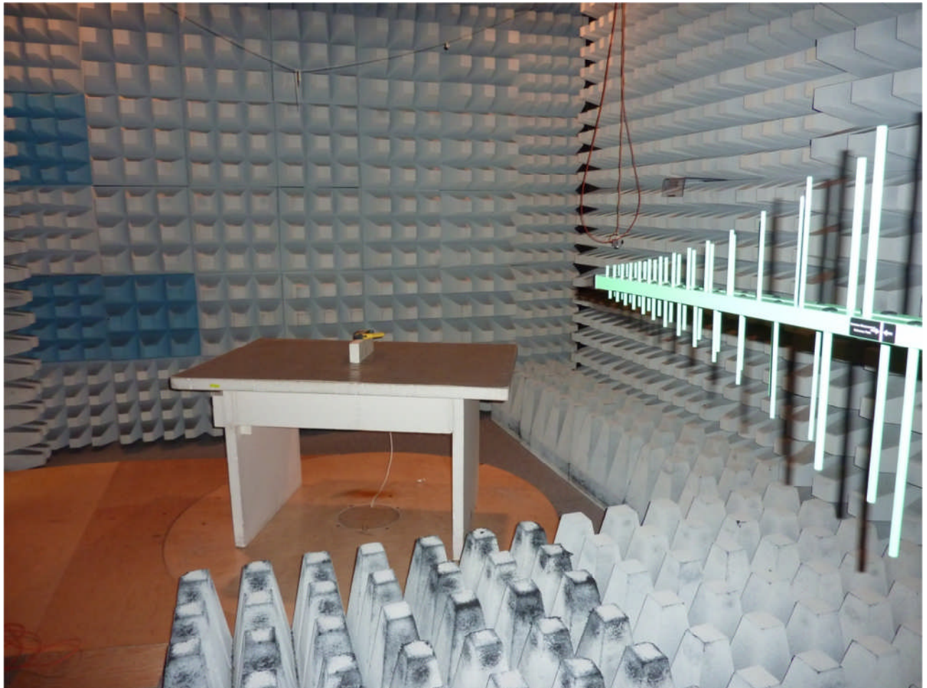
113539emi2.JPG: Test set-up radiated emission (E-Field)
