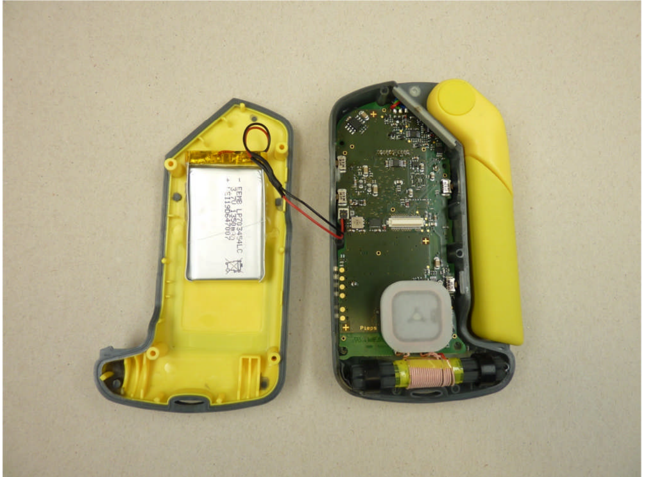
113539eut3.JPG: EUT, PCB front-view
