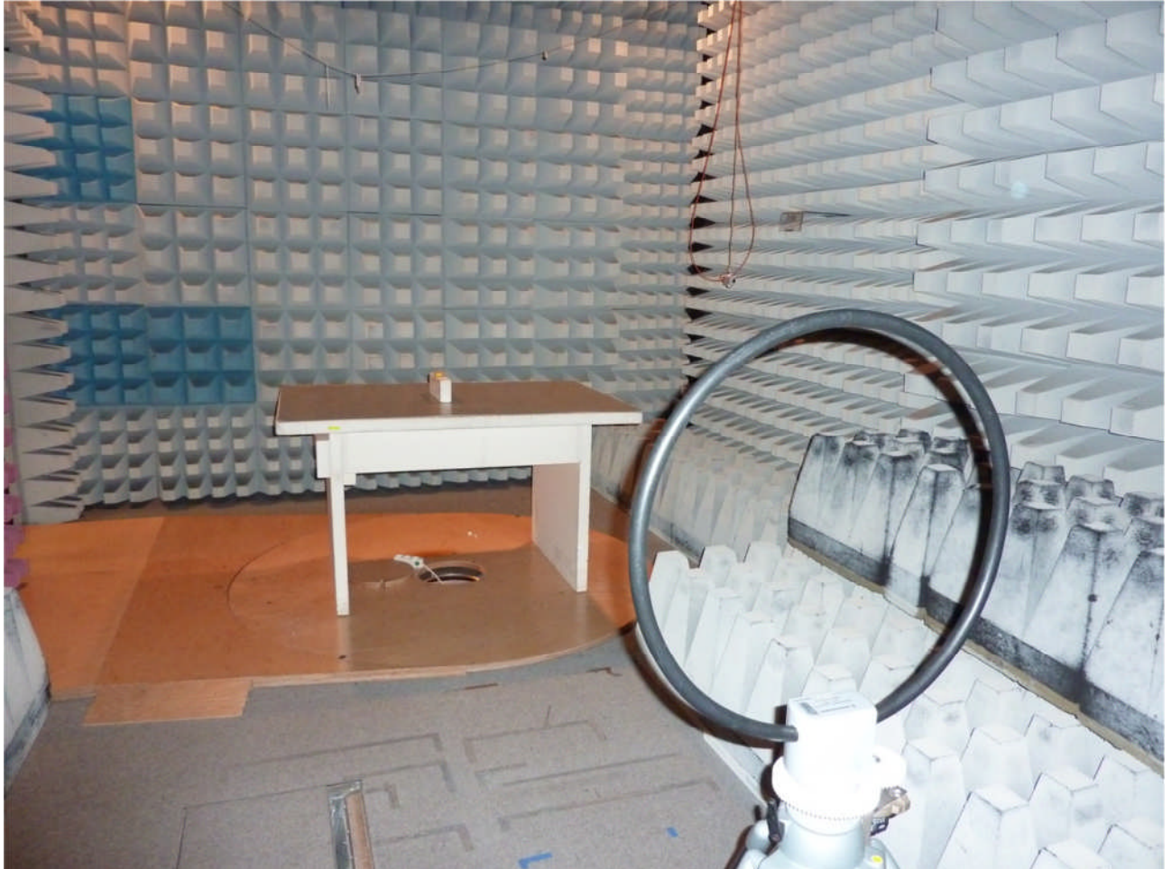
113540emi1.JPG: Test set-up preliminary radiated emission (H-Field)
