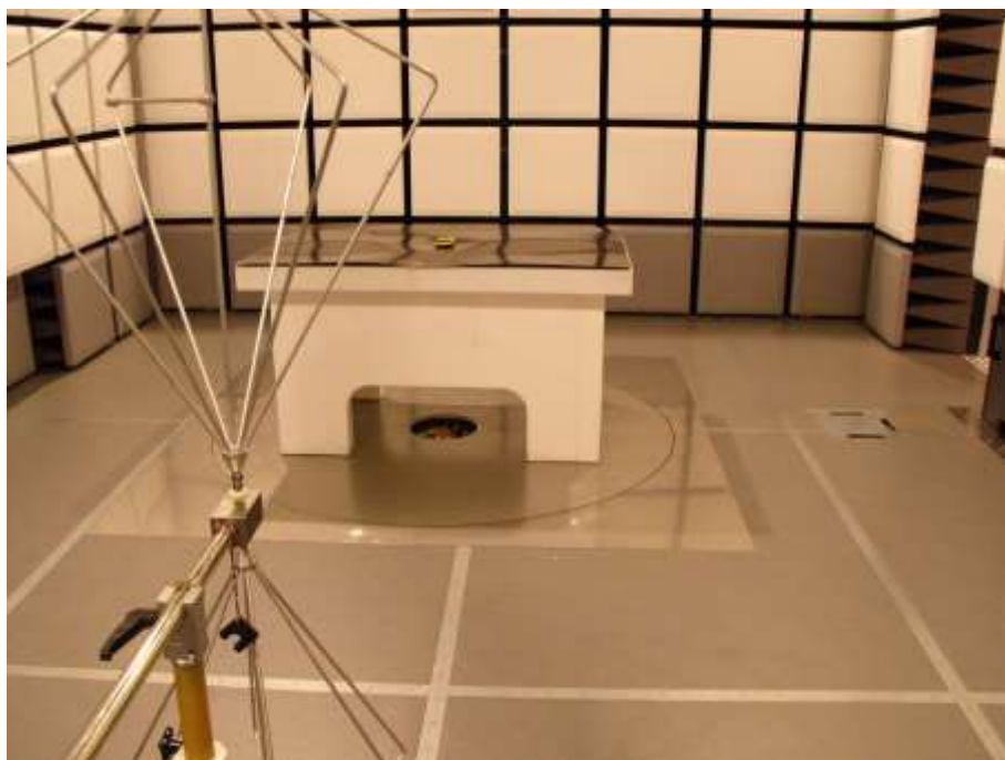
Figure 2: Radiated emission test, 30 MHz – 200 MHz - SAC
