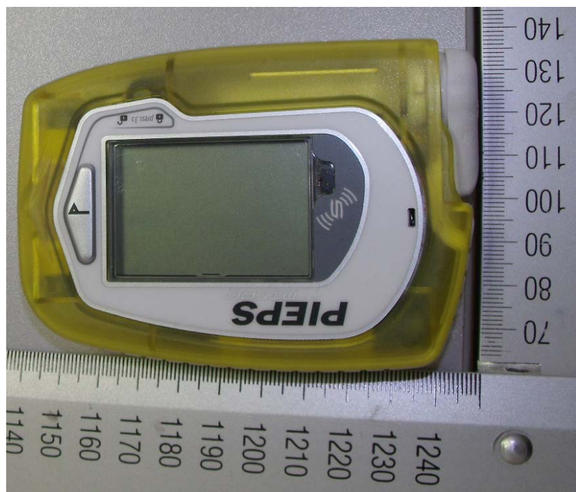
Figure 1: PIEPS MICRO – Top side
