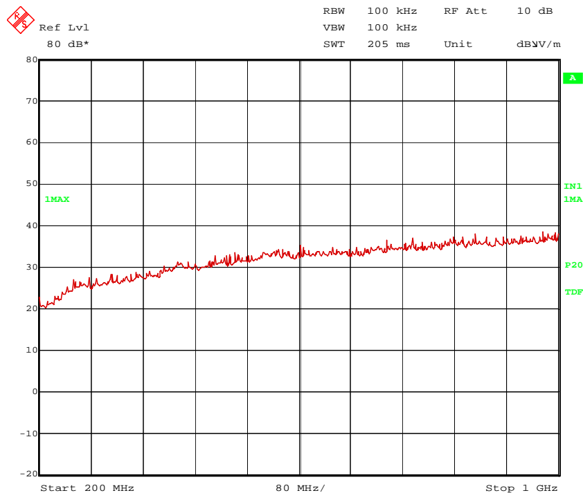
131845tx4.wmf: Spurious emissions from 200 MHz to 1000 MHz
