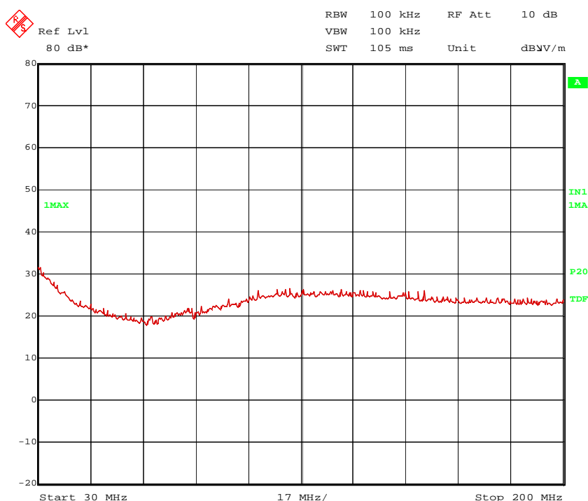
131845tx3.wmf: Spurious emissions from 30 MHz to 200 MHz
