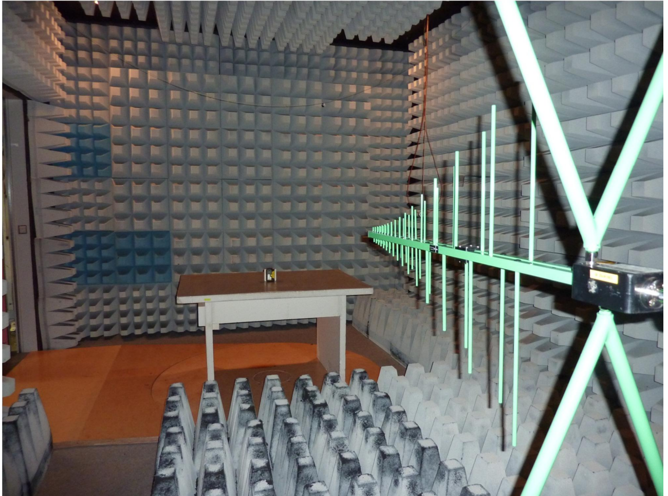
131845emi2.JPG: Test set-up radiated emission (E-Field)
