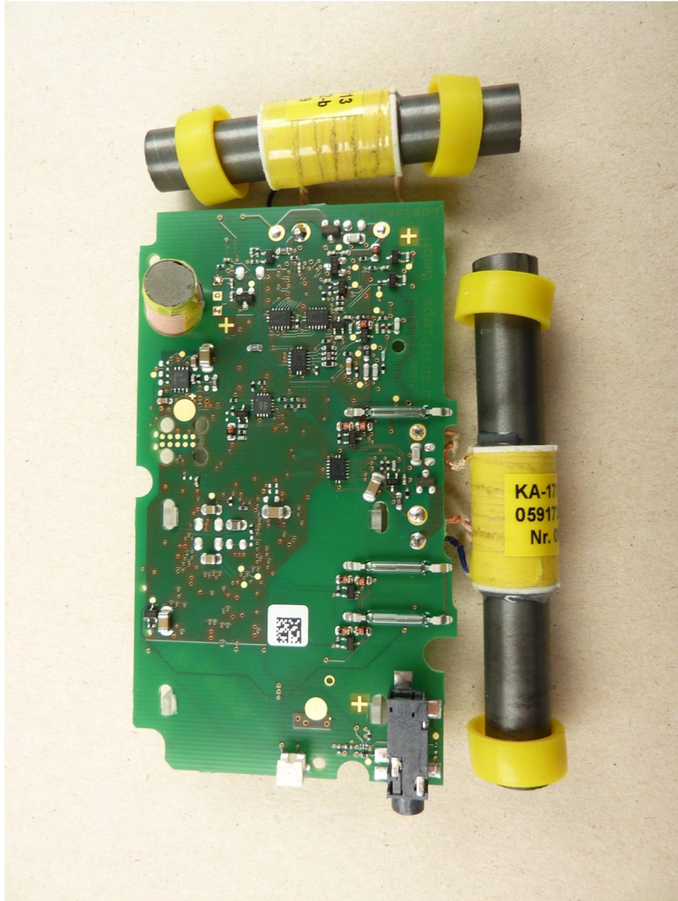
131845eut5.JPG: EUT, PCB rear-view
