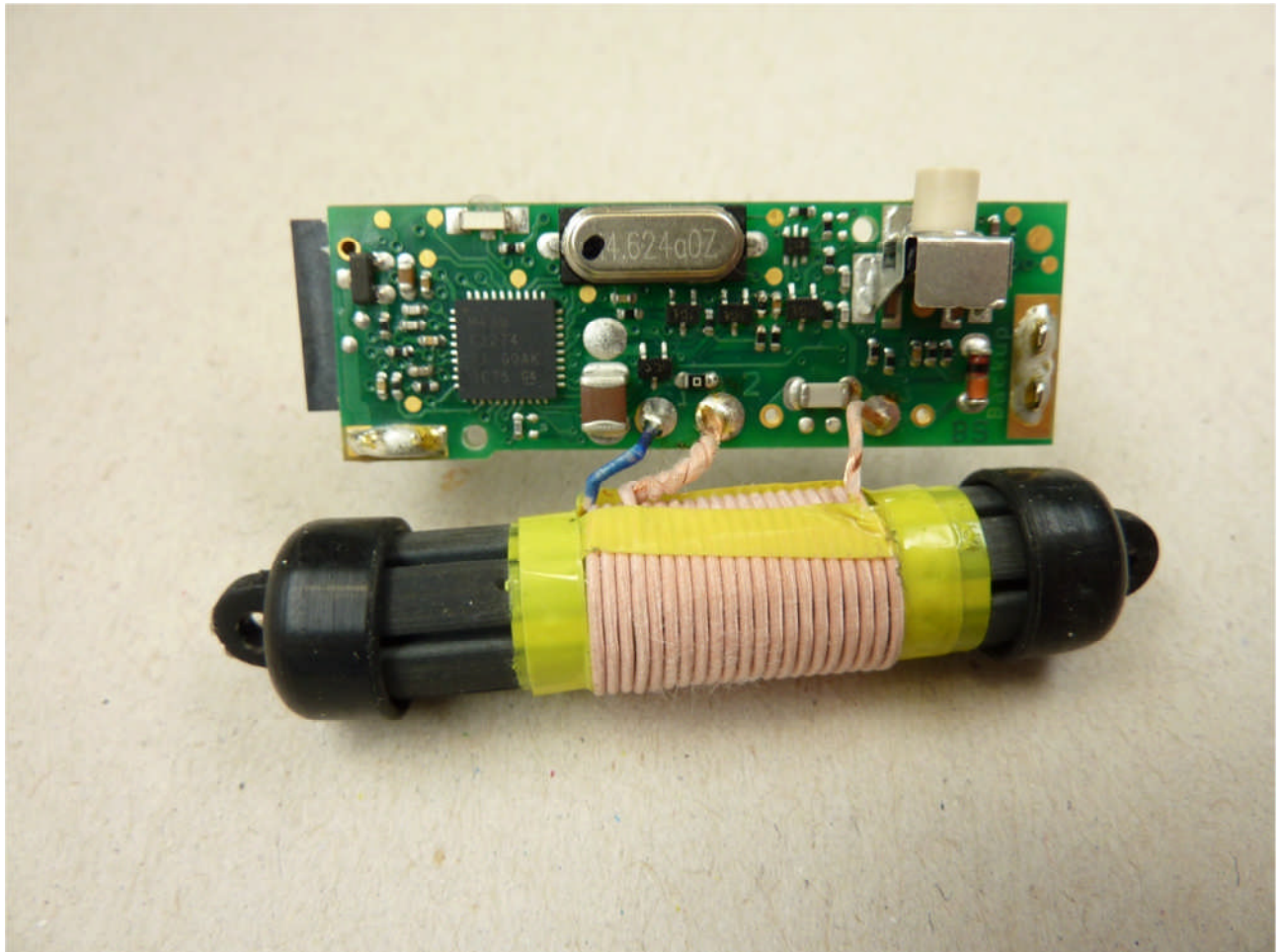
113943eut4.JPG: PCB, front view
