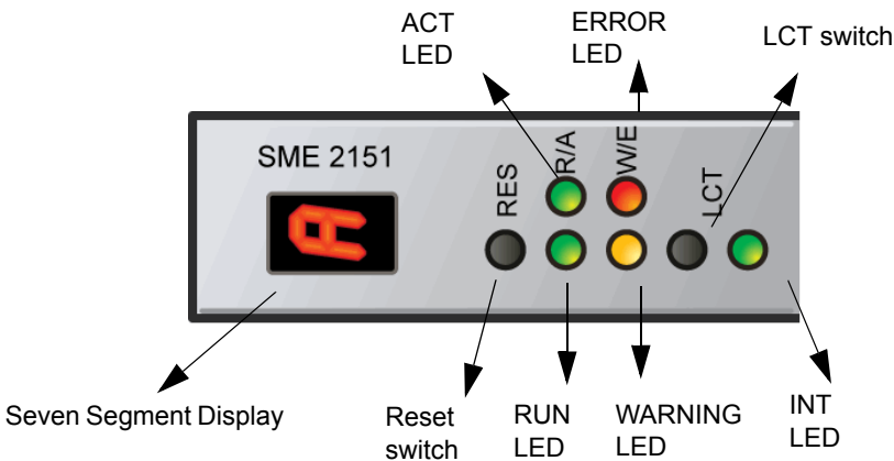
Figure 32 HiPath Wireless Controller's C2400 LED lights and switches
