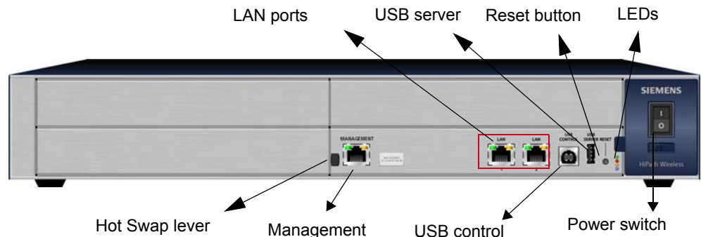
Figure 34 HiPath Wireless Controller C20 front panel
