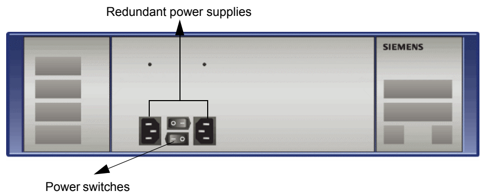
Figure 33 HiPath Wireless Controller C2400 back panel
