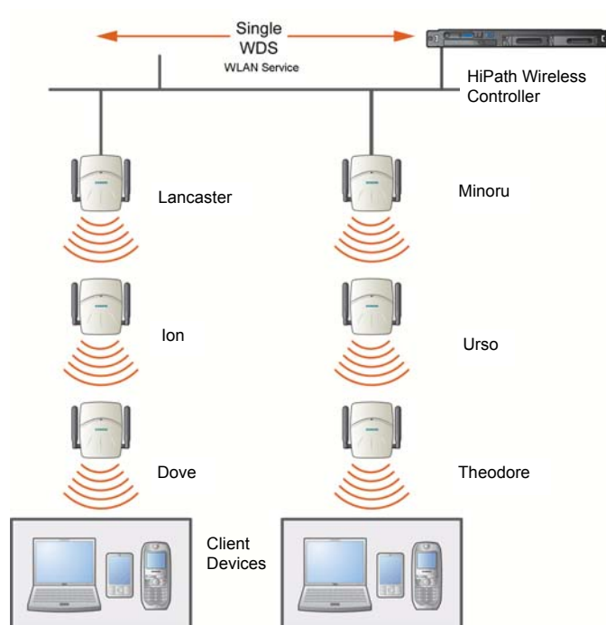
Figure 19 WDS setup with a single WDS WLAN Service
