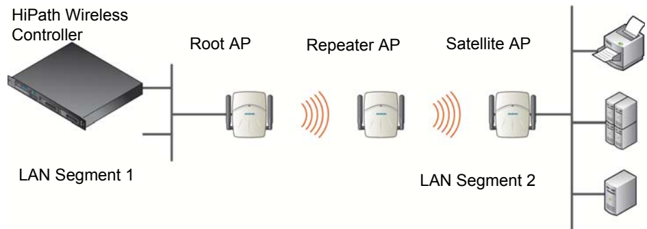
Figure 16 Wireless Bridge configuration
