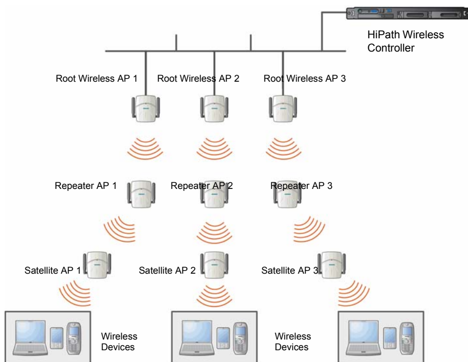
Figure 22 Multiple-root WDS topology
