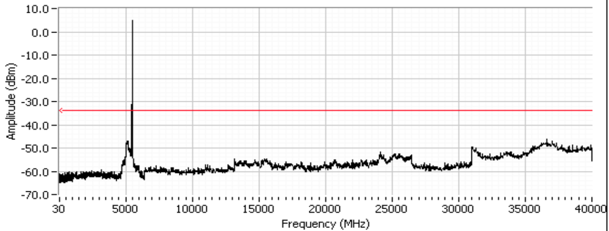
30 - 40,000MHz, Channel 100 @ 5500MHz
