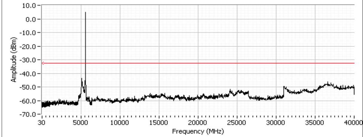
30 - 40,000MHz, Channel 120 @ 5600MHz
