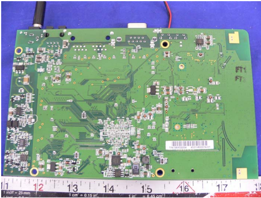
Board 3 – Component View
