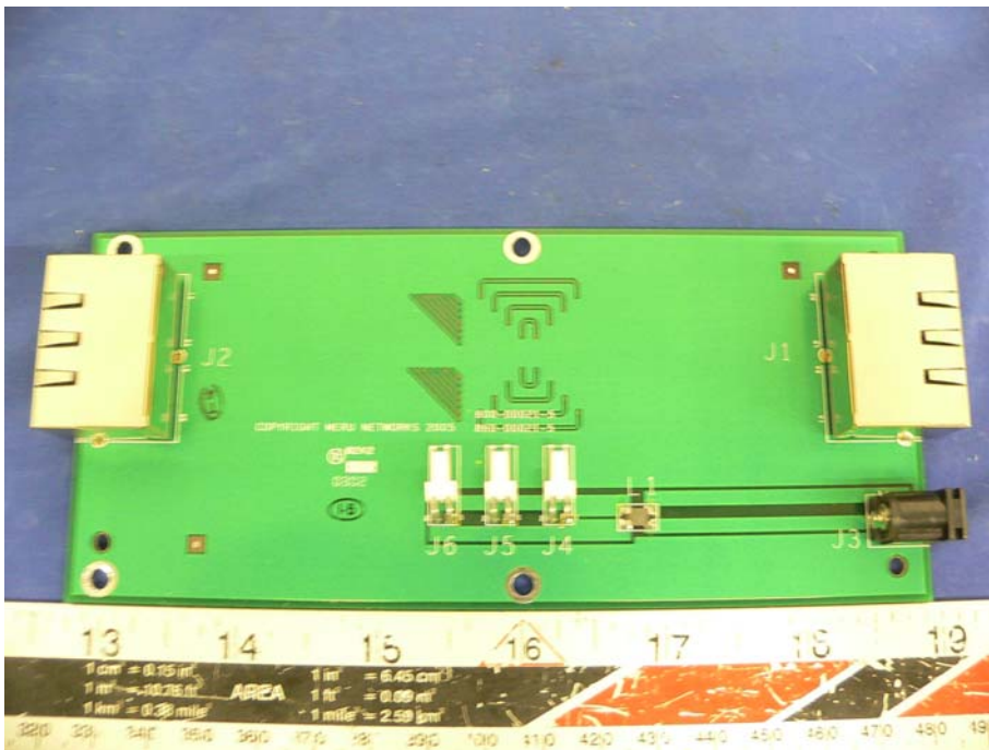
Board 4 – Component View
