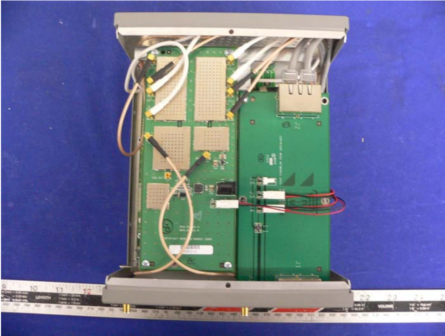
Antenna 1 Front View
