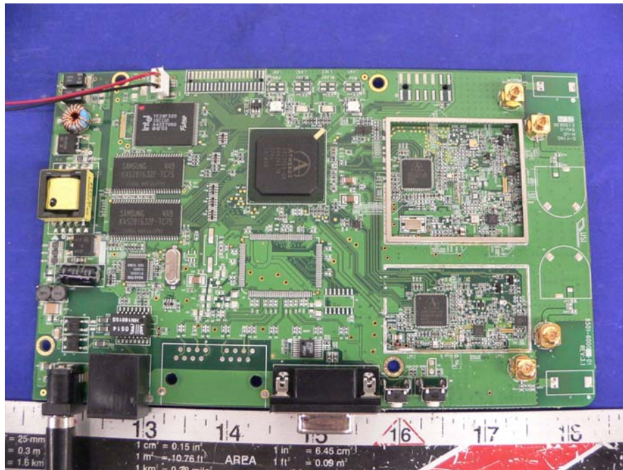
TX Board 1 – Component View 1
