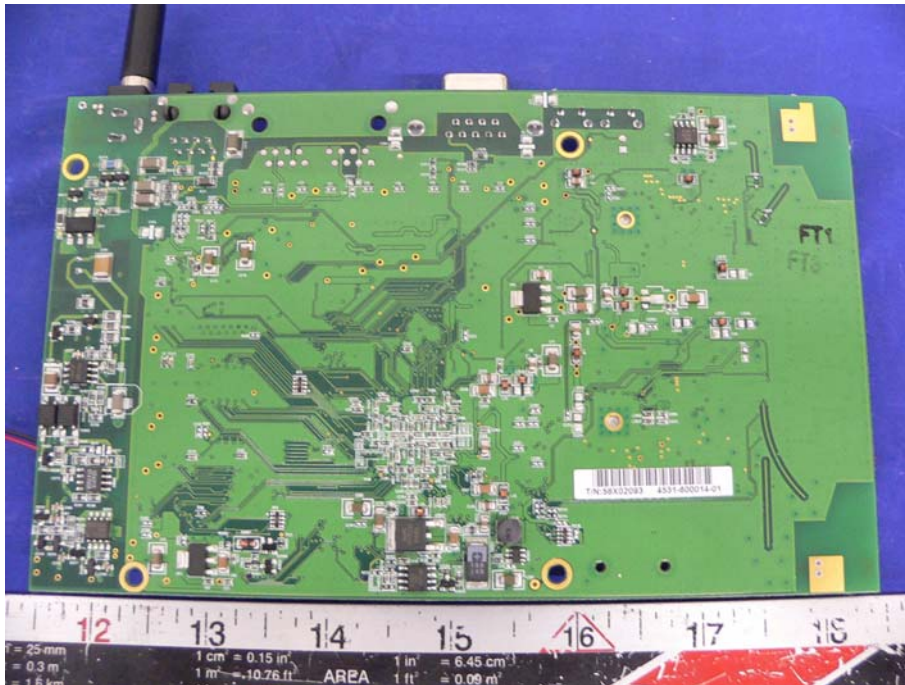
TX Board 1 – Solder View
