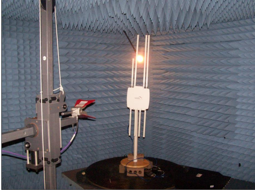
Photograph 5. Radiated Spurious Emissions, Test Setup, High Frequency, Omni Antenna
