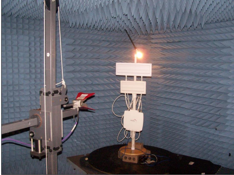
Photograph 3. Radiated Spurious Emissions, Test Setup, High Frequency, Panel Antenna
