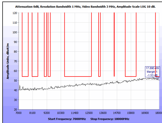
Plot 391. Co-location, Radiated Spurious Emissions, 802.11n 20 MHz, 2437 & 5300 MHz, 7 GHz – 18 GHz, Peak
