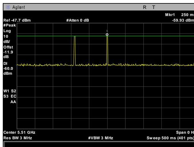
Plot 465. Radar Type 6 Calibration, 5510 MHz
