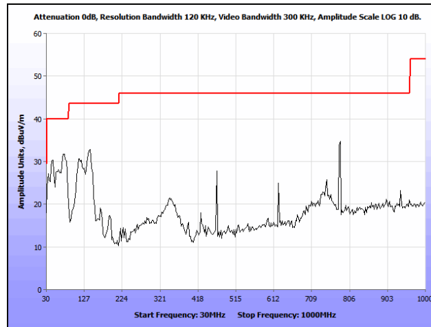
Plot 408. Co-location, Radiated Spurious Emissions, 802.11n 20 MHz, 2462 & 5580 MHz, 30 MHz – 1 GHz
