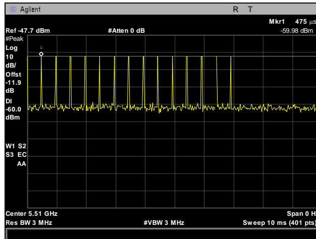
Plot 463. Radar Type 4 Calibration, 5510 MHz
