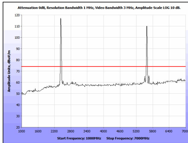
Plot 394. Co-location, Radiated Spurious Emissions, 802.11n 20 MHz, 2437 & 5580 MHz, 1 GHz – 7 GHz, Peak
