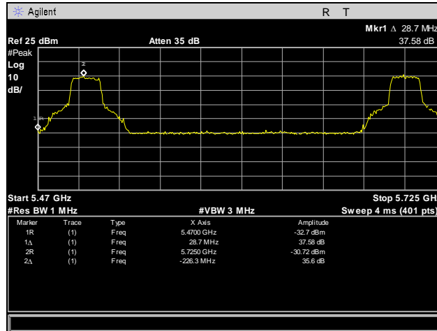
Plot 434. Frequency Stability, 5470 – 5725 MHz, 10°C, 120 V
