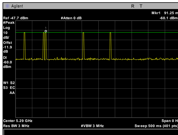
Plot 453. Radar Type 6 Calibration, 5290 MHz
