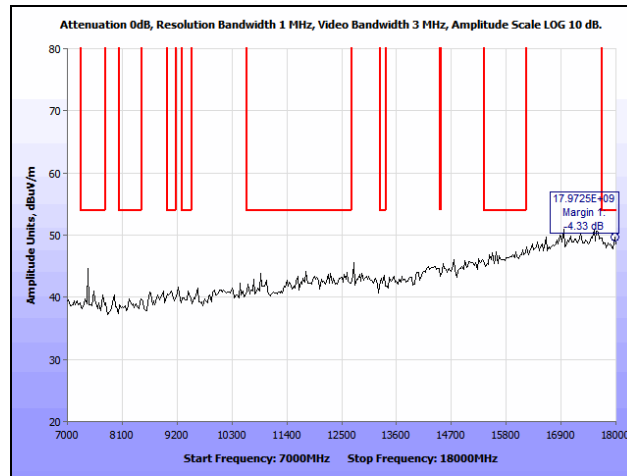
Plot 274. Radiated Spurious Emissions, 802.11n 40 MHz, Mid Channel, 7 GHz – 18 GHz, Internal, 5550 MHz
