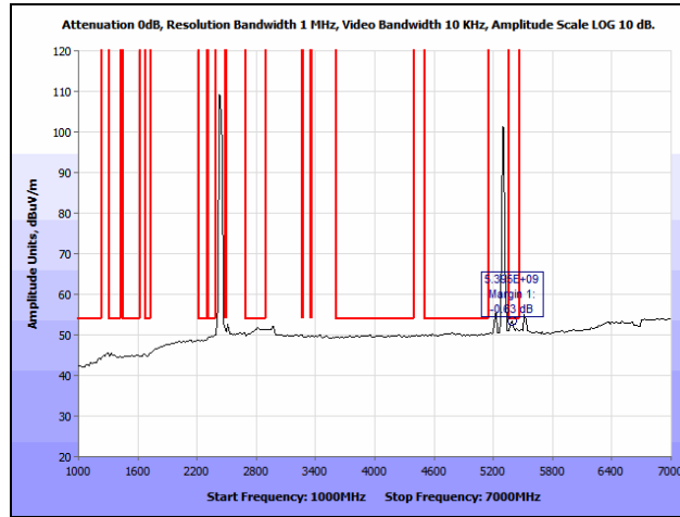
Plot 389. Co-location, Radiated Spurious Emissions, 802.11n 20 MHz, 2437 & 5300 MHz, 1 GHz – 7 GHz, Avg.
