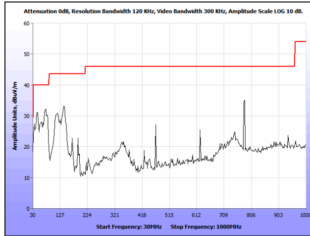
Plot 368. Co-location, Radiated Spurious Emissions, 802.11n 20 MHz, 2412 & 5200 MHz, 30 MHz – 1 GHz
