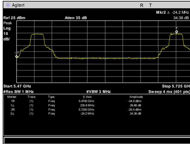
Plot 440. Frequency Stability, 5470 – 5725 MHz, 50°C, 120 V
