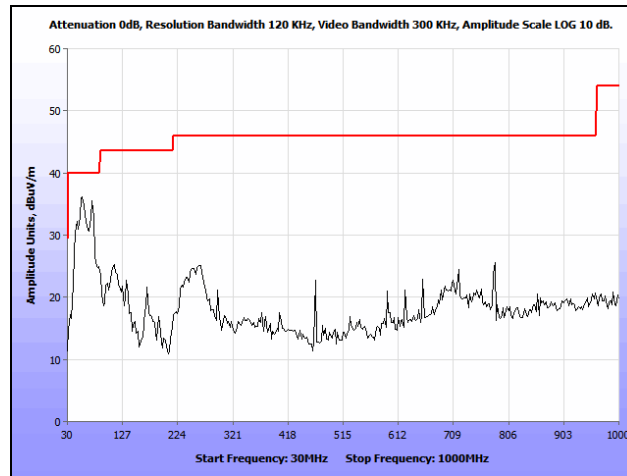
Plot 271. Radiated Spurious Emissions, 802.11n 40 MHz, Mid Channel, 30 MHz – 1 GHz, Internal, 5550 MHz
