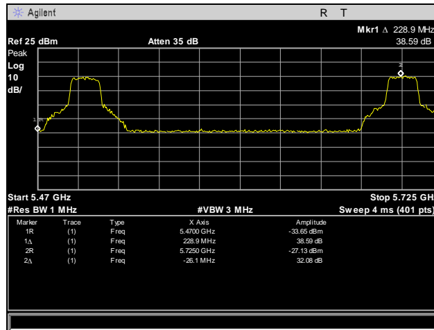
Plot 435. Frequency Stability, 5470 – 5725 MHz, 20°C, 108 V
