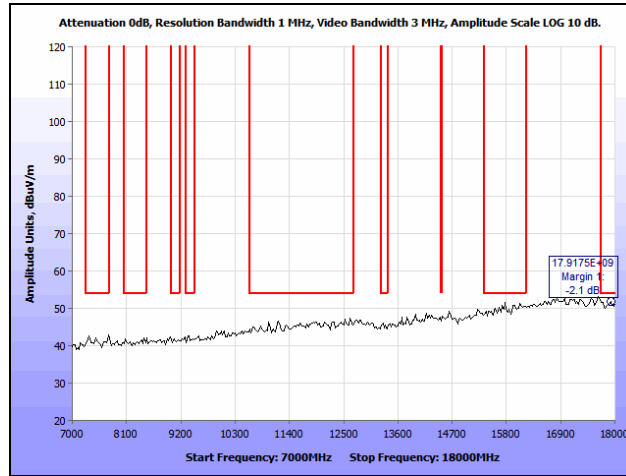
Plot 395. Co-location, Radiated Spurious Emissions, 802.11n 20 MHz, 2437 & 5580 MHz, 7 GHz – 18 GHz, Peak
