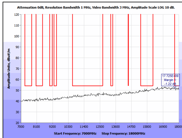
Plot 403. Co-location, Radiated Spurious Emissions, 802.11n 20 MHz, 2462 & 5200 MHz, 7 GHz – 18 GHz, Peak
