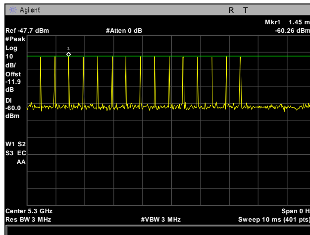
Plot 456. Radar Type 3 Calibration, 5300 MHz
