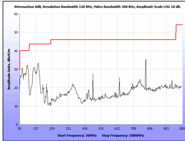
Plot 404. Co-location, Radiated Spurious Emissions, 802.11n 20 MHz, 2462 & 5300 MHz, 30 MHz – 1 GHz
