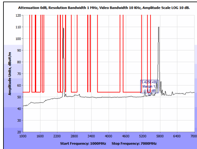
Plot 381. Co-location, Radiated Spurious Emissions, 802.11n 20 MHz, 2412 & 5785 MHz, 1 GHz – 7 GHz, Avg.
