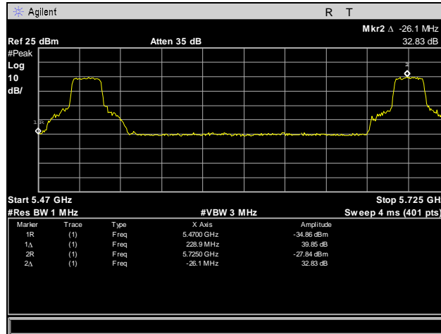
Plot 431. Frequency Stability, 5470 – 5725 MHz, -20°C, 120 V
