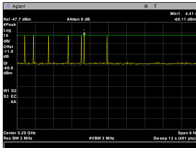
Plot 452. Radar Type 5 Calibration, 5290 MHz
