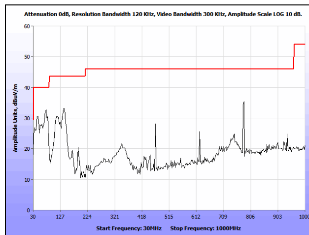
Plot 400. Co-location, Radiated Spurious Emissions, 802.11n 20 MHz, 2462 & 5200 MHz, 30 MHz – 1 GHz
