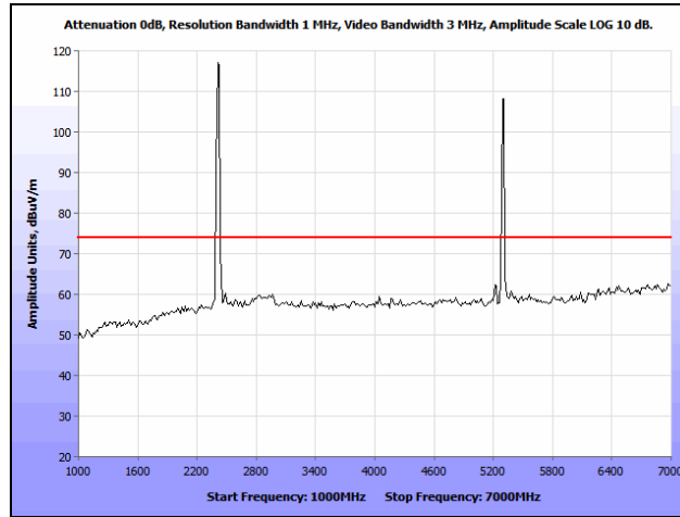
Plot 374. Co-location, Radiated Spurious Emissions, 802.11n 20 MHz, 2412 & 5300 MHz, 1 GHz – 7 GHz, Peak
