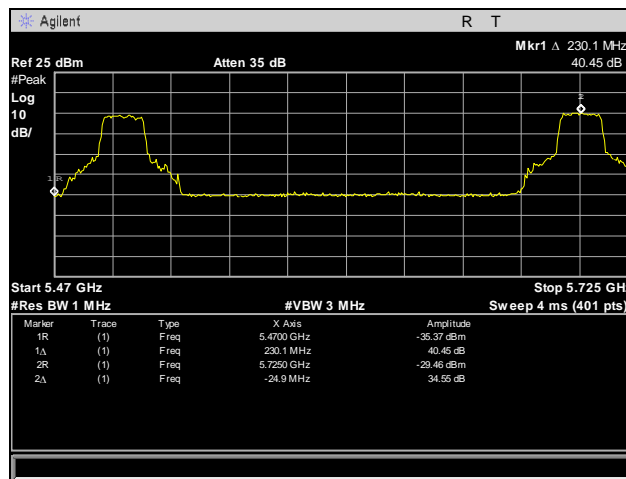
Plot 432. Frequency Stability, 5470 – 5725 MHz, -10°C, 120 V
