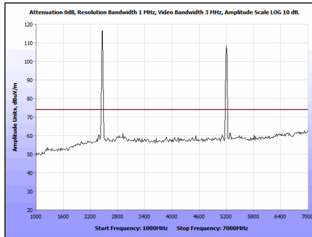
Plot 402. Co-location, Radiated Spurious Emissions, 802.11n 20 MHz, 2462 & 5200 MHz, 1 GHz – 7 GHz, Peak
