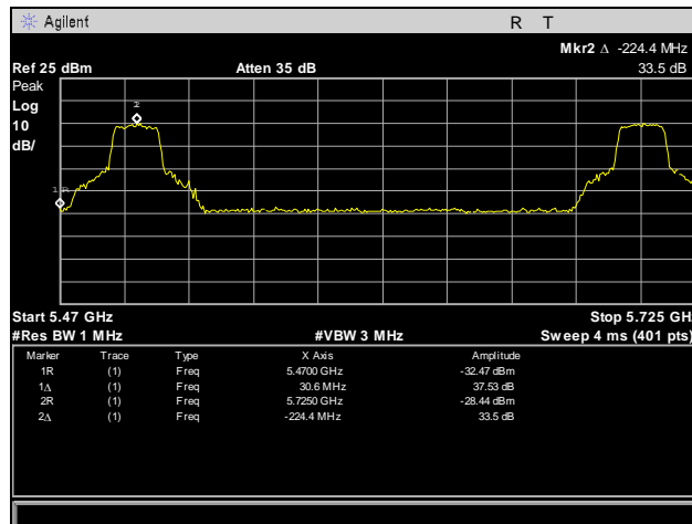
Plot 436. Frequency Stability, 5470 – 5725 MHz, 20°C, 120 V
