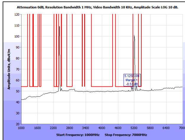
Plot 369. Co-location, Radiated Spurious Emissions, 802.11n 20 MHz, 2412 & 5200 MHz, 1 GHz – 7 GHz, Avg.
