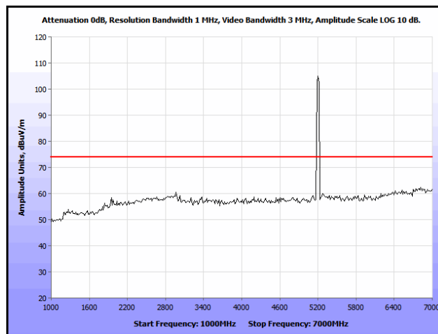
Plot 330. Co-location, Radiated Spurious Emissions, 802.11n 20 MHz, 5200 & 5200 MHz, 1 GHz – 7 GHz, Peak
