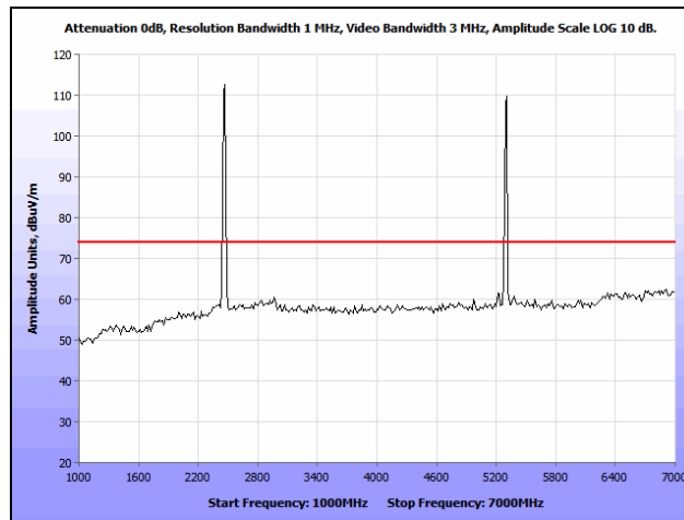
Plot 406. Co-location, Radiated Spurious Emissions, 802.11n 20 MHz, 2462 & 5300 MHz, 1 GHz – 7 GHz, Peak
