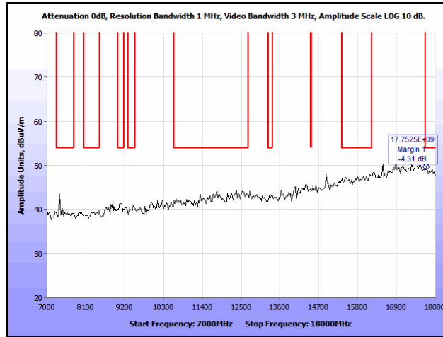
Plot 258. Radiated Spurious Emissions, 802.11n 20 MHz, Low Channel, 7 GHz – 18 GHz, Internal, 5500 MHz
