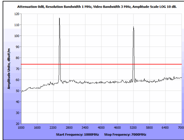
Plot 386. Co-location, Radiated Spurious Emissions, 802.11n 20 MHz, 2437 & 5200 MHz, 1 GHz – 7 GHz, Peak
