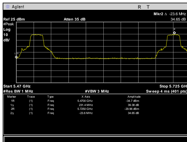
Plot 433. Frequency Stability, 5470 – 5725 MHz, 0°C, 120 V
