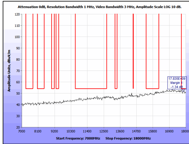
Plot 371. Co-location, Radiated Spurious Emissions, 802.11n 20 MHz, 2412 & 5200 MHz, 7 GHz – 18 GHz, Peak
