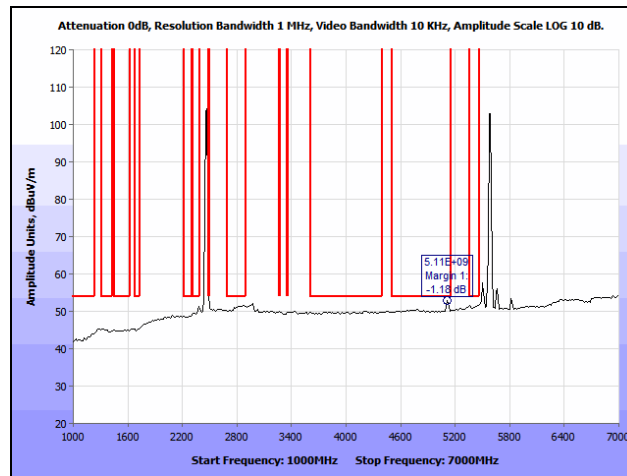
Plot 409. Co-location, Radiated Spurious Emissions, 802.11n 20 MHz, 2462 & 5580 MHz, 1 GHz – 7 GHz, Avg.
