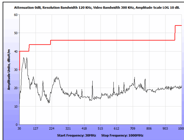
Plot 263. Radiated Spurious Emissions, 802.11n 20 MHz, High Channel, 30 MHz – 1 GHz, Internal, 5700 MHz
