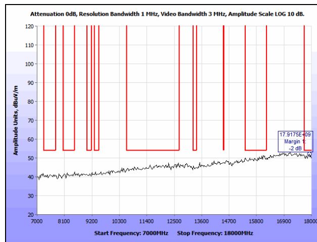
Plot 399. Co-location, Radiated Spurious Emissions, 802.11n 20 MHz, 2437 & 5785 MHz, 7 GHz – 18 GHz, Peak
