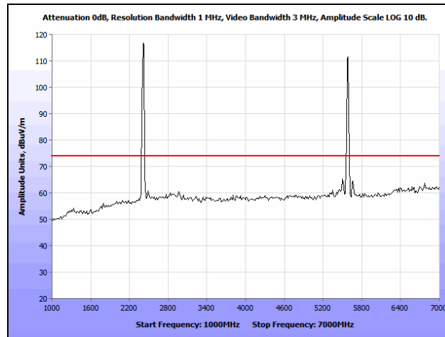
Plot 378. Co-location, Radiated Spurious Emissions, 802.11n 20 MHz, 2412 & 5580 MHz, 1 GHz – 7 GHz, Peak
