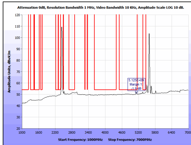
Plot 393. Co-location, Radiated Spurious Emissions, 802.11n 20 MHz, 2437 & 5580 MHz, 1 GHz – 7 GHz, Avg.
