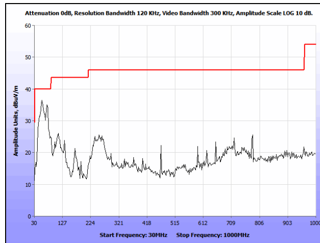
Plot 275. Radiated Spurious Emissions, 802.11n 40 MHz, High Channel, 30 MHz – 1 GHz, Internal, 5670 MHz
