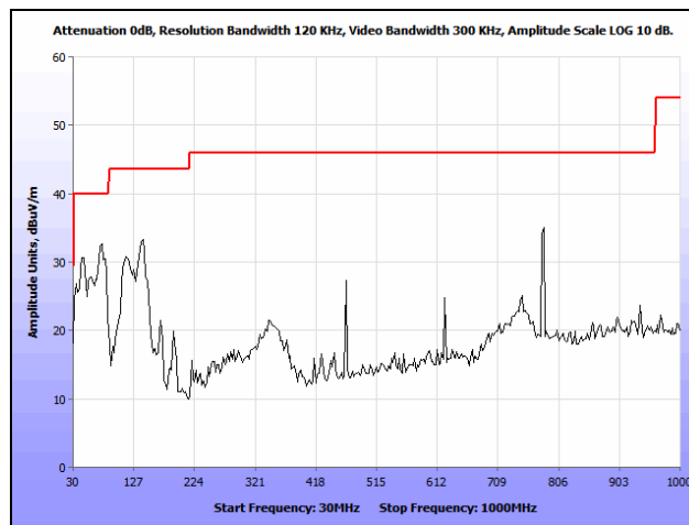
Plot 412. Co-location, Radiated Spurious Emissions, 802.11n 20 MHz, 2462 & 5785 MHz, 30 MHz – 1 GHz
