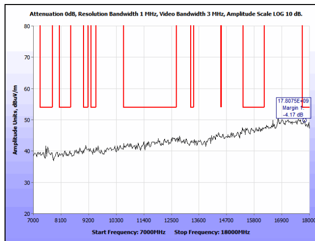
Plot 286. Radiated Spurious Emissions, 802.11n 80 MHz, 7 GHz – 18 GHz, Peak, Internal, 5610 MHz
