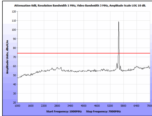
Plot 261. Radiated Spurious Emissions, 802.11n 20 MHz, Mid Channel, 1 GHz – 7 GHz, Peak, Internal, 5580 MHz
