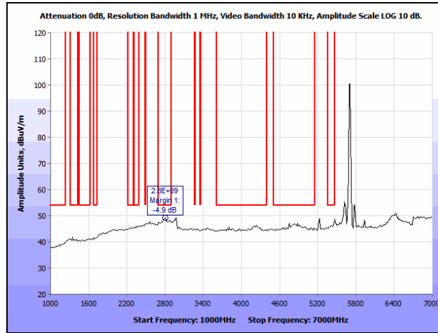
Plot 264. Radiated Spurious Emissions, 802.11n 20 MHz, High Channel, 1 GHz – 7 GHz, Avg., Internal, 5700 MHz
