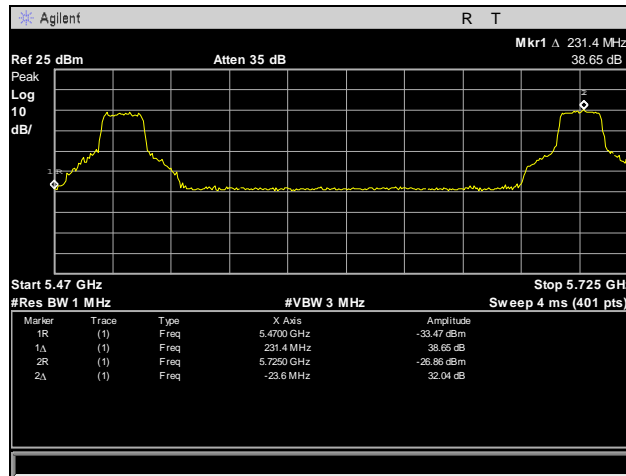
Plot 441. Frequency Stability, 5470 – 5725 MHz, 55°C, 120 V
