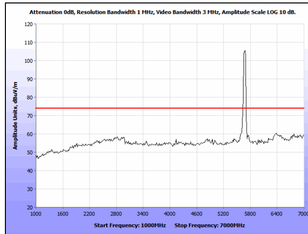
Plot 277. Radiated Spurious Emissions, 802.11n 40 MHz, High Channel, 1 GHz – 7 GHz, Peak, Internal, 5670 MHz
