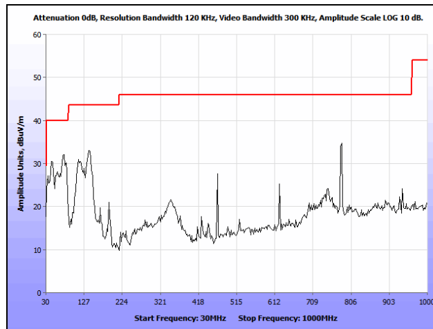
Plot 388. Co-location, Radiated Spurious Emissions, 802.11n 20 MHz, 2437 & 5300 MHz, 30 MHz – 1 GHz
