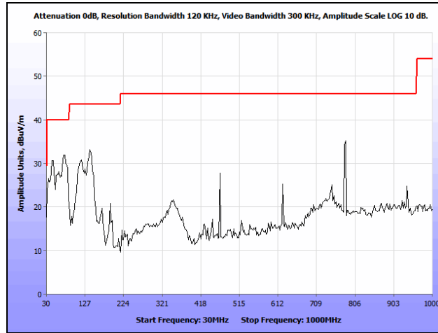
Plot 392. Co-location, Radiated Spurious Emissions, 802.11n 20 MHz, 2437 & 5580 MHz, 30 MHz – 1 GHz
