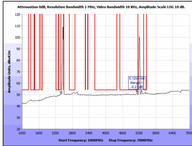
Plot 401. Co-location, Radiated Spurious Emissions, 802.11n 20 MHz, 2462 & 5200 MHz, 1 GHz – 7 GHz, Avg.
