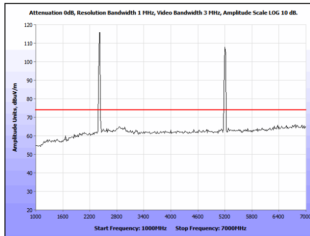
Plot 370. Co-location, Radiated Spurious Emissions, 802.11n 20 MHz, 2412 & 5200 MHz, 1 GHz – 7 GHz, Peak
