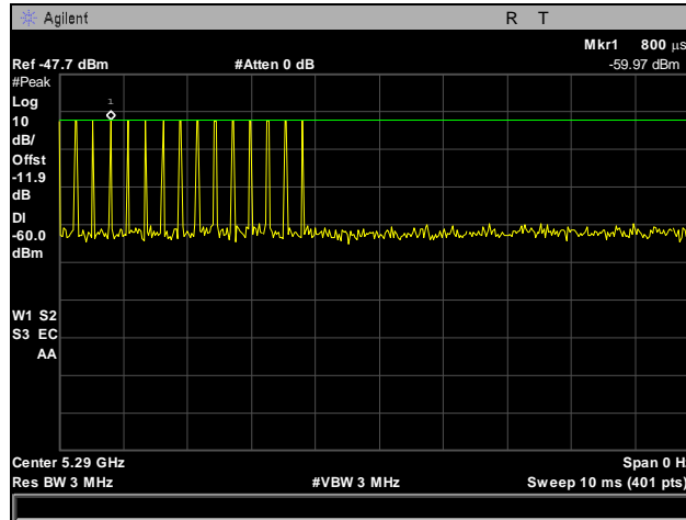
Plot 451. Radar Type 4 Calibration, 5290 MHz
