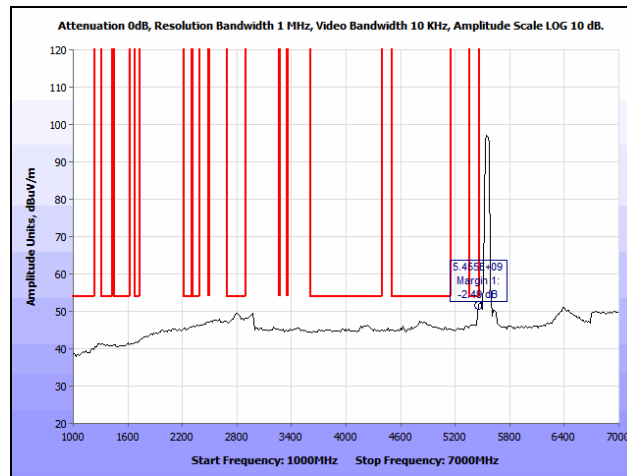
Plot 272. Radiated Spurious Emissions, 802.11n 40 MHz, Mid Channel, 1 GHz – 7 GHz, Avg., Internal, 5550 MHz
