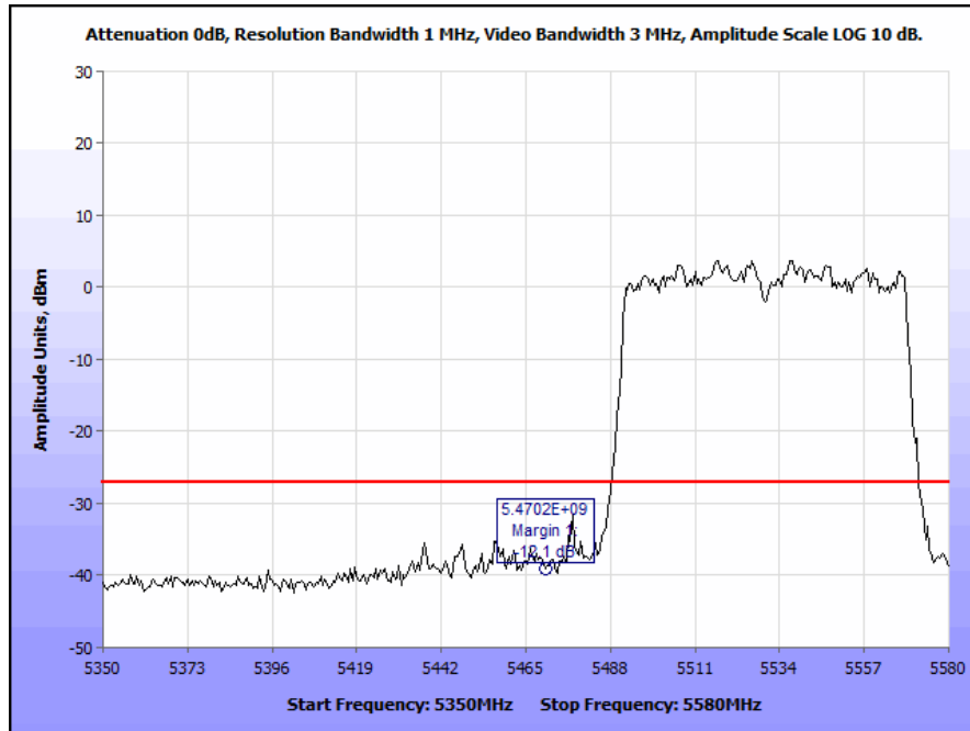
Plot 301. Radiated Band Edge 802.11n 80 MHz, 5530 MHz, Internal (Band Edge @ 5470 MHz)
