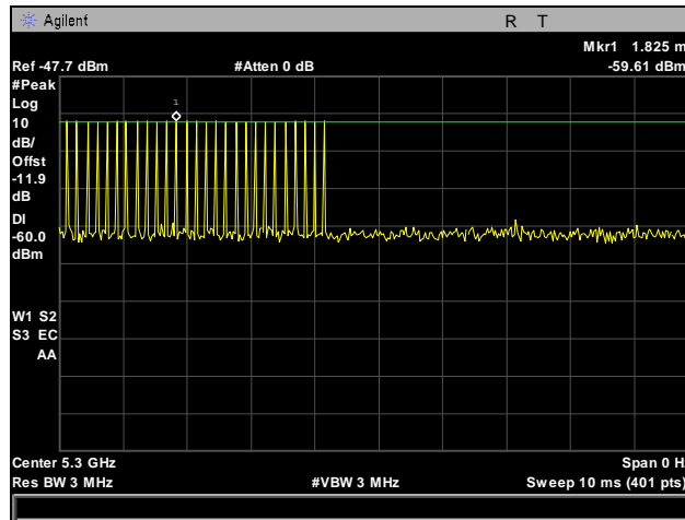
Plot 455. Radar Type 2 Calibration, 5300 MHz
