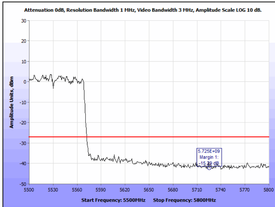
Plot 302. Radiated Band Edge 802.11n 80 MHz, 5530 MHz, Internal (Band Edge @ 5725 MHz)
