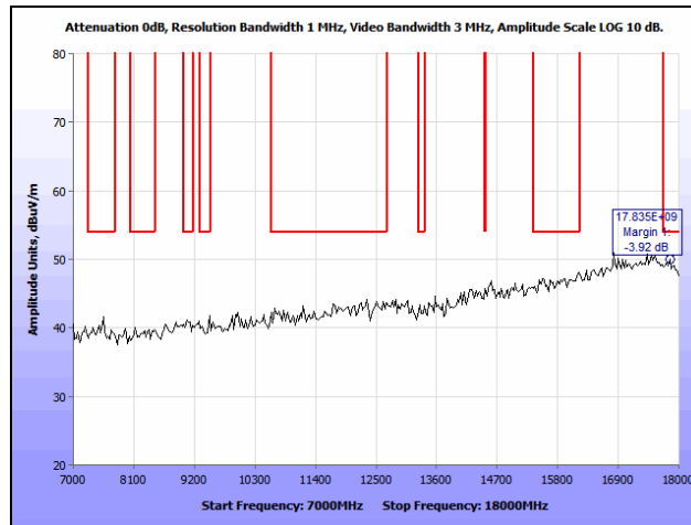
Plot 262. Radiated Spurious Emissions, 802.11n 20 MHz, Mid Channel, 7 GHz – 18 GHz, Internal, 5580 MHz
