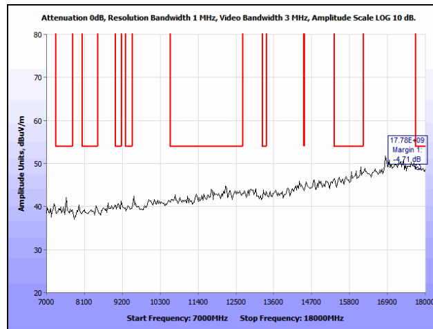
Plot 278. Radiated Spurious Emissions, 802.11n 40 MHz, High Channel, 7 GHz – 18 GHz, Internal, 5670 MHz
