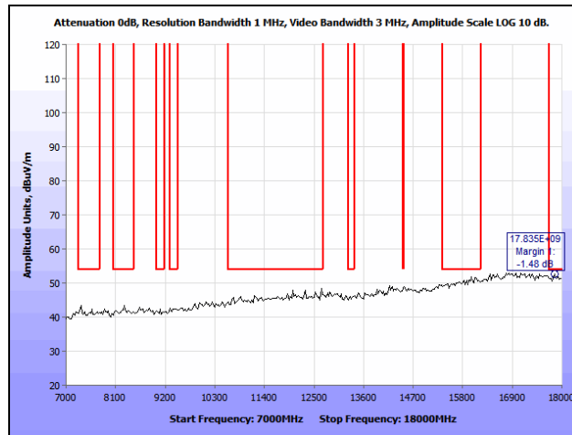
Plot 387. Co-location, Radiated Spurious Emissions, 802.11n 20 MHz, 2437 & 5200 MHz, 7 GHz – 18 GHz, Peak
