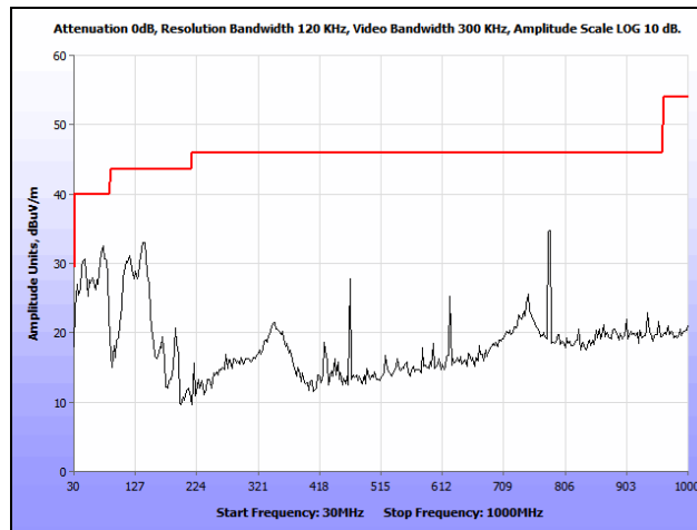
Plot 376. Co-location, Radiated Spurious Emissions, 802.11n 20 MHz, 2412 & 5580 MHz, 30 MHz – 1 GHz
