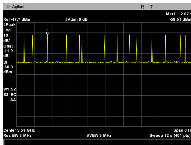
Plot 464. Radar Type 5 Calibration, 5510 MHz
