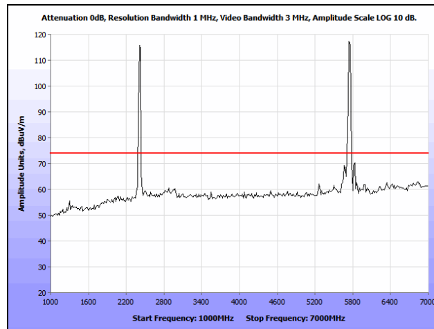
Plot 382. Co-location, Radiated Spurious Emissions, 802.11n 20 MHz, 2412 & 5785 MHz, 1 GHz – 7 GHz, Peak
