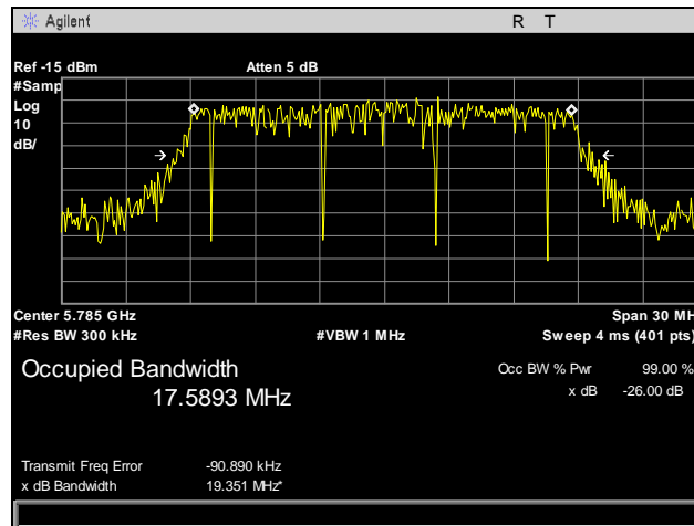
Plot 41. 99% Occupied Bandwidth, 802.11n 20 MHz, Port 3, Mid Channel
