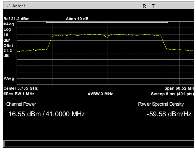
Plot 61. RF Power Output, Low Channel, 802.11n 40 MHz, Port 1
