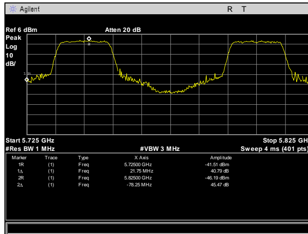
Plot 179. Frequency Stability, 5725 – 5825 MHz, 20°C, 120 V
