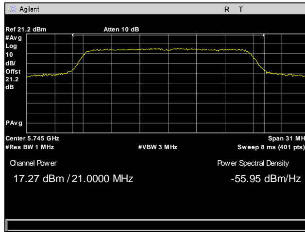
Plot 52. RF Power Output, Low Channel, 802.11n 20 MHz, Port 1
