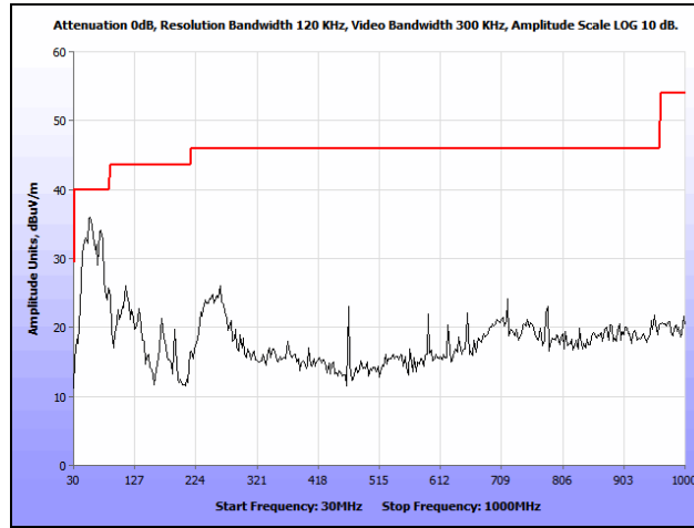
Plot 144. Radiated Spurious Emissions, 802.11n 80 MHz, 30 MHz – 1 GHz, Internal
