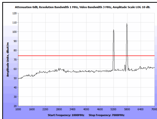
Plot 158. Co-location, Radiated Spurious Emissions, PIFA, 802.11n 20 MHz, 5200 & 5785 MHz, 1 GHz – 7 GHz, Peak
