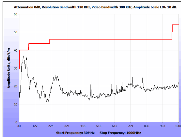
Plot 132. Radiated Spurious Emissions, 802.11n 20 MHz, High Channel, 30 MHz – 1 GHz, Internal
