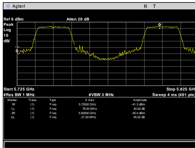
Plot 180. Frequency Stability, 5725 – 5825 MHz, 20°C, 132 V
