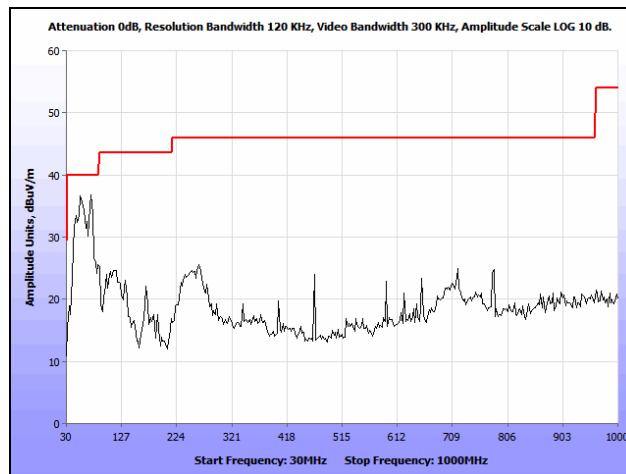
Plot 120. Radiated Spurious Emissions, 802.11a, High Channel, 30 MHz – 1 GHz, Internal
