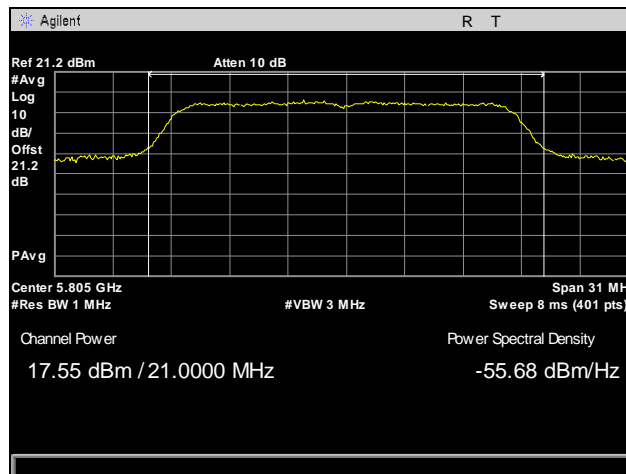
Plot 51. RF Power Output, High Channel, 802.11a
