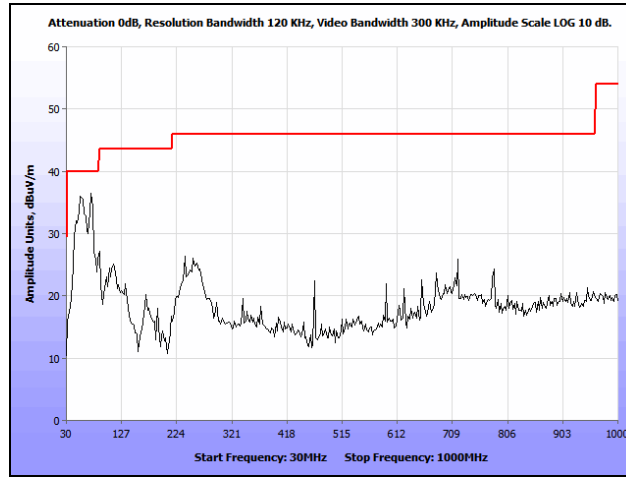
Plot 136. Radiated Spurious Emissions, 802.11n 40 MHz, Low Channel, 30 MHz – 1 GHz, Internal
