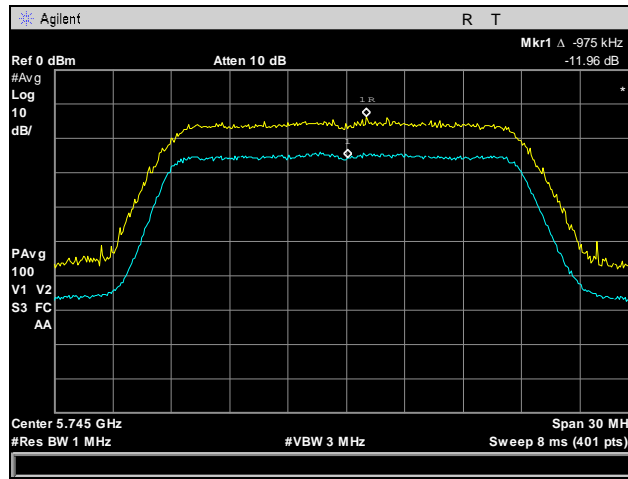
Plot 100. Peak Excursion Ratio, Low Channel, 802.11n 20 MHz, Port 3
