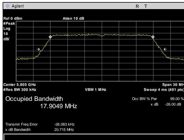
Plot 18. 26 dB Occupied Bandwidth, 802.11n 20 MHz, Port 1, High Channel
