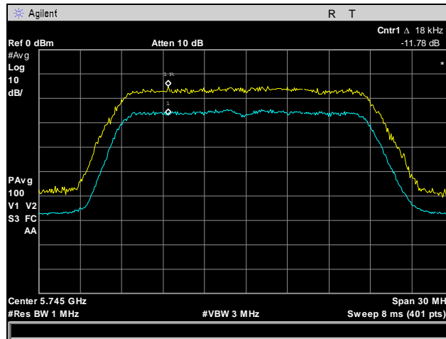
Plot 91. Peak Excursion Ratio, Low Channel, 802.11a
