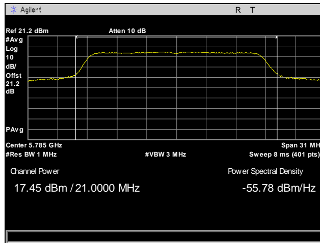
Plot 53. RF Power Output, Mid Channel, 802.11n 20 MHz, Port 1
