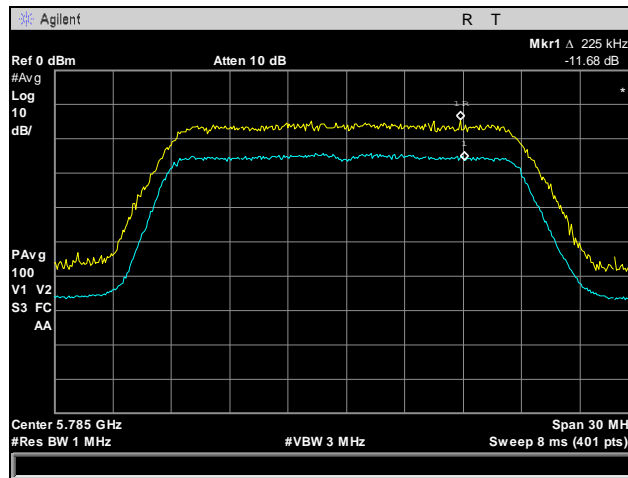
Plot 101. Peak Excursion Ratio, Mid Channel, 802.11n 20 MHz, Port 3
