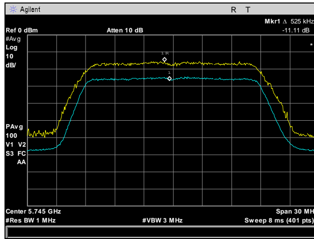
Plot 94. Peak Excursion Ratio, Low Channel, 802.11n 20 MHz, Port 1
