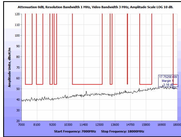
Plot 171. Co-location, Radiated Spurious Emissions, PIFA, 802.11n 20 MHz, 5785 & 5785 MHz, 7 GHz – 18 GHz, Peak
