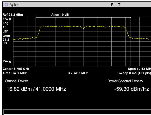
Plot 62. RF Power Output, High Channel, 802.11n 40 MHz, Port 1
