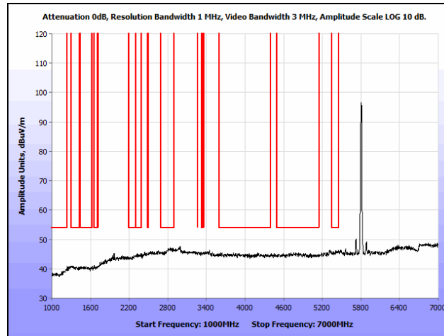
Plot 133. Radiated Spurious Emissions, 802.11n 20 MHz, High Channel, 1 GHz – 7 GHz, Avg., Internal
