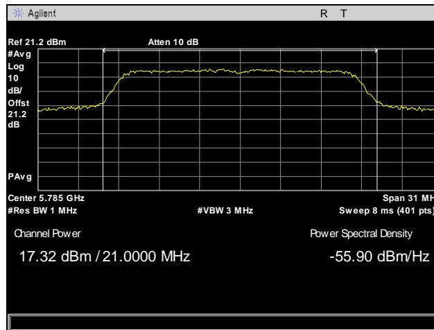
Plot 50. RF Power Output, Mid Channel, 802.11a
