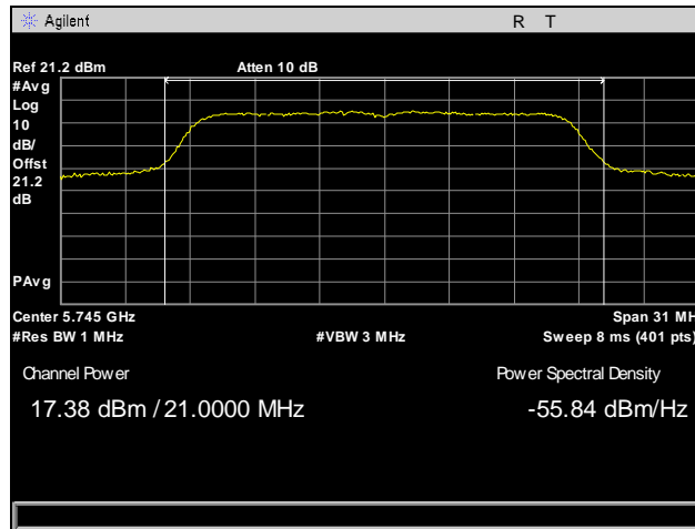
Plot 49. RF Power Output, Low Channel, 802.11a
