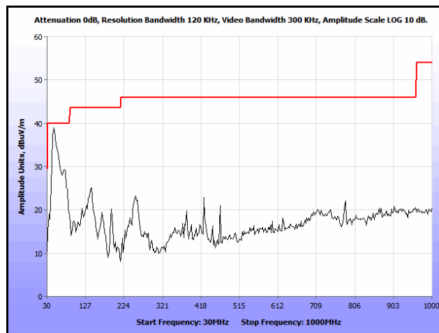
Plot 164. Co-location, Radiated Spurious Emissions, PIFA, 802.11n 20 MHz, 5580 & 5785 MHz, 30 MHz – 1 GHz
