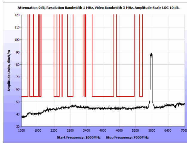
Plot 145. Radiated Spurious Emissions, 802.11n 80 MHz, 1 GHz – 7 GHz, Avg., Internal
