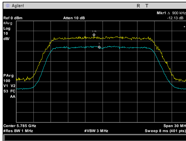
Plot 92. Peak Excursion Ratio, Mid Channel, 802.11a
