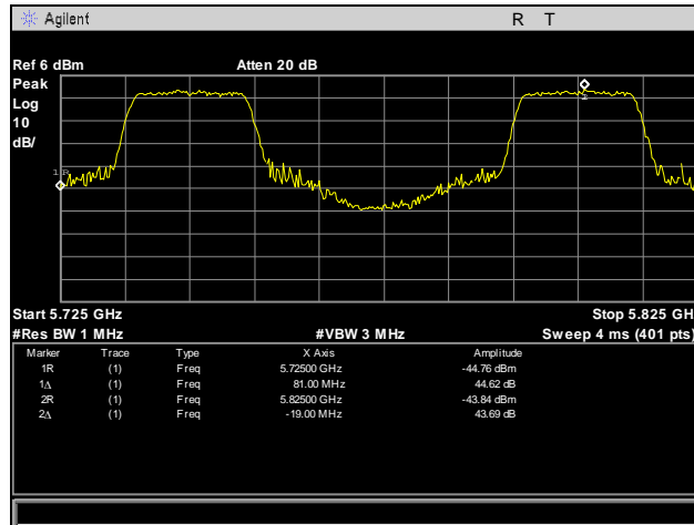
Plot 178. Frequency Stability, 5725 – 5825 MHz, 20°C, 108 V
