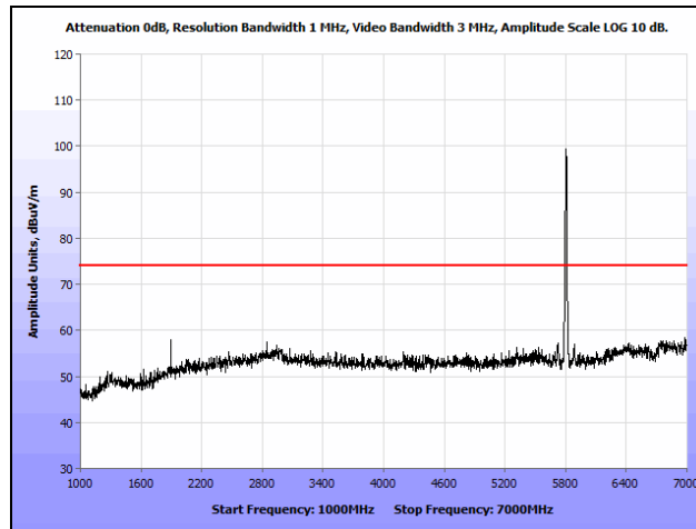
Plot 122. Radiated Spurious Emissions, 802.11a, High Channel, 1 GHz – 7 GHz, Peak, Internal
