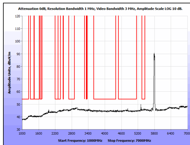
Plot 141. Radiated Spurious Emissions, 802.11n 40 MHz, High Channel, 1 GHz – 7 GHz, Avg., Internal
