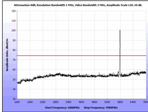
Plot 118. Radiated Spurious Emissions, 802.11a, Mid Channel, 1 GHz – 7 GHz, Peak, Internal
