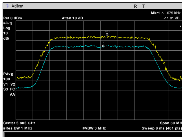
Plot 93. Peak Excursion Ratio, High Channel, 802.11a
