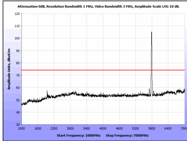
Plot 130. Radiated Spurious Emissions, 802.11n 20 MHz, Mid Channel, 1 GHz – 7 GHz, Peak, Internal
