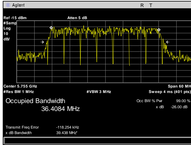
Plot 45. 99% Occupied Bandwidth, 802.11n 40 MHz, Port 2, Low Channel
