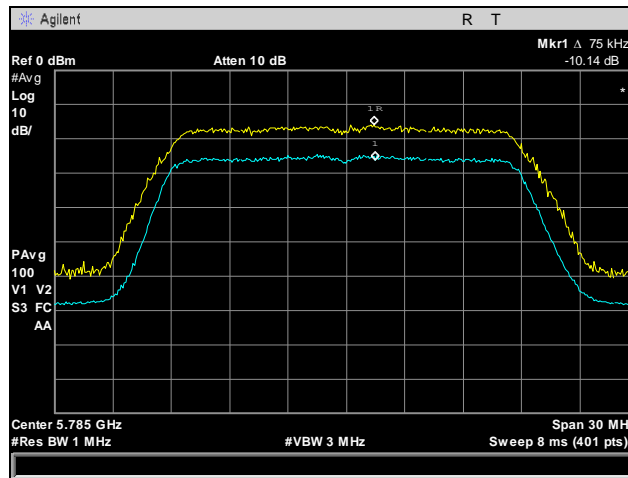
Plot 95. Peak Excursion Ratio, Mid Channel, 802.11n 20 MHz, Port 1
