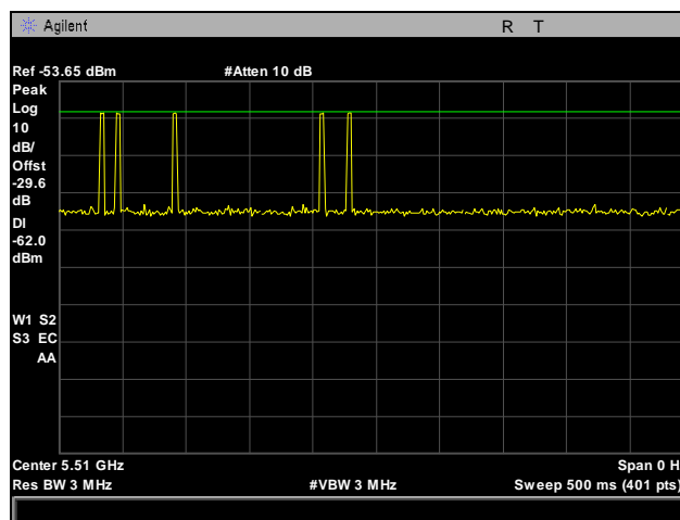
Plot 767. Radar Type 6 Calibration, 5510 MHz
