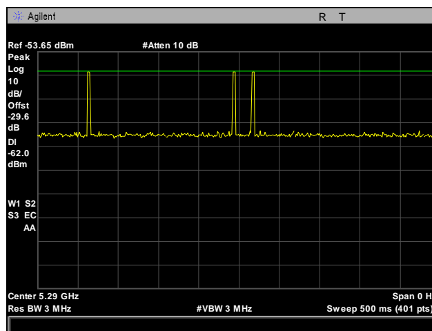
Plot 755. Radar Type 6 Calibration, 5290 MHz
