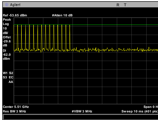
Plot 765. Radar Type 4 Calibration, 5510 MHz
