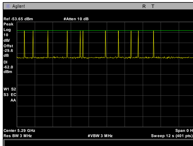
Plot 754. Radar Type 5 Calibration, 5290 MHz
