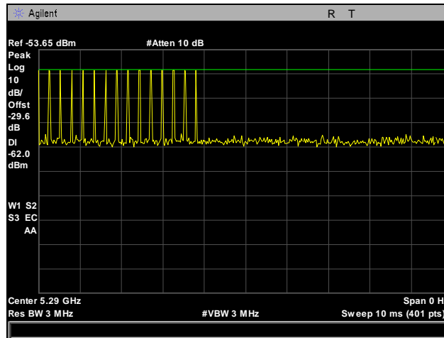
Plot 753. Radar Type 4 Calibration, 5290 MHz
