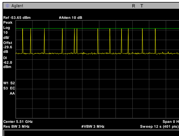
Plot 766. Radar Type 5 Calibration, 5510 MHz
