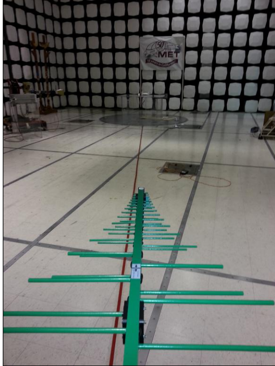
Photograph 5. Radiated Emission, Test Setup, AC-DC Power Supply
