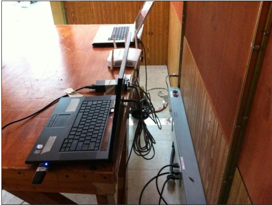
Photograph 4. Conducted Emissions, Test Setup, PoE, 2
