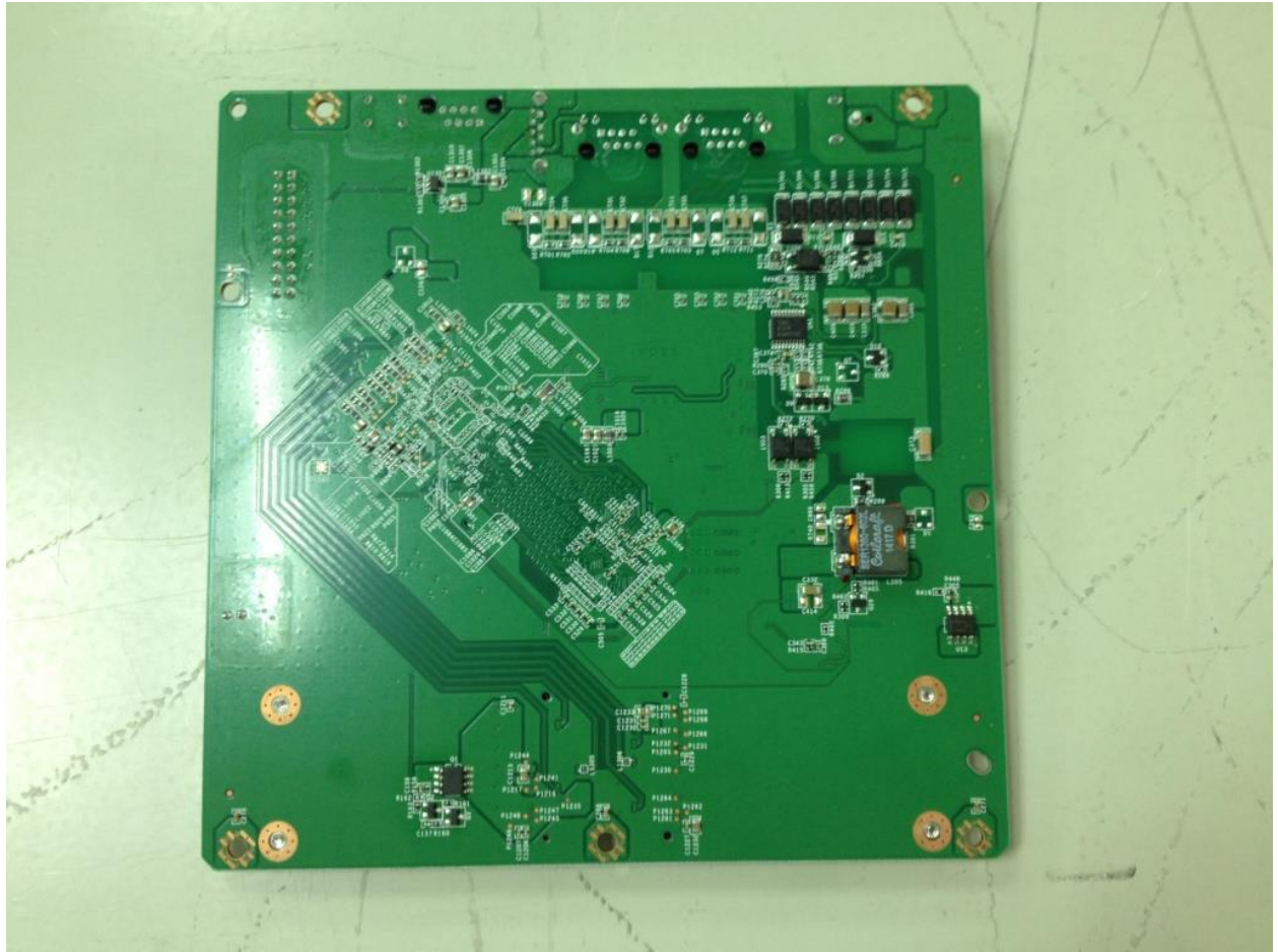
Photograph 4. MB Bottom
