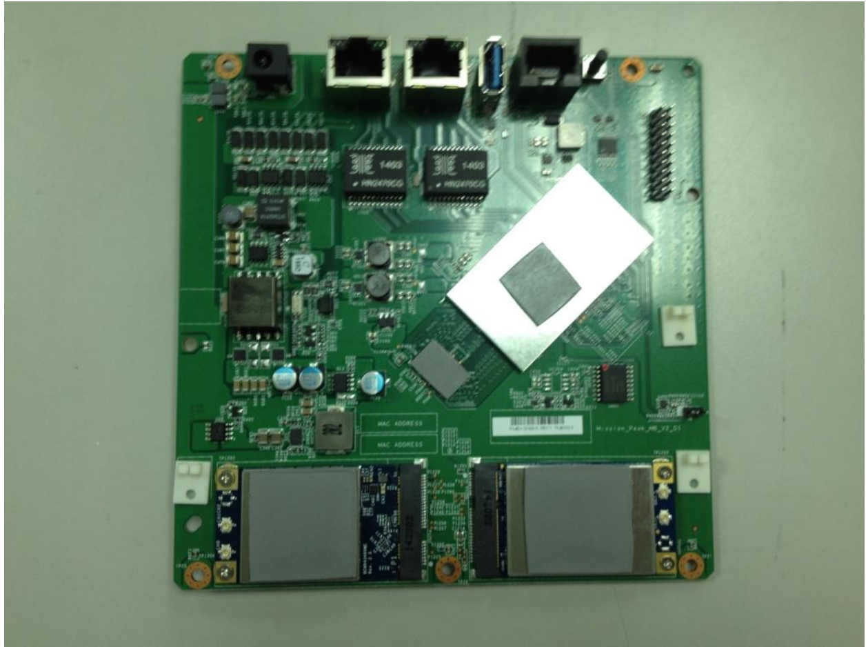
Photograph 1. Top
