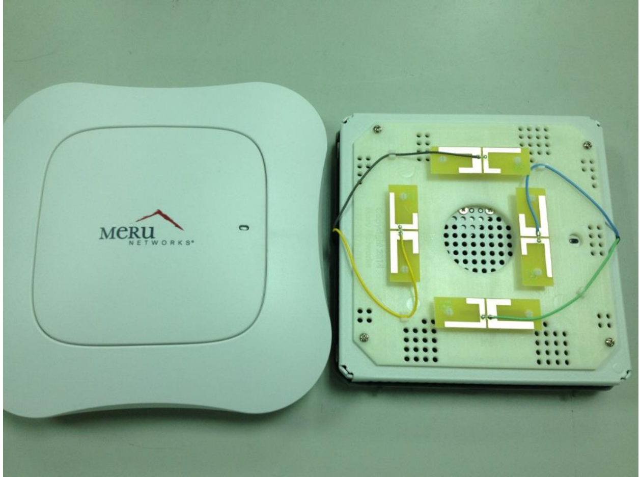
Photograph 2. Antenna
