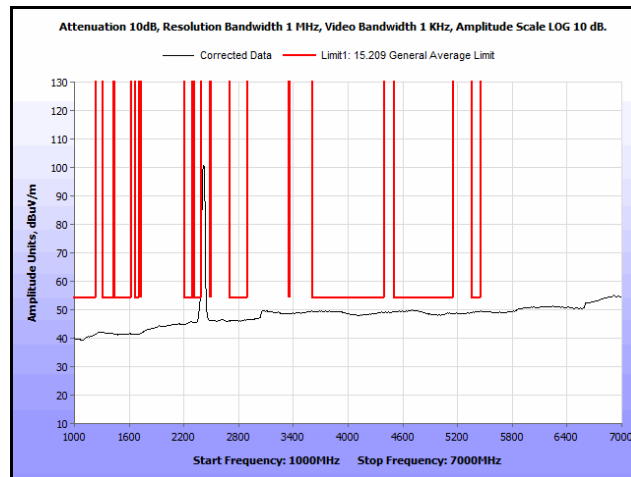
Plot 90. Radiated Spurs, Co-Location, 802.11n 20 MHz, 2412 MHz & 2412 MHz, 1 GHz – 7 GHz, Avg., Omni
