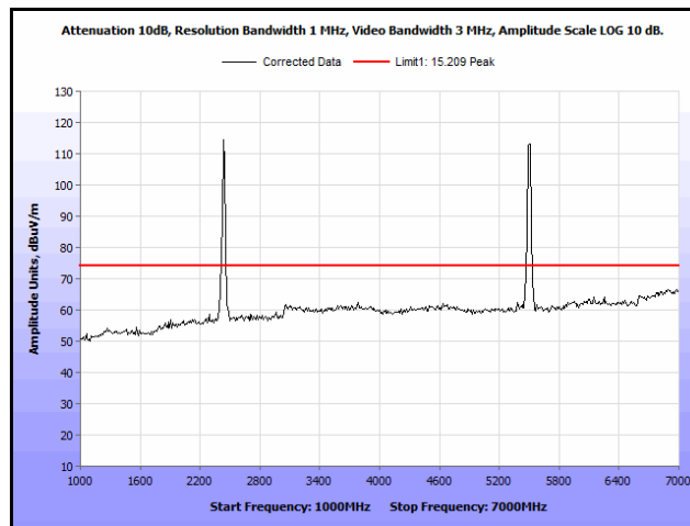
Plot 227. Radiated Spurs, Co-Location, 802.11n 20 MHz, 2437 MHz & 5580 MHz, 1 GHz – 7 GHz, Peak, Patch
