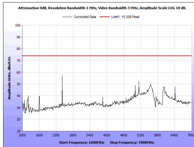
Plot 71. Radiated Spurious Emissions, 802.11ac 80 MHz, 1 GHz – 7 GHz, Peak
