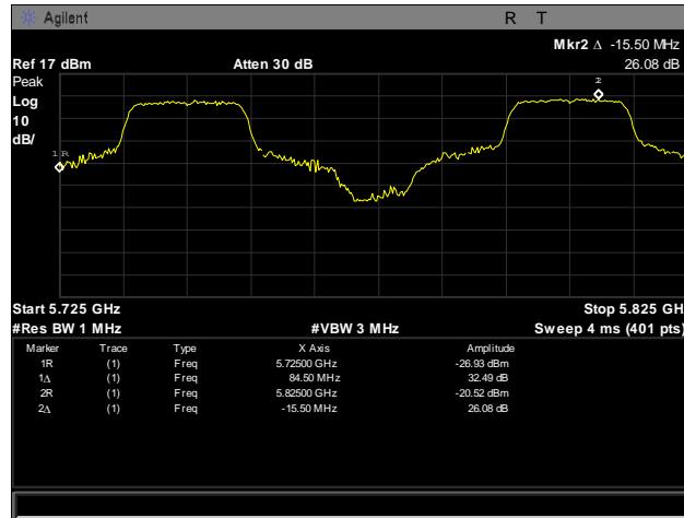
Plot 258. Frequency Stability, 5725 – 5825 MHz, 50°C, 120 V
