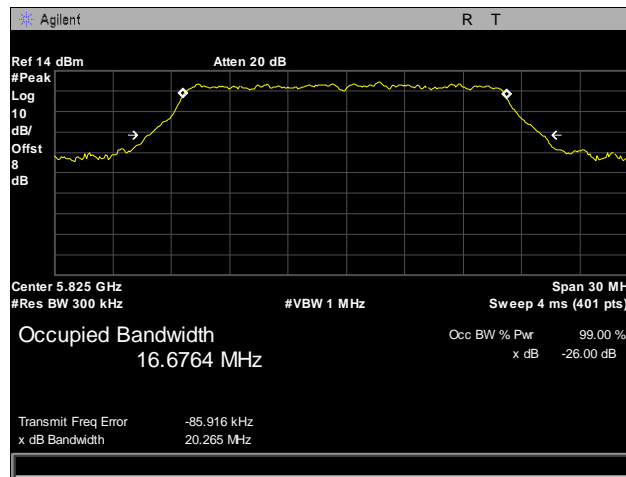
Plot 17. 26 dB Occupied Bandwidth, 802.11a, 5825 MHz
