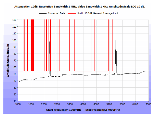
Plot 154. Radiated Spurs, Co-Location, 802.11n 20 MHz, 2462 MHz & 5580 MHz, 1 GHz – 7 GHz, Avg., Omni
