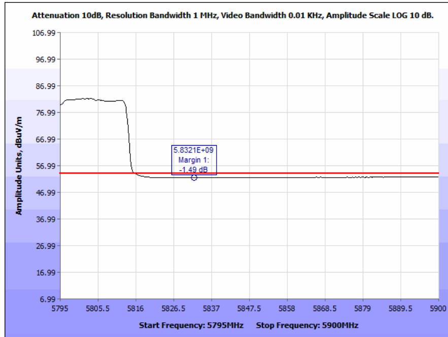
Plot 87. Radiated Band Edge, 802.11n 80 MHz (5832 & 5835 MHz), Average
