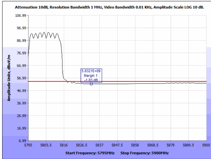
Plot 79. Radiated Band Edge, 802.11n 20 MHz, High Channel (5825 & 5835 MHz), Average
