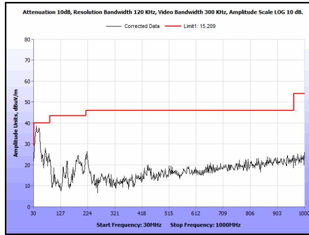
Plot 89. Radiated Spurs, Co-Location, 802.11n 20 MHz, 2412 MHz & 2412 MHz, 30 MHz – 1 GHz, Peak, Omni
