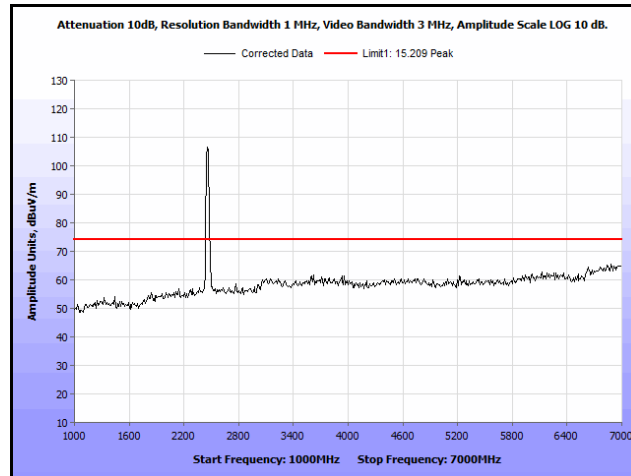
Plot 111. Radiated Spurs, Co-Location, 802.11n 20 MHz, 2462 MHz & 2462 MHz, 1 GHz – 7 GHz, Peak, Omni
