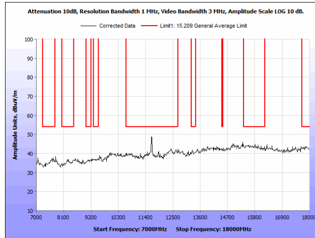
Plot 64. Radiated Spurious Emissions, 802.11n 20 MHz, High Channel, 7 GHz – 18 GHz
