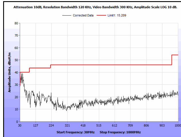
Plot 153. Radiated Spurs, Co-Location, 802.11n 20 MHz, 2462 MHz & 5580 MHz, 30 MHz – 1 GHz, Peak, Omni
