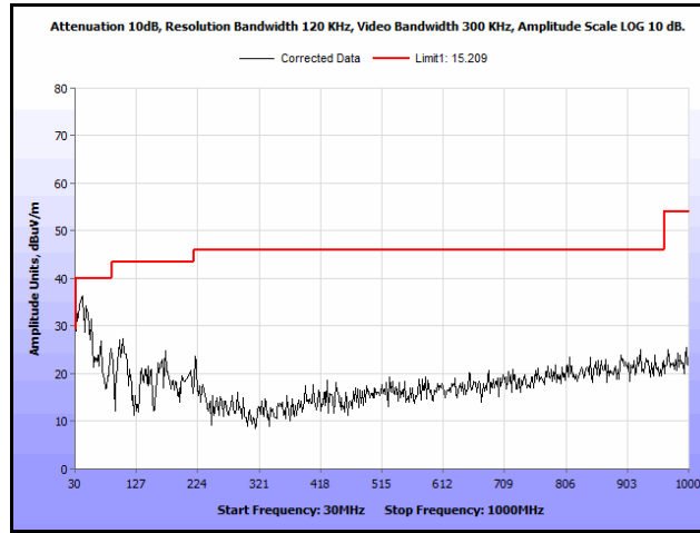
Plot 237. Radiated Spurs, Co-Location, 802.11n 20 MHz, 2462 MHz & 5300 MHz, 30 MHz – 1 GHz, Peak, Patch
