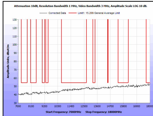
Plot 132. Radiated Spurs, Co-Location, 802.11n 20 MHz, 2437 MHz & 5200 MHz, 7 GHz – 18 GHz, Peak, Omni
