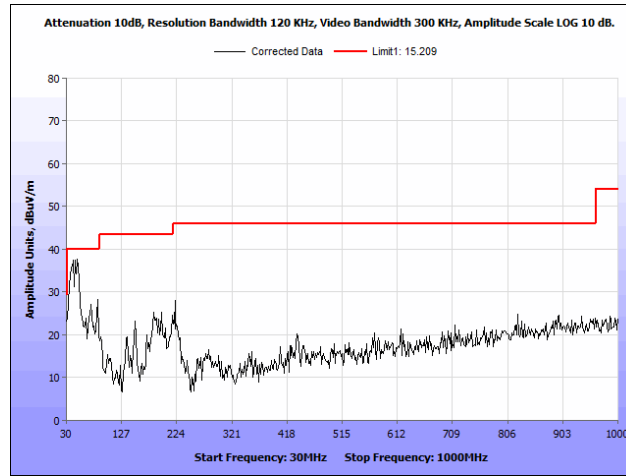
Plot 45. Radiated Spurious Emissions, 802.11a 40 MHz, High Channel, 30 MHz – 1 GHz
