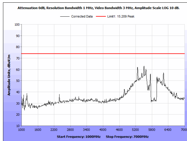
Plot 43. Radiated Spurious Emissions, 802.11a 20 MHz, High Channel, 1 GHz – 7 GHz, Peak
