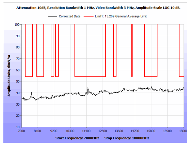
Plot 56. Radiated Spurious Emissions, 802.11n 40 MHz, Low Channel, 7 GHz – 18 GHz
