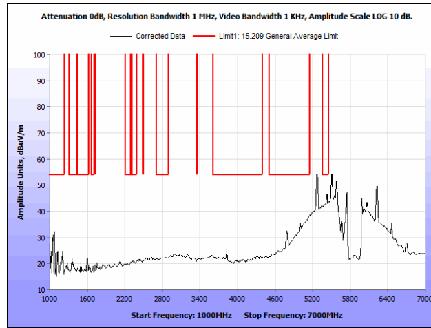
Plot 50. Radiated Spurious Emissions, 802.11n 20 MHz, Low Channel, 1 GHz – 7 GHz, Average
