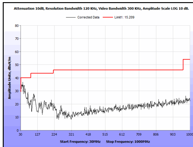
Plot 157. Radiated Spurs, Co-Location, 802.11n 20 MHz, 2462 MHz & 5785 MHz, 30 MHz – 1 GHz, Peak, Omni
