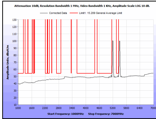
Plot 170. Radiated Spurs, Co-Location, 802.11n 20 MHz, 5200 MHz & 5580 MHz, 1 GHz – 7 GHz, Avg., Omni
