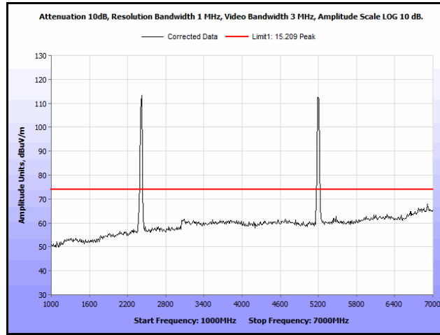
Plot 219. Radiated Spurs, Co-Location, 802.11n 20 MHz, 2437 MHz & 5200 MHz, 1 GHz – 7 GHz, Peak, Patch
