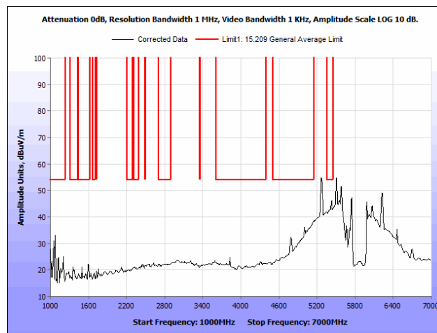
Plot 66. Radiated Spurious Emissions, 802.11n 40 MHz, High Channel, 1 GHz – 7 GHz, Average
