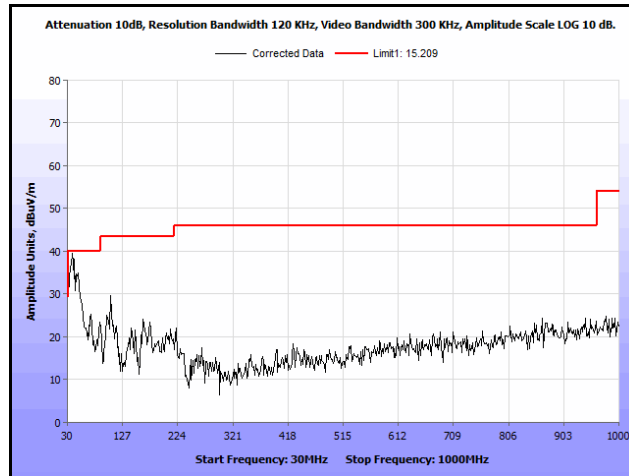
Plot 129. Radiated Spurs, Co-Location, 802.11n 20 MHz, 2437 MHz & 5200 MHz, 30 MHz – 1 GHz, Peak, Omni
