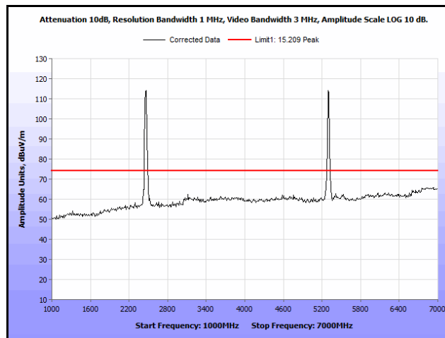
Plot 239. Radiated Spurs, Co-Location, 802.11n 20 MHz, 2462 MHz & 5300 MHz, 1 GHz – 7 GHz, Peak, Patch
