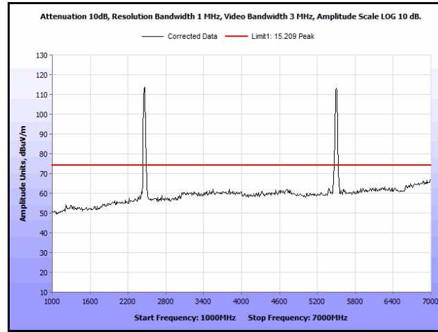
Plot 243. Radiated Spurs, Co-Location, 802.11n 20 MHz, 2462 MHz & 5580 MHz, 1 GHz – 7 GHz, Peak, Patch
