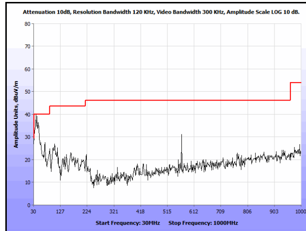
Plot 229. Radiated Spurs, Co-Location, 802.11n 20 MHz, 2437 MHz & 5785 MHz, 30 MHz – 1 GHz, Peak, Patch
