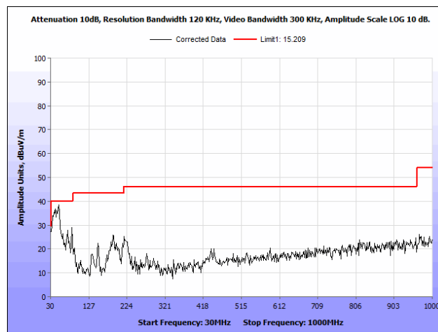
Plot 57. Radiated Spurious Emissions, 802.11n 20 MHz, Mid Channel, 30 MHz – 1 GHz
