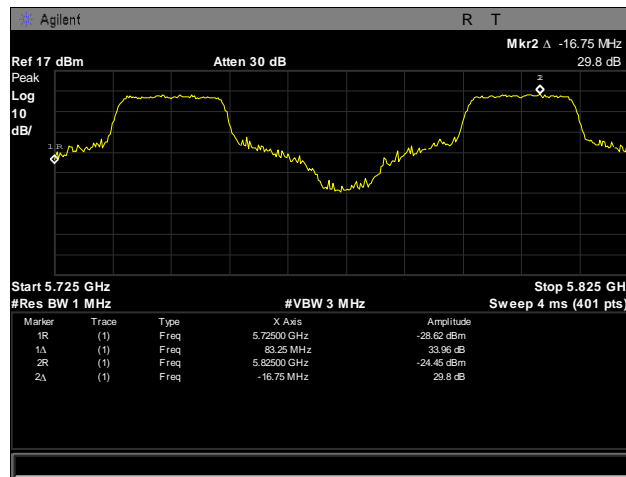
Plot 256. Frequency Stability, 5725 – 5825 MHz, 30°C, 120 V
