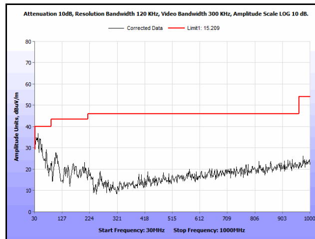
Plot 245. Radiated Spurs, Co-Location, 802.11n 20 MHz, 2462 MHz & 5785 MHz, 30 MHz – 1 GHz, Peak, Patch
