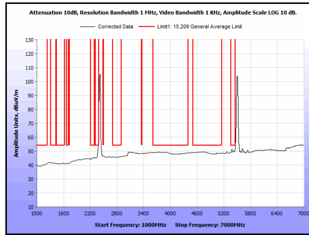
Plot 210. Radiated Spurs, Co-Location, 802.11n 20 MHz, 2412 MHz & 5580 MHz, 1 GHz – 7 GHz, Avg., Patch
