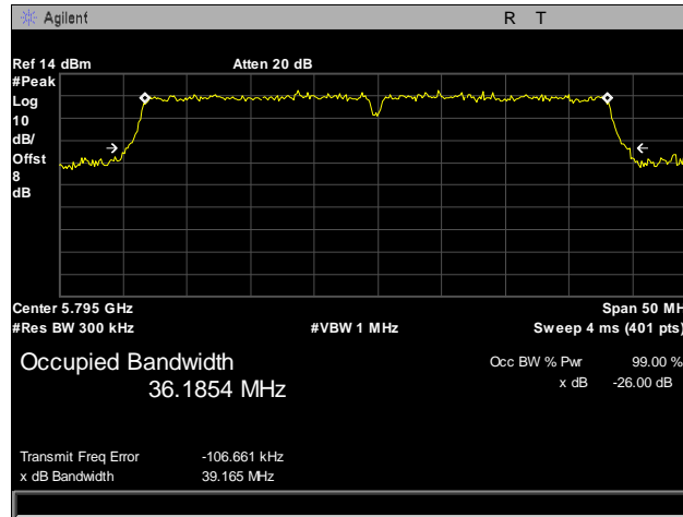
Plot 21. 26 dB Occupied Bandwidth, 802.11n, 5795 MHz, Port 1
