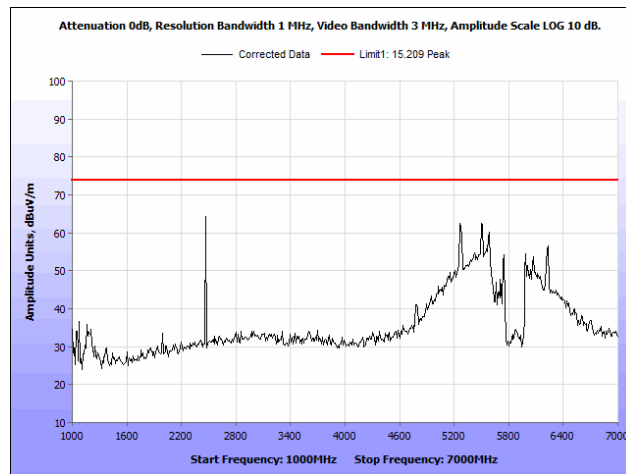
Plot 32. Radiated Spurious Emissions, 802.11a 20 MHz, Low Channel, 1 GHz – 7 GHz, Peak
