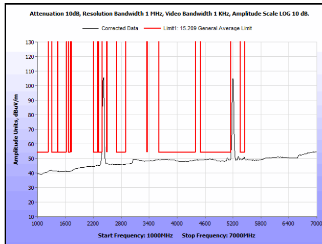
Plot 202. Radiated Spurs, Co-Location, 802.11n 20 MHz, 2412 MHz & 5200 MHz, 1 GHz – 7 GHz, Avg., Patch
