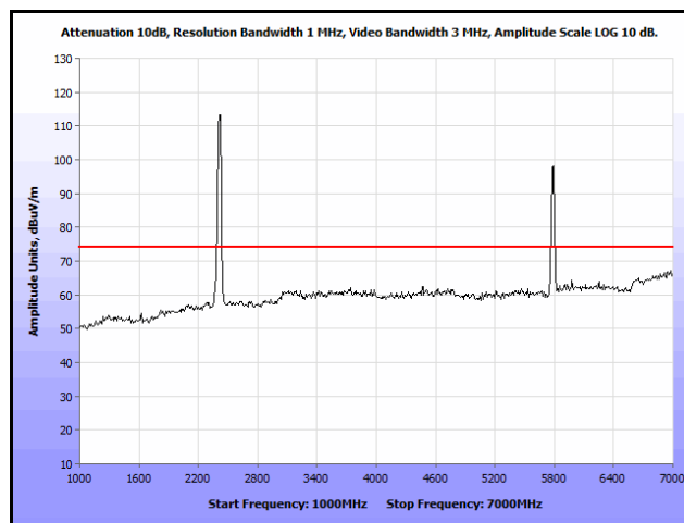
Plot 215. Radiated Spurs, Co-Location, 802.11n 20 MHz, 2412 MHz & 5785 MHz, 1 GHz – 7 GHz, Peak, Patch
