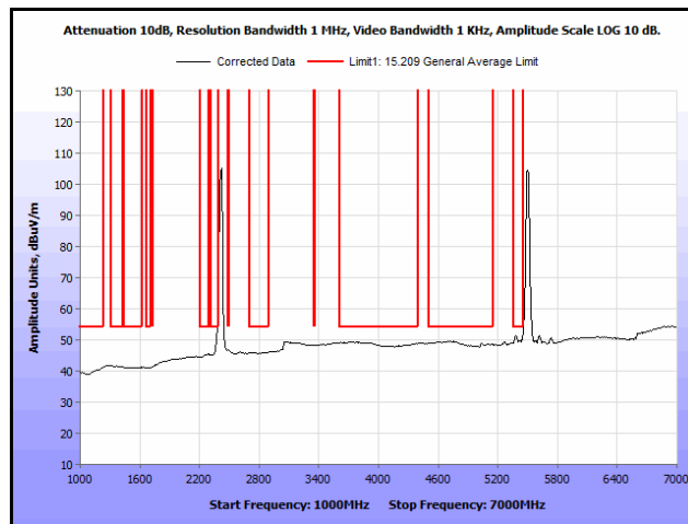
Plot 242. Radiated Spurs, Co-Location, 802.11n 20 MHz, 2462 MHz & 5580 MHz, 1 GHz – 7 GHz, Avg., Patch
