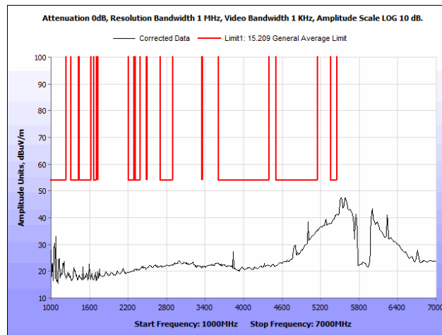
Plot 46. Radiated Spurious Emissions, 802.11a 40 MHz, High Channel, 1 GHz – 7 GHz, Average
