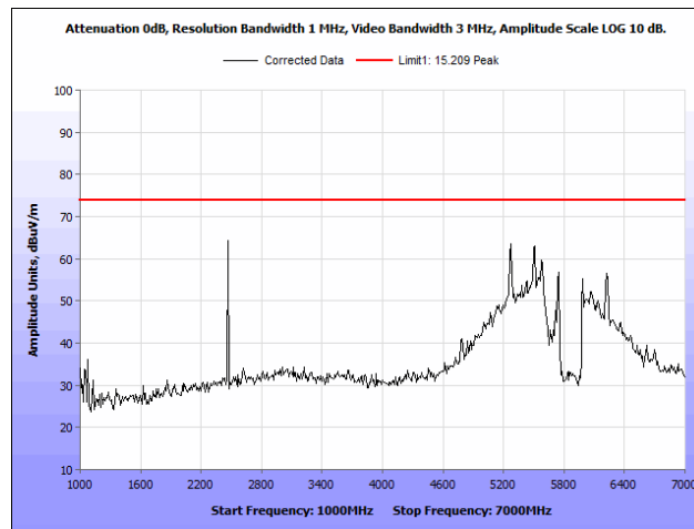
Plot 40. Radiated Spurious Emissions, 802.11a 20 MHz, Mid Channel, 1 GHz – 7 GHz, Peak
