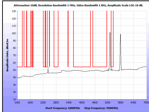
Plot 186. Radiated Spurs, Co-Location, 802.11n 20 MHz, 5300 MHz & 5785 MHz, 1 GHz – 7 GHz, Avg., Omni
