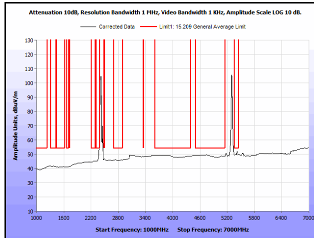
Plot 238. Radiated Spurs, Co-Location, 802.11n 20 MHz, 2462 MHz & 5300 MHz, 1 GHz – 7 GHz, Avg., Patch
