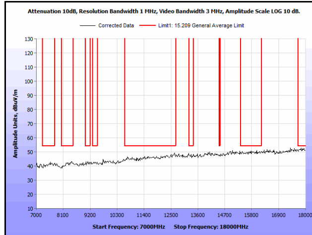
Plot 192. Radiated Spurs, Co-Location, 802.11n 20 MHz, 5580 MHz & 5580 MHz, 7 GHz – 18 GHz, Peak, Omni
