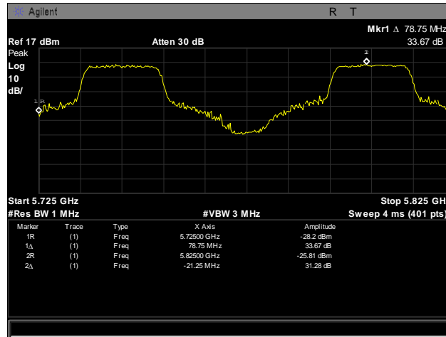
Plot 252. Frequency Stability, 5725 – 5825 MHz, -10°C, 120 V
