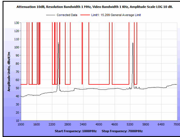
Plot 222. Radiated Spurs, Co-Location, 802.11n 20 MHz, 2437 MHz & 5300 MHz, 1 GHz – 7 GHz, Avg., Patch
