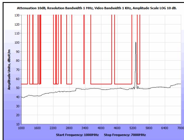
Plot 178. Radiated Spurs, Co-Location, 802.11n 20 MHz, 5300 MHz & 5300 MHz, 1 GHz – 7 GHz, Avg., Omni
