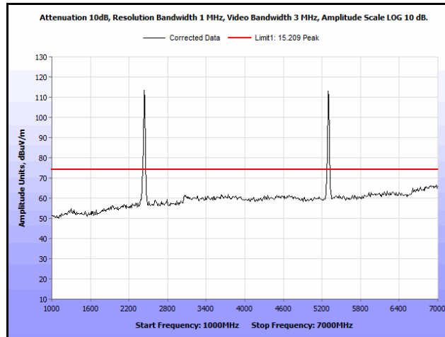
Plot 223. Radiated Spurs, Co-Location, 802.11n 20 MHz, 2437 MHz & 5300 MHz, 1 GHz – 7 GHz, Peak, Patch
