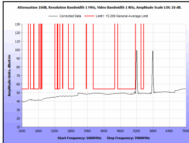
Plot 174. Radiated Spurs, Co-Location, 802.11n 20 MHz, 5200 MHz & 5785 MHz, 1 GHz – 7 GHz, Avg., Omni
