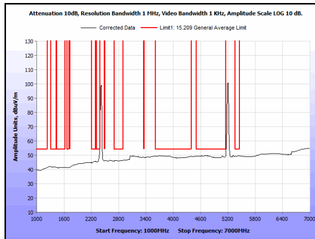
Plot 114. Radiated Spurs, Co-Location, 802.11n 20 MHz, 2412 MHz & 5200 MHz, 1 GHz – 7 GHz, Avg., Omni
