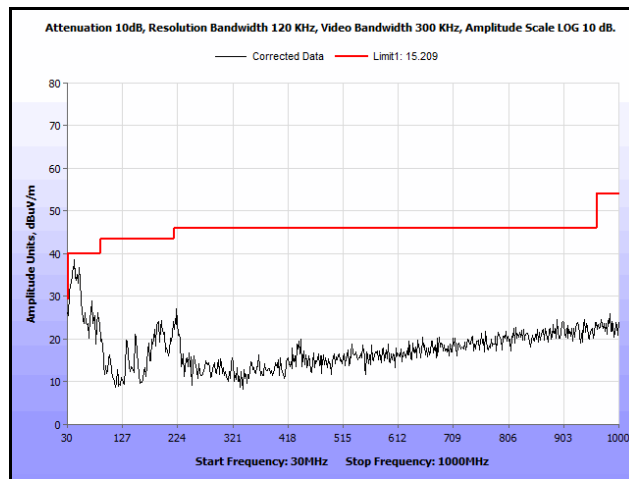
Plot 169. Radiated Spurs, Co-Location, 802.11n 20 MHz, 5200 MHz & 5580 MHz, 30 MHz – 1 GHz, Peak, Omni
