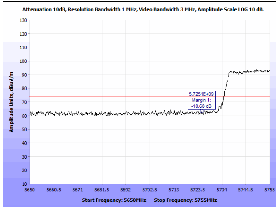
Plot 74. Radiated Band Edge, 802.11a, Low Channel (5715 & 5725 MHz), Peak
