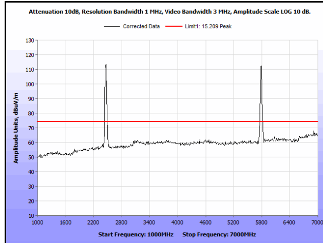
Plot 247. Radiated Spurs, Co-Location, 802.11n 20 MHz, 2462 MHz & 5785 MHz, 1 GHz – 7 GHz, Peak, Patch
