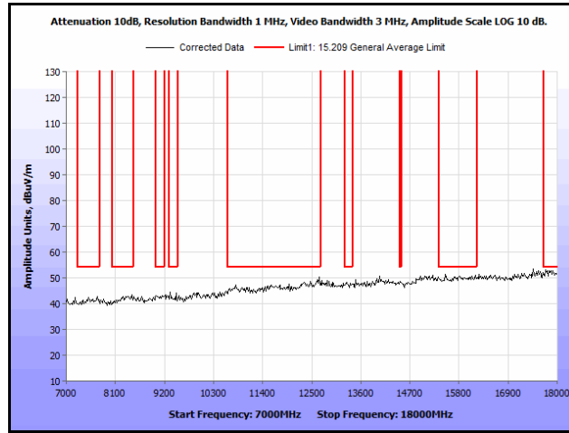
Plot 240. Radiated Spurs, Co-Location, 802.11n 20 MHz, 2462 MHz & 5300 MHz, 7 GHz – 18 GHz, Peak, Patch
