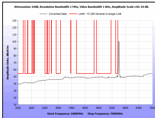
Plot 190. Radiated Spurs, Co-Location, 802.11n 20 MHz, 5580 MHz & 5580 MHz, 1 GHz – 7 GHz, Avg., Omni
