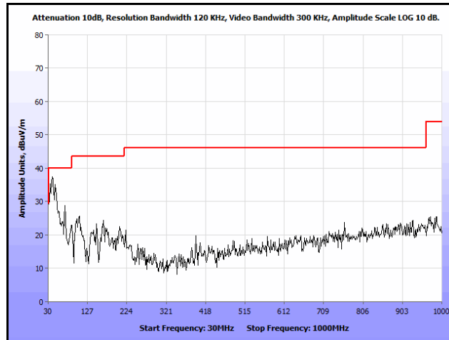
Plot 189. Radiated Spurs, Co-Location, 802.11n 20 MHz, 5580 MHz & 5580 MHz, 30 MHz – 1 GHz, Peak, Omni
