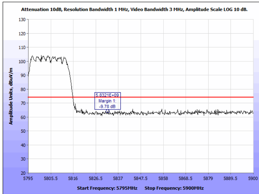
Plot 80. Radiated Band Edge, 802.11n 20 MHz, High Channel (5825 & 5835 MHz), Peak
