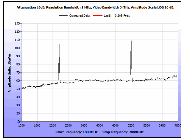
Plot 131. Radiated Spurs, Co-Location, 802.11n 20 MHz, 2437 MHz & 5200 MHz, 1 GHz – 7 GHz, Peak, Omni
