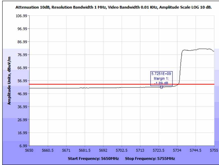
Plot 85. Radiated Band Edge, 802.11n 80 MHz (5715 & 5725 MHz), Average
