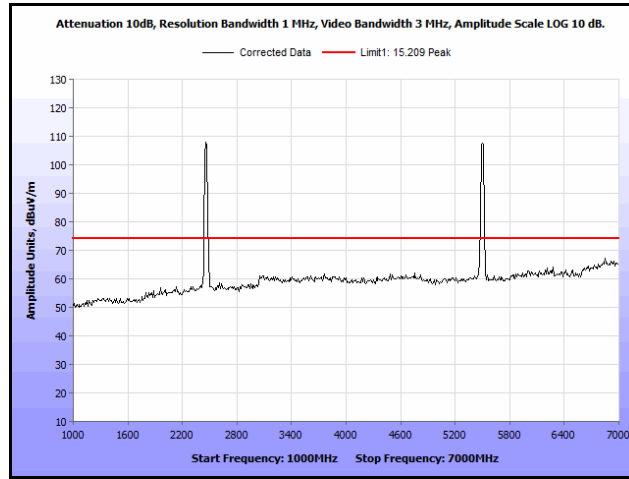
Plot 155. Radiated Spurs, Co-Location, 802.11n 20 MHz, 2462 MHz & 5580 MHz, 1 GHz – 7 GHz, Peak, Omni
