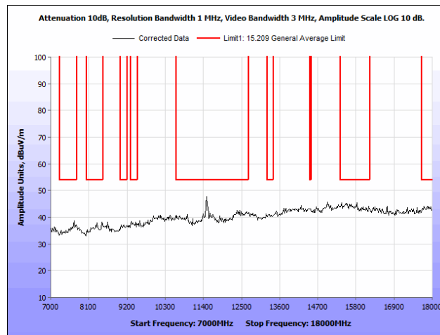
Plot 37. Radiated Spurious Emissions, 802.11a 40 MHz, Low Channel, 7 GHz – 18 GHz
