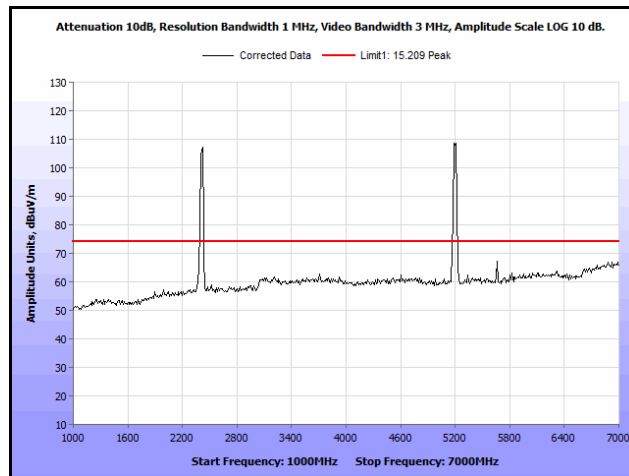
Plot 115. Radiated Spurs, Co-Location, 802.11n 20 MHz, 2412 MHz & 5200 MHz, 1 GHz – 7 GHz, Peak, Omni
