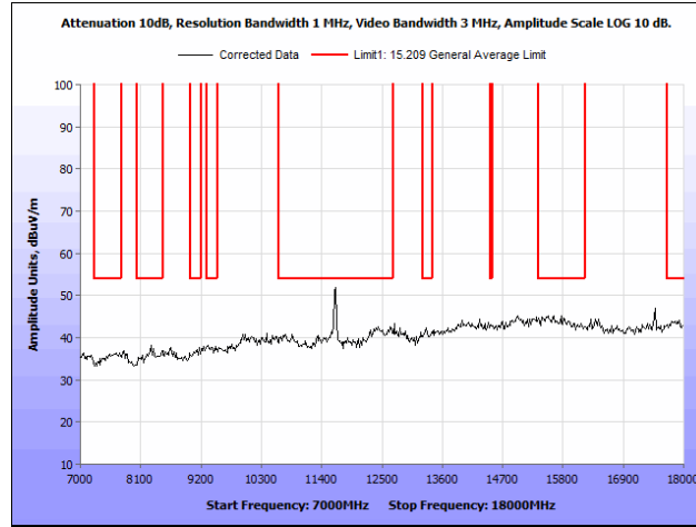
Plot 44. Radiated Spurious Emissions, 802.11a 20 MHz, High Channel, 7 GHz – 18 GHz
