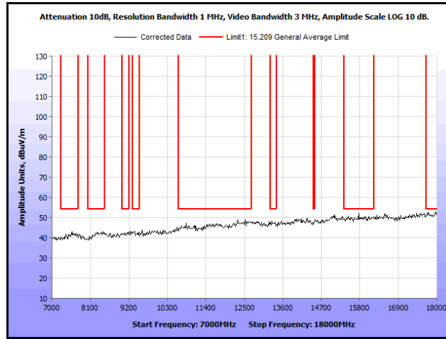
Plot 188. Radiated Spurs, Co-Location, 802.11n 20 MHz, 5300 MHz & 5785 MHz, 7 GHz – 18 GHz, Peak, Omni
