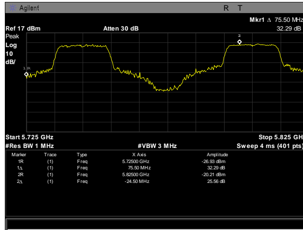
Plot 255. Frequency Stability, 5725 – 5825 MHz, 20°C, 120 V
