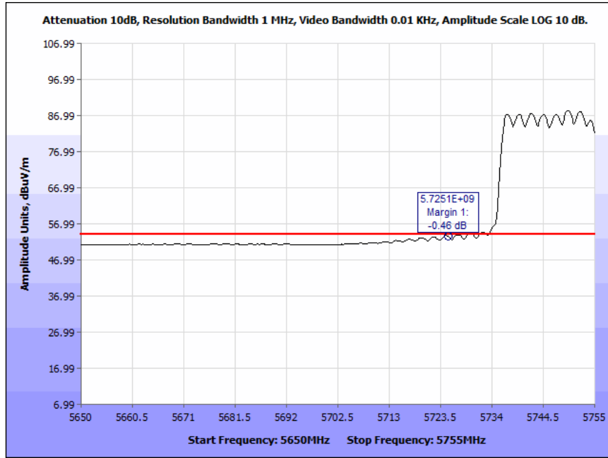
Plot 73. Radiated Band Edge, 802.11a, Low Channel (5715 & 5725 MHz), Average
