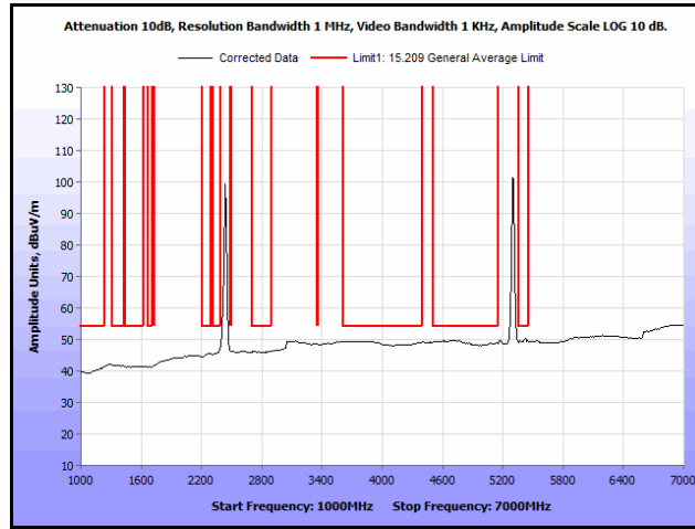
Plot 134. Radiated Spurs, Co-Location, 802.11n 20 MHz, 2437 MHz & 5300 MHz, 1 GHz – 7 GHz, Avg., Omni
