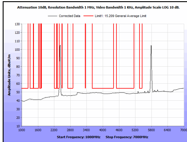
Plot 214. Radiated Spurs, Co-Location, 802.11n 20 MHz, 2412 MHz & 5785 MHz, 1 GHz – 7 GHz, Avg., Patch
