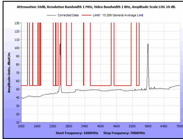
Plot 246. Radiated Spurs, Co-Location, 802.11n 20 MHz, 2462 MHz & 5785 MHz, 1 GHz – 7 GHz, Avg., Patch
