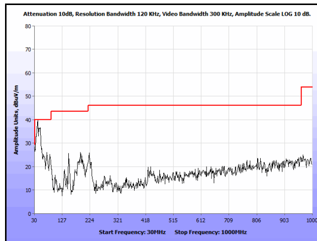
Plot 109. Radiated Spurs, Co-Location, 802.11n 20 MHz, 2462 MHz & 2462 MHz, 30 MHz – 1 GHz, Peak, Omni
