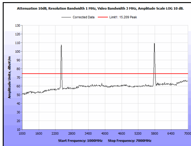
Plot 127. Radiated Spurs, Co-Location, 802.11n 20 MHz, 2412 MHz & 5785 MHz, 1 GHz – 7 GHz, Peak, Omni
