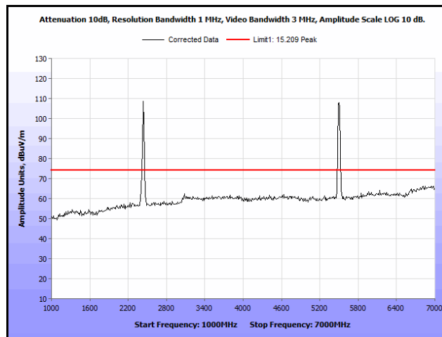
Plot 139. Radiated Spurs, Co-Location, 802.11n 20 MHz, 2437 MHz & 5580 MHz, 1 GHz – 7 GHz, Peak, Omni
