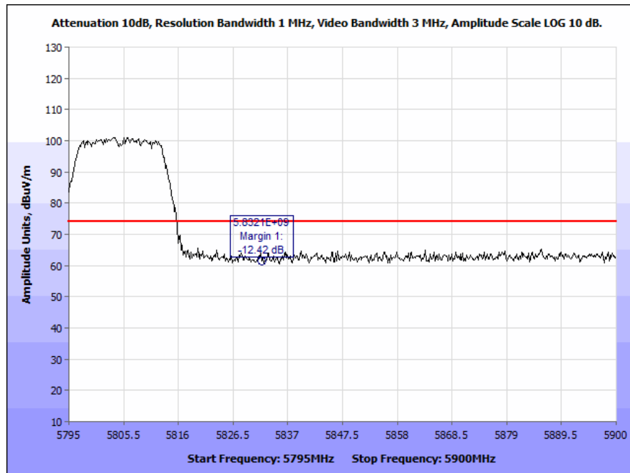
Plot 76. Radiated Band Edge, 802.11a, High Channel (5825 & 5835 MHz), Peak
