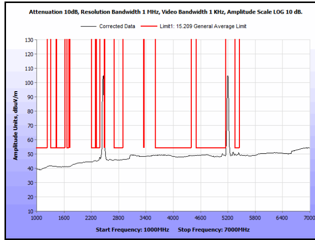
Plot 234. Radiated Spurs, Co-Location, 802.11n 20 MHz, 2462 MHz & 5200 MHz, 1 GHz – 7 GHz, Avg., Patch
