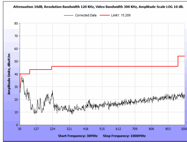
Plot 49. Radiated Spurious Emissions, 802.11n 20 MHz, Low Channel, 30 MHz – 1 GHz
