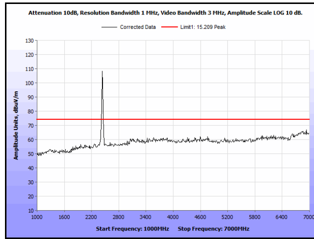
Plot 107. Radiated Spurs, Co-Location, 802.11n 20 MHz, 2437 MHz & 2462 MHz, 1 GHz – 7 GHz, Peak, Omni
