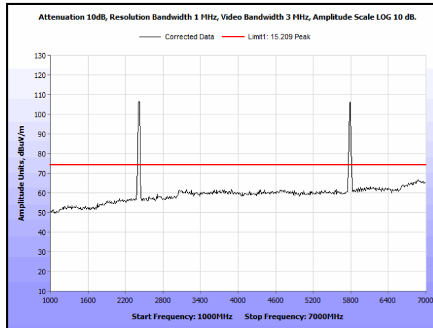
Plot 159. Radiated Spurs, Co-Location, 802.11n 20 MHz, 2462 MHz & 5785 MHz, 1 GHz – 7 GHz, Peak, Omni
