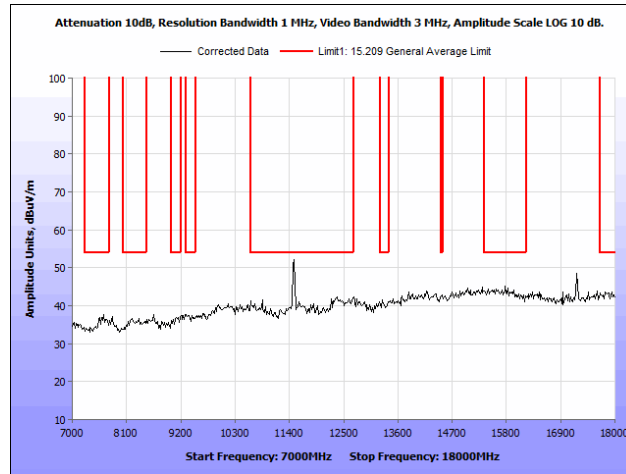
Plot 33. Radiated Spurious Emissions, 802.11a 20 MHz, Low Channel, 7 GHz – 18 GHz
