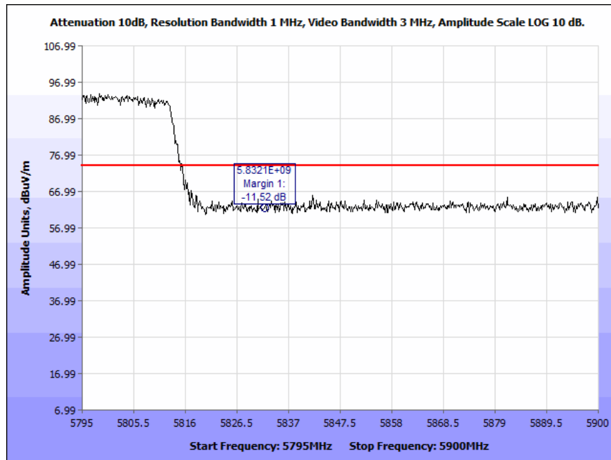
Plot 88. Radiated Band Edge, 802.11n 80 MHz (5832 & 5835 MHz), Peak
