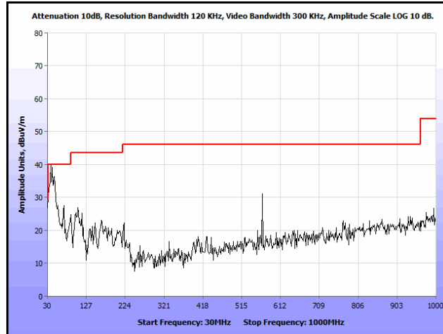
Plot 141. Radiated Spurs, Co-Location, 802.11n 20 MHz, 2437 MHz & 5785 MHz, 30 MHz – 1 GHz, Peak, Omni
