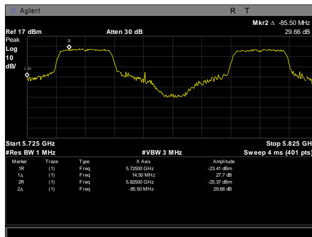
Plot 254. Frequency Stability, 5725 – 5825 MHz, 10°C, 120 V
