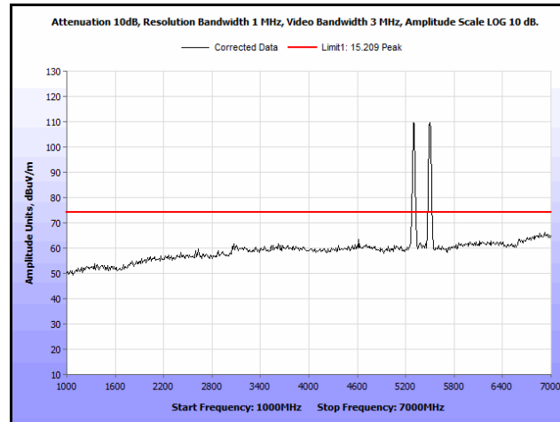
Plot 183. Radiated Spurs, Co-Location, 802.11n 20 MHz, 5300 MHz & 5580 MHz, 1 GHz – 7 GHz, Peak, Omni
