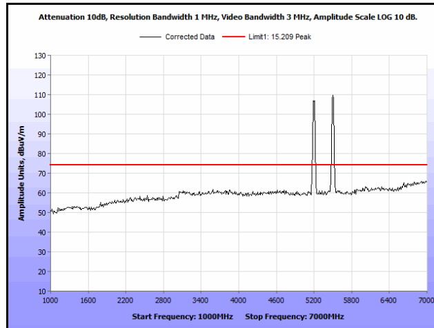
Plot 171. Radiated Spurs, Co-Location, 802.11n 20 MHz, 5200 MHz & 5580 MHz, 1 GHz – 7 GHz, Peak, Omni
