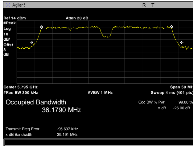
Plot 16. 26 dB Occupied Bandwidth, 802.11a, 5795 MHz
