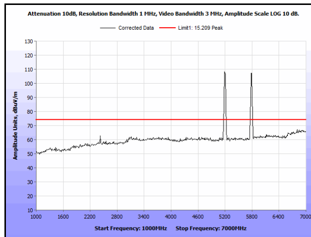
Plot 175. Radiated Spurs, Co-Location, 802.11n 20 MHz, 5200 MHz & 5785 MHz, 1 GHz – 7 GHz, Peak, Omni
