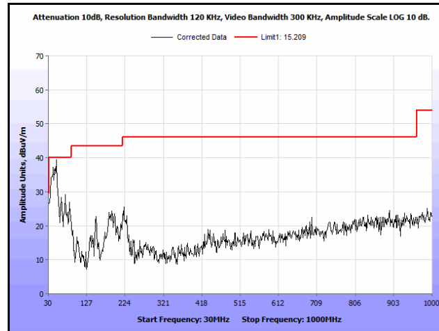
Plot 205. Radiated Spurs, Co-Location, 802.11n 20 MHz, 2412 MHz & 5300 MHz, 30 MHz – 1 GHz, Peak, Patch
