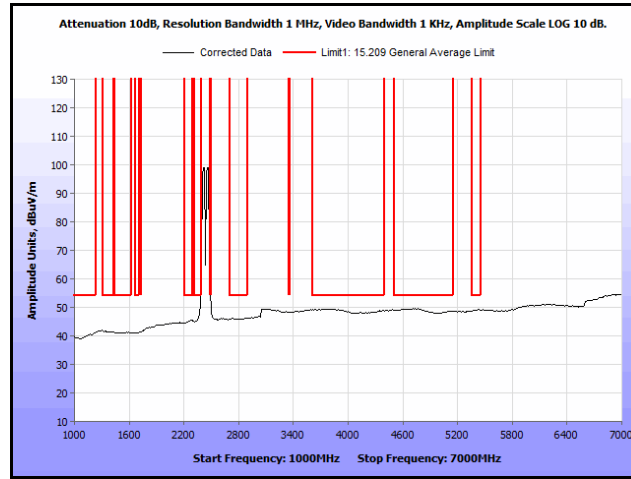
Plot 98. Radiated Spurs, Co-Location, 802.11n 20 MHz, 2412 MHz & 2462 MHz, 1 GHz – 7 GHz, Avg., Omni
