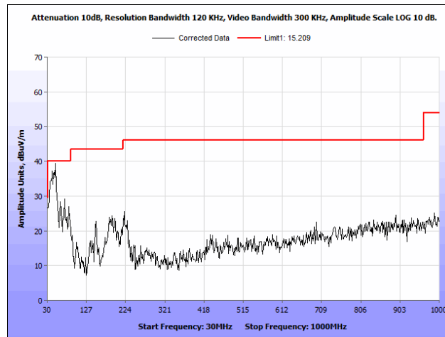
Plot 53. Radiated Spurious Emissions, 802.11n 40 MHz, Low Channel, 30 MHz – 1 GHz
