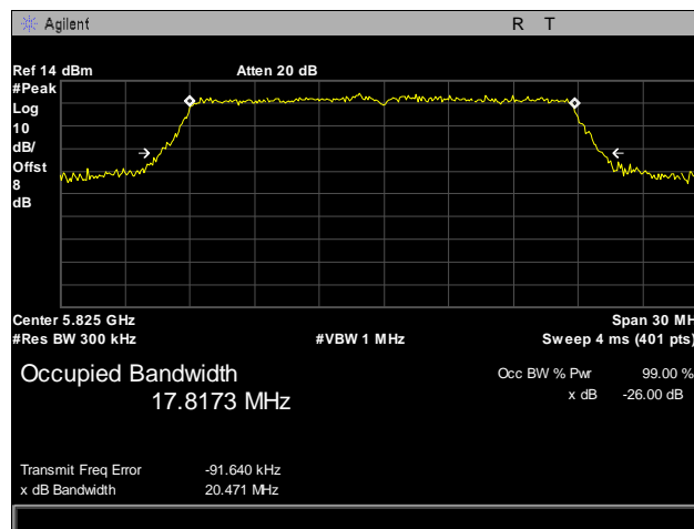
Plot 22. 26 dB Occupied Bandwidth, 802.11n, 5825 MHz, Port 1
