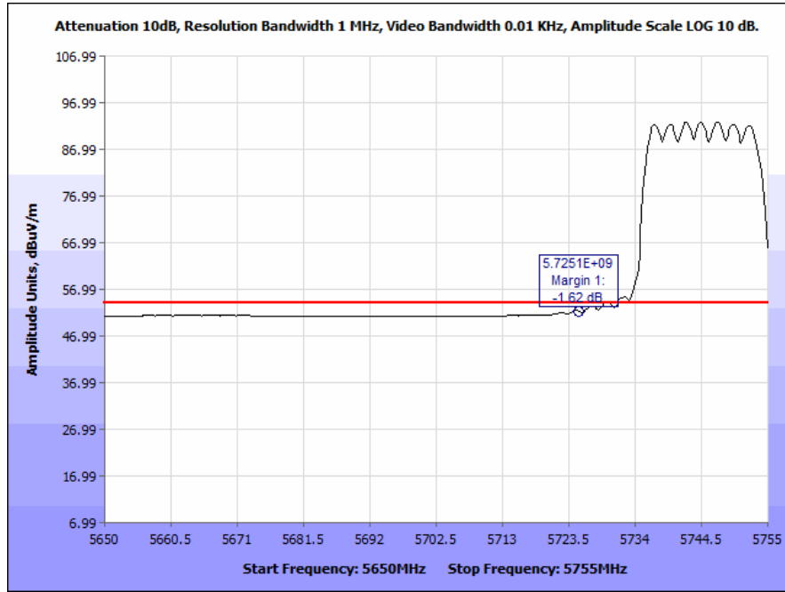
Plot 77. Radiated Band Edge, 802.11n 20 MHz, Low Channel (5715 & 5725 MHz), Average
