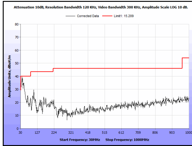
Plot 185. Radiated Spurs, Co-Location, 802.11n 20 MHz, 5300 MHz & 5785 MHz, 30 MHz – 1 GHz, Peak, Omni
