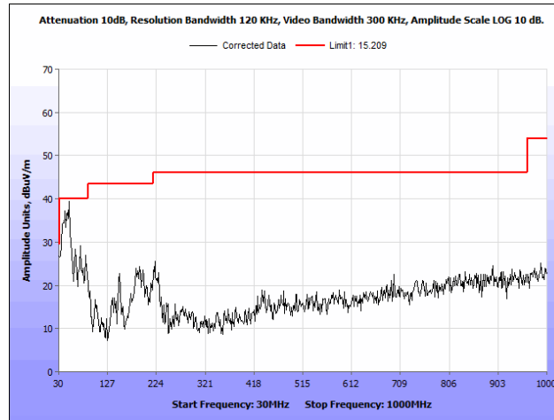
Plot 61. Radiated Spurious Emissions, 802.11n 20 MHz, High Channel, 30 MHz – 1 GHz
