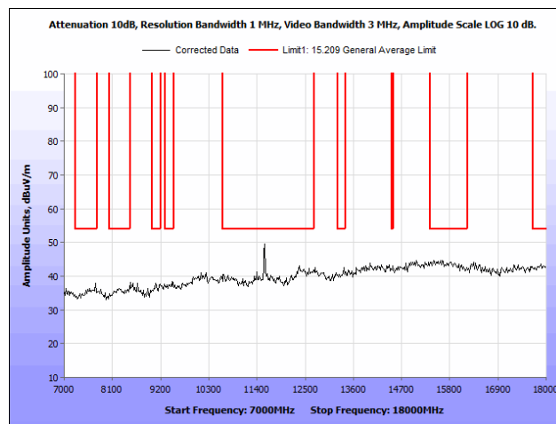
Plot 60. Radiated Spurious Emissions, 802.11n 20 MHz, Mid Channel, 7 GHz – 18 GHz
