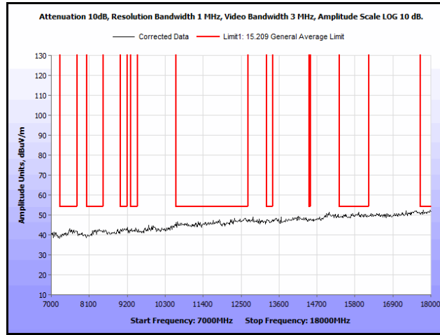
Plot 164. Radiated Spurs, Co-Location, 802.11n 20 MHz, 5200 MHz & 5200 MHz, 7 GHz – 18 GHz, Peak, Omni
