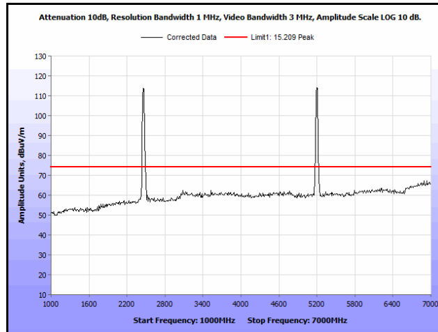
Plot 235. Radiated Spurs, Co-Location, 802.11n 20 MHz, 2462 MHz & 5200 MHz, 1 GHz – 7 GHz, Peak, Patch
