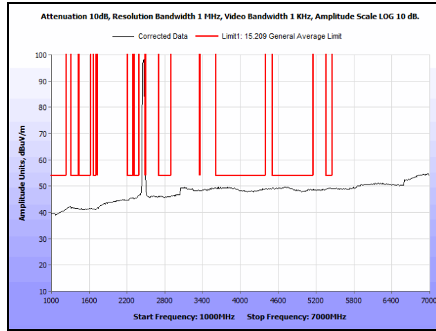
Plot 110. Radiated Spurs, Co-Location, 802.11n 20 MHz, 2462 MHz & 2462 MHz, 1 GHz – 7 GHz, Avg., Omni
