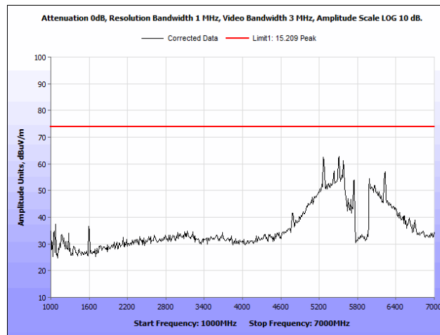
Plot 59. Radiated Spurious Emissions, 802.11n 20 MHz, Mid Channel, 1 GHz – 7 GHz, Peak
