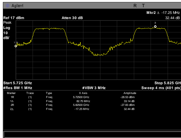
Plot 259. Frequency Stability, 5725 – 5825 MHz, 55°C, 120 V
