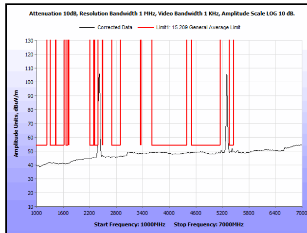
Plot 206. Radiated Spurs, Co-Location, 802.11n 20 MHz, 2412 MHz & 5300 MHz, 1 GHz – 7 GHz, Avg., Patch
