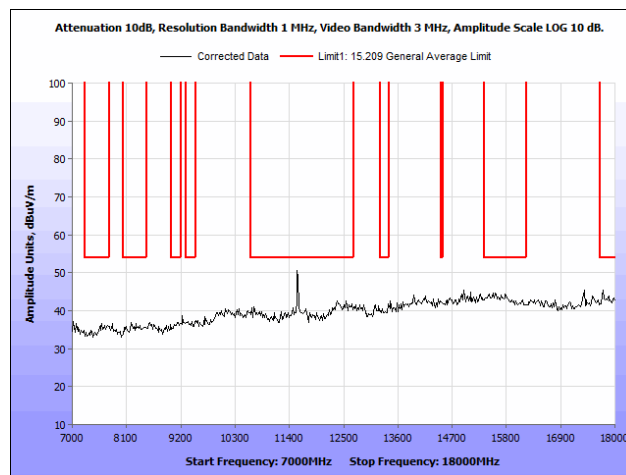
Plot 41. Radiated Spurious Emissions, 802.11a 20 MHz, Mid Channel, 7 GHz – 18 GHz
