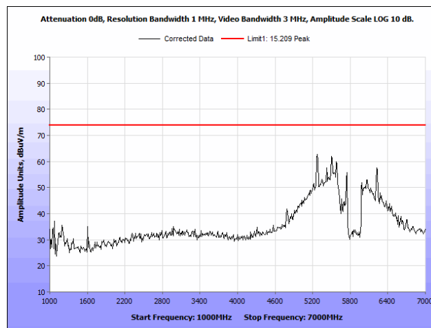
Plot 63. Radiated Spurious Emissions, 802.11n 20 MHz, High Channel, 1 GHz – 7 GHz, Peak
