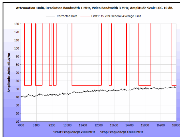
Plot 124. Radiated Spurs, Co-Location, 802.11n 20 MHz, 2412 MHz & 5580 MHz, 7 GHz – 18 GHz, Peak, Omni
