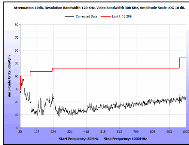
Plot 213. Radiated Spurs, Co-Location, 802.11n 20 MHz, 2412 MHz & 5785 MHz, 30 MHz – 1 GHz, Peak, Patch
