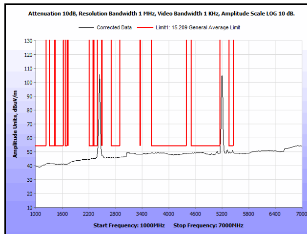
Plot 218. Radiated Spurs, Co-Location, 802.11n 20 MHz, 2437 MHz & 5200 MHz, 1 GHz – 7 GHz, Avg., Patch
