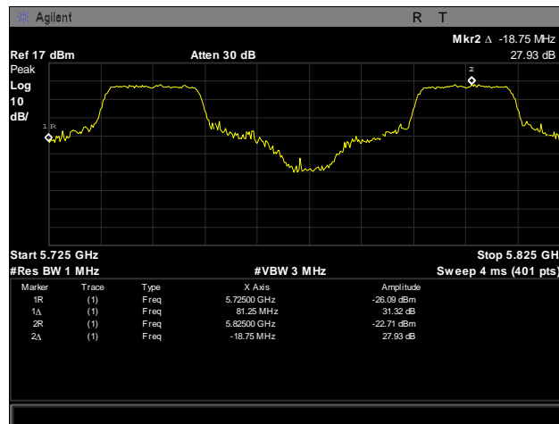
Plot 257. Frequency Stability, 5725 – 5825 MHz, 40°C, 120 V
