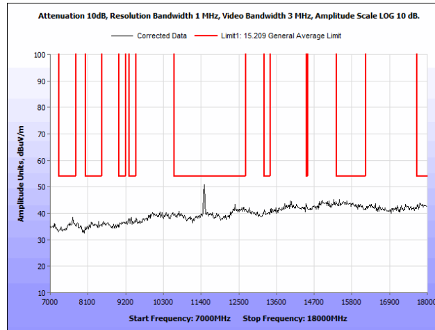
Plot 52. Radiated Spurious Emissions, 802.11n 20 MHz, Low Channel, 7 GHz – 18 GHz
