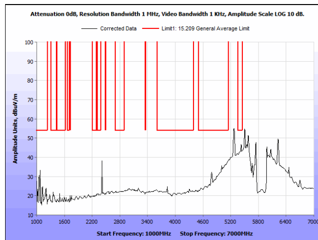
Plot 54. Radiated Spurious Emissions, 802.11n 40 MHz, Low Channel, 1 GHz – 7 GHz, Average
