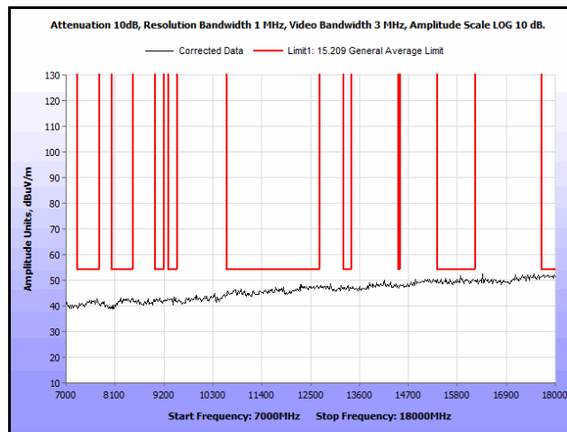
Plot 196. Radiated Spurs, Co-Location, 802.11n 20 MHz, 5580 MHz & 5785 MHz, 7 GHz – 18 GHz, Peak, Omni
