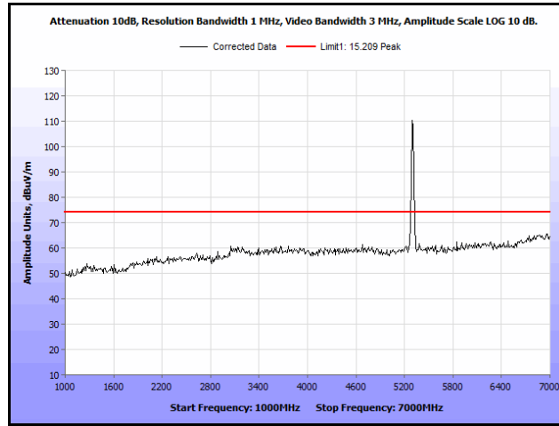
Plot 179. Radiated Spurs, Co-Location, 802.11n 20 MHz, 5300 MHz & 5300 MHz, 1 GHz – 7 GHz, Peak, Omni
