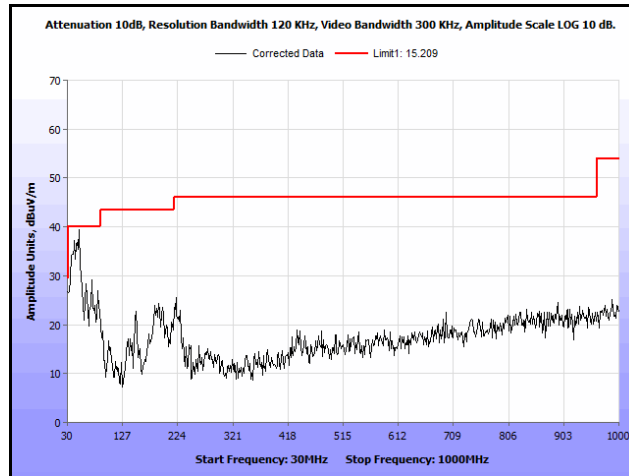
Plot 117. Radiated Spurs, Co-Location, 802.11n 20 MHz, 2412 MHz & 5300 MHz, 30 MHz – 1 GHz, Peak, Omni
