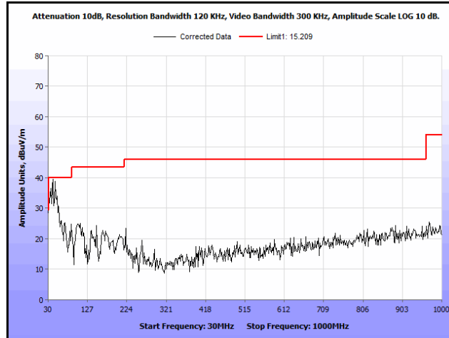
Plot 241. Radiated Spurs, Co-Location, 802.11n 20 MHz, 2462 MHz & 5580 MHz, 30 MHz – 1 GHz, Peak, Patch
