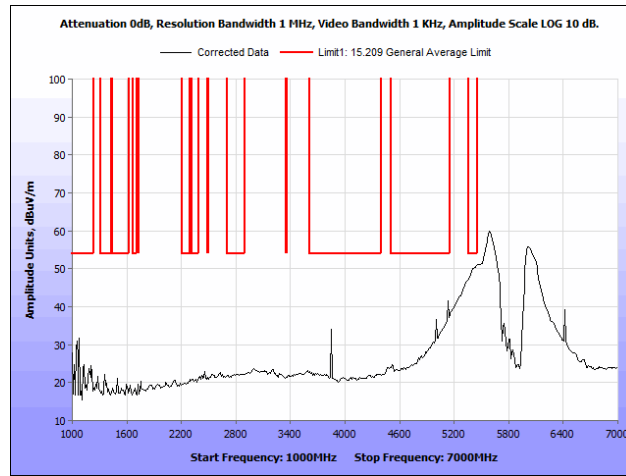
Plot 70. Radiated Spurious Emissions, 802.11ac 80 MHz, 1 GHz – 7 GHz, Average
