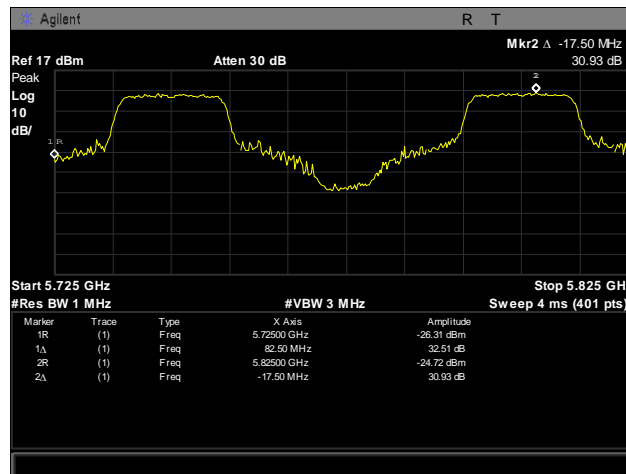
Plot 251. Frequency Stability, 5725 – 5825 MHz, -20°C, 120 V
