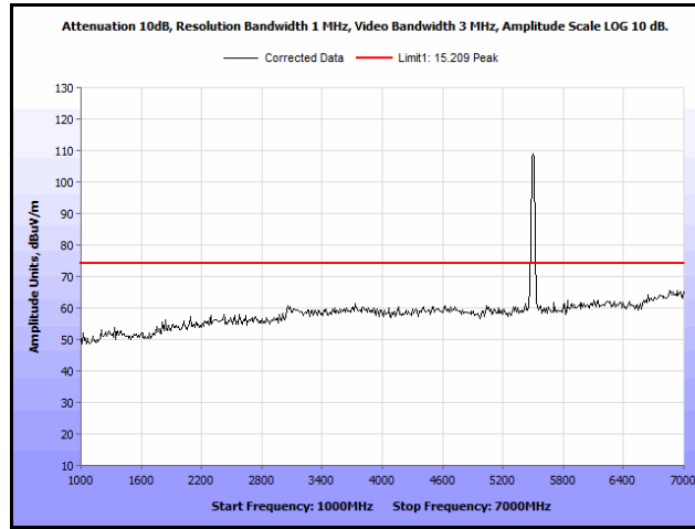
Plot 191. Radiated Spurs, Co-Location, 802.11n 20 MHz, 5580 MHz & 5580 MHz, 1 GHz – 7 GHz, Peak, Omni
