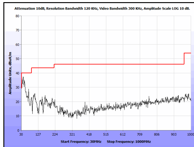
Plot 133. Radiated Spurs, Co-Location, 802.11n 20 MHz, 2437 MHz & 5300 MHz, 30 MHz – 1 GHz, Peak, Omni
