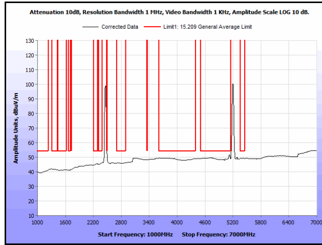
Plot 146. Radiated Spurs, Co-Location, 802.11n 20 MHz, 2462 MHz & 5200 MHz, 1 GHz – 7 GHz, Avg., Omni
