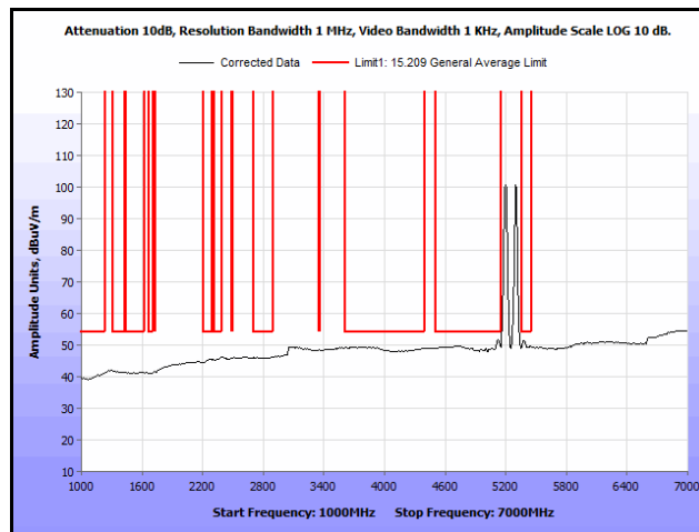
Plot 166. Radiated Spurs, Co-Location, 802.11n 20 MHz, 5200 MHz & 5300 MHz, 1 GHz – 7 GHz, Avg., Omni
