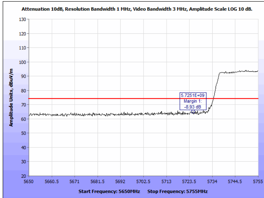
Plot 86. Radiated Band Edge, 802.11n 80 MHz (5715 & 5725 MHz), Peak
