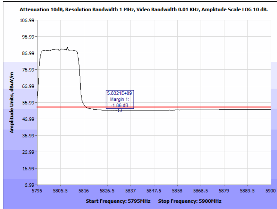
Plot 83. Radiated Band Edge, 802.11n 40 MHz, High Channel (5832 & 5835 MHz), Average
