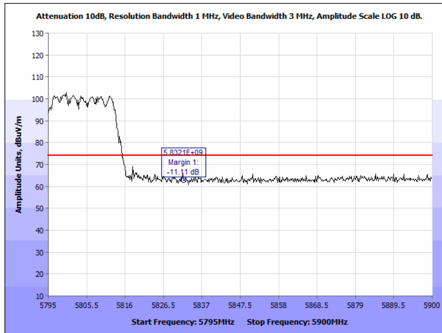
Plot 84. Radiated Band Edge, 802.11n 40 MHz, High Channel (5832 & 5835 MHz), Peak
