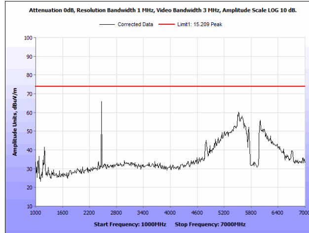
Plot 55. Radiated Spurious Emissions, 802.11n 40 MHz, Low Channel, 1 GHz – 7 GHz, Peak
