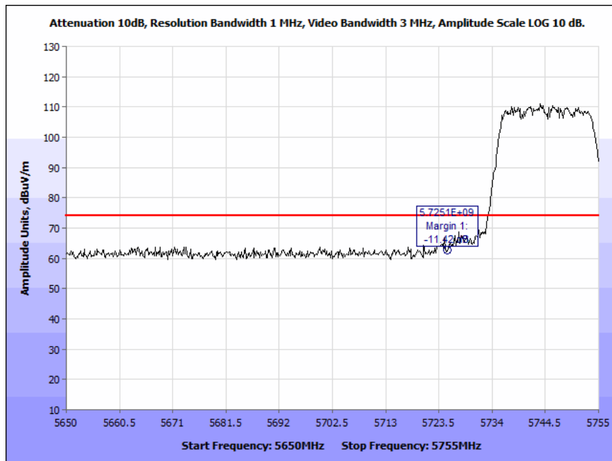
Plot 78. Radiated Band Edge, 802.11n 20 MHz, Low Channel (5715 & 5725 MHz), Peak
