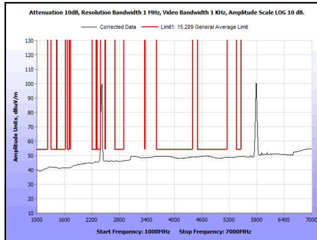
Plot 126. Radiated Spurs, Co-Location, 802.11n 20 MHz, 2412 MHz & 5785 MHz, 1 GHz – 7 GHz, Avg., Omni
