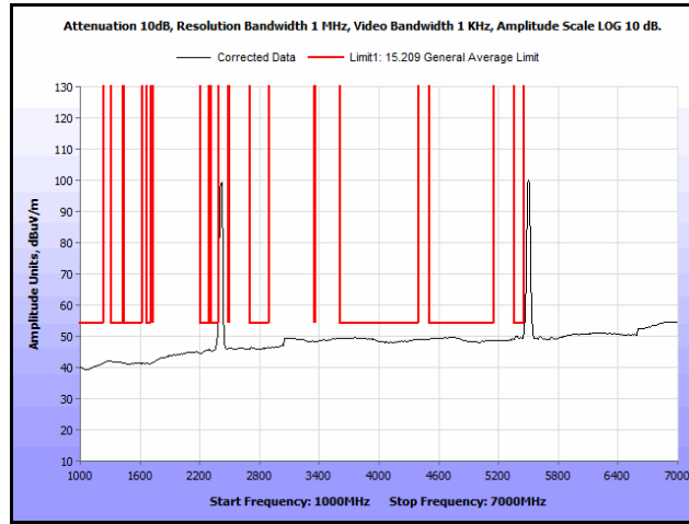
Plot 122. Radiated Spurs, Co-Location, 802.11n 20 MHz, 2412 MHz & 5580 MHz, 1 GHz – 7 GHz, Avg., Omni
