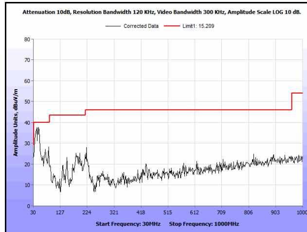
Plot 105. Radiated Spurs, Co-Location, 802.11n 20 MHz, 2437 MHz & 2462 MHz, 30 MHz – 1 GHz, Peak, Omni
