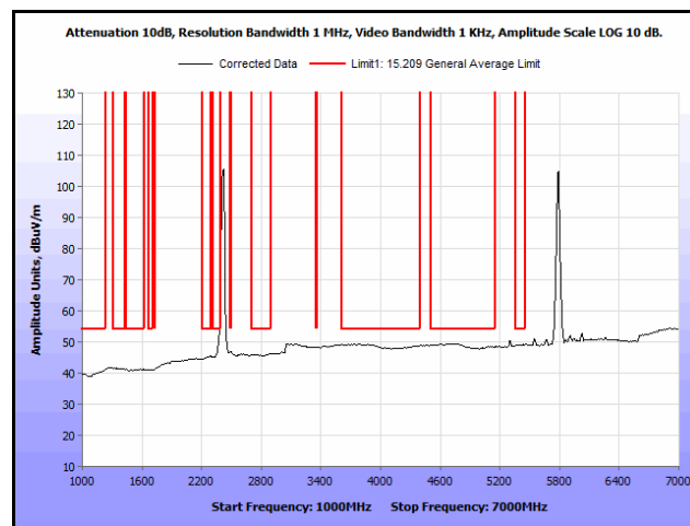
Plot 230. Radiated Spurs, Co-Location, 802.11n 20 MHz, 2437 MHz & 5785 MHz, 1 GHz – 7 GHz, Avg., Patch
