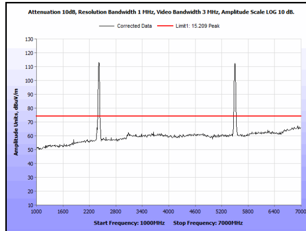
Plot 211. Radiated Spurs, Co-Location, 802.11n 20 MHz, 2412 MHz & 5580 MHz, 1 GHz – 7 GHz, Peak, Patch
