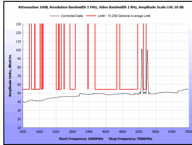
Plot 182. Radiated Spurs, Co-Location, 802.11n 20 MHz, 5300 MHz & 5580 MHz, 1 GHz – 7 GHz, Avg., Omni
