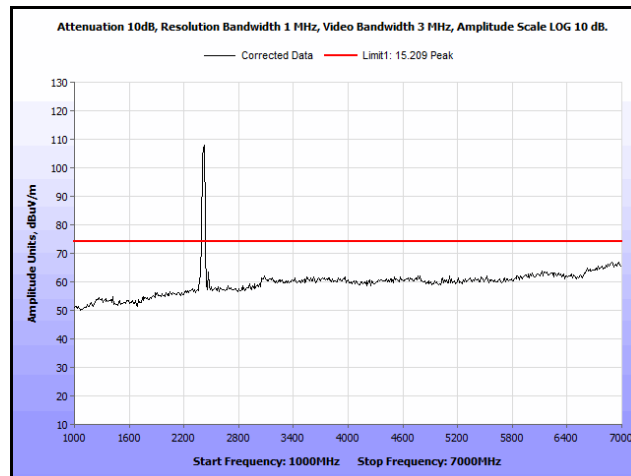
Plot 91. Radiated Spurs, Co-Location, 802.11n 20 MHz, 2412 MHz & 2412 MHz, 1 GHz – 7 GHz, Peak, Omni
