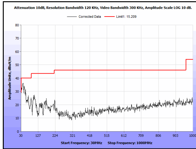
Plot 154. Radiated Spurs, Co-Location, 802.11n 20 MHz, 2462 MHz & 5300 MHz, 30 MHz – 1 GHz, Peak
