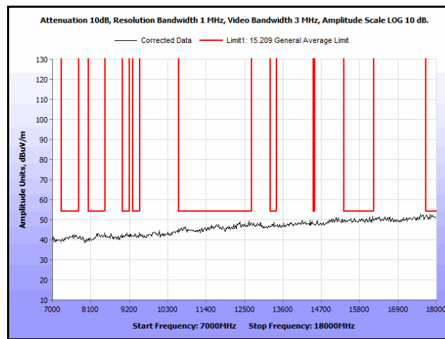
Plot 101. Radiated Spurs, Co-Location, 802.11n 20 MHz, 2412 MHz & 2437 MHz, 7 GHz – 18 GHz, Peak
