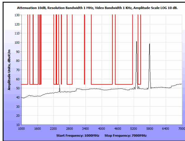
Plot 191. Radiated Spurs, Co-Location, 802.11n 20 MHz, 5300 MHz & 5785 MHz, 1 GHz – 7 GHz, Avg.
