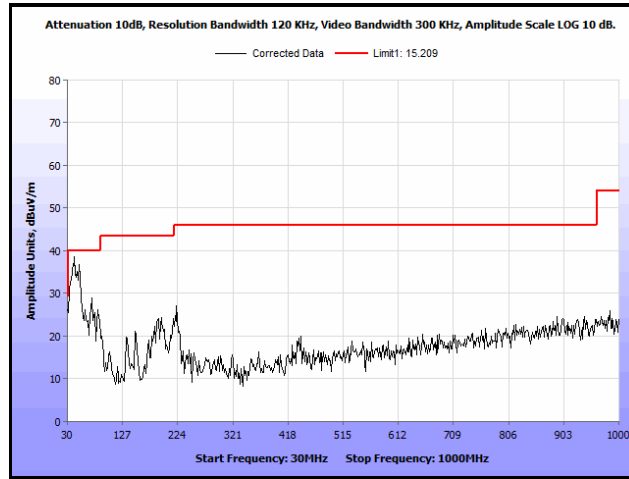
Plot 118. Radiated Spurs, Co-Location, 802.11n 20 MHz, 2412 MHz & 5200 MHz, 30 MHz – 1 GHz, Peak
