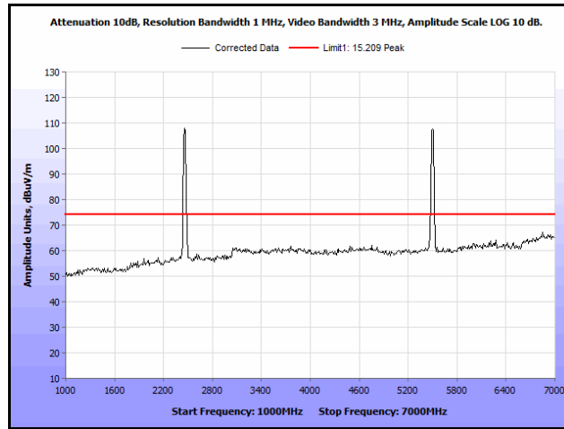
Plot 160. Radiated Spurs, Co-Location, 802.11n 20 MHz, 2462 MHz & 5580 MHz, 1 GHz – 7 GHz, Peak
