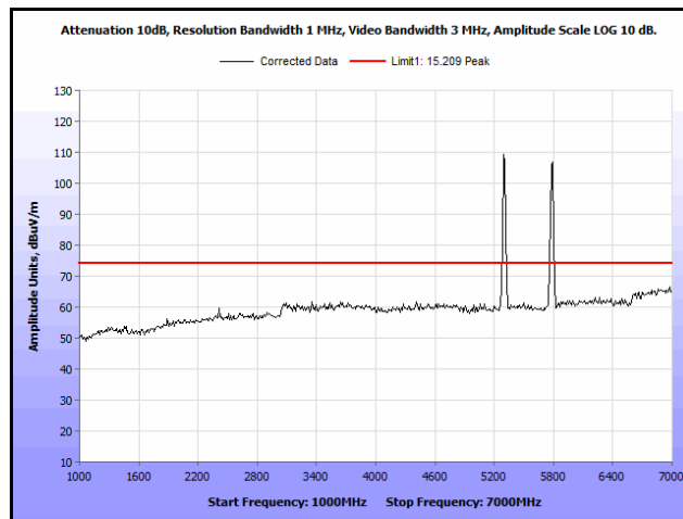
Plot 192. Radiated Spurs, Co-Location, 802.11n 20 MHz, 5300 MHz & 5785 MHz, 1 GHz – 7 GHz, Peak
