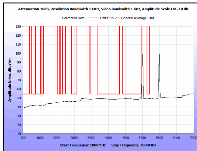
Plot 179. Radiated Spurs, Co-Location, 802.11n 20 MHz, 5200 MHz & 5785 MHz, 1 GHz – 7 GHz, Avg.
