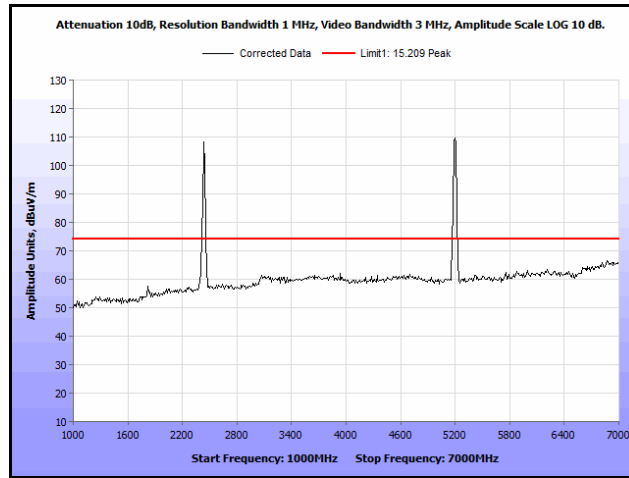
Plot 136. Radiated Spurs, Co-Location, 802.11n 20 MHz, 2437 MHz & 5200 MHz, 1 GHz – 7 GHz, Peak
