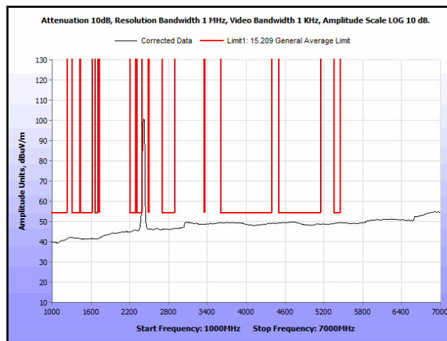
Plot 174. Radiated Spurs, Co-Location, 802.11n 20 MHz, 2412 MHz & 2412 MHz, 1 GHz – 7 GHz, Avg.
