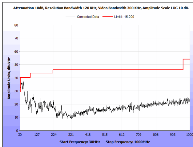
Plot 89. Radiated Spurious Emissions, High Channel, 802.11n 40 MHz, 30 MHz – 1 GHz
