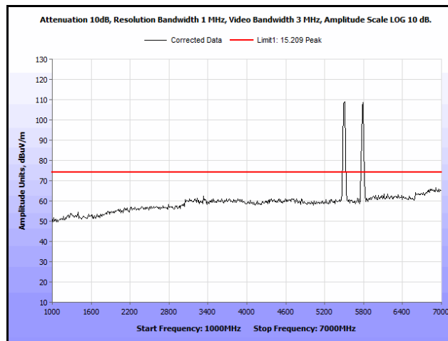
Plot 279. Radiated Spurs, Co-Location, 802.11n 20 MHz, 5580 MHz & 5785 MHz, 1 GHz – 7 GHz, Peak
