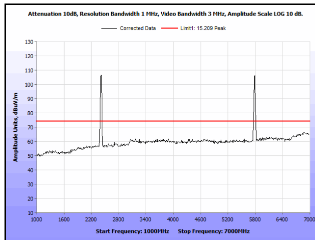
Plot 243. Radiated Spurs, Co-Location, 802.11n 20 MHz, 2462 MHz & 5785 MHz, 1 GHz – 7 GHz, Peak
