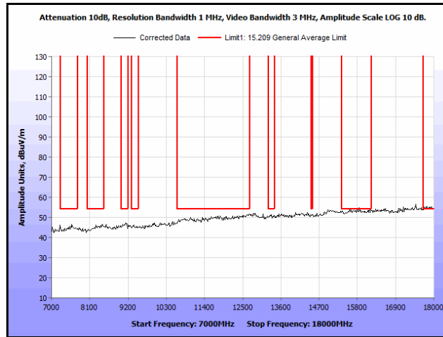
Plot 200. Radiated Spurs, Co-Location, 802.11n 20 MHz, 2412 MHz & 5200 MHz, 7 GHz – 18 GHz
