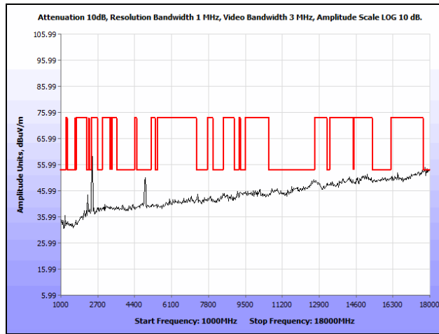
Plot 88. Radiated Spurious Emissions, Mid Channel, 802.11n 40 MHz, 1 GHz – 18 GHz
