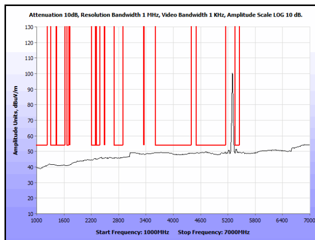
Plot 262. Radiated Spurs, Co-Location, 802.11n 20 MHz, 5300 MHz & 5300 MHz, 1 GHz – 7 GHz, Avg.
