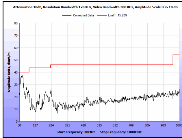
Plot 173. Radiated Spurs, Co-Location, 802.11n 20 MHz, 2412 MHz & 2412 MHz, 30 MHz – 1 GHz, Peak
