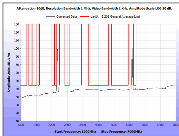
Plot 202. Radiated Spurs, Co-Location, 802.11n 20 MHz, 2412 MHz & 5300 MHz, 1 GHz – 7 GHz, Avg.
