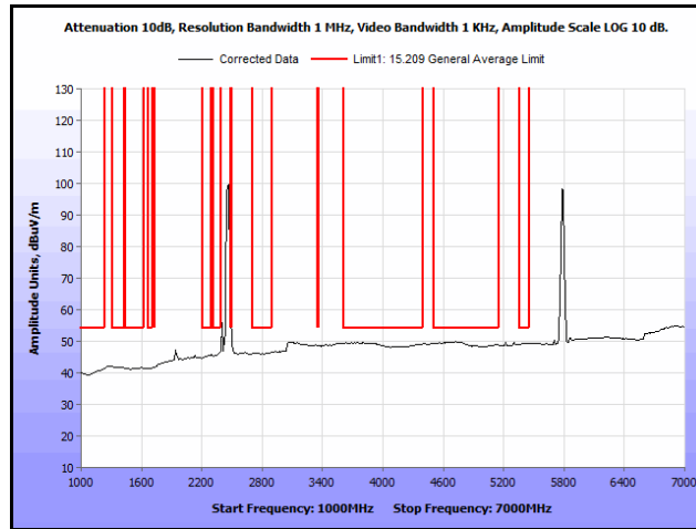
Plot 242. Radiated Spurs, Co-Location, 802.11n 20 MHz, 2462 MHz & 5785 MHz, 1 GHz – 7 GHz, Avg.
