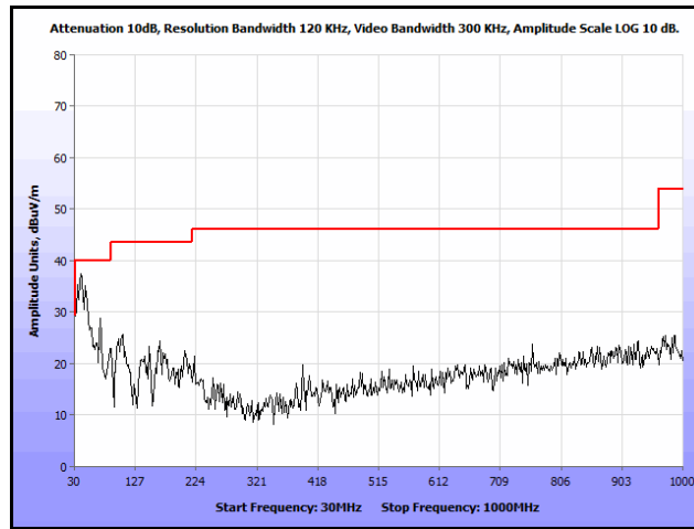
Plot 273. Radiated Spurs, Co-Location, 802.11n 20 MHz, 5580 MHz & 5580 MHz, 30 MHz – 1 GHz, Peak
