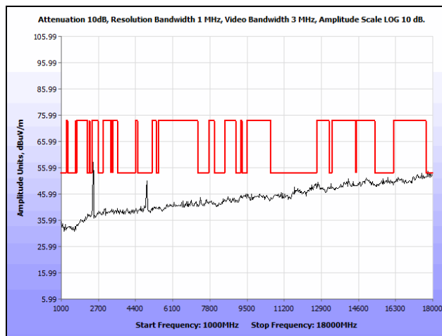
Plot 90. Radiated Spurious Emissions, High Channel, 802.11n 40 MHz, 1 GHz – 18 GHz
