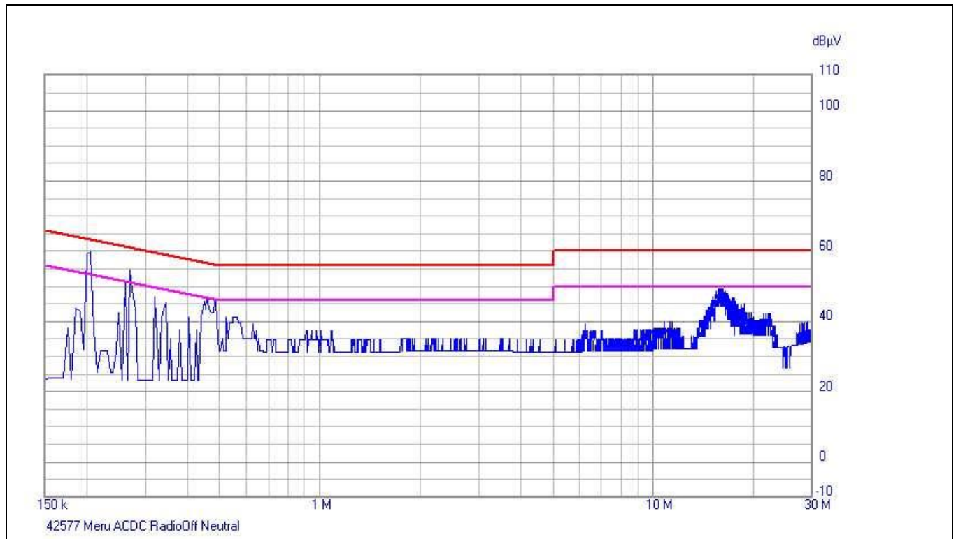
Plot 4. Conducted Emissions, Neutral Line, AC/DC
