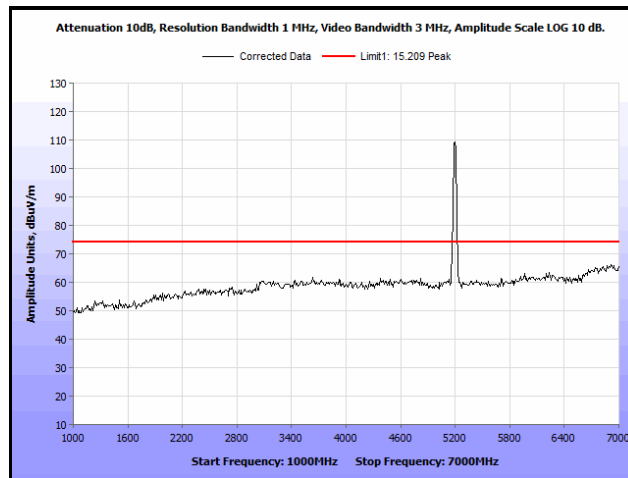
Plot 247. Radiated Spurs, Co-Location, 802.11n 20 MHz, 5200 MHz & 5200 MHz, 1 GHz – 7 GHz, Peak
