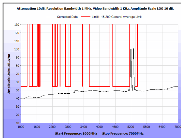
Plot 250. Radiated Spurs, Co-Location, 802.11n 20 MHz, 5200 MHz & 5300 MHz, 1 GHz – 7 GHz, Avg.
