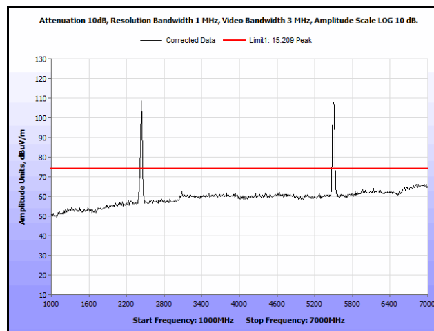
Plot 223. Radiated Spurs, Co-Location, 802.11n 20 MHz, 2437 MHz & 5580 MHz, 1 GHz – 7 GHz, Peak
