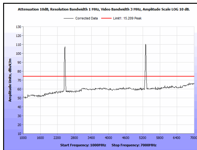
Plot 235. Radiated Spurs, Co-Location, 802.11n 20 MHz, 2462 MHz & 5300 MHz, 1 GHz – 7 GHz, Peak
