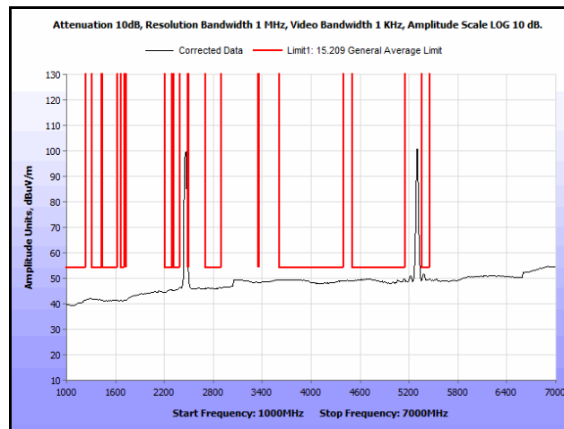
Plot 234. Radiated Spurs, Co-Location, 802.11n 20 MHz, 2462 MHz & 5300 MHz, 1 GHz – 7 GHz, Avg.
