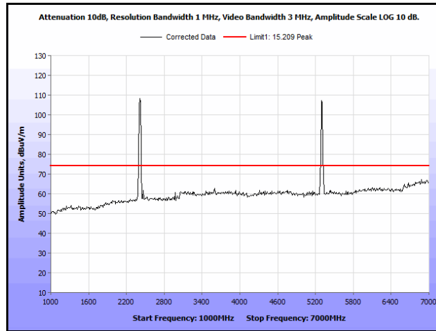
Plot 203. Radiated Spurs, Co-Location, 802.11n 20 MHz, 2412 MHz & 5300 MHz, 1 GHz – 7 GHz, Peak
