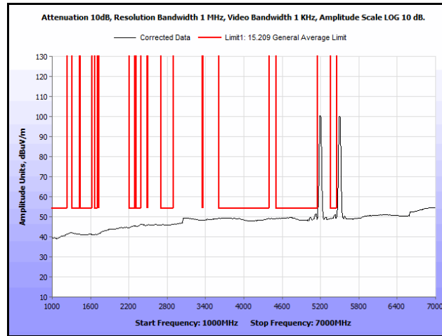
Plot 254. Radiated Spurs, Co-Location, 802.11n 20 MHz, 5200 MHz & 5580 MHz, 1 GHz – 7 GHz, Avg.
