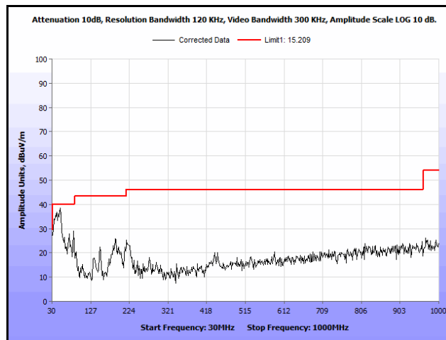
Plot 249. Radiated Spurs, Co-Location, 802.11n 20 MHz, 5200 MHz & 5300 MHz, 30 MHz – 1 GHz, Peak
