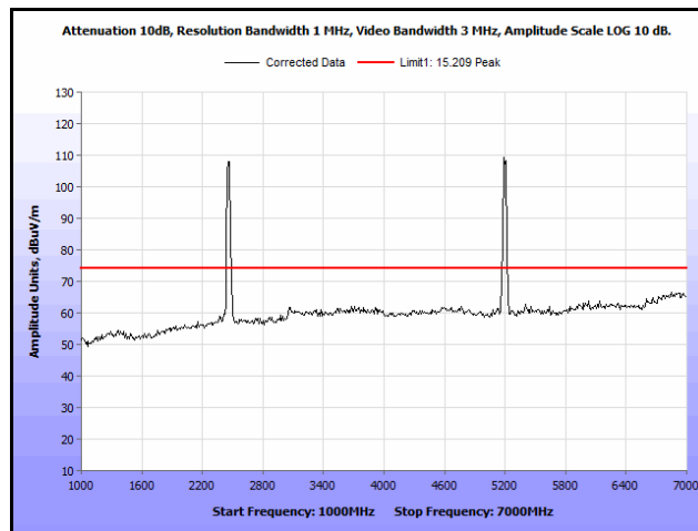
Plot 231. Radiated Spurs, Co-Location, 802.11n 20 MHz, 2462 MHz & 5200 MHz, 1 GHz – 7 GHz, Peak
