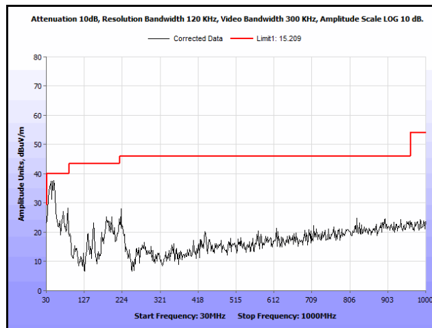
Plot 189. Radiated Spurs, Co-Location, 802.11n 20 MHz, 2437 MHz & 2462 MHz, 30 MHz – 1 GHz, Peak
