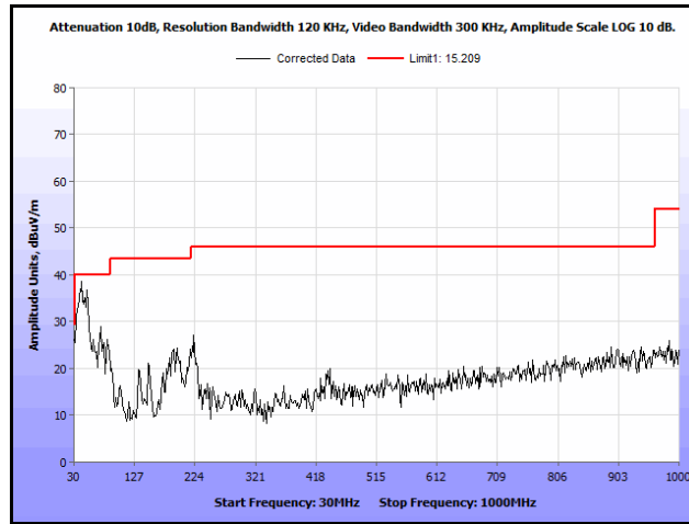
Plot 197. Radiated Spurs, Co-Location, 802.11n 20 MHz, 2412 MHz & 5200 MHz, 30 MHz – 1 GHz, Peak
