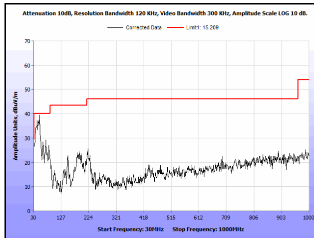
Plot 205. Radiated Spurs, Co-Location, 802.11n 20 MHz, 2412 MHz & 5580 MHz, 30 MHz – 1 GHz, Peak
