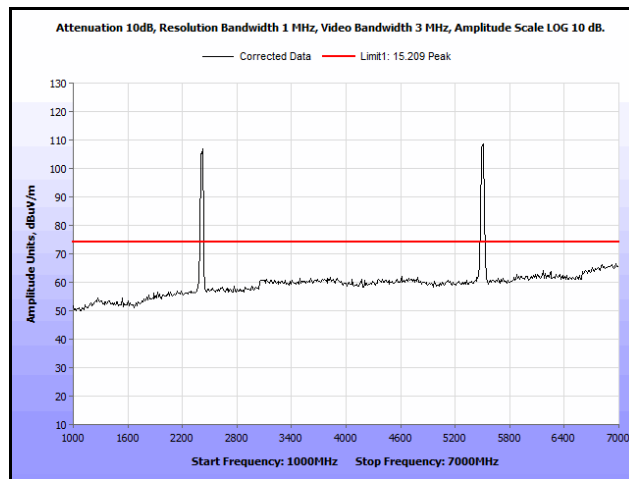
Plot 207. Radiated Spurs, Co-Location, 802.11n 20 MHz, 2412 MHz & 5580 MHz, 1 GHz – 7 GHz, Peak
