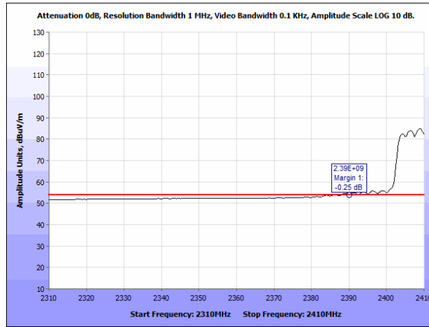
Plot 103. Radiated Restricted Band Edge, 802.11n 40 MHz, 2412 MHz @ 2390 MHz, Average
