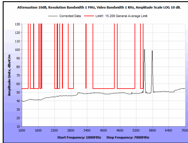
Plot 278. Radiated Spurs, Co-Location, 802.11n 20 MHz, 5580 MHz & 5785 MHz, 1 GHz – 7 GHz, Avg.
