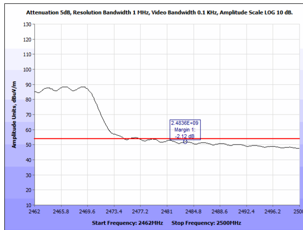
Plot 105. Radiated Restricted Band Edge, 802.11n 40 MHz, 2452 MHz @ 2483.5 MHz, Average
