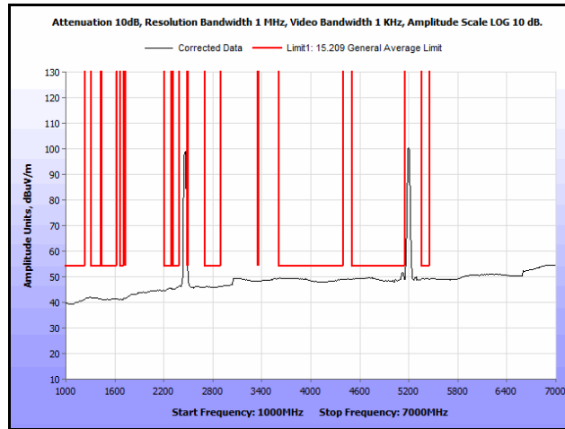
Plot 230. Radiated Spurs, Co-Location, 802.11n 20 MHz, 2462 MHz & 5200 MHz, 1 GHz – 7 GHz, Avg.
