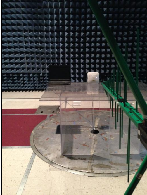
Photograph 3. Radiated Emissions, Test Setup, 30 MHz – 1 GHz
