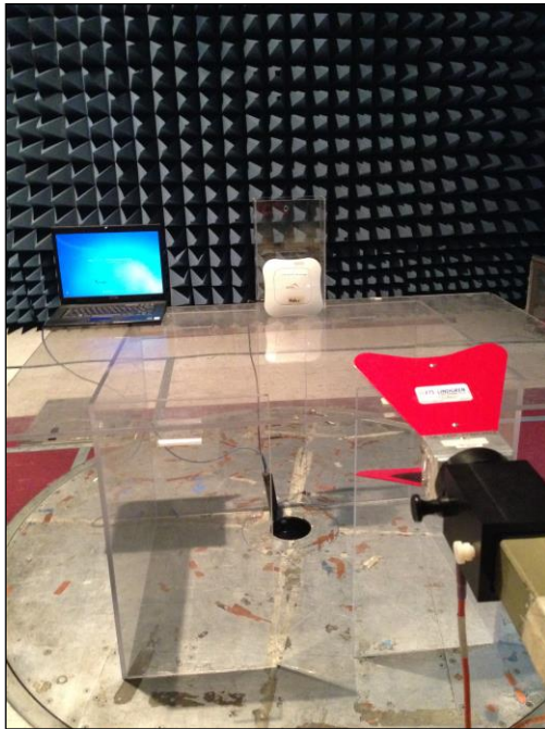
Photograph 6. Radiated Spurious Emissions, Test Setup, 1-18 GHz
