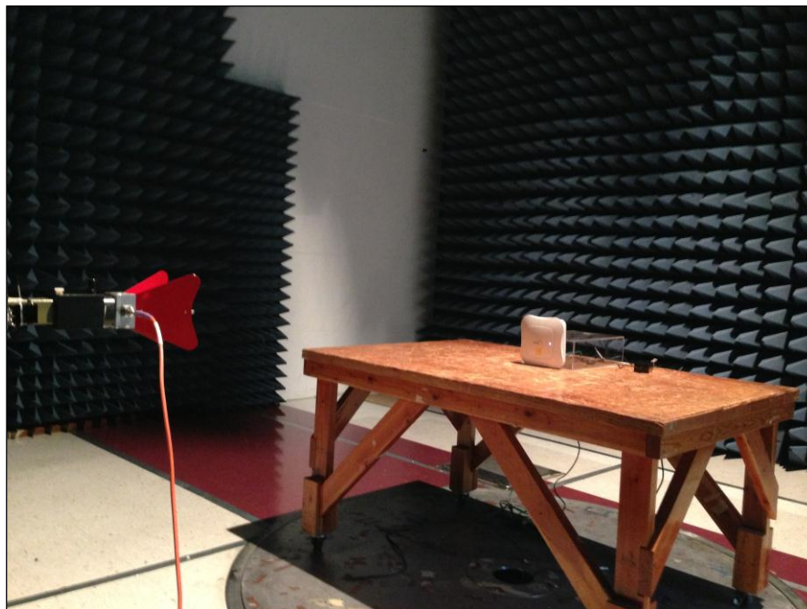
Photograph 10. Radiated Spurious Emissions, Test Setup, Above 1 GHz
