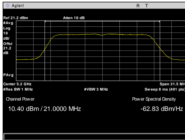
Plot 56. RF Power Output, Mid Channel, 802.11a
