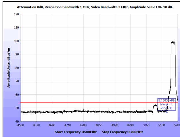
Plot 164. Restricted Band Edge, 802.11n 20 MHz, 5180 MHz, Low Channel @ 5150 MHz Edge, Average
