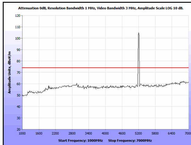
Plot 172. Co-location, Radiated Spurious Emissions, PIFA, 802.11n 20 MHz, 5200 & 5200 MHz, 1 GHz – 7 GHz, Peak
