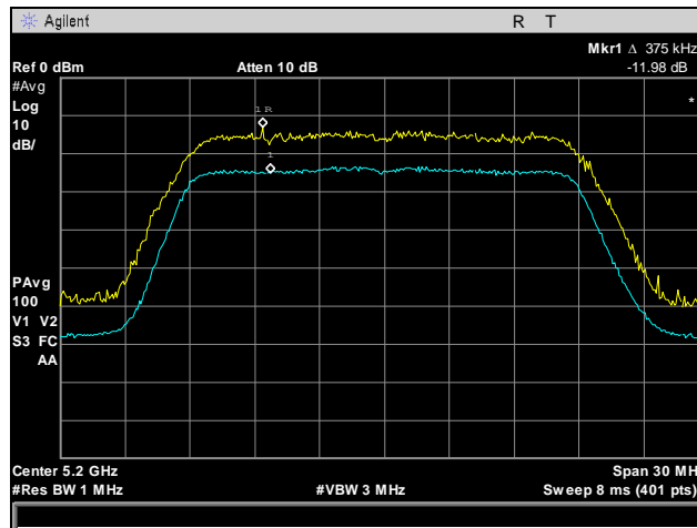
Plot 107. Peak Excursion Ratio, Mid Channel, 802.11n 20 MHz, Port 3
