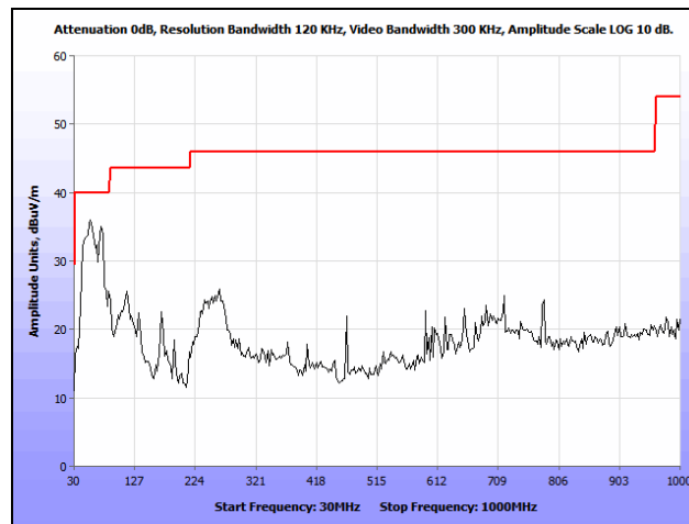
Plot 126. Radiated Spurious Emissions, 802.11a, High Channel, 30 MHz – 1 GHz, Internal
