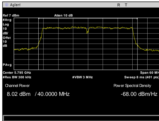
Plot 70. RF Power Output, High Channel, 802.11n 40 MHz, Port 2
