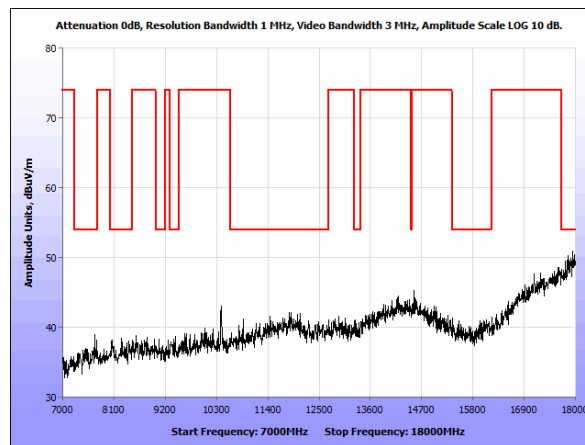
Plot 137. Radiated Spurious Emissions, 802.11n 20 MHz, Mid Channel, 7 GHz – 18 GHz, Peak, Internal
