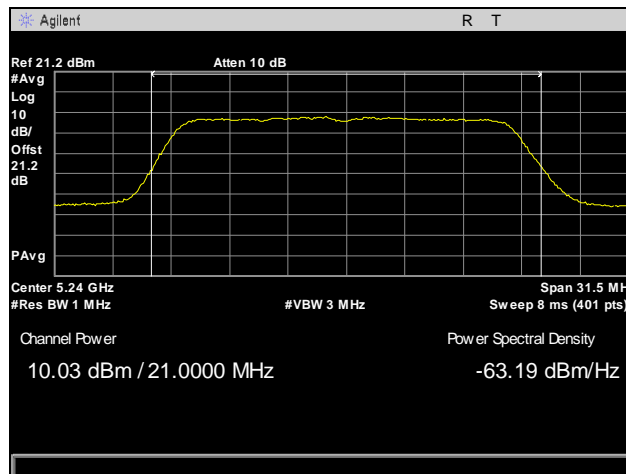
Plot 57. RF Power Output, High Channel, 802.11a
