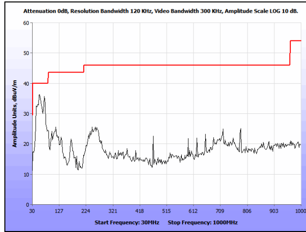
Plot 130. Radiated Spurious Emissions, 802.11n 20 MHz, Low Channel, 30 MHz – 1 GHz, Internal
