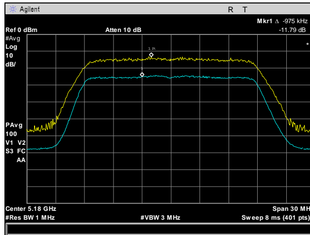
Plot 106. Peak Excursion Ratio, Low Channel, 802.11n 20 MHz, Port 3
