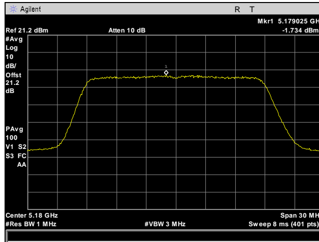
Plot 79. Power Spectral Density, Low Channel, 802.11n 20 MHz, Port 1
