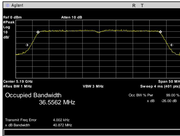
Plot 29. 26 dB Occupied Bandwidth, 802.11n 40 MHz, Port 3, Low Channel
