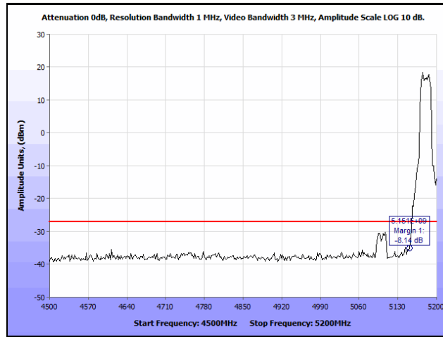
Plot 156. Radiated Band Edge 802.11n 20 MHz, Low Channel, Internal Antenna (Band Edge @ 5150 MHz)
