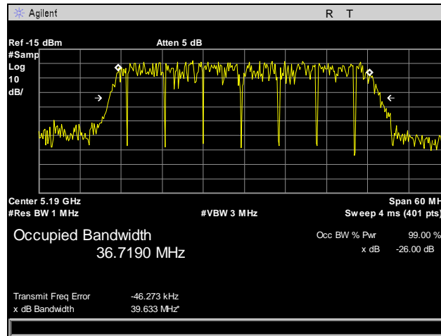
Plot 48. 99% Occupied Bandwidth, 802.11n 40 MHz, Port 2, Low Channel
