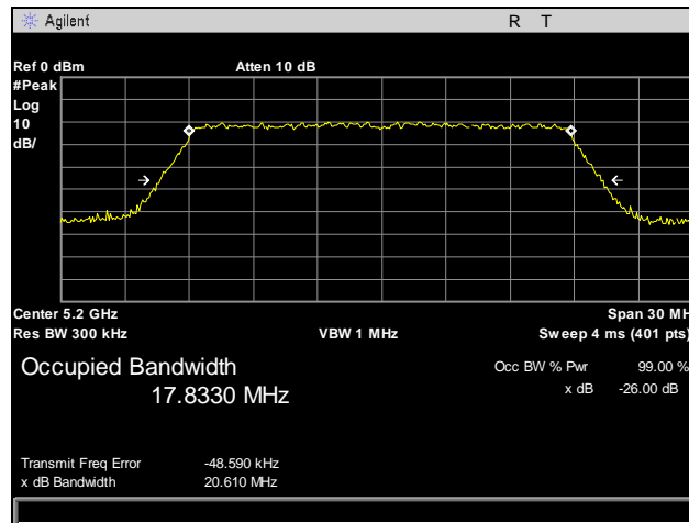
Plot 23. 26 dB Occupied Bandwidth, 802.11n 20 MHz, Port 3, Mid Channel
