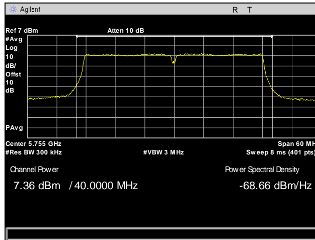
Plot 69. RF Power Output, Low Channel, 802.11n 40 MHz, Port 2
