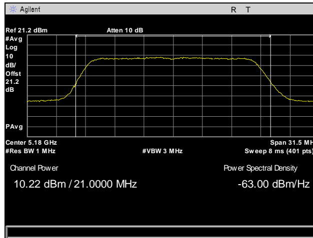
Plot 55. RF Power Output, Low Channel, 802.11a
