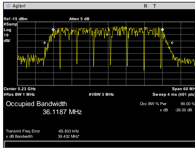
Plot 51. 99% Occupied Bandwidth, 802.11n 40 MHz, Port 3, High Channel
