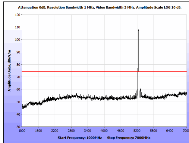
Plot 140. Radiated Spurious Emissions, 802.11n 20 MHz, High Channel, 1 GHz – 7 GHz, Peak, Internal
