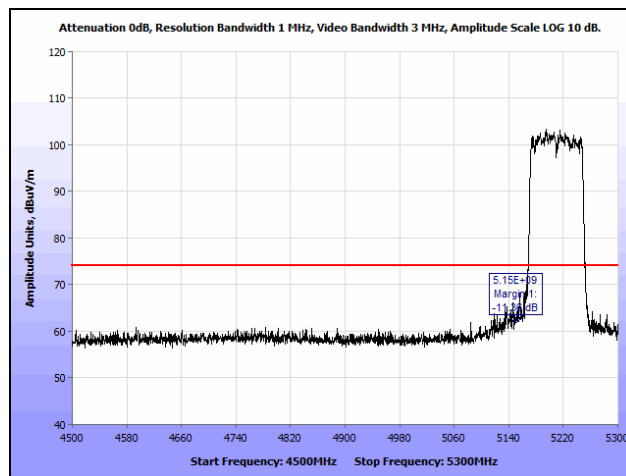
Plot 169. Restricted Band Edge, 802.11n 80 MHz, 5210 MHz @ 5150 MHz Edge, Peak
