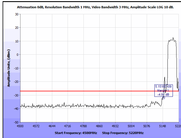
Plot 158. Radiated Band Edge 802.11n 40 MHz, Low Channel, Internal Antenna (Band Edge @ 5150 MHz)
