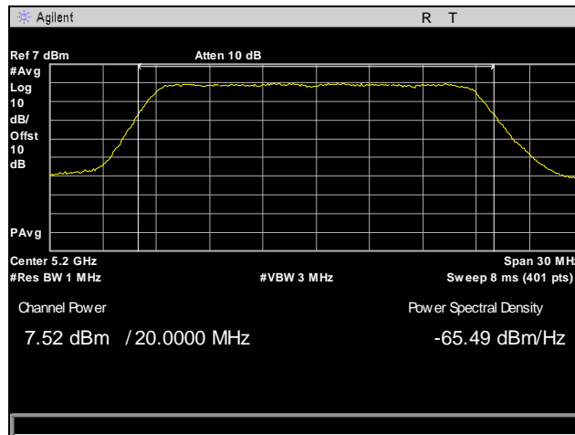
Plot 59. RF Power Output, Mid Channel, 802.11n 20 MHz, Port 1
