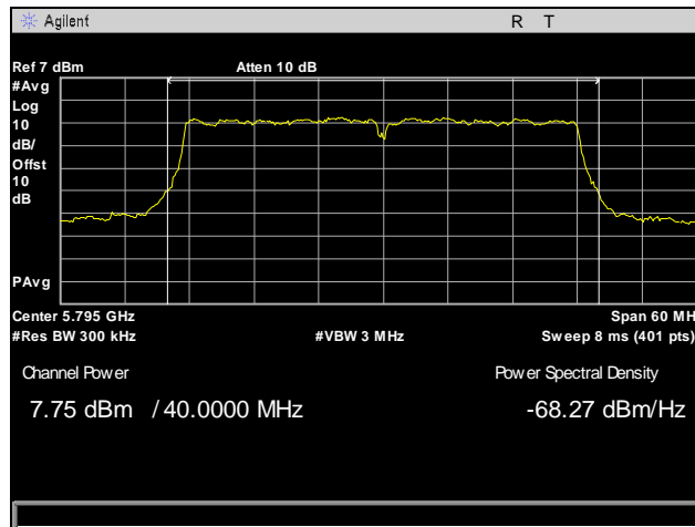
Plot 72. RF Power Output, High Channel, 802.11n 40 MHz, Port 3
