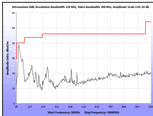
Plot 178. Co-location, Radiated Spurious Emissions, PIFA, 802.11n 20 MHz, 5200 & 5580 MHz, 30 MHz – 1 GHz
