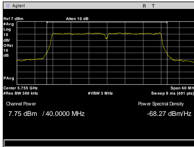
Plot 71. RF Power Output, Low Channel, 802.11n 40 MHz, Port 3
