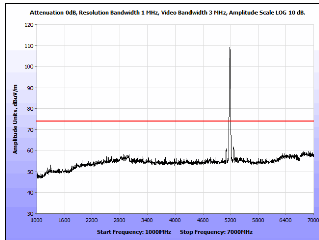
Plot 132. Radiated Spurious Emissions, 802.11n 20 MHz, Low Channel, 1 GHz – 7 GHz, Peak, Internal
