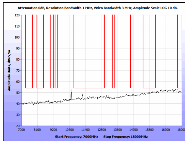
Plot 181. Co-location, Radiated Spurious Emissions, PIFA, 802.11n 20 MHz, 5200 & 5580 MHz, 7 GHz – 18 GHz, Peak
