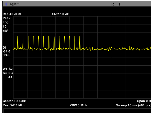
Plot 574. Radar Type 4 Calibration, 5300 MHz
