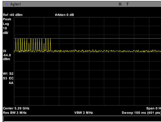
Plot 563. Radar Type 0 Calibration, 5290 MHz
