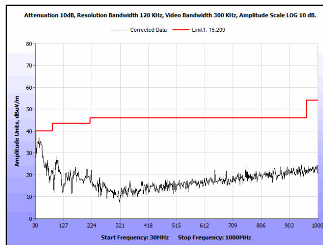
Plot 437. Radiated Spurs, Co-Location, 802.11n 20 MHz, 2462 MHz & 5200 MHz, 30 MHz – 1 GHz, Peak, Omni
