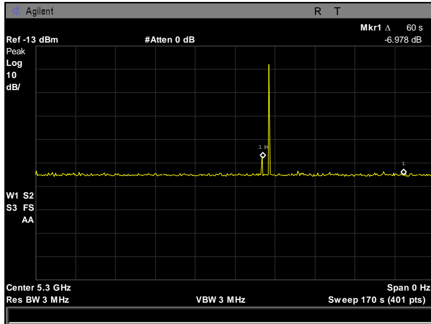
Plot 589. Radar Burst at the End of CACT, 5300 MHz
