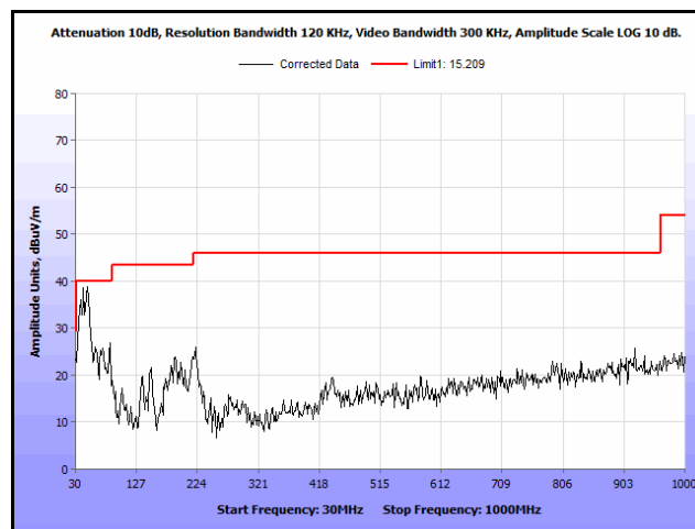
Plot 389. Radiated Spurs, Co-Location, 802.11n 20 MHz, 2412 MHz & 2462 MHz, 30 MHz – 1 GHz, Peak, Omni
