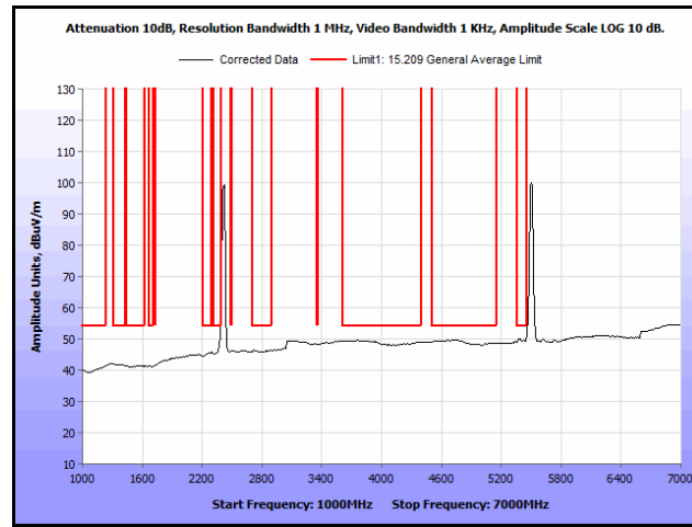
Plot 414. Radiated Spurs, Co-Location, 802.11n 20 MHz, 2412 MHz & 5580 MHz, 1 GHz – 7 GHz, Avg., Omni
