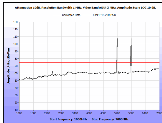
Plot 467. Radiated Spurs, Co-Location, 802.11n 20 MHz, 5200 MHz & 5785 MHz, 1 GHz – 7 GHz, Peak, Omni
