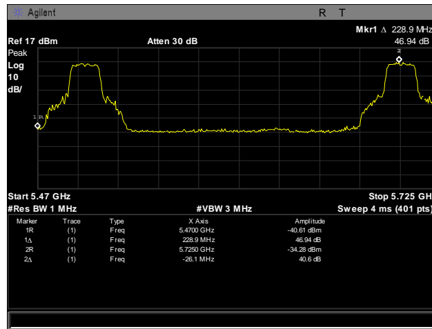
Plot 552. Frequency Stability, 5470 – 5725 MHz, -40°C, 120 V
