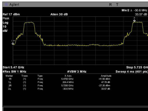
Plot 554. Frequency Stability, 5470 – 5725 MHz, -20°C, 120 V
