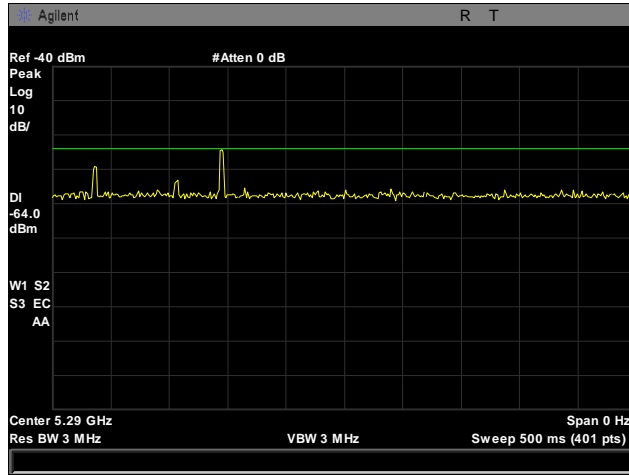
Plot 569. Radar Type 6 Calibration, 5290 MHz
