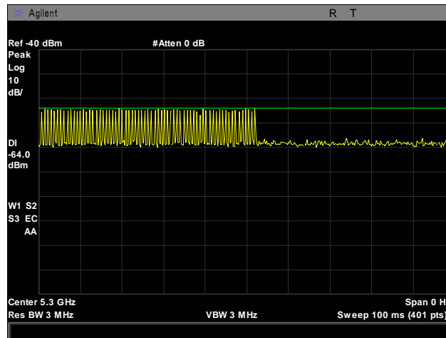
Plot 571. Radar Type 1 Calibration, 5300 MHz
