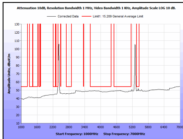
Plot 498. Radiated Spurs, Co-Location, 802.11n 20 MHz, 2412 MHz & 5300 MHz, 1 GHz – 7 GHz, Avg., Patch
