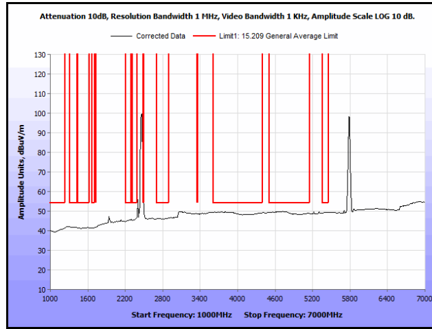
Plot 450. Radiated Spurs, Co-Location, 802.11n 20 MHz, 2462 MHz & 5785 MHz, 1 GHz – 7 GHz, Avg., Omni
