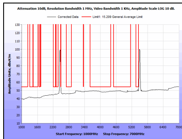
Plot 446. Radiated Spurs, Co-Location, 802.11n 20 MHz, 2462 MHz & 5580 MHz, 1 GHz – 7 GHz, Avg., Omni
