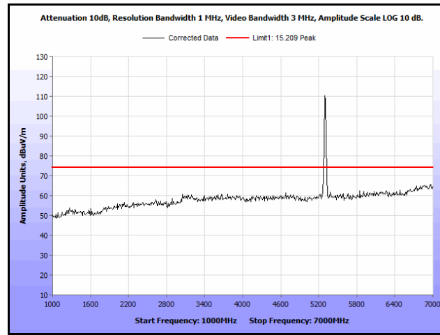
Plot 471. Radiated Spurs, Co-Location, 802.11n 20 MHz, 5300 MHz & 5300 MHz, 1 GHz – 7 GHz, Peak, Omni
