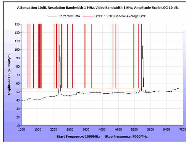
Plot 502. Radiated Spurs, Co-Location, 802.11n 20 MHz, 2412 MHz & 5580 MHz, 1 GHz – 7 GHz, Avg., Patch
