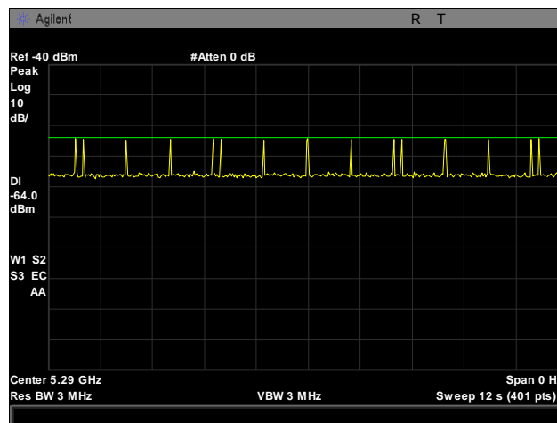
Plot 568. Radar Type 5 Calibration, 5290 MHz
