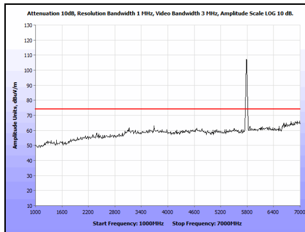
Plot 491. Radiated Spurs, Co-Location, 802.11n 20 MHz, 5785 MHz & 5785 MHz, 1 GHz – 7 GHz, Peak, Omni
