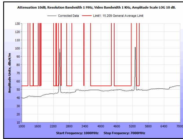
Plot 426. Radiated Spurs, Co-Location, 802.11n 20 MHz, 2437 MHz & 5300 MHz, 1 GHz – 7 GHz, Avg., Omni
