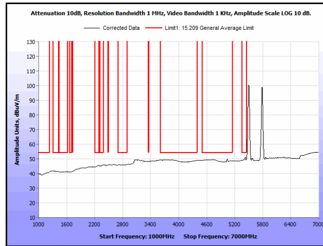
Plot 486. Radiated Spurs, Co-Location, 802.11n 20 MHz, 5580 MHz & 5785 MHz, 1 GHz – 7 GHz, Avg., Omni
