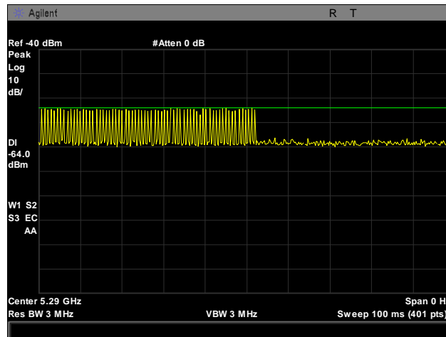
Plot 564. Radar Type 1 Calibration, 5290 MHz
