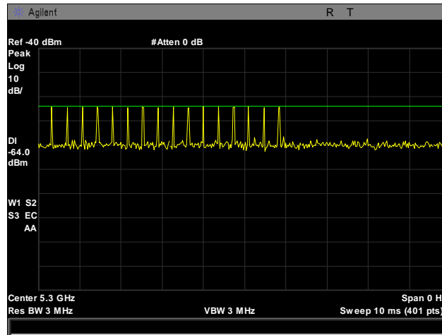
Plot 573. Radar Type 3 Calibration, 5300 MHz
