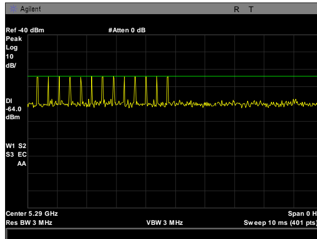
Plot 567. Radar Type 4 Calibration, 5290 MHz
