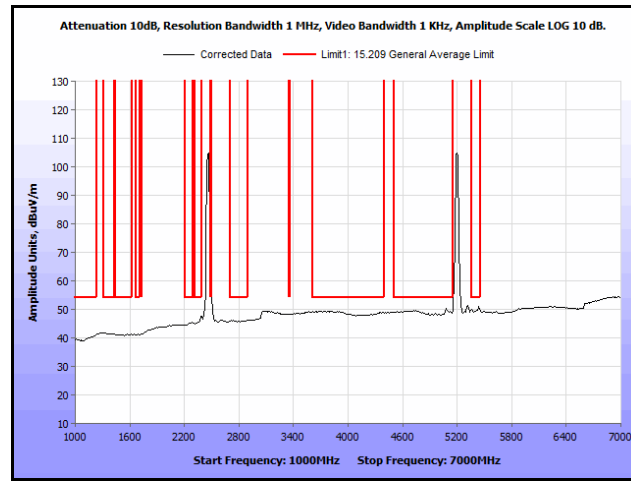
Plot 526. Radiated Spurs, Co-Location, 802.11n 20 MHz, 2462 MHz & 5200 MHz, 1 GHz – 7 GHz, Avg., Patch
