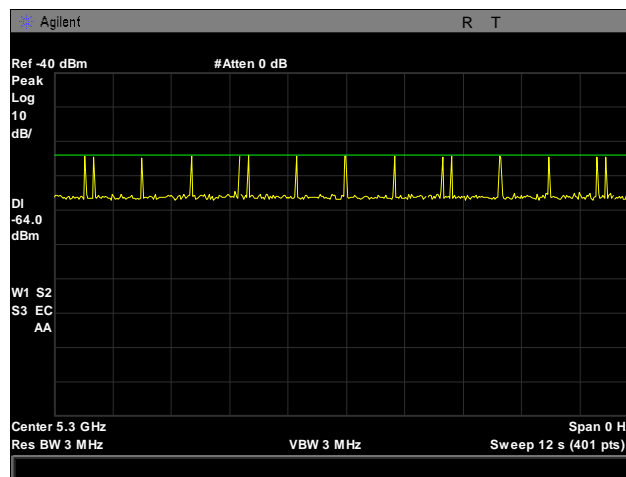
Plot 575. Radar Type 5 Calibration, 5300 MHz
