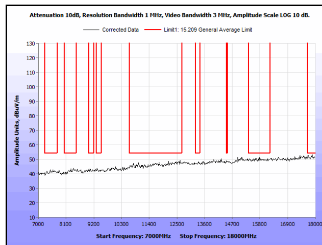
Plot 528. Radiated Spurs, Co-Location, 802.11n 20 MHz, 2462 MHz & 5200 MHz, 7 GHz – 18 GHz, Peak, Patch
