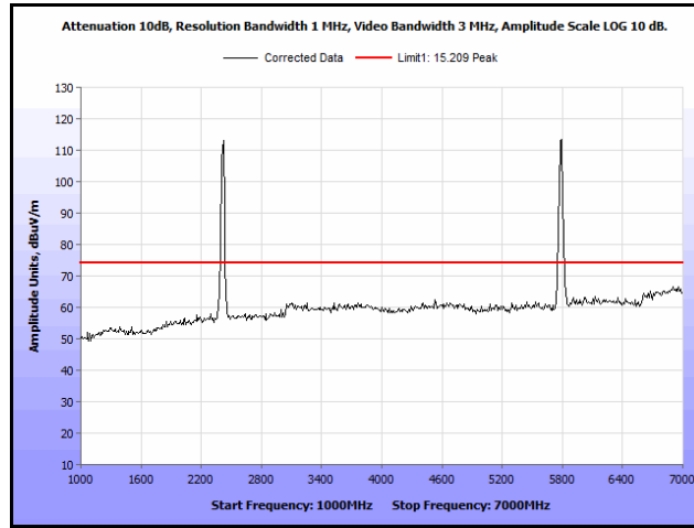
Plot 523. Radiated Spurs, Co-Location, 802.11n 20 MHz, 2437 MHz & 5785 MHz, 1 GHz – 7 GHz, Peak, Patch
