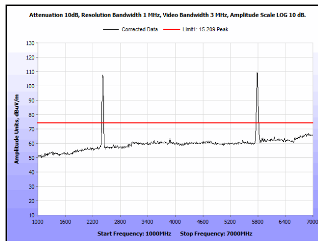
Plot 419. Radiated Spurs, Co-Location, 802.11n 20 MHz, 2412 MHz & 5785 MHz, 1 GHz – 7 GHz, Peak, Omni
