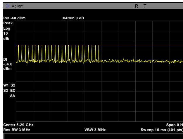
Plot 565. Radar Type 2 Calibration, 5290 MHz
