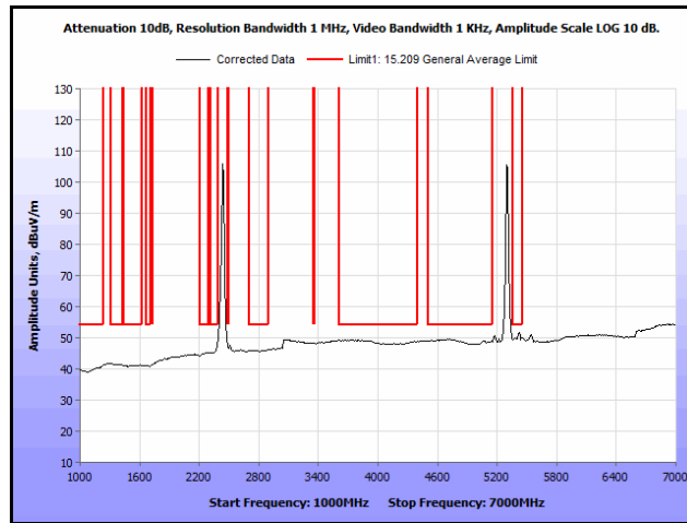
Plot 514. Radiated Spurs, Co-Location, 802.11n 20 MHz, 2437 MHz & 5300 MHz, 1 GHz – 7 GHz, Avg., Patch
