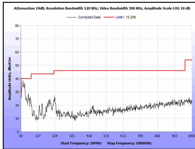
Plot 493. Radiated Spurs, Co-Location, 802.11n 20 MHz, 2412 MHz & 5200 MHz, 30 MHz – 1 GHz, Peak, Patch
