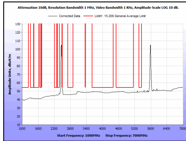
Plot 538. Radiated Spurs, Co-Location, 802.11n 20 MHz, 2462 MHz & 5785 MHz, 1 GHz – 7 GHz, Avg., Patch
