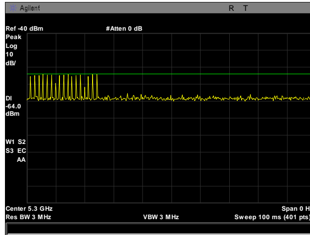
Plot 570. Radar Type 0 Calibration, 5300 MHz
