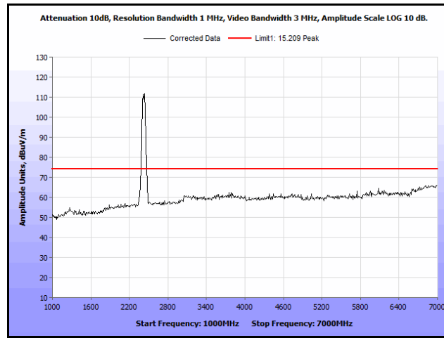
Plot 387. Radiated Spurs, Co-Location, 802.11n 20 MHz, 2412 MHz & 2437 MHz, 1 GHz – 7 GHz, Peak, Omni
