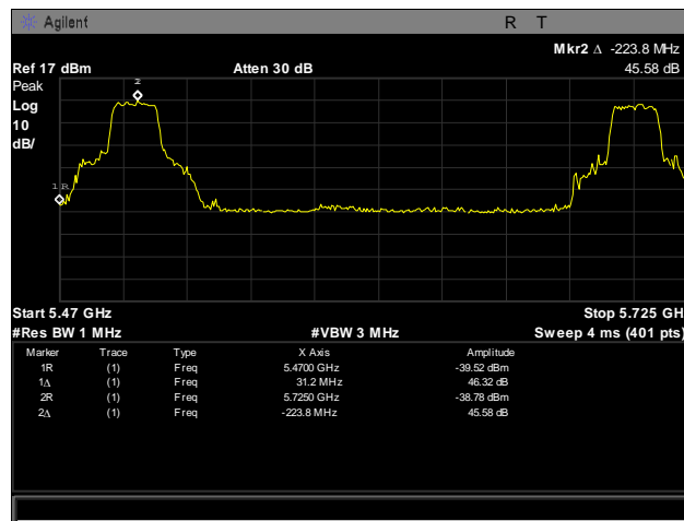
Plot 553. Frequency Stability, 5470 – 5725 MHz, -30°C, 120 V
