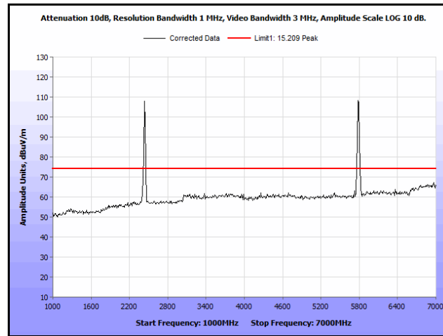
Plot 435. Radiated Spurs, Co-Location, 802.11n 20 MHz, 2437 MHz & 5785 MHz, 1 GHz – 7 GHz, Peak, Omni
