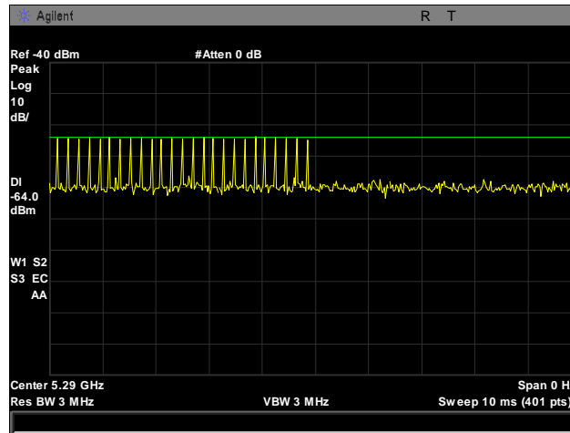
Plot 566. Radar Type 3 Calibration, 5290 MHz
