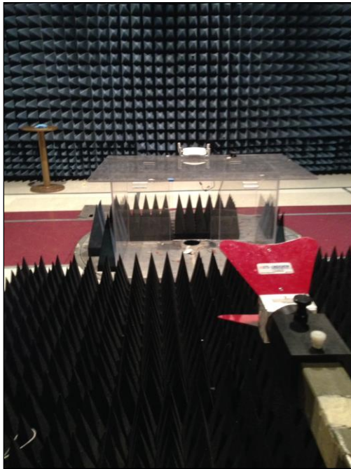
Photograph 4. Radiated Emissions, Test Setup, 1 GHz – 2 GHz
