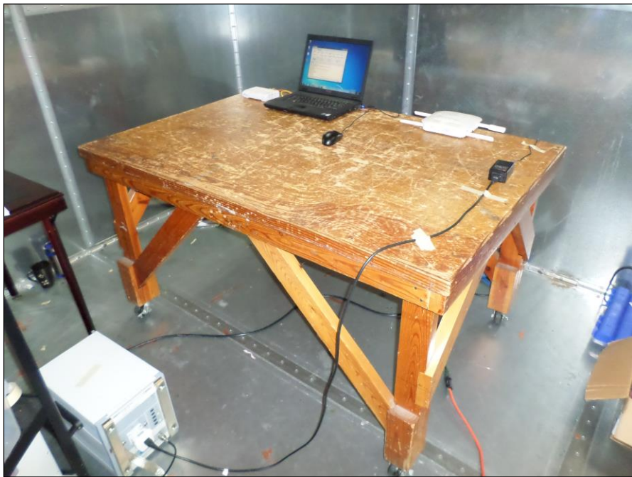
Photograph 2. Conducted Emissions, Test Setup, AC/DC
