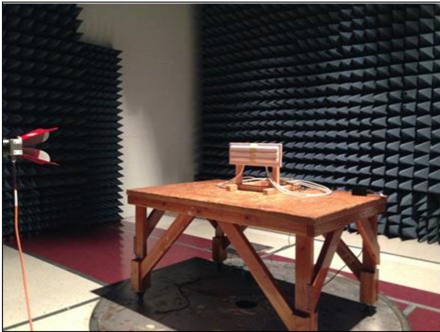
Photograph 10. Radiated Spurious Emissions, Test Setup, Above 1 GHz, Patch Antenna
