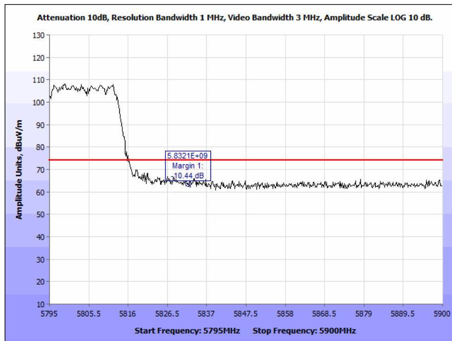
Plot 183. Radiated Band Edge, 802.11n 40 MHz, High Channel, Omni Antenna (5832 & 5835 MHz), Peak
