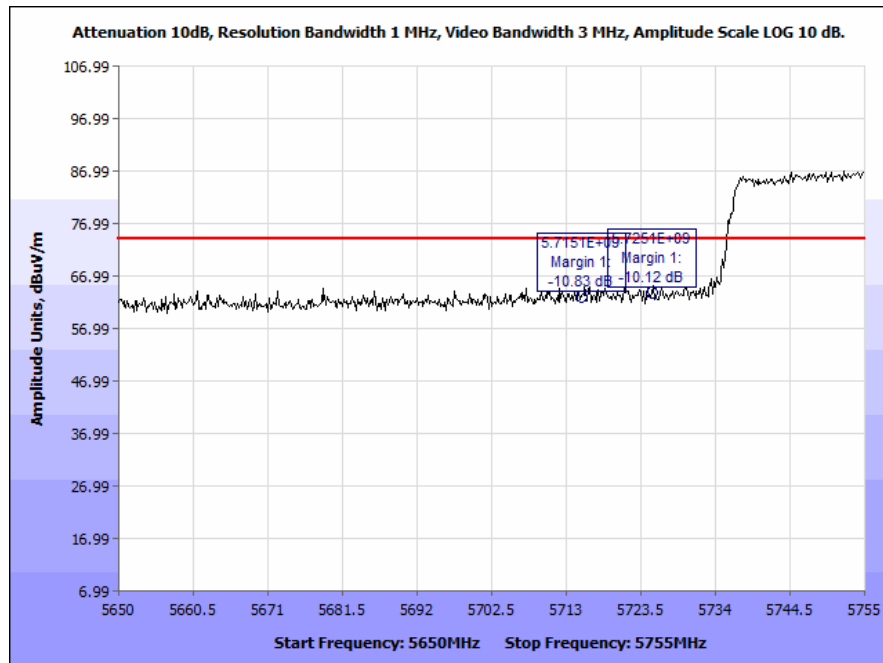
Plot 201. Radiated Band Edge, 802.11n 80 MHz, Patch Antenna (5725 & 5715 MHz), Peak
