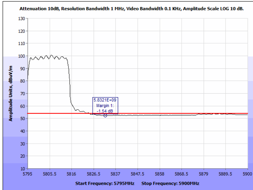
Plot 174. Radiated Band Edge, 802.11a, High Channel, Omni Antenna (5832 & 5835 MHz), Average
