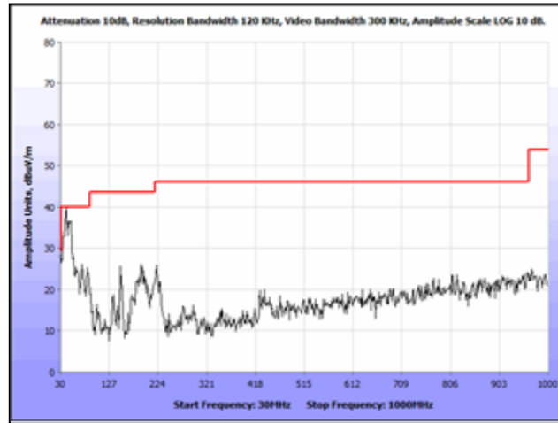
Plot 76. Radiated Spurious Emissions, 802.11a 40 MHz, Low Channel, 30 MHz – 1 GHz, Omni Antenna
