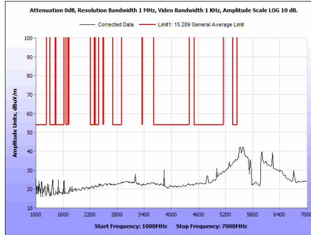
Plot 88. Radiated Spurious Emissions, 802.11a 40 MHz, High Channel, 1 GHz – 7 GHz, Average, Omni Antenna
