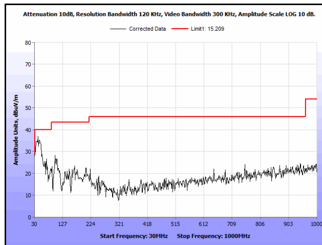
Plot 348. Radiated Spurs, Co-Location, 802.11n 20 MHz, 2462 MHz & 5200 MHz, 30 MHz – 1 GHz, Peak, Patch
