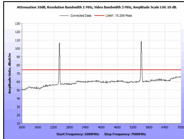
Plot 238. Radiated Spurs, Co-Location, 802.11n 20 MHz, 2412 MHz & 5580 MHz, 1 GHz – 7 GHz, Peak, Omni
