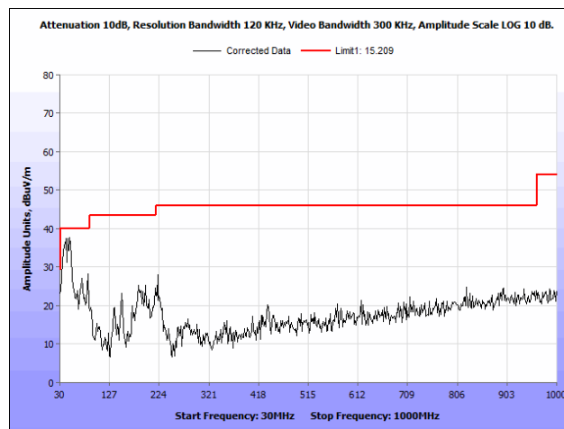
Plot 45. Radiated Spurious Emissions, 802.11a 40 MHz, High Channel, 30 MHz – 1 GHz, Ceiling Antenna
