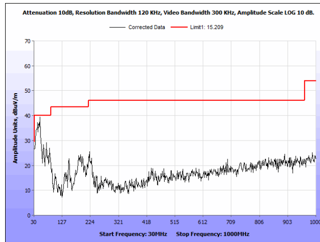
Plot 53. Radiated Spurious Emissions, 802.11n 40 MHz, Low Channel, 30 MHz – 1 GHz, Ceiling Antenna
