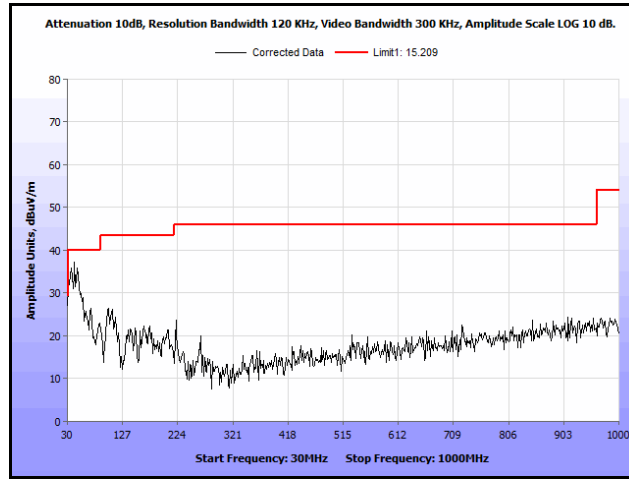
Plot 340. Radiated Spurs, Co-Location, 802.11n 20 MHz, 2437 MHz & 5580 MHz, 30 MHz – 1 GHz, Peak, Patch
