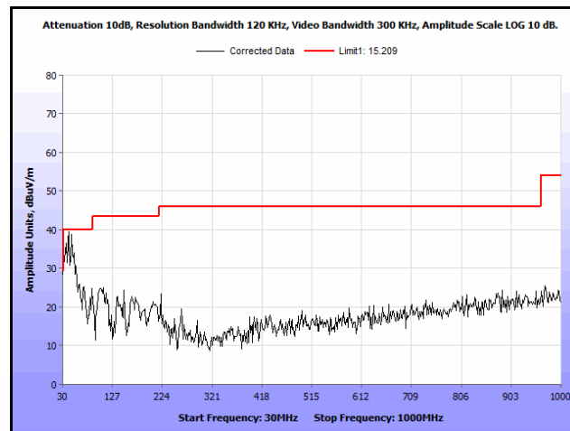
Plot 268. Radiated Spurs, Co-Location, 802.11n 20 MHz, 2462 MHz & 5580 MHz, 30 MHz – 1 GHz, Peak, Omni
