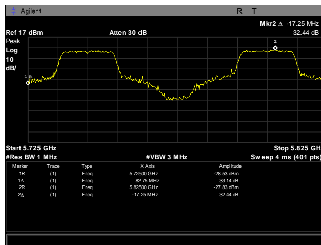
Plot 374. Frequency Stability, 5725 – 5825 MHz, 55°C, 120 V
