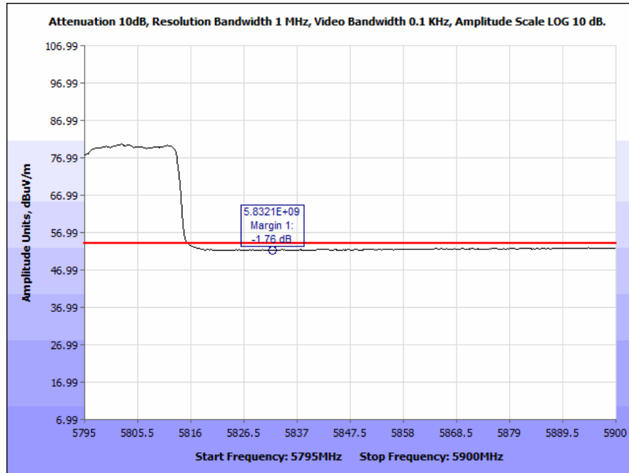
Plot 186. Radiated Band Edge, 802.11ac 80 MHz, Omni Antenna (5832 & 5835 MHz), Average
