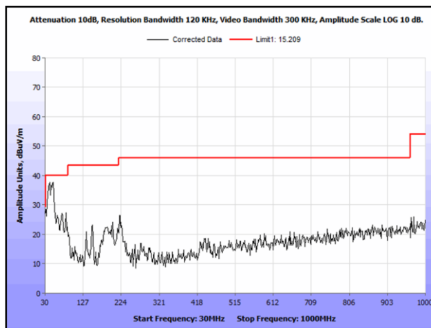
Plot 105. Radiated Spurious Emissions, 802.11n 40 MHz, High Channel, 30 MHz – 1 GHz, Omni Antenna
