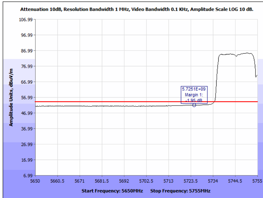
Plot 180. Radiated Band Edge, 802.11n 40 MHz, Low Channel, Omni Antenna (5715 & 5725 MHz), Average
