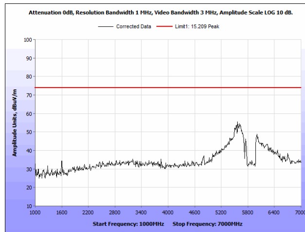
Plot 89. Radiated Spurious Emissions, 802.11a 40 MHz, High Channel, 1 GHz – 7 GHz, Peak, Omni Antenna
