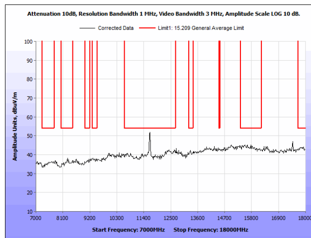
Plot 86. Radiated Spurious Emissions, 802.11a 20 MHz, High Channel, 7 GHz – 18 GHz, Omni Antenna
