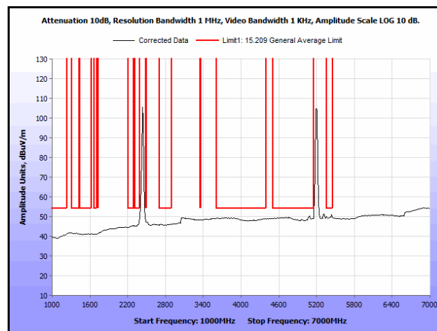
Plot 333. Radiated Spurs, Co-Location, 802.11n 20 MHz, 2437 MHz & 5200 MHz, 1 GHz – 7 GHz, Avg., Patch
