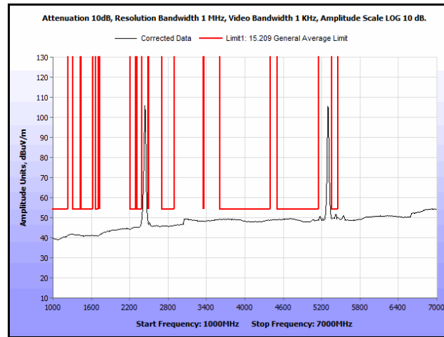
Plot 337. Radiated Spurs, Co-Location, 802.11n 20 MHz, 2437 MHz & 5300 MHz, 1 GHz – 7 GHz, Avg., Patch
