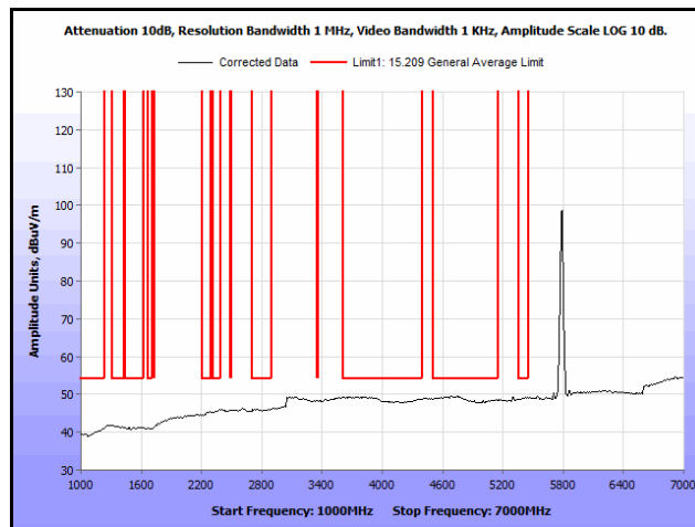
Plot 313. Radiated Spurs, Co-Location, 802.11n 20 MHz, 5785 MHz & 5785 MHz, 1 GHz – 7 GHz, Avg., Omni
