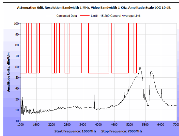
Plot 70. Radiated Spurious Emissions, 802.11ac 80 MHz, 1 GHz – 7 GHz, Average, Ceiling Antenna
