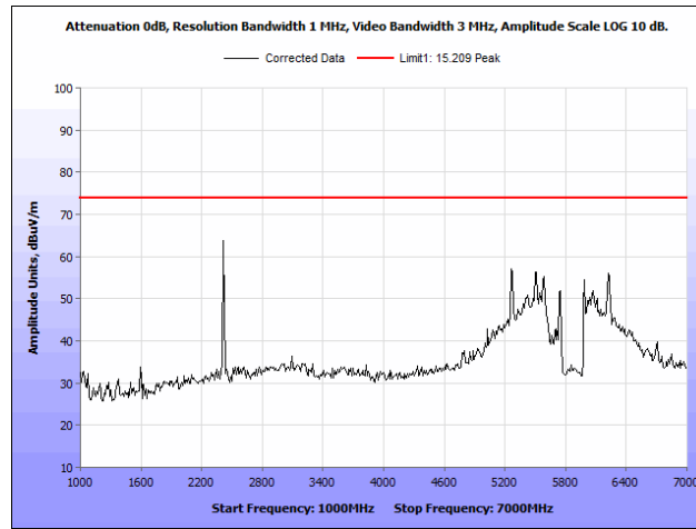
Plot 92. Radiated Spurious Emissions, 802.11n 20 MHz, Low Channel, 1 GHz – 7 GHz, Peak, Omni Antenna
