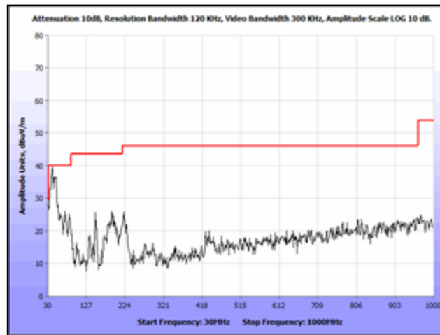
Plot 80. Radiated Spurious Emissions, 802.11a 20 MHz, Mid Channel, 30 MHz – 1 GHz, Omni Antenna
