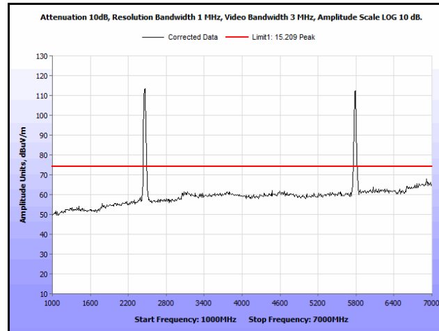
Plot 362. Radiated Spurs, Co-Location, 802.11n 20 MHz, 2462 MHz & 5785 MHz, 1 GHz – 7 GHz, Peak, Patch
