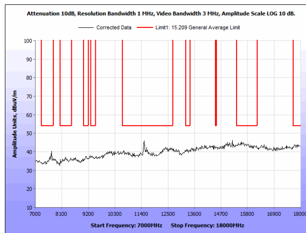
Plot 108. Radiated Spurious Emissions, 802.11n 40 MHz, High Channel, 7 GHz – 18 GHz, Peak, Omni Antenna
