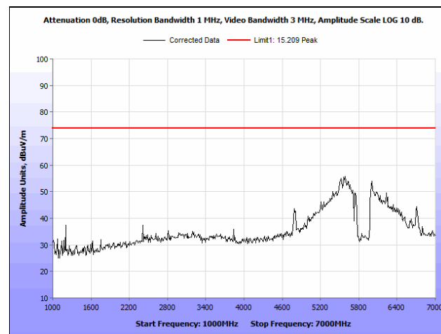
Plot 96. Radiated Spurious Emissions, 802.11n 40 MHz, Low Channel, 1 GHz – 7 GHz, Peak, Omni Antenna
