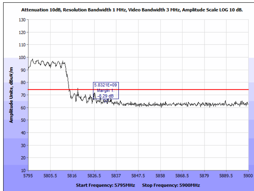
Plot 199. Radiated Band Edge, 802.11n 40 MHz, High Channel, Patch Antenna (5832 & 5835 MHz), Peak
