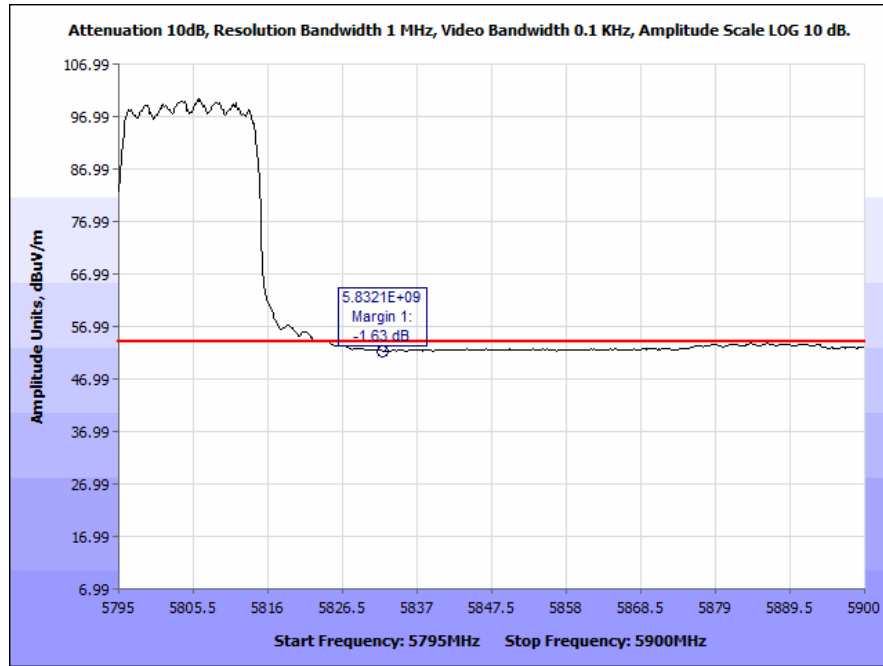
Plot 178. Radiated Band Edge, 802.11n 20 MHz, High Channel, Omni Antenna (5832 & 5835 MHz), Average
