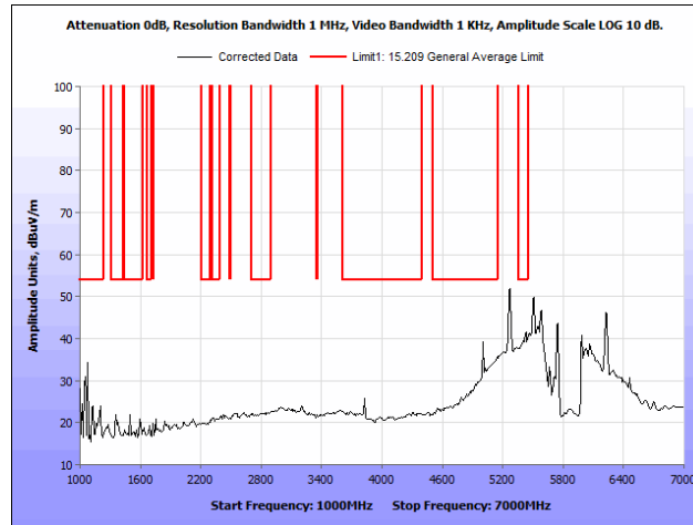
Plot 121. Radiated Spurious Emissions, 802.11a 20 MHz, Mid Channel, 1 GHz – 7 GHz, Average, Patch Antenna
