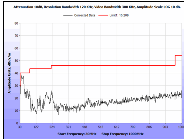
Plot 94. Radiated Spurious Emissions, 802.11n 40 MHz, Low Channel, 30 MHz – 1 GHz, Omni Antenna
