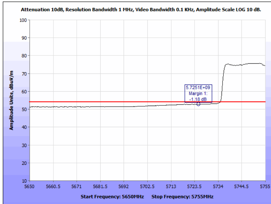
Plot 200. Radiated Band Edge, 802.11n 80 MHz, Patch Antenna (5725 & 5715 MHz), Average
