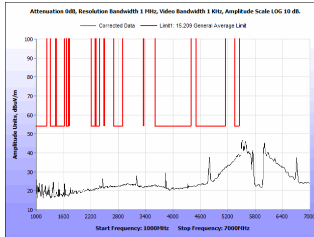
Plot 106. Radiated Spurious Emissions, 802.11n 40 MHz, High Channel, 1 GHz – 7 GHz, Average, Omni Antenna
