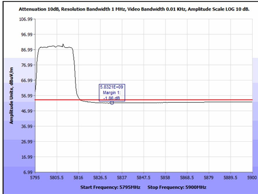
Plot 198. Radiated Band Edge, 802.11n 40 MHz, High Channel, Patch Antenna (5832 & 5835 MHz), Average
