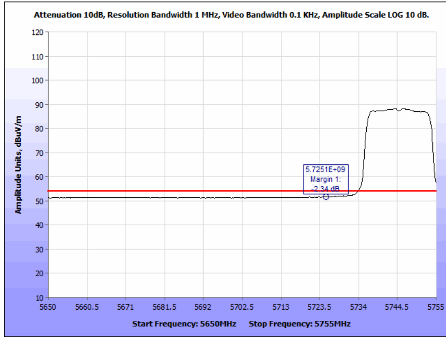
Plot 176. Radiated Band Edge, 802.11n 20 MHz, Low Channel, Omni Antenna (5715 & 5725 MHz), Average
