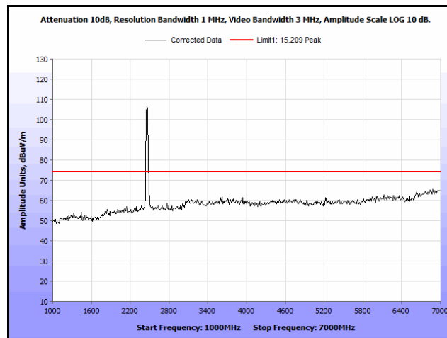
Plot 226. Radiated Spurs, Co-Location, 802.11n 20 MHz, 2462 MHz & 2462 MHz, 1 GHz – 7 GHz, Peak, Omni
