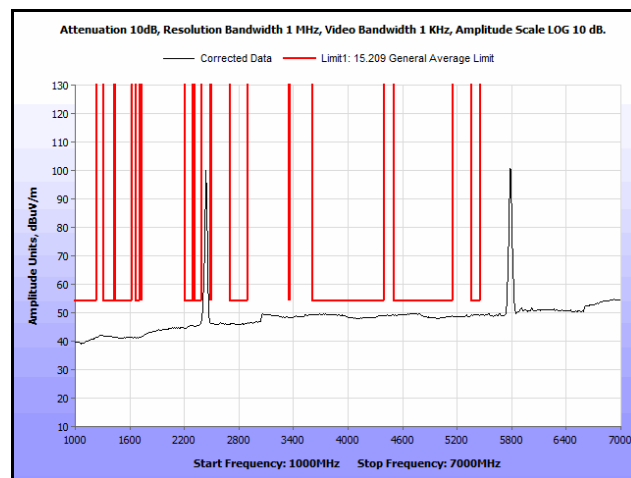
Plot 257. Radiated Spurs, Co-Location, 802.11n 20 MHz, 2437 MHz & 5785 MHz, 1 GHz – 7 GHz, Avg., Omni
