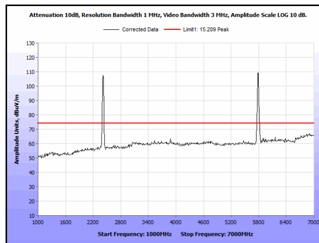
Plot 242. Radiated Spurs, Co-Location, 802.11n 20 MHz, 2412 MHz & 5785 MHz, 1 GHz – 7 GHz, Peak, Omni
