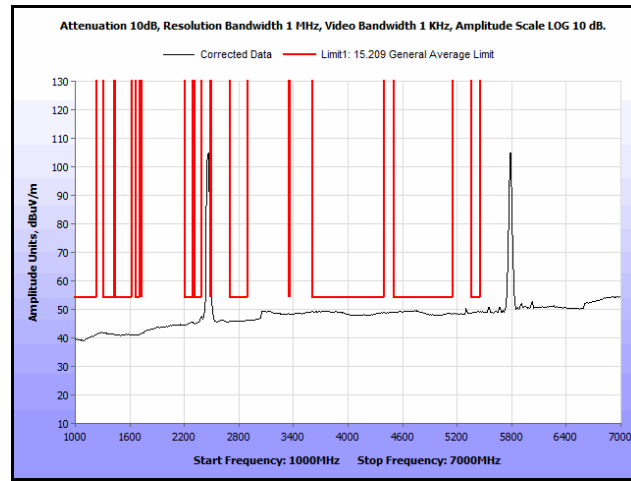
Plot 361. Radiated Spurs, Co-Location, 802.11n 20 MHz, 2462 MHz & 5785 MHz, 1 GHz – 7 GHz, Avg., Patch
