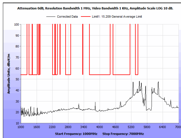
Plot 99. Radiated Spurious Emissions, 802.11n 20 MHz, Mid Channel, 1 GHz – 7 GHz, Average, Omni Antenna
