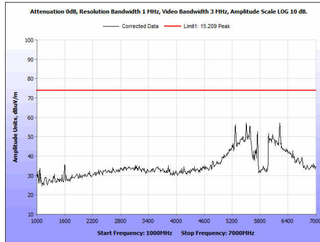
Plot 103. Radiated Spurious Emissions, 802.11n 20 MHz, High Channel, 1 GHz – 7 GHz, Peak, Omni Antenna
