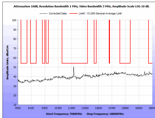
Plot 83. Radiated Spurious Emissions, 802.11a 20 MHz, Mid Channel, 7 GHz – 18 GHz, Omni Antenna
