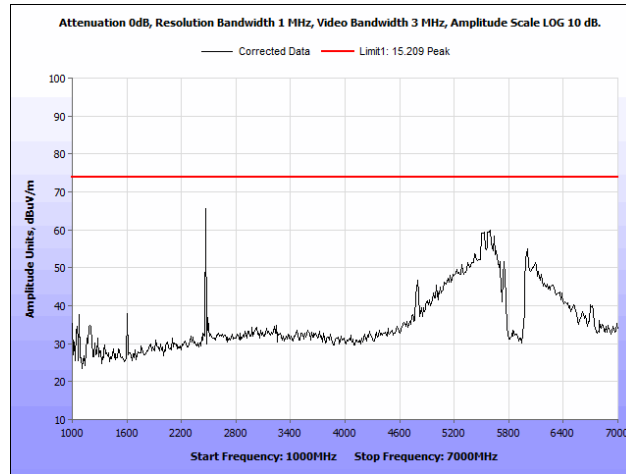
Plot 47. Radiated Spurious Emissions, 802.11a 40 MHz, High Channel, 1 GHz – 7 GHz, Peak, Ceiling Antenna
