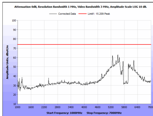
Plot 43. Radiated Spurious Emissions, 802.11a 20 MHz, High Channel, 1 GHz – 7 GHz, Peak, Ceiling Antenna
