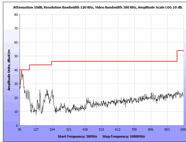
Plot 152. Radiated Spurious Emissions, 802.11ac 80 MHz, 30 MHz – 1 GHz, Patch Antenna
