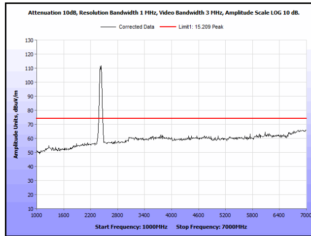
Plot 210. Radiated Spurs, Co-Location, 802.11n 20 MHz, 2412 MHz & 2437 MHz, 1 GHz – 7 GHz, Peak, Omni
