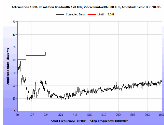
Plot 136. Radiated Spurious Emissions, 802.11n 40 MHz, Low Channel, 30 MHz – 1 GHz, Patch Antenna
