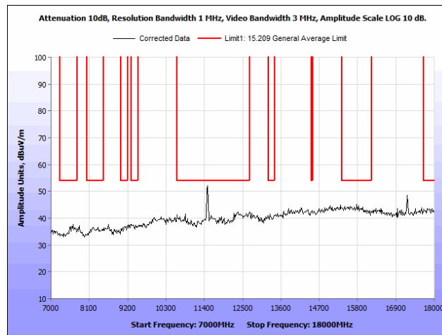
Plot 75. Radiated Spurious Emissions, 802.11a 20 MHz, Low Channel, 7 GHz – 18 GHz, Omni Antenna
