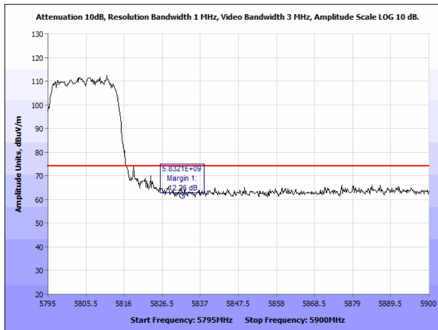
Plot 175. Radiated Band Edge, 802.11a, High Channel, Omni Antenna (5832 & 5835 MHz), Peak
