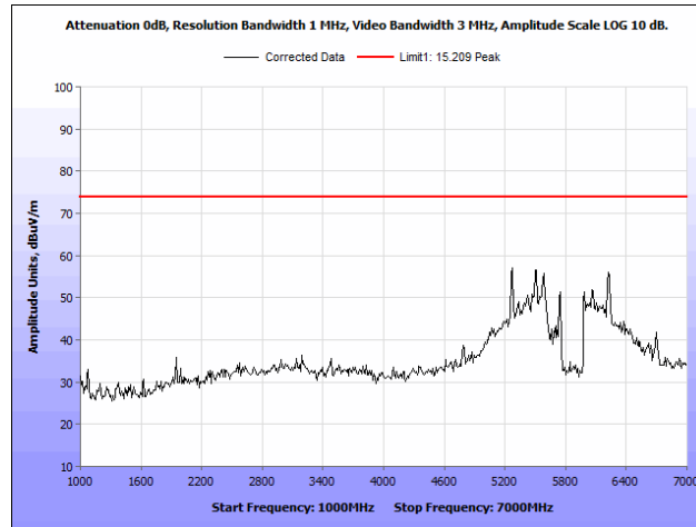
Plot 100. Radiated Spurious Emissions, 802.11n 20 MHz, Mid Channel, 1 GHz – 7 GHz, Peak, Omni Antenna
