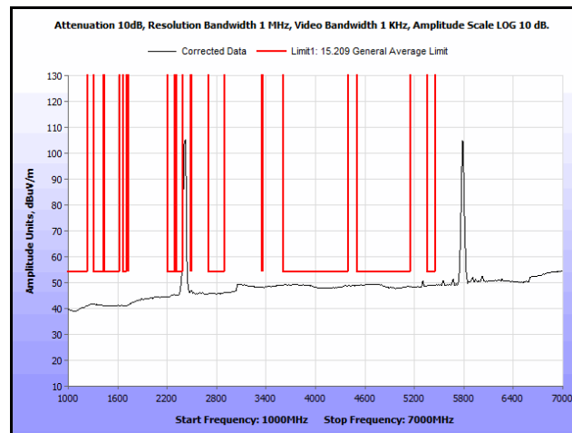
Plot 329. Radiated Spurs, Co-Location, 802.11n 20 MHz, 2412 MHz & 5785 MHz, 1 GHz – 7 GHz, Avg., Patch
