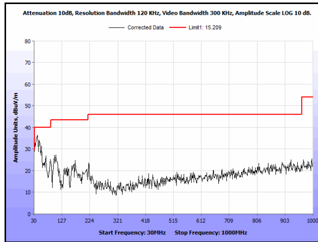
Plot 352. Radiated Spurs, Co-Location, 802.11n 20 MHz, 2462 MHz & 5300 MHz, 30 MHz – 1 GHz, Peak, Patch
