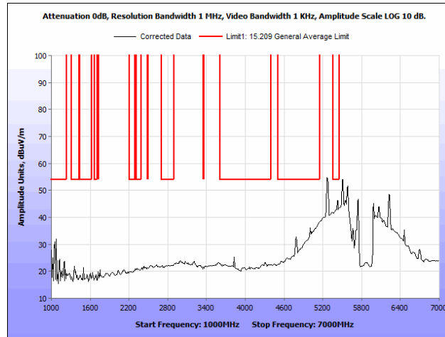
Plot 141. Radiated Spurious Emissions, 802.11n 20 MHz, Mid Channel, 1 GHz – 7 GHz, Average, Patch Antenna
