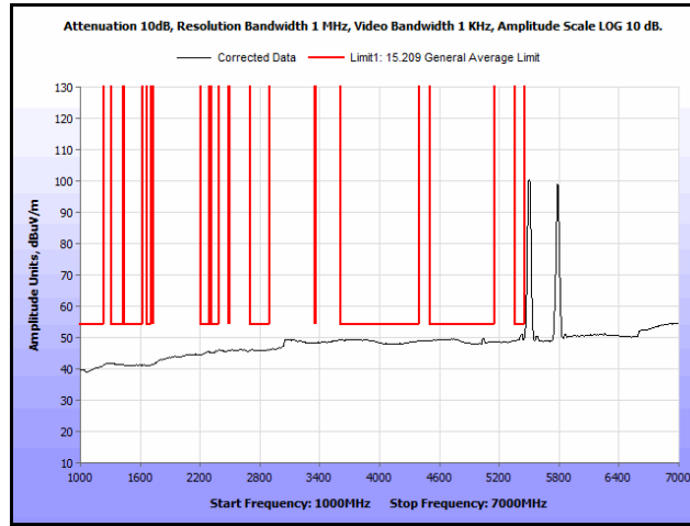
Plot 309. Radiated Spurs, Co-Location, 802.11n 20 MHz, 5580 MHz & 5785 MHz, 1 GHz – 7 GHz, Avg., Omni
