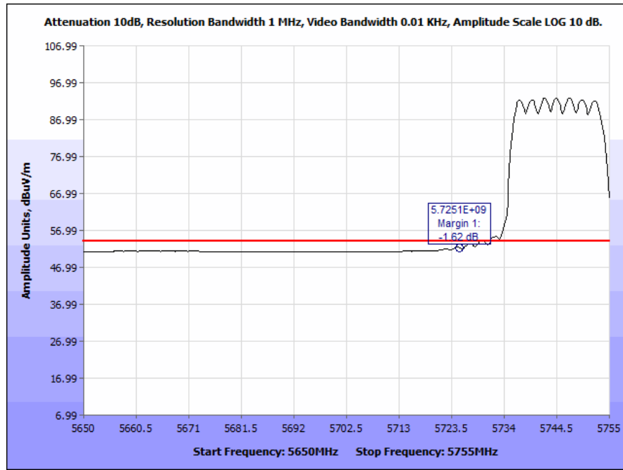
Plot 160. Radiated Band Edge, 802.11n 20 MHz, Low Channel, Ceiling Antenna (5715 & 5725 MHz), Average
