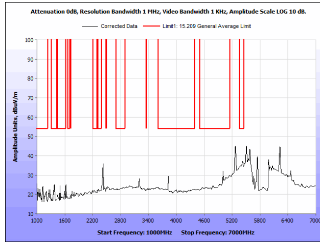
Plot 73. Radiated Spurious Emissions, 802.11a 20 MHz, Low Channel, 1 GHz – 7 GHz, Average, Omni Antenna
