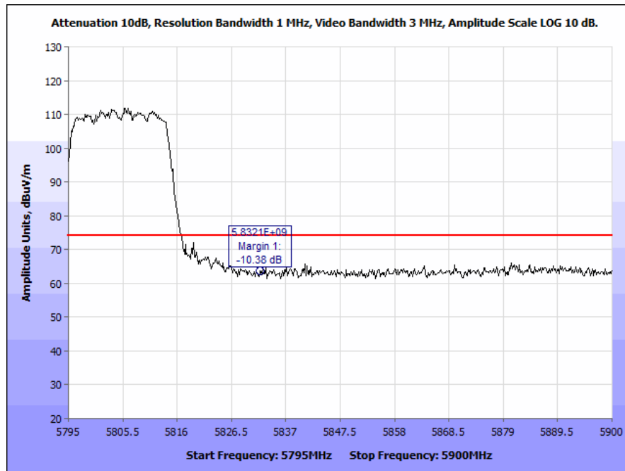
Plot 179. Radiated Band Edge, 802.11n 20 MHz, High Channel, Omni Antenna (5832 & 5835 MHz), Peak
