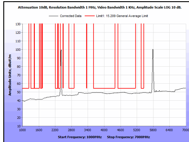
Plot 241. Radiated Spurs, Co-Location, 802.11n 20 MHz, 2412 MHz & 5785 MHz, 1 GHz – 7 GHz, Avg., Omni
