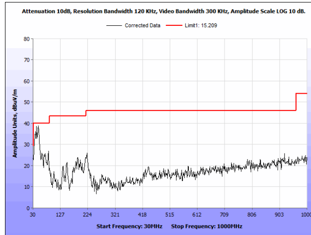
Plot 124. Radiated Spurious Emissions, 802.11a 20 MHz, High Channel, 30 MHz – 1 GHz, Patch Antenna
