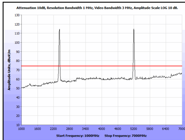
Plot 318. Radiated Spurs, Co-Location, 802.11n 20 MHz, 2412 MHz & 5200 MHz, 1 GHz – 7 GHz, Peak, Patch
