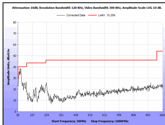
Plot 212. Radiated Spurs, Co-Location, 802.11n 20 MHz, 2412 MHz & 2462 MHz, 30 MHz – 1 GHz, Peak, Omni
