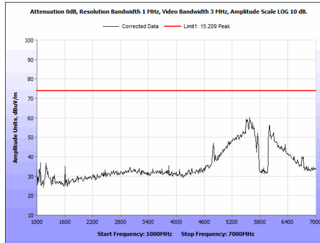
Plot 118. Radiated Spurious Emissions, 802.11a 40 MHz, Low Channel, 1 GHz – 7 GHz, Peak, Patch Antenna
