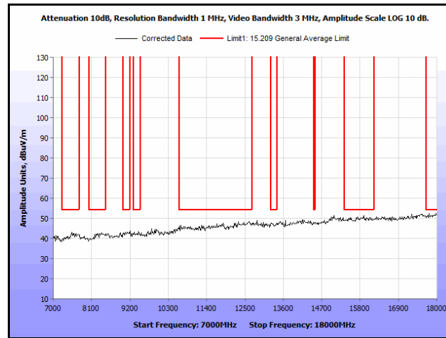
Plot 279. Radiated Spurs, Co-Location, 802.11n 20 MHz, 5200 MHz & 5200 MHz, 7 GHz – 18 GHz, Peak, Omni
