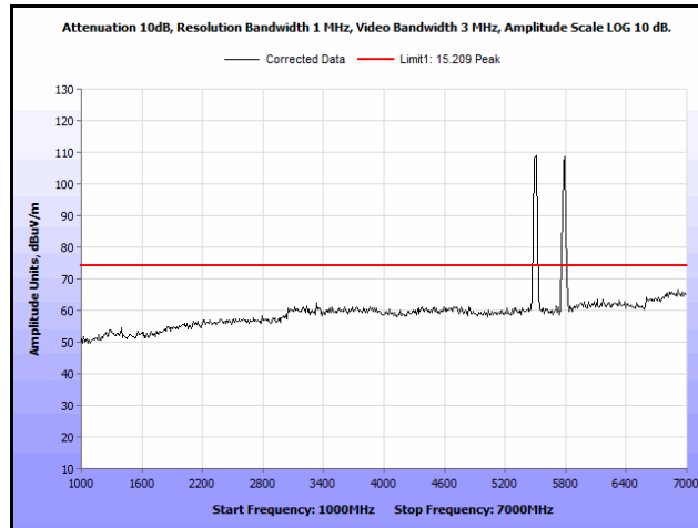
Plot 310. Radiated Spurs, Co-Location, 802.11n 20 MHz, 5580 MHz & 5785 MHz, 1 GHz – 7 GHz, Peak, Omni
