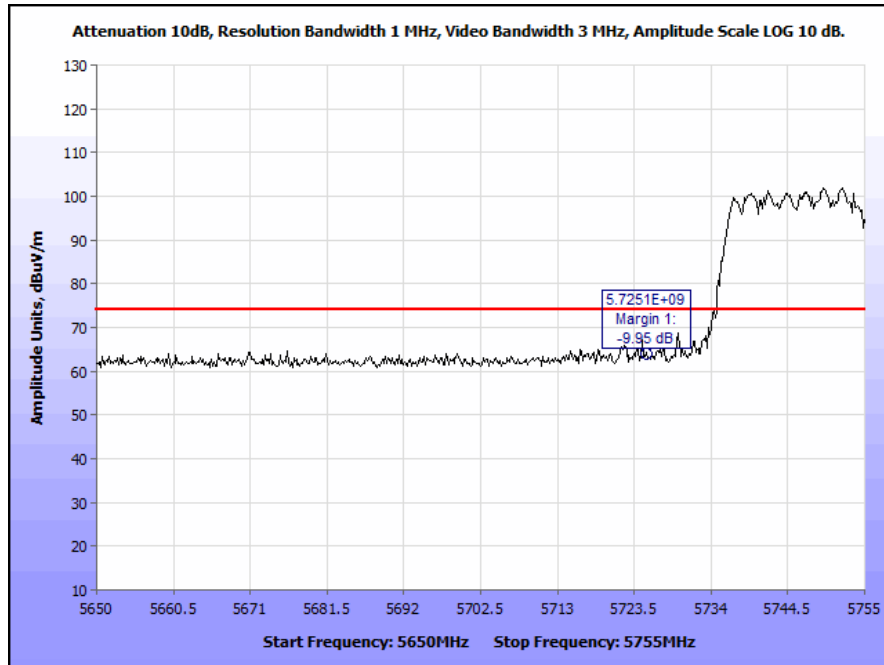
Plot 161. Radiated Band Edge, 802.11n 20 MHz, Low Channel, Ceiling Antenna (5715 & 5725 MHz), Peak
