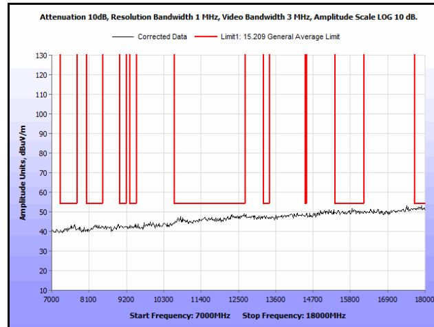
Plot 359. Radiated Spurs, Co-Location, 802.11n 20 MHz, 2462 MHz & 5580 MHz, 7 GHz – 18 GHz, Peak, Patch
