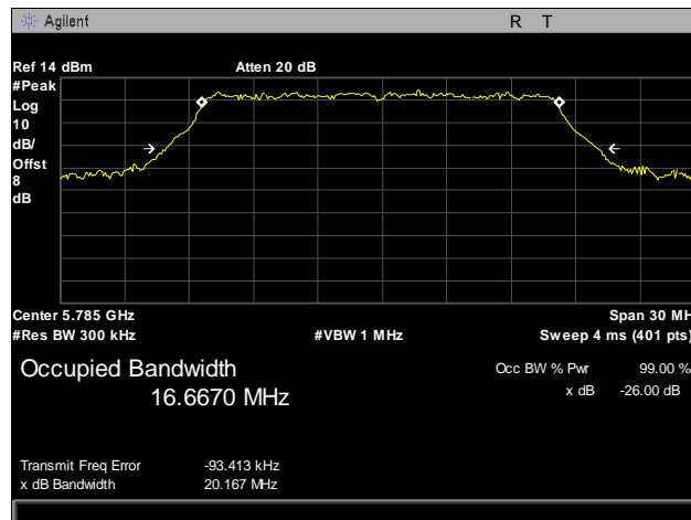
Plot 15. 26 dB Occupied Bandwidth, 802.11a, 5785 MHz
