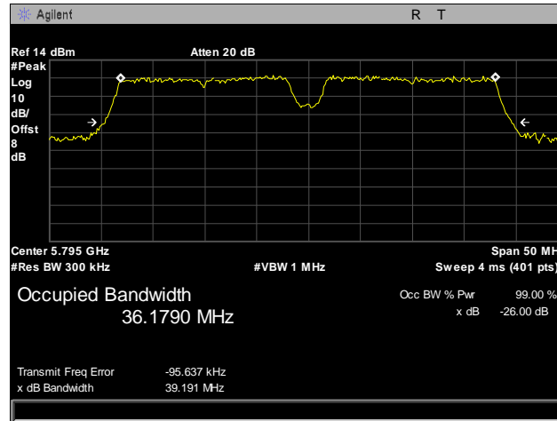
Plot 16. 26 dB Occupied Bandwidth, 802.11a, 5795 MHz
