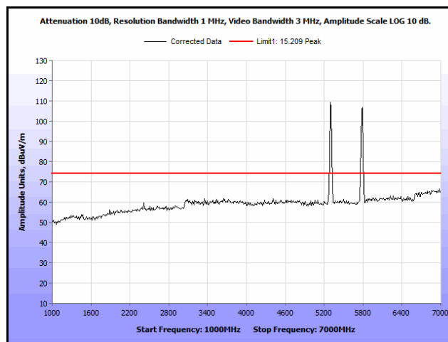
Plot 302. Radiated Spurs, Co-Location, 802.11n 20 MHz, 5300 MHz & 5785 MHz, 1 GHz – 7 GHz, Peak, Omni
