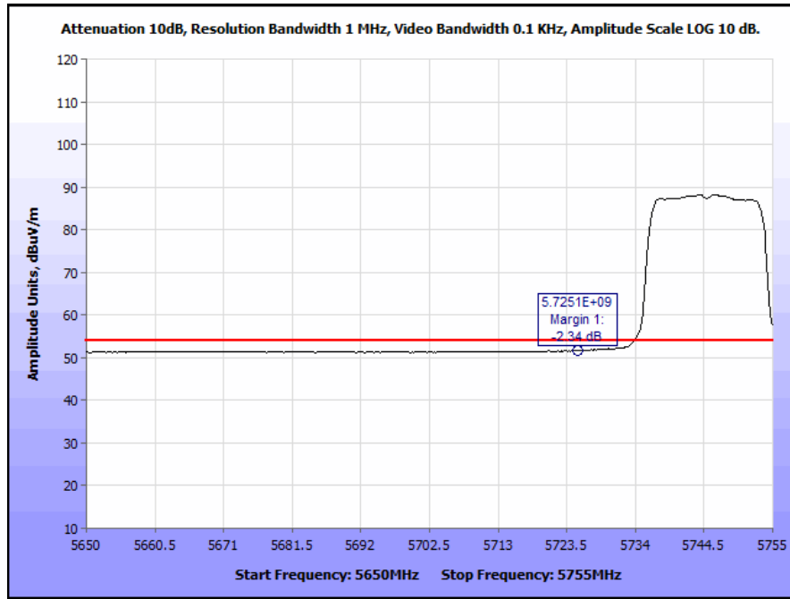
Plot 188. Radiated Band Edge, 802.11a, Low Channel, Patch Antenna (5725 & 5715 MHz), Average
