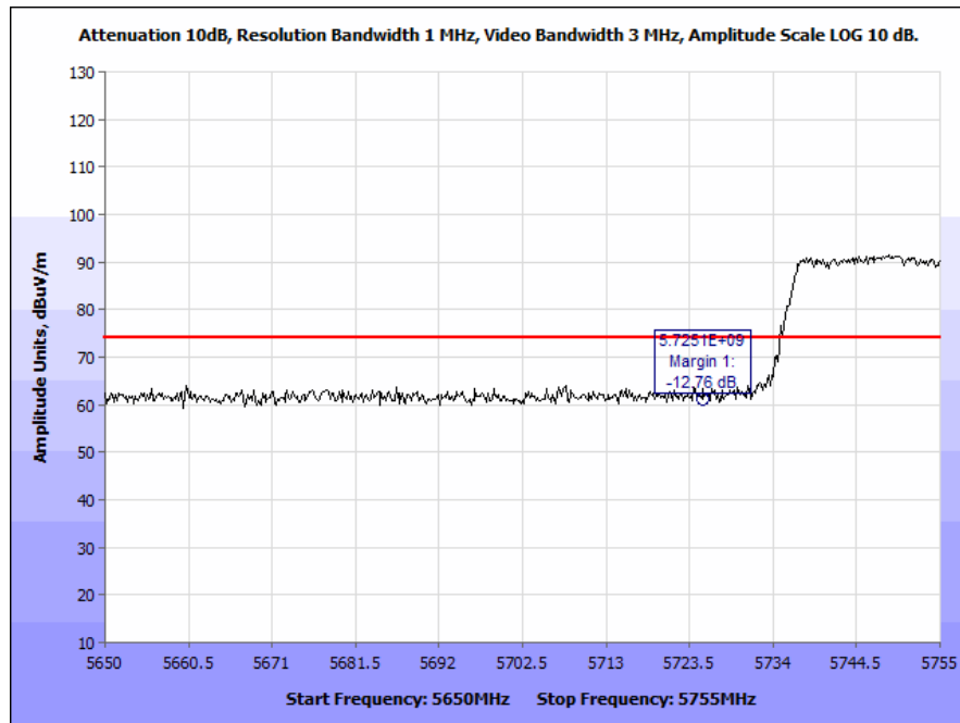
Plot 185. Radiated Band Edge, 802.11ac 80 MHz, Omni Antenna (5715 & 5725 MHz), Peak
