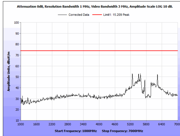
Plot 85. Radiated Spurious Emissions, 802.11a 20 MHz, High Channel, 1 GHz – 7 GHz, Peak, Omni Antenna
