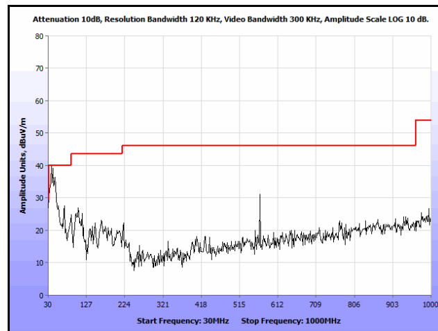
Plot 256. Radiated Spurs, Co-Location, 802.11n 20 MHz, 2437 MHz & 5785 MHz, 30 MHz – 1 GHz, Peak, Omni
