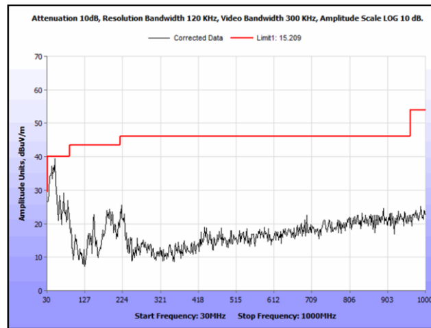
Plot 98. Radiated Spurious Emissions, 802.11n 20 MHz, Mid Channel, 30 MHz – 1 GHz, Omni Antenna
