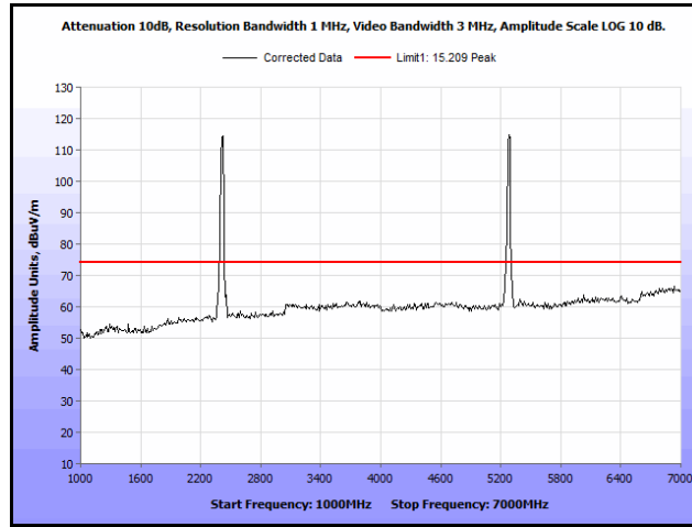
Plot 322. Radiated Spurs, Co-Location, 802.11n 20 MHz, 2412 MHz & 5300 MHz, 1 GHz – 7 GHz, Peak, Patch
