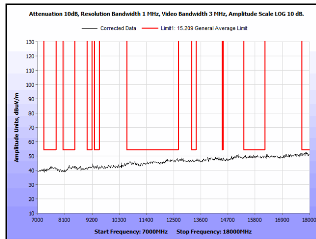
Plot 295. Radiated Spurs, Co-Location, 802.11n 20 MHz, 5300 MHz & 5300 MHz, 7 GHz – 18 GHz, Peak, Omni
