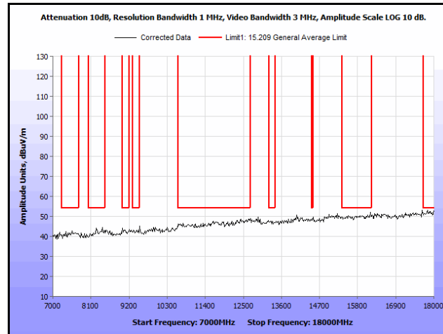
Plot 259. Radiated Spurs, Co-Location, 802.11n 20 MHz, 2437 MHz & 5785 MHz, 7 GHz – 18 GHz, Peak, Omni
