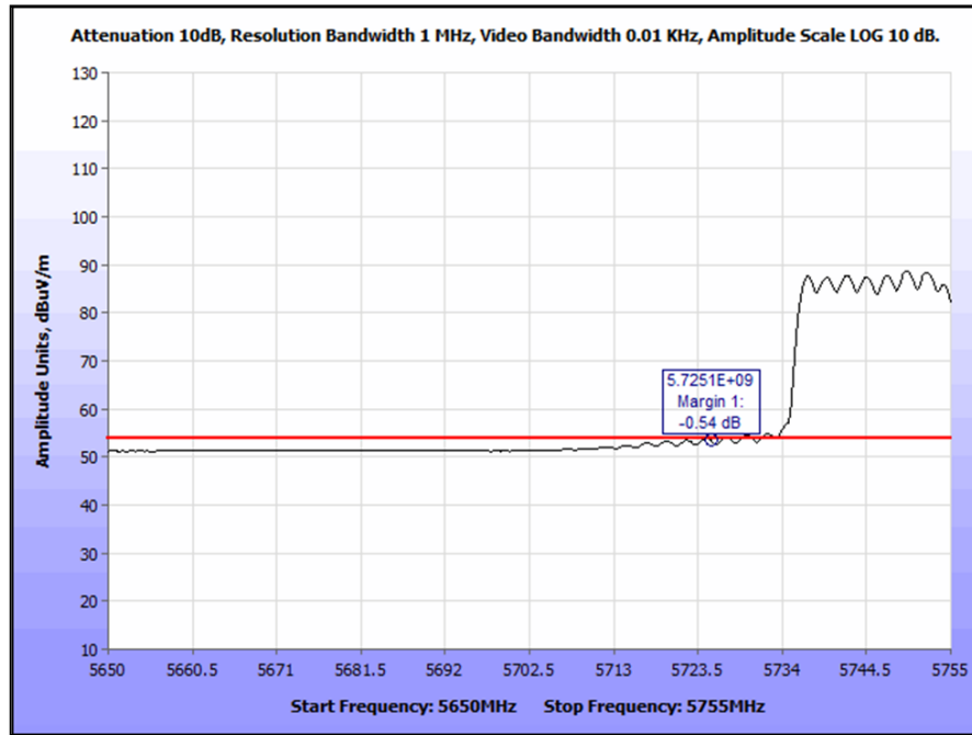
Plot 196. Radiated Band Edge, 802.11n 40 MHz, Low Channel, Patch Antenna (5725 & 5715 MHz), Average
