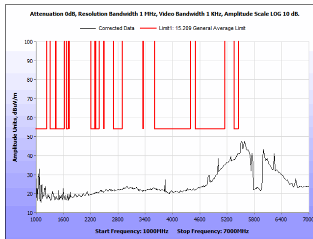
Plot 129. Radiated Spurious Emissions, 802.11a 40 MHz, High Channel, 1 GHz – 7 GHz, Average, Patch Antenna
