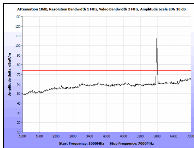
Plot 314. Radiated Spurs, Co-Location, 802.11n 20 MHz, 5785 MHz & 5785 MHz, 1 GHz – 7 GHz, Peak, Omni
