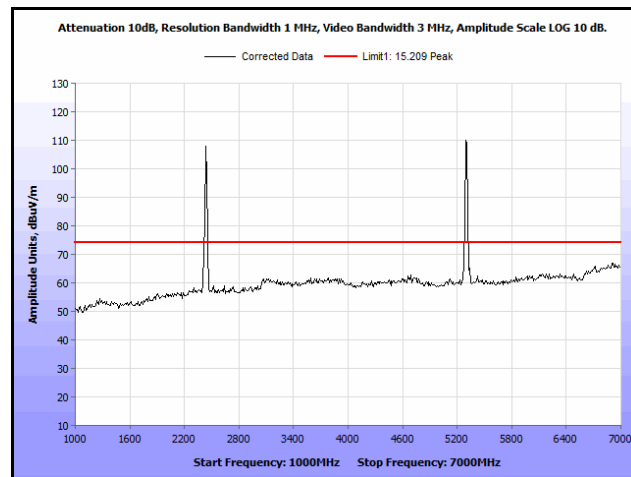
Plot 250. Radiated Spurs, Co-Location, 802.11n 20 MHz, 2437 MHz & 5300 MHz, 1 GHz – 7 GHz, Peak, Omni
