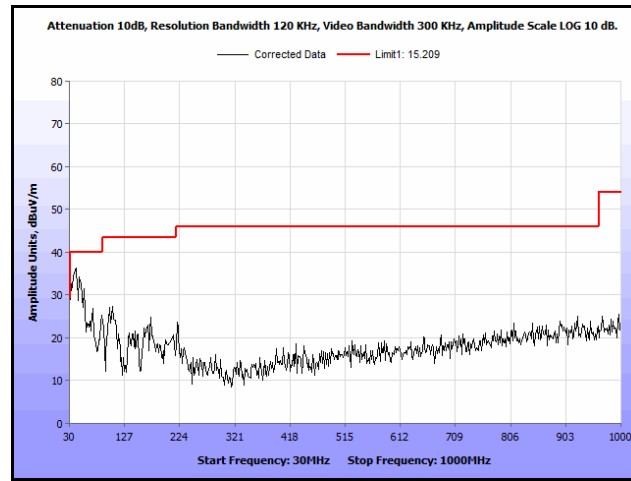
Plot 264. Radiated Spurs, Co-Location, 802.11n 20 MHz, 2462 MHz & 5300 MHz, 30 MHz – 1 GHz, Peak, Omni
