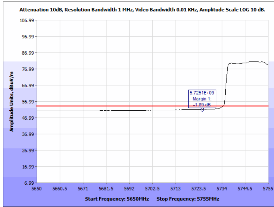
Plot 168. Radiated Band Edge, 802.11n 80 MHz, Ceiling Antenna (5715 & 5725 MHz), Average
