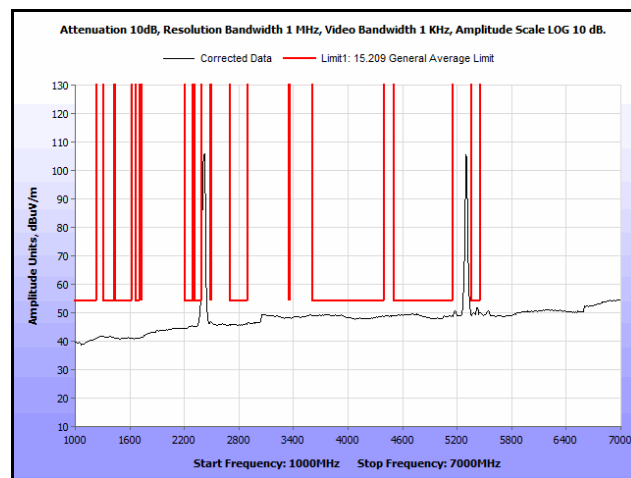
Plot 321. Radiated Spurs, Co-Location, 802.11n 20 MHz, 2412 MHz & 5300 MHz, 1 GHz – 7 GHz, Avg., Patch
