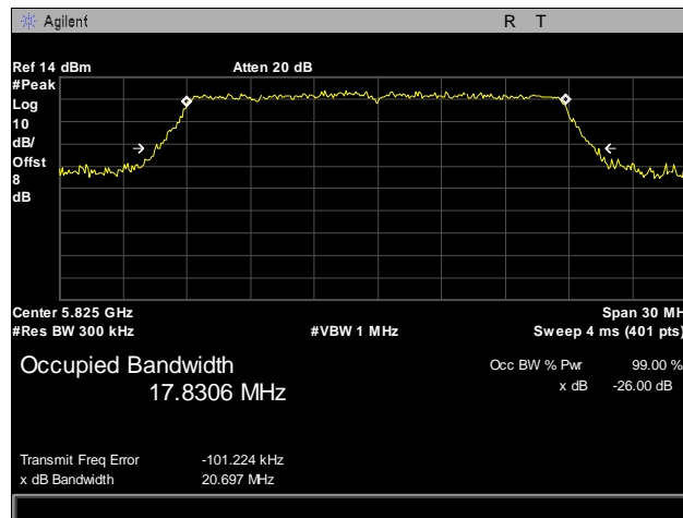
Plot 27. 26 dB Occupied Bandwidth, 802.11n, 5825 MHz, Port 2
