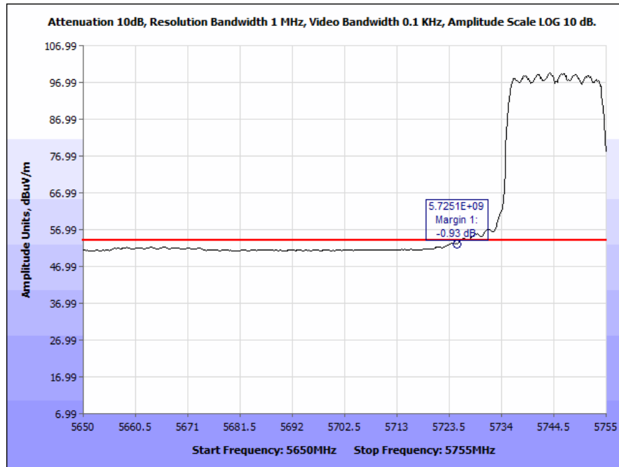
Plot 172. Radiated Band Edge, 802.11a, Low Channel, Omni Antenna (5715 & 5725 MHz), Average
