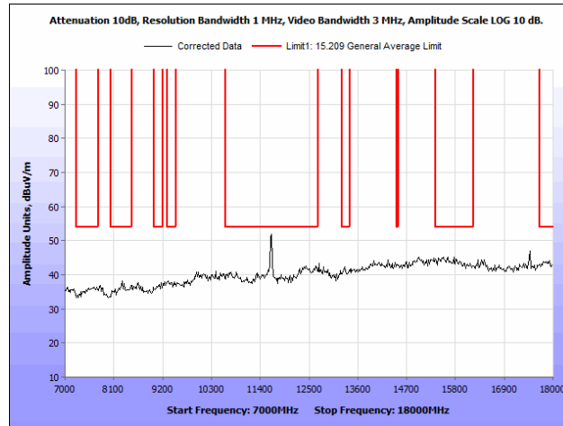
Plot 147. Radiated Spurious Emissions, 802.11n 20 MHz, High Channel, 7 GHz – 18 GHz, Patch Antenna
