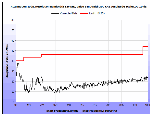
Plot 120. Radiated Spurious Emissions, 802.11a 20 MHz, Mid Channel, 30 MHz – 1 GHz, Patch Antenna
