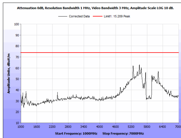
Plot 126. Radiated Spurious Emissions, 802.11a 20 MHz, High Channel, 1 GHz – 7 GHz, Peak, Patch Antenna
