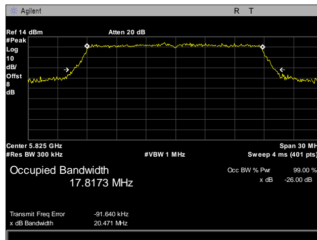
Plot 22. 26 dB Occupied Bandwidth, 802.11n, 5825 MHz, Port 1
