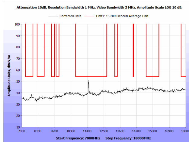
Plot 93. Radiated Spurious Emissions, 802.11n 20 MHz, Low Channel, 7 GHz – 18 GHz, Omni Antenna
