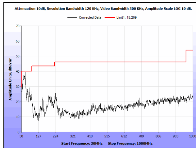
Plot 320. Radiated Spurs, Co-Location, 802.11n 20 MHz, 2412 MHz & 5300 MHz, 30 MHz – 1 GHz, Peak, Patch
