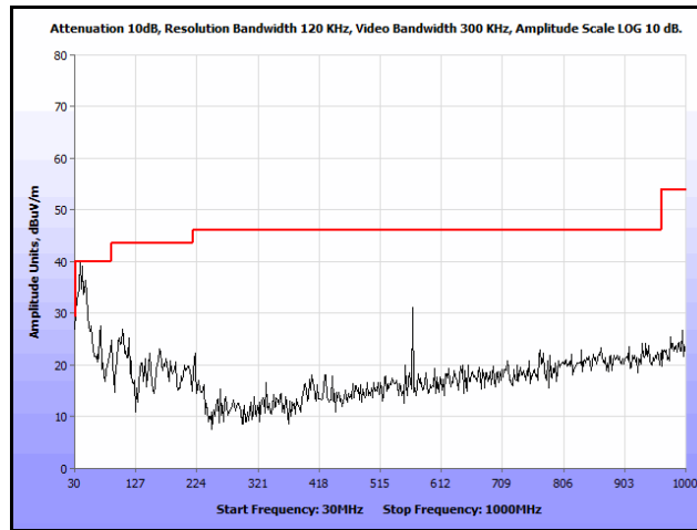
Plot 312. Radiated Spurs, Co-Location, 802.11n 20 MHz, 5785 MHz & 5785 MHz, 30 MHz – 1 GHz, Peak, Omni
