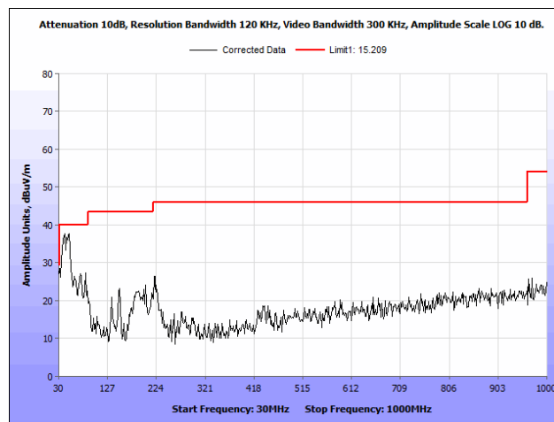
Plot 65. Radiated Spurious Emissions, 802.11n 40 MHz, High Channel, 30 MHz – 1 GHz, Ceiling Antenna
