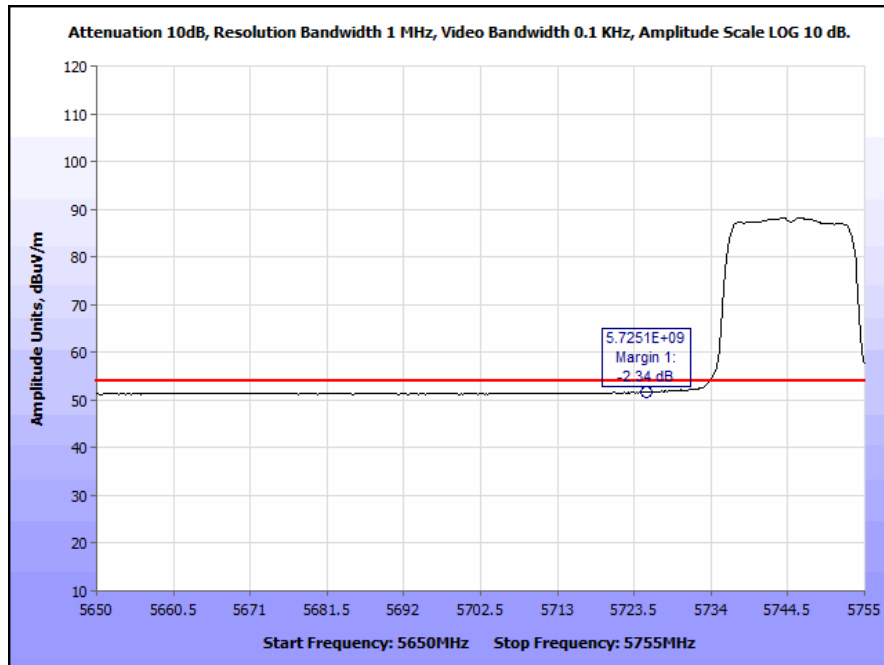
Plot 189. Radiated Band Edge, 802.11a, Low Channel, Patch Antenna (5725 & 5715 MHz), Peak
