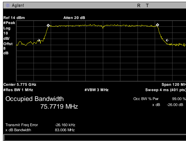
Plot 28. 26 dB Occupied Bandwidth, 802.11ac, 5775 MHz, Port 1
