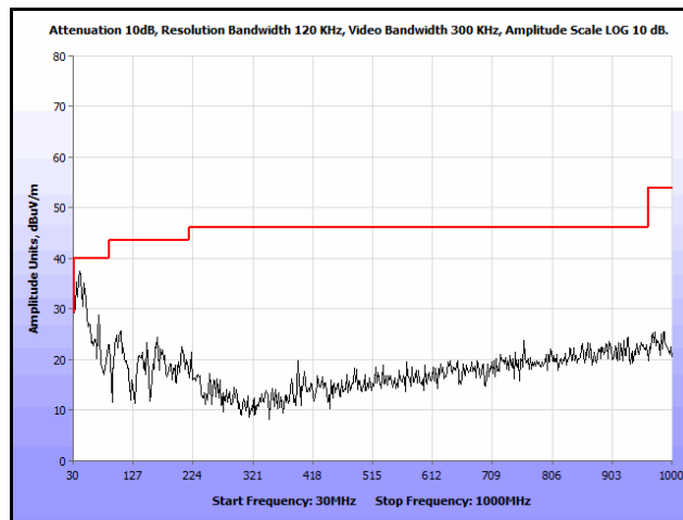
Plot 336. Radiated Spurs, Co-Location, 802.11n 20 MHz, 2437 MHz & 5300 MHz, 30 MHz – 1 GHz, Peak, Patch
