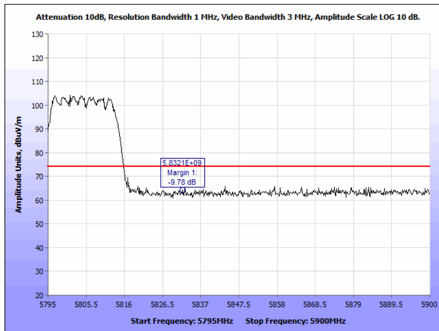
Plot 163. Radiated Band Edge, 802.11n 20 MHz, High Channel, Ceiling Antenna (5825 & 5835 MHz), Peak
