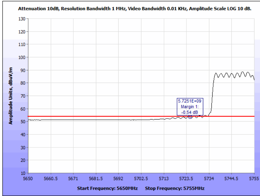
Plot 164. Radiated Band Edge, 802.11n 40 MHz, Low Channel, Ceiling Antenna (5715 & 5725 MHz), Average
