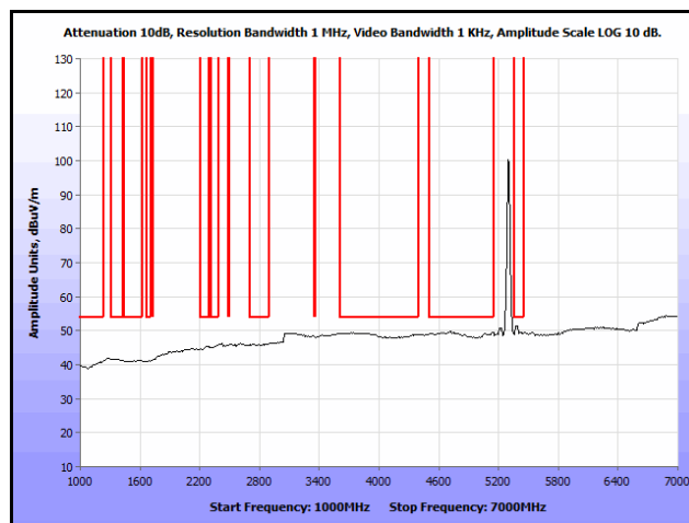
Plot 293. Radiated Spurs, Co-Location, 802.11n 20 MHz, 5300 MHz & 5300 MHz, 1 GHz – 7 GHz, Avg., Omni
