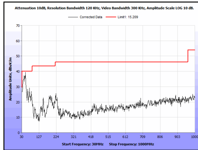
Plot 288. Radiated Spurs, Co-Location, 802.11n 20 MHz, 5200 MHz & 5785 MHz, 30 MHz – 1 GHz, Peak, Omni
