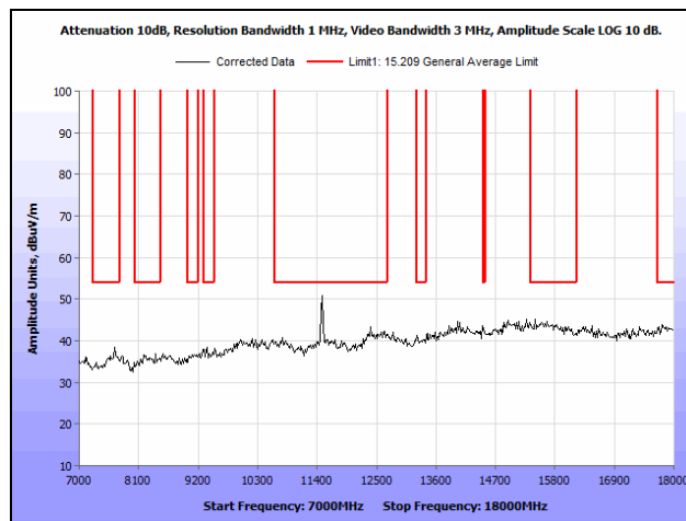
Plot 111. Radiated Spurious Emissions, 802.11ac 80 MHz, 7 GHz – 18 GHz, Omni Antenna
