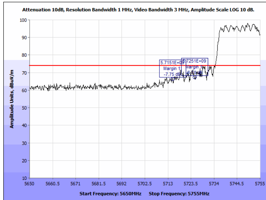
Plot 197. Radiated Band Edge, 802.11n 40 MHz, Low Channel, Patch Antenna (5725 & 5715 MHz), Peak
