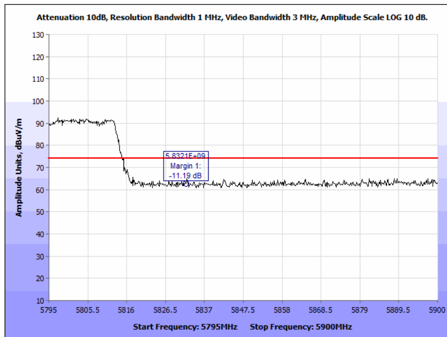
Plot 187. Radiated Band Edge, 802.11ac 80 MHz, Omni Antenna (5832 & 5835 MHz), Peak
