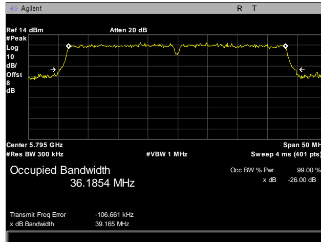
Plot 21. 26 dB Occupied Bandwidth, 802.11n, 5795 MHz, Port 1
