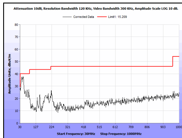
Plot 296. Radiated Spurs, Co-Location, 802.11n 20 MHz, 5300 MHz & 5580 MHz, 30 MHz – 1 GHz, Peak, Omni
