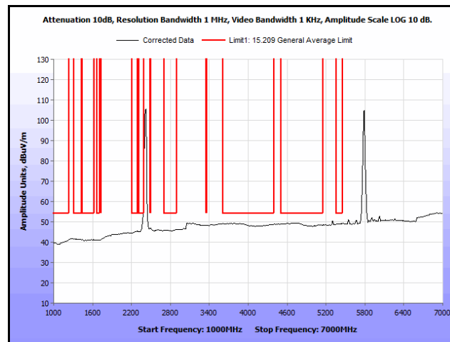
Plot 345. Radiated Spurs, Co-Location, 802.11n 20 MHz, 2437 MHz & 5785 MHz, 1 GHz – 7 GHz, Avg., Patch
