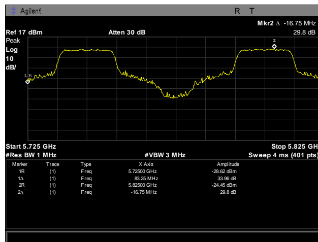
Plot 371. Frequency Stability, 5725 – 5825 MHz, 30°C, 120 V
