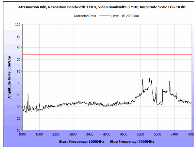
Plot 82. Radiated Spurious Emissions, 802.11a 20 MHz, Mid Channel, 1 GHz – 7 GHz, Peak, Omni Antenna
