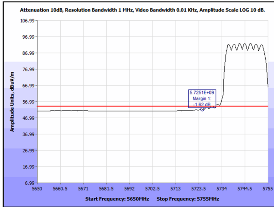
Plot 192. Radiated Band Edge, 802.11n 20 MHz, Low Channel, Patch Antenna (5725 & 5715 MHz), Average
