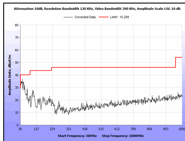
Plot 360. Radiated Spurs, Co-Location, 802.11n 20 MHz, 2462 MHz & 5785 MHz, 30 MHz – 1 GHz, Peak, Patch
