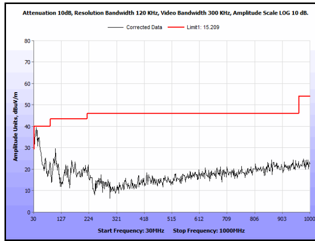
Plot 300. Radiated Spurs, Co-Location, 802.11n 20 MHz, 5300 MHz & 5785 MHz, 30 MHz – 1 GHz, Peak, Omni
