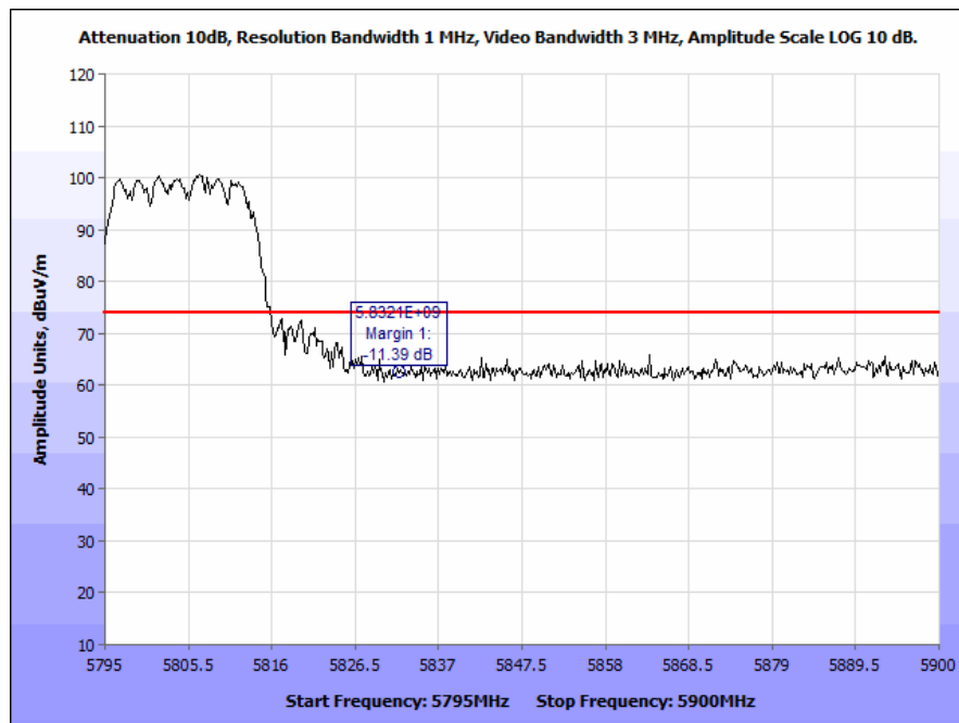
Plot 195. Radiated Band Edge, 802.11n 20 MHz, High Channel, Patch Antenna (5832 & 5835 MHz), Peak
