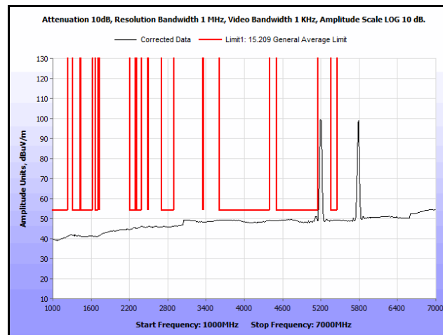
Plot 289. Radiated Spurs, Co-Location, 802.11n 20 MHz, 5200 MHz & 5785 MHz, 1 GHz – 7 GHz, Avg., Omni
