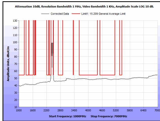
Plot 213. Radiated Spurs, Co-Location, 802.11n 20 MHz, 2412 MHz & 2462 MHz, 1 GHz – 7 GHz, Avg., Omni
