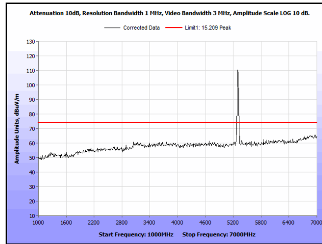
Plot 294. Radiated Spurs, Co-Location, 802.11n 20 MHz, 5300 MHz & 5300 MHz, 1 GHz – 7 GHz, Peak, Omni
