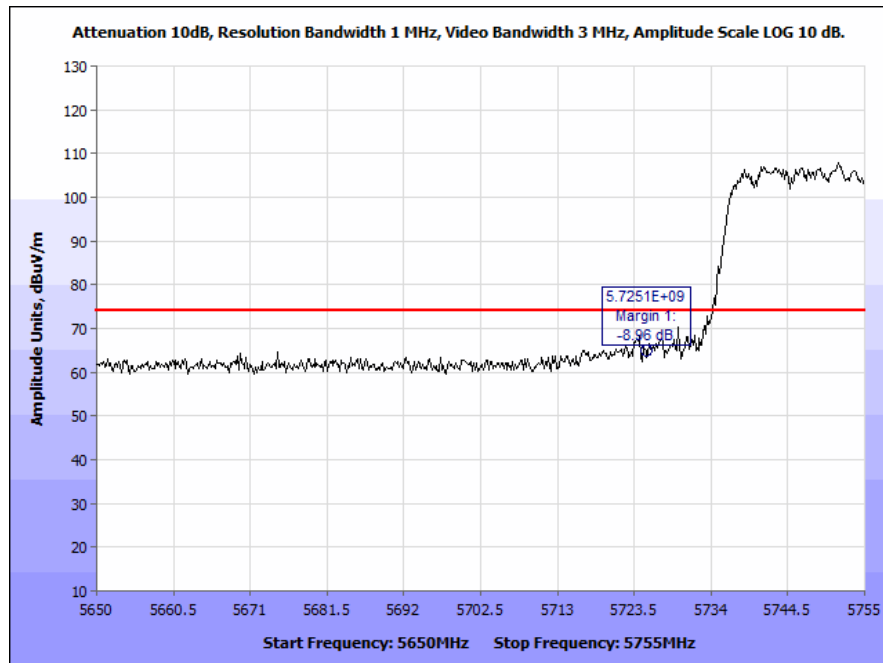
Plot 181. Radiated Band Edge, 802.11n 40 MHz, Low Channel, Omni Antenna (5715 & 5725 MHz), Peak
