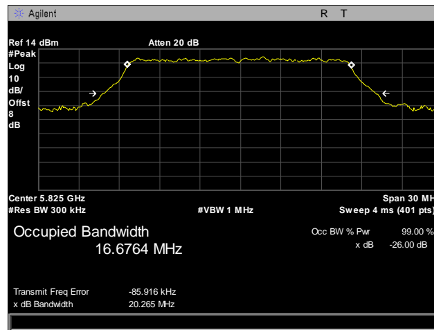
Plot 17. 26 dB Occupied Bandwidth, 802.11a, 5825 MHz
