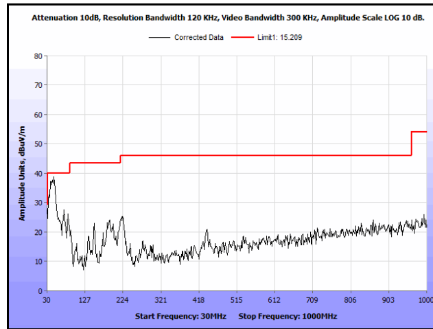
Plot 216. Radiated Spurs, Co-Location, 802.11n 20 MHz, 2437 MHz & 2437 MHz, 30 MHz – 1 GHz, Peak, Omni
