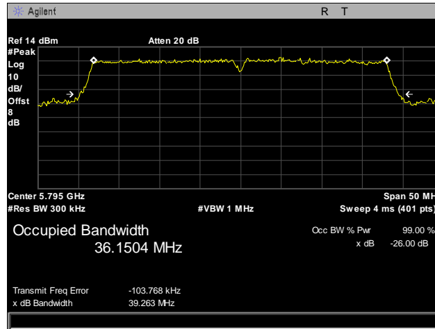
Plot 26. 26 dB Occupied Bandwidth, 802.11n, 5795 MHz, Port 2
