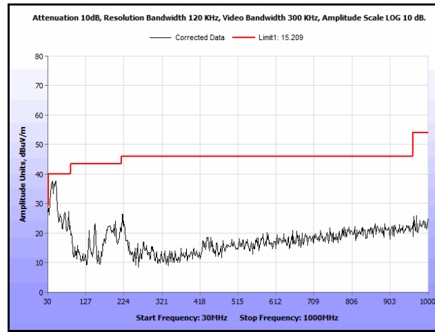
Plot 240. Radiated Spurs, Co-Location, 802.11n 20 MHz, 2412 MHz & 5785 MHz, 30 MHz – 1 GHz, Peak, Omni
