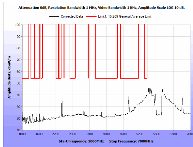
Plot 109. Radiated Spurious Emissions, 802.11ac 80 MHz, 1 GHz – 7 GHz, Average, Omni Antenna
