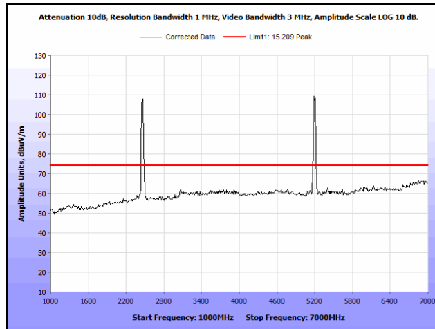
Plot 262. Radiated Spurs, Co-Location, 802.11n 20 MHz, 2462 MHz & 5200 MHz, 1 GHz – 7 GHz, Peak, Omni
