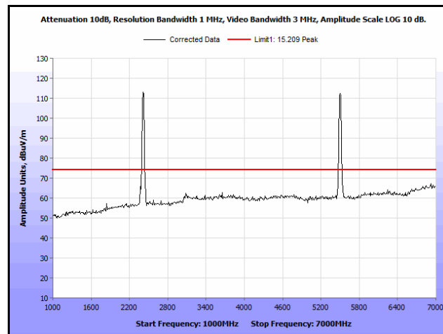
Plot 326. Radiated Spurs, Co-Location, 802.11n 20 MHz, 2412 MHz & 5580 MHz, 1 GHz – 7 GHz, Peak, Patch
