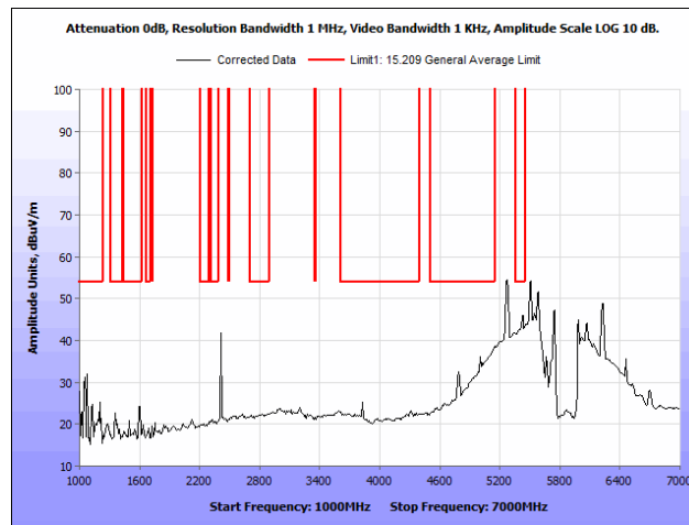
Plot 62. Radiated Spurious Emissions, 802.11n 20 MHz, High Channel, 1 GHz – 7 GHz, Average, Ceiling Antenna
