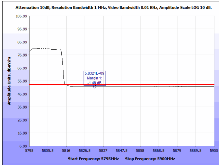
Plot 170. Radiated Band Edge, 802.11n 80 MHz, Ceiling Antenna (5832 & 5835 MHz), Average
