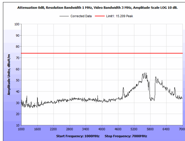
Plot 107. Radiated Spurious Emissions, 802.11n 40 MHz, High Channel, 1 GHz – 7 GHz, Peak, Omni Antenna
