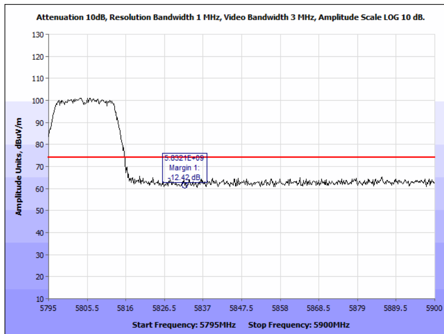
Plot 159. Radiated Band Edge, 802.11a, High Channel, Ceiling Antenna (5825 & 5835 MHz), Peak
