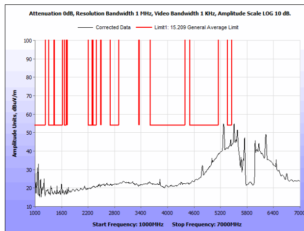
Plot 66. Radiated Spurious Emissions, 802.11n 40 MHz, High Channel, 1 GHz – 7 GHz, Average, Ceiling Antenna
