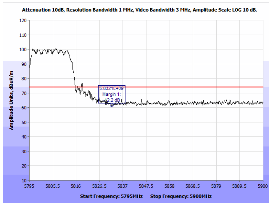
Plot 191. Radiated Band Edge, 802.11a, High Channel, Patch Antenna (5832 & 5835 MHz), Peak
