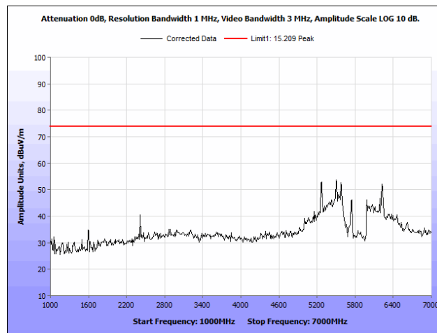
Plot 74. Radiated Spurious Emissions, 802.11a 20 MHz, Low Channel, 1 GHz – 7 GHz, Peak, Omni Antenna
