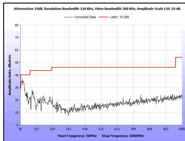
Plot 260. Radiated Spurs, Co-Location, 802.11n 20 MHz, 2462 MHz & 5200 MHz, 30 MHz – 1 GHz, Peak, Omni
