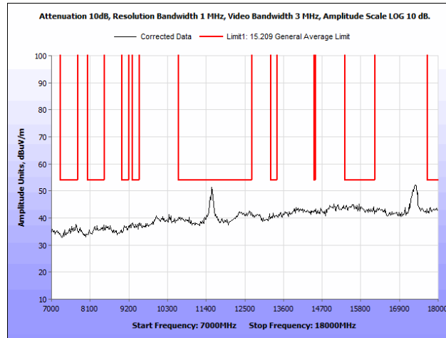
Plot 155. Radiated Spurious Emissions, 802.11ac 80 MHz, 7 GHz – 18 GHz, Patch Antenna
