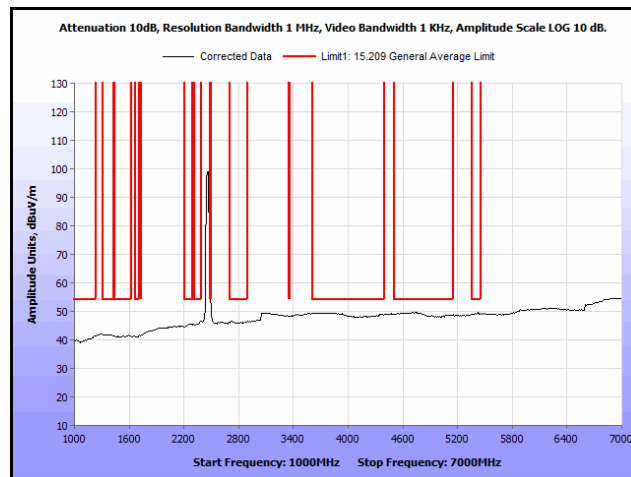
Plot 217. Radiated Spurs, Co-Location, 802.11n 20 MHz, 2437 MHz & 2437 MHz, 1 GHz – 7 GHz, Avg., Omni
