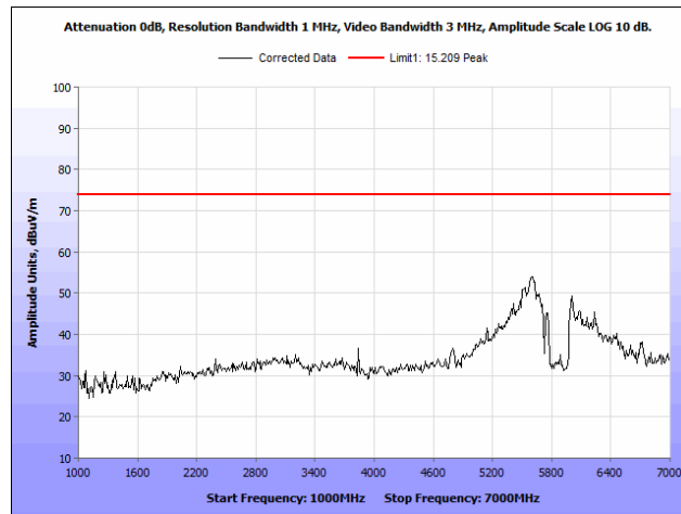
Plot 78. Radiated Spurious Emissions, 802.11a 40 MHz, Low Channel, 1 GHz – 7 GHz, Peak, Omni Antenna
