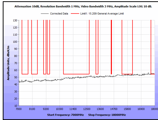
Plot 231. Radiated Spurs, Co-Location, 802.11n 20 MHz, 2412 MHz & 5200 MHz, 7 GHz – 18 GHz, Peak, Omni
