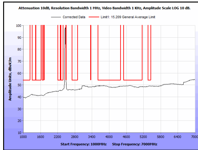
Plot 225. Radiated Spurs, Co-Location, 802.11n 20 MHz, 2462 MHz & 2462 MHz, 1 GHz – 7 GHz, Avg., Omni
