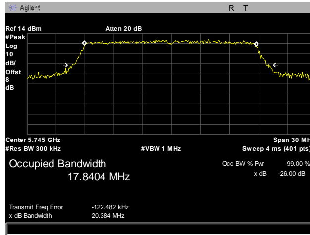
Plot 23. 26 dB Occupied Bandwidth, 802.11n, 5745 MHz, Port 2
