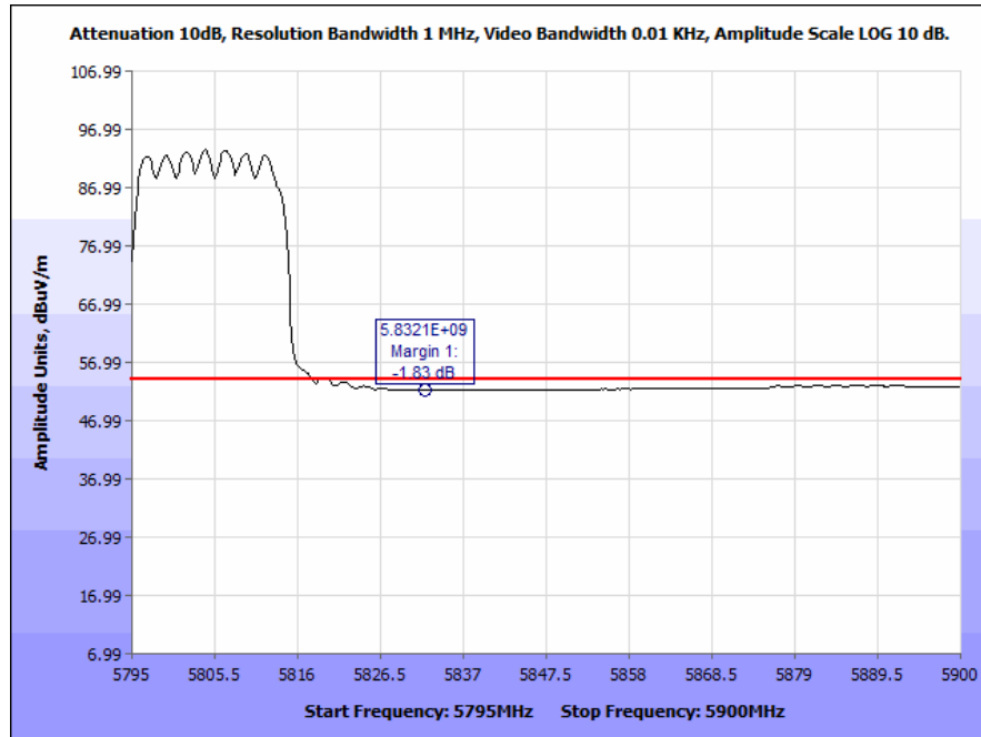
Plot 162. Radiated Band Edge, 802.11n 20 MHz, High Channel, Ceiling Antenna (5825 & 5835 MHz), Average
