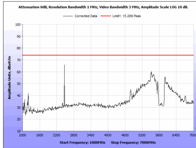
Plot 55. Radiated Spurious Emissions, 802.11n 40 MHz, Low Channel, 1 GHz – 7 GHz, Peak, Ceiling Antenna
