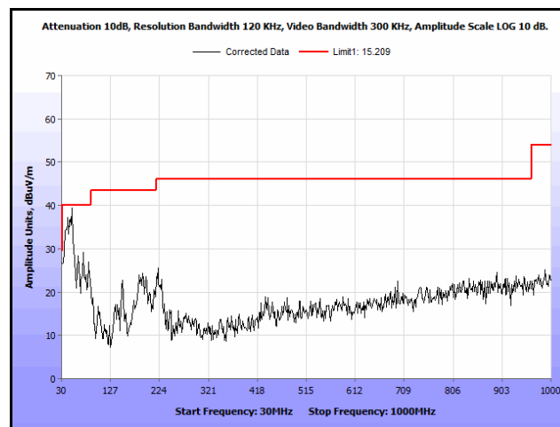
Plot 236. Radiated Spurs, Co-Location, 802.11n 20 MHz, 2412 MHz & 5580 MHz, 30 MHz – 1 GHz, Peak, Omni
