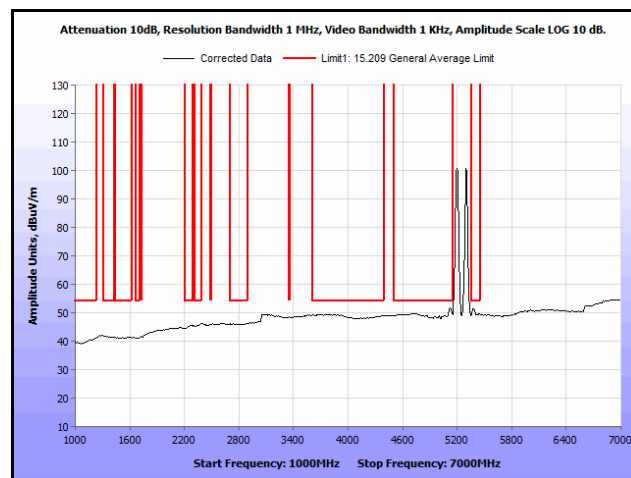
Plot 281. Radiated Spurs, Co-Location, 802.11n 20 MHz, 5200 MHz & 5300 MHz, 1 GHz – 7 GHz, Avg., Omni
