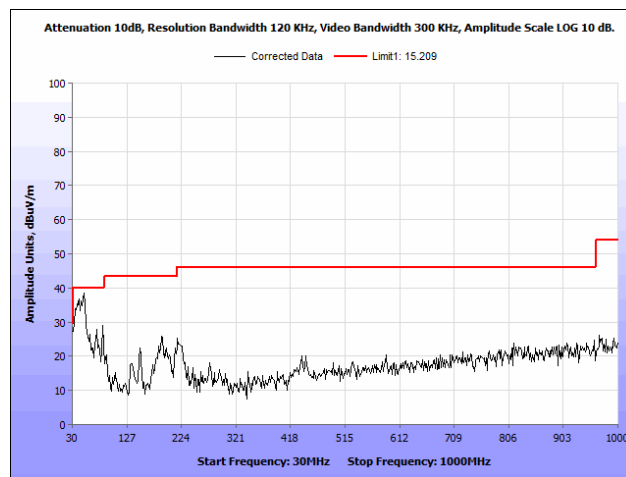
Plot 57. Radiated Spurious Emissions, 802.11n 20 MHz, Mid Channel, 30 MHz – 1 GHz, Ceiling Antenna
