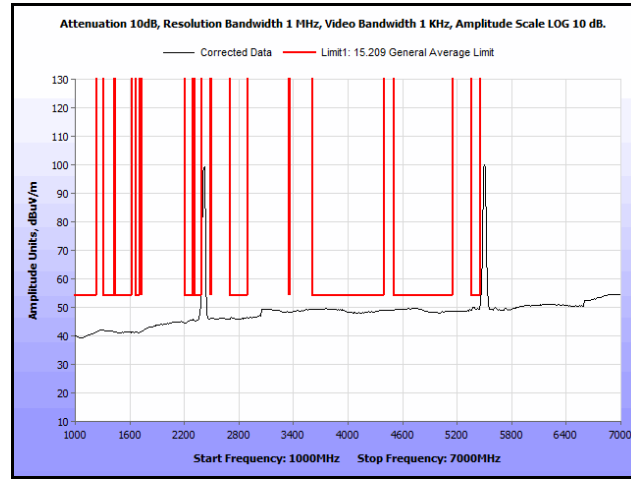
Plot 237. Radiated Spurs, Co-Location, 802.11n 20 MHz, 2412 MHz & 5580 MHz, 1 GHz – 7 GHz, Avg., Omni
