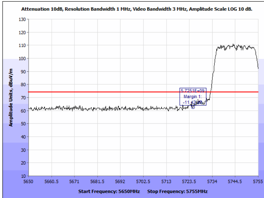
Plot 177. Radiated Band Edge, 802.11n 20 MHz, Low Channel, Omni Antenna (5715 & 5725 MHz), Peak
