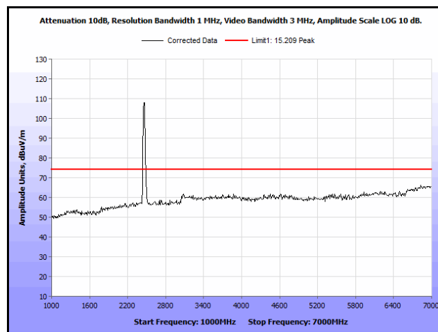
Plot 218. Radiated Spurs, Co-Location, 802.11n 20 MHz, 2437 MHz & 2437 MHz, 1 GHz – 7 GHz, Peak, Omni
