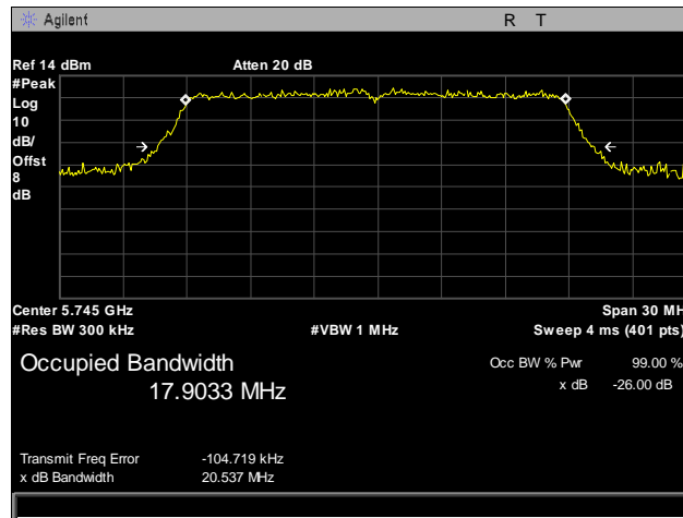
Plot 18. 26 dB Occupied Bandwidth, 802.11n, 5745 MHz, Port 1
