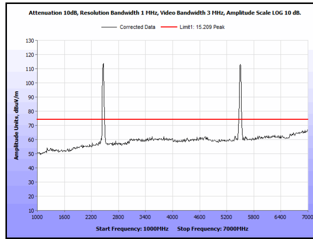
Plot 358. Radiated Spurs, Co-Location, 802.11n 20 MHz, 2462 MHz & 5580 MHz, 1 GHz – 7 GHz, Peak, Patch
