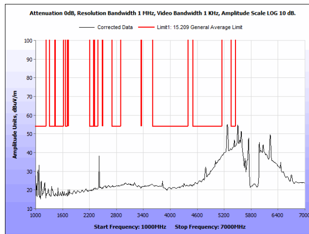
Plot 54. Radiated Spurious Emissions, 802.11n 40 MHz, Low Channel, 1 GHz – 7 GHz, Average, Ceiling Antenna
