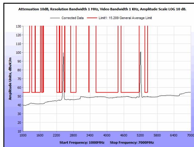
Plot 245. Radiated Spurs, Co-Location, 802.11n 20 MHz, 2437 MHz & 5200 MHz, 1 GHz – 7 GHz, Avg., Omni
