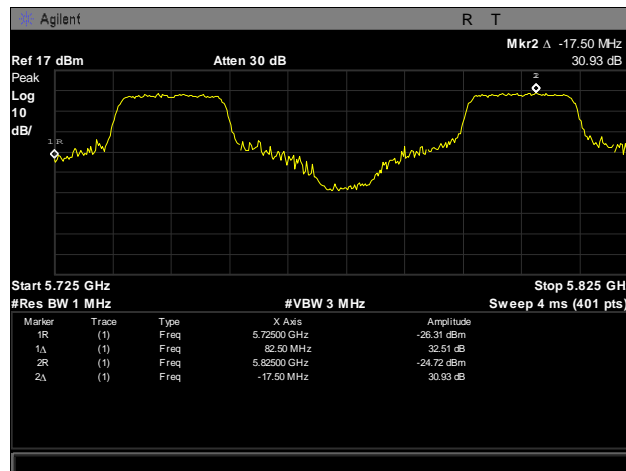
Plot 366. Frequency Stability, 5725 – 5825 MHz, -20°C, 120 V
