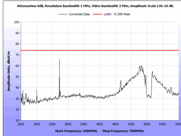
Plot 150. Radiated Spurious Emissions, 802.11n 40 MHz, High Channel, 1 GHz – 7 GHz, Peak, Patch Antenna
