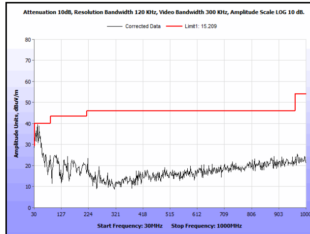
Plot 356. Radiated Spurs, Co-Location, 802.11n 20 MHz, 2462 MHz & 5580 MHz, 30 MHz – 1 GHz, Peak, Patch
