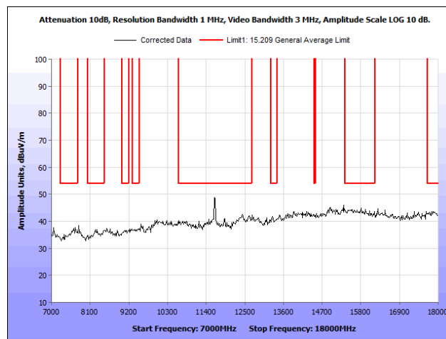
Plot 104. Radiated Spurious Emissions, 802.11n 20 MHz, High Channel, 7 GHz – 18 GHz, Omni Antenna
