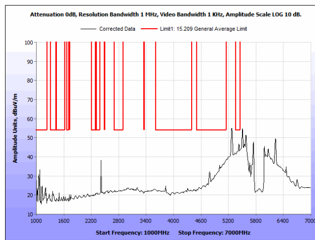
Plot 137. Radiated Spurious Emissions, 802.11n 40 MHz, Low Channel, 1 GHz – 7 GHz, Average, Patch Antenna
