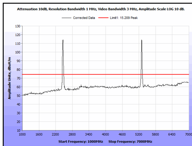
Plot 354. Radiated Spurs, Co-Location, 802.11n 20 MHz, 2462 MHz & 5300 MHz, 1 GHz – 7 GHz, Peak, Patch
