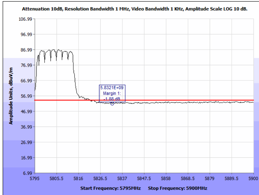
Plot 194. Radiated Band Edge, 802.11n 20 MHz, High Channel, Patch Antenna (5832 & 5835 MHz), Average
