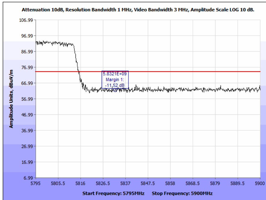
Plot 171. Radiated Band Edge, 802.11n 80 MHz, Ceiling Antenna (5832 & 5835 MHz), Peak
