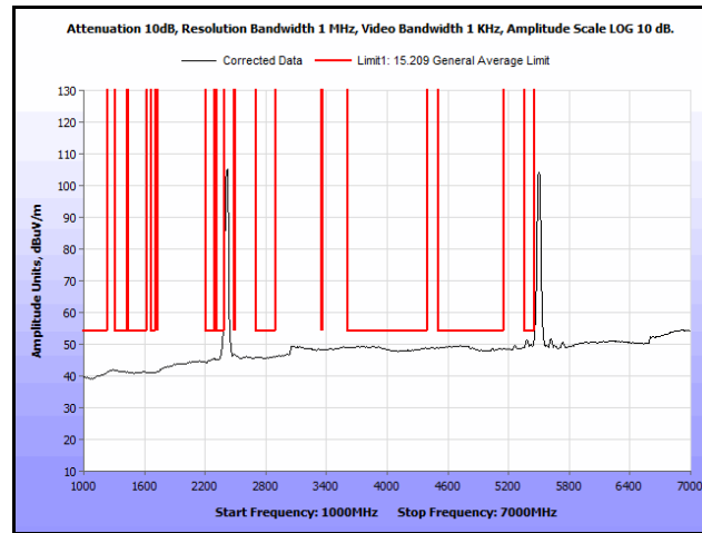
Plot 325. Radiated Spurs, Co-Location, 802.11n 20 MHz, 2412 MHz & 5580 MHz, 1 GHz – 7 GHz, Avg., Patch
