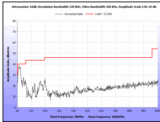
Plot 204. Radiated Spurs, Co-Location, 802.11n 20 MHz, 2412 MHz & 2412 MHz, 30 MHz – 1 GHz, Peak, Omni
