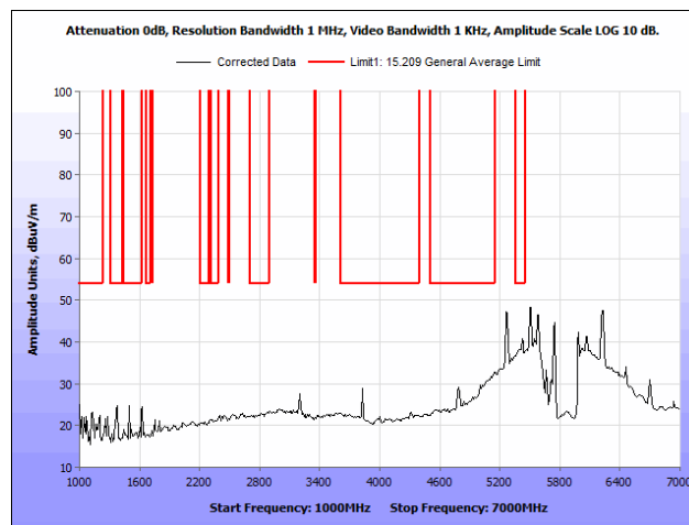
Plot 102. Radiated Spurious Emissions, 802.11n 20 MHz, High Channel, 1 GHz – 7 GHz, Average, Omni Antenna
