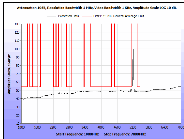
Plot 277. Radiated Spurs, Co-Location, 802.11n 20 MHz, 5200 MHz & 5200 MHz, 1 GHz – 7 GHz, Avg., Omni
