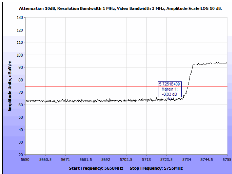
Plot 169. Radiated Band Edge, 802.11n 80 MHz, Ceiling Antenna (5715 & 5725 MHz), Peak
