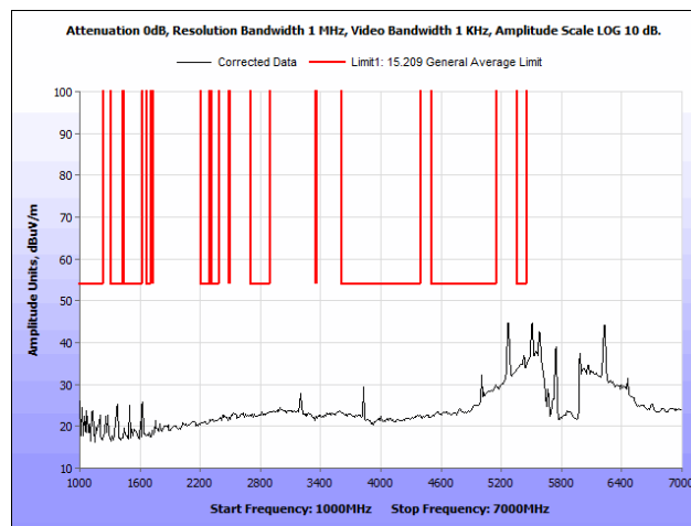
Plot 84. Radiated Spurious Emissions, 802.11a 20 MHz, High Channel, 1 GHz – 7 GHz, Average, Omni Antenna
