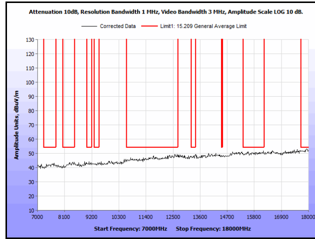
Plot 343. Radiated Spurs, Co-Location, 802.11n 20 MHz, 2437 MHz & 5580 MHz, 7 GHz – 18 GHz, Peak, Patch
