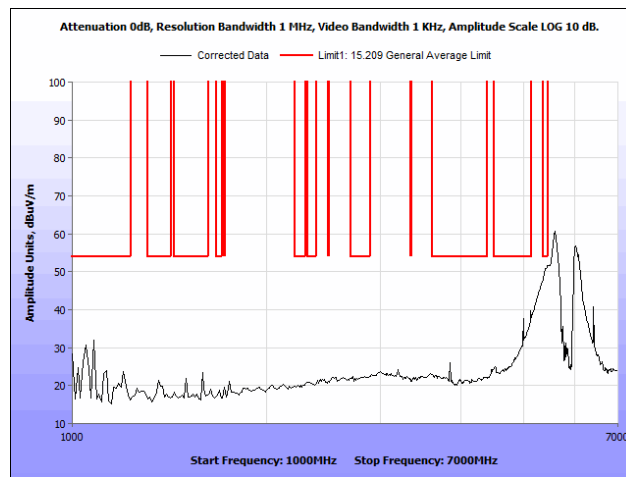
Plot 31. Radiated Spurious Emissions, 802.11a 20 MHz, Low Channel, 1 GHz – 7 GHz, Average, Ceiling Antenna
