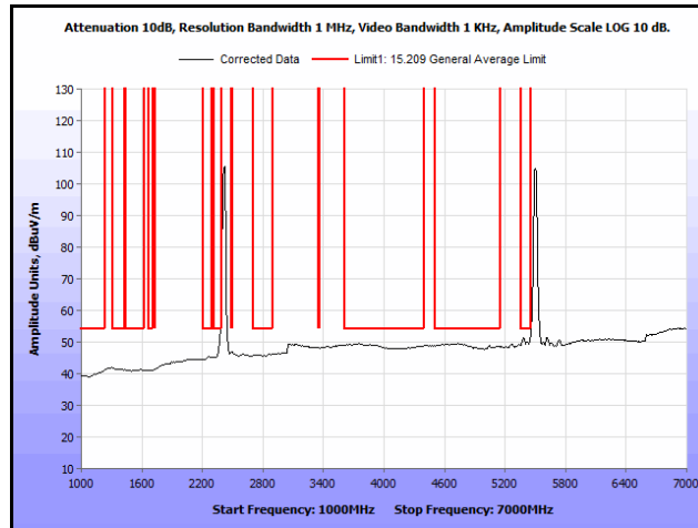
Plot 341. Radiated Spurs, Co-Location, 802.11n 20 MHz, 2437 MHz & 5580 MHz, 1 GHz – 7 GHz, Avg., Patch
