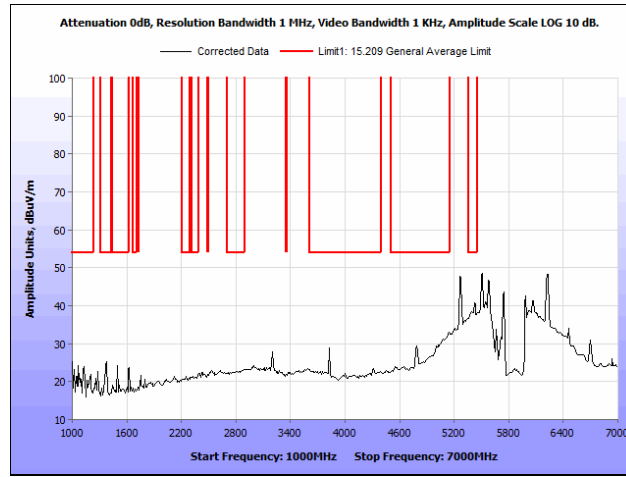
Plot 91. Radiated Spurious Emissions, 802.11n 20 MHz, Low Channel, 1 GHz – 7 GHz, Average, Omni Antenna
