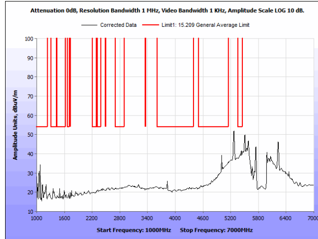
Plot 39. Radiated Spurious Emissions, 802.11a 20 MHz, Mid Channel, 1 GHz – 7 GHz, Average, Ceiling Antenna
