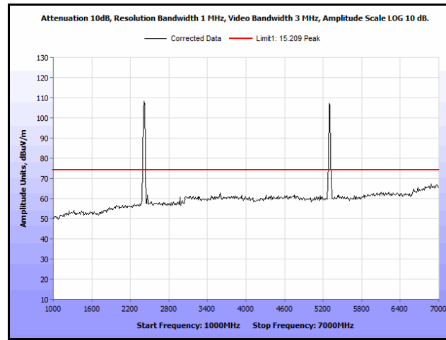
Plot 234. Radiated Spurs, Co-Location, 802.11n 20 MHz, 2412 MHz & 5300 MHz, 1 GHz – 7 GHz, Peak, Omni
