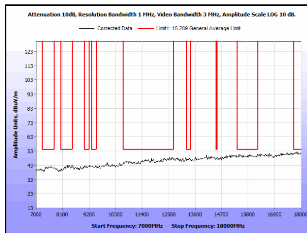
Plot 227. Radiated Spurs, Co-Location, 802.11n 20 MHz, 2462 MHz & 2462 MHz, 7 GHz – 18 GHz, Peak, Omni
