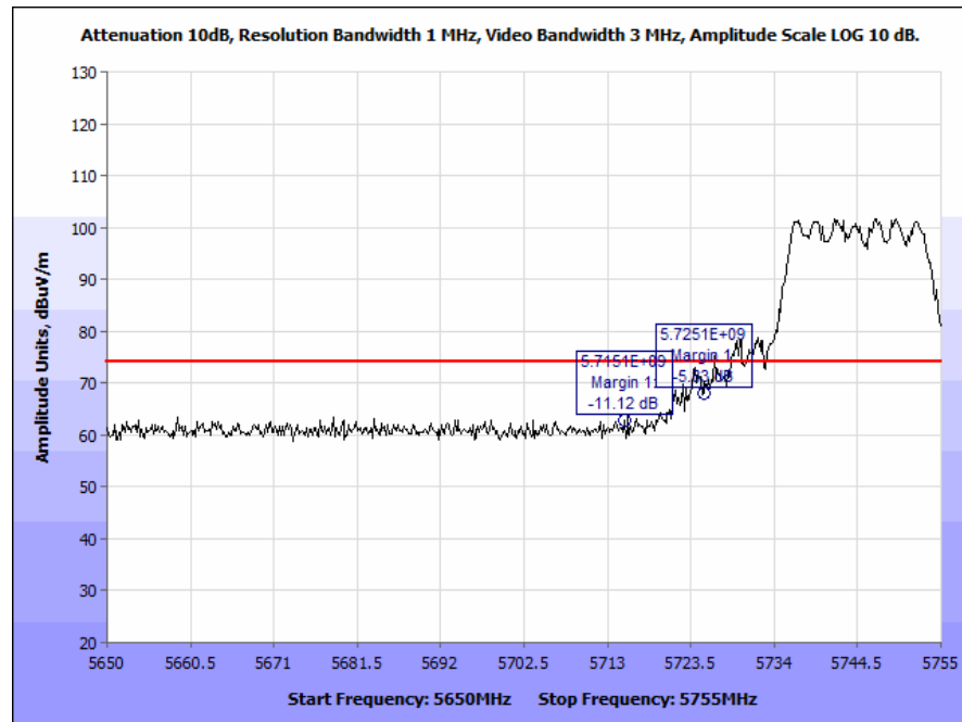
Plot 193. Radiated Band Edge, 802.11n 20 MHz, Low Channel, Patch Antenna (5725 & 5715 MHz), Peak
