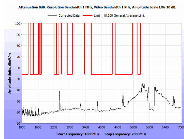
Plot 95. Radiated Spurious Emissions, 802.11n 40 MHz, Low Channel, 1 GHz – 7 GHz, Average, Omni Antenna
