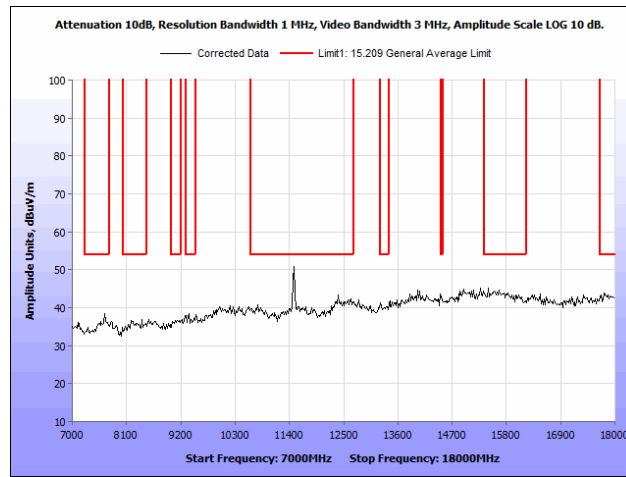
Plot 52. Radiated Spurious Emissions, 802.11n 20 MHz, Low Channel, 7 GHz – 18 GHz, Ceiling Antenna
