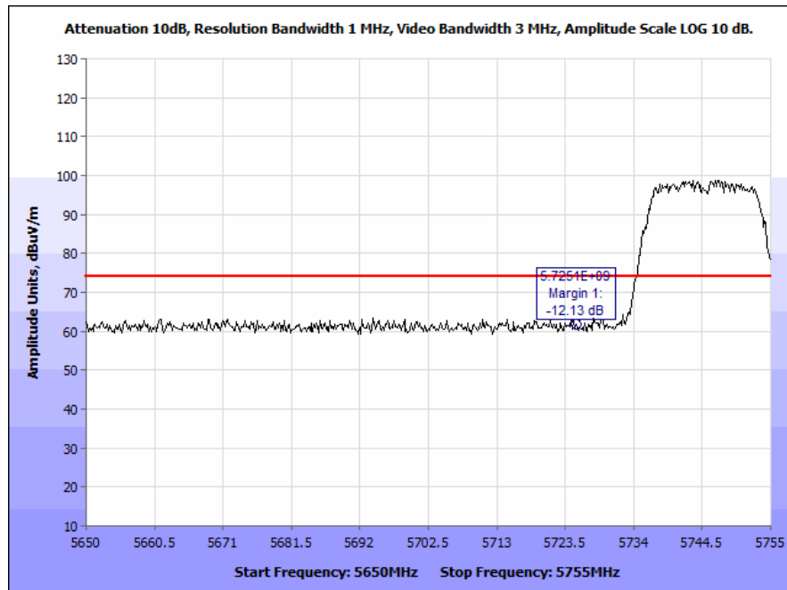
Plot 173. Radiated Band Edge, 802.11a, Low Channel, Omni Antenna (5715 & 5725 MHz), Peak
