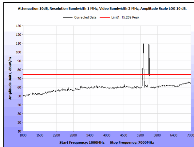
Plot 298. Radiated Spurs, Co-Location, 802.11n 20 MHz, 5300 MHz & 5580 MHz, 1 GHz – 7 GHz, Peak, Omni
