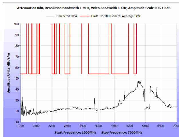
Plot 35. Radiated Spurious Emissions, 802.11a 40 MHz, Low Channel, 1 GHz – 7 GHz, Average, Ceiling Antenna
