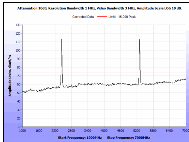
Plot 338. Radiated Spurs, Co-Location, 802.11n 20 MHz, 2437 MHz & 5300 MHz, 1 GHz – 7 GHz, Peak, Patch
