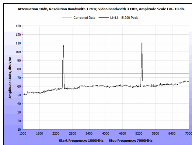
Plot 266. Radiated Spurs, Co-Location, 802.11n 20 MHz, 2462 MHz & 5300 MHz, 1 GHz – 7 GHz, Peak, Omni
