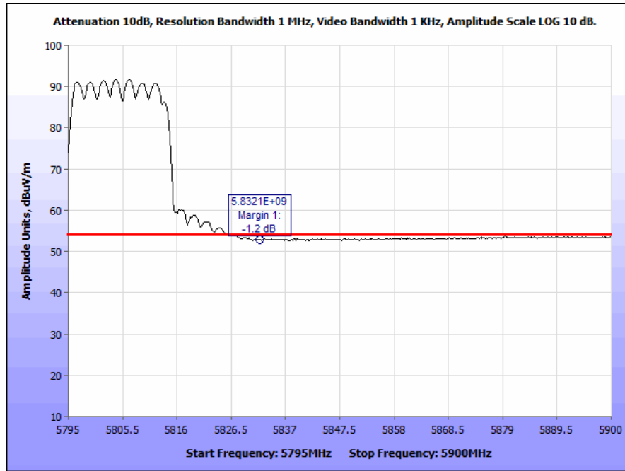
Plot 190. Radiated Band Edge, 802.11a, High Channel, Patch Antenna (5832 & 5835 MHz), Average
