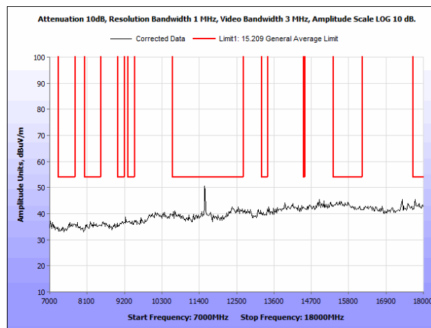
Plot 123. Radiated Spurious Emissions, 802.11a 20 MHz, Mid Channel, 7 GHz – 18 GHz, Patch Antenna
