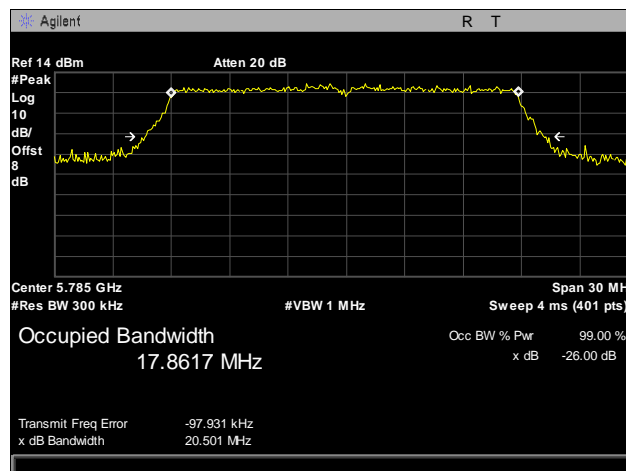
Plot 20. 26 dB Occupied Bandwidth, 802.11n, 5785 MHz, Port 1
