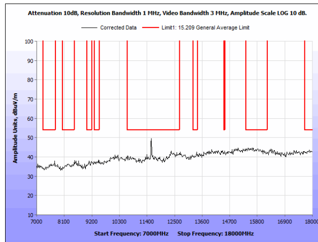
Plot 101. Radiated Spurious Emissions, 802.11n 20 MHz, Mid Channel, 7 GHz – 18 GHz, Omni Antenna
