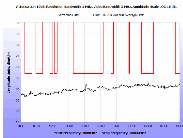
Plot 97. Radiated Spurious Emissions, 802.11n 40 MHz, Low Channel, 7 GHz – 18 GHz, Omni Antenna
