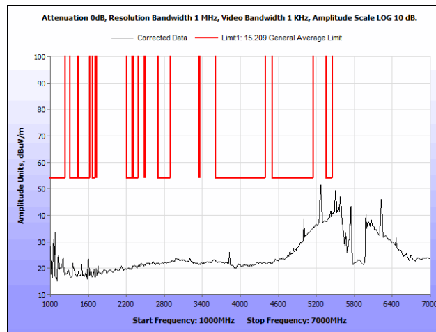
Plot 125. Radiated Spurious Emissions, 802.11a 20 MHz, High Channel, 1 GHz – 7 GHz, Average, Patch Antenna
