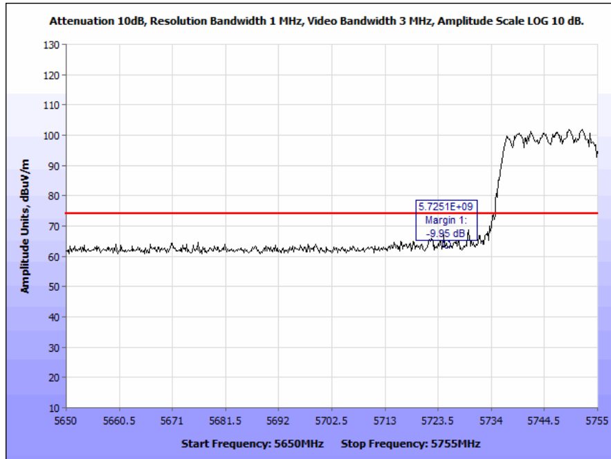
Plot 165. Radiated Band Edge, 802.11n 40 MHz, Low Channel, Ceiling Antenna (5715 & 5725 MHz), Peak
