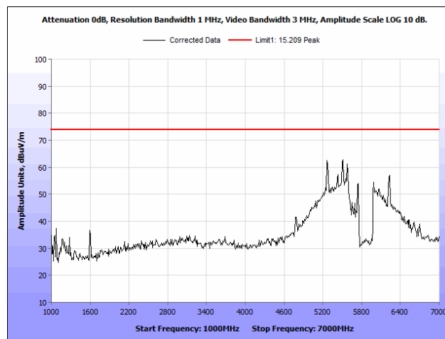
Plot 142. Radiated Spurious Emissions, 802.11n 20 MHz, Mid Channel, 1 GHz – 7 GHz, Peak, Patch Antenna
