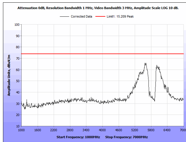
Plot 110. Radiated Spurious Emissions, 802.11ac 80 MHz, 1 GHz – 7 GHz, Peak, Omni Antenna
