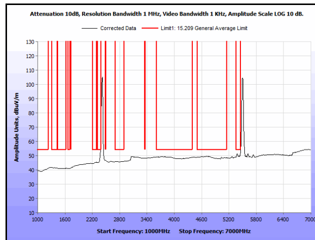
Plot 357. Radiated Spurs, Co-Location, 802.11n 20 MHz, 2462 MHz & 5580 MHz, 1 GHz – 7 GHz, Avg., Patch
