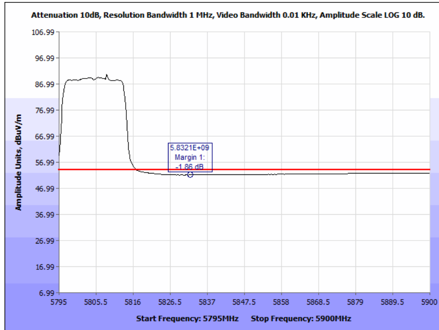
Plot 158. Radiated Band Edge, 802.11a, High Channel, Ceiling Antenna (5825 & 5835 MHz), Average
