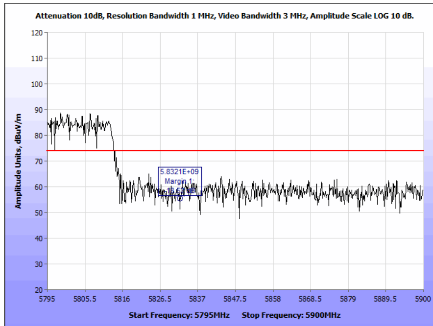
Plot 203. Radiated Band Edge, 802.11n 80 MHz, Patch Antenna (5832 & 5835 MHz), Peak
