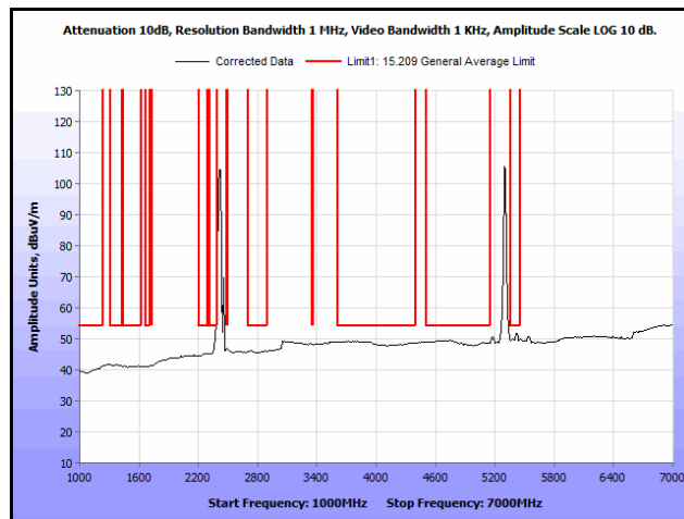
Plot 353. Radiated Spurs, Co-Location, 802.11n 20 MHz, 2462 MHz & 5300 MHz, 1 GHz – 7 GHz, Avg., Patch
