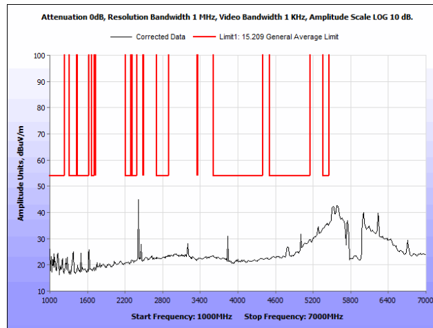
Plot 77. Radiated Spurious Emissions, 802.11a 40 MHz, Low Channel, 1 GHz – 7 GHz, Average, Omni Antenna
