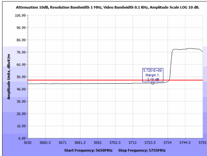
Plot 184. Radiated Band Edge, 802.11ac 80 MHz, Omni Antenna (5715 & 5725 MHz), Average
