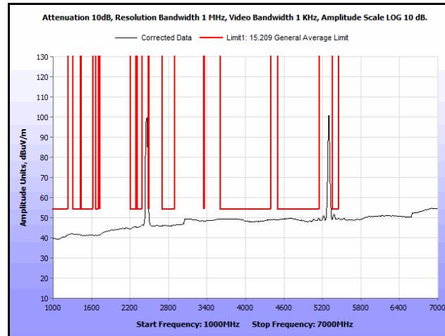
Plot 265. Radiated Spurs, Co-Location, 802.11n 20 MHz, 2462 MHz & 5300 MHz, 1 GHz – 7 GHz, Avg., Omni
