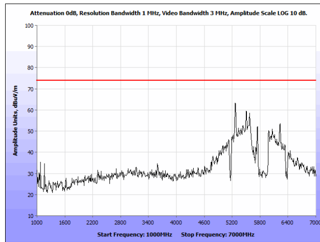
Plot 51. Radiated Spurious Emissions, 802.11n 20 MHz, Low Channel, 1 GHz – 7 GHz, Peak, Ceiling Antenna
