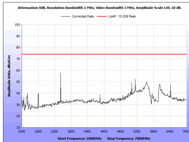
Plot 154. Radiated Spurious Emissions, 802.11ac 80 MHz, 1 GHz – 7 GHz, Peak, Patch Antenna
