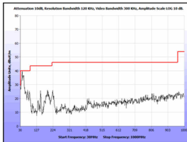
Plot 87. Radiated Spurious Emissions, 802.11a 40 MHz, High Channel, 30 MHz – 1 GHz, Omni Antenna
