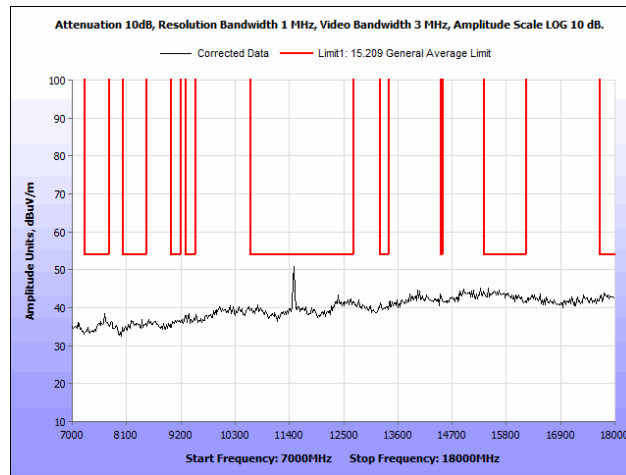
Plot 135. Radiated Spurious Emissions, 802.11n 20 MHz, Low Channel, 7 GHz – 18 GHz, Patch Antenna
