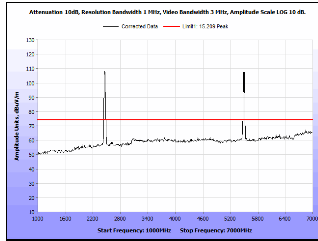
Plot 270. Radiated Spurs, Co-Location, 802.11n 20 MHz, 2462 MHz & 5580 MHz, 1 GHz – 7 GHz, Peak, Omni
