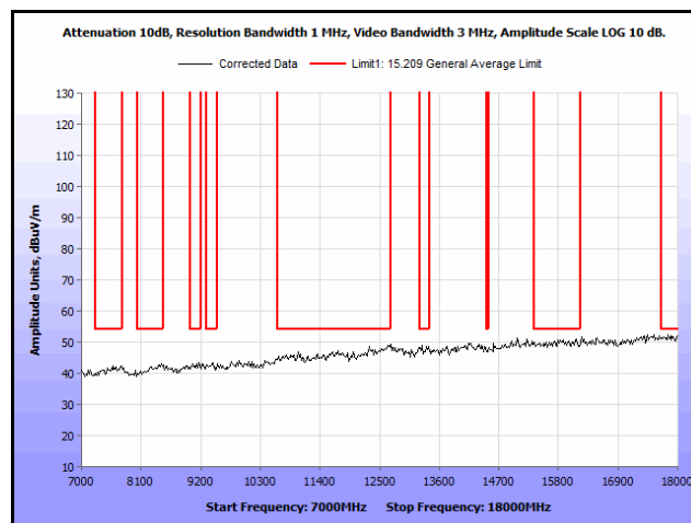
Plot 215. Radiated Spurs, Co-Location, 802.11n 20 MHz, 2412 MHz & 2462 MHz, 7 GHz – 18 GHz, Peak, Omni
