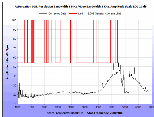
Plot 50. Radiated Spurious Emissions, 802.11n 20 MHz, Low Channel, 1 GHz – 7 GHz, Average, Ceiling Antenna
