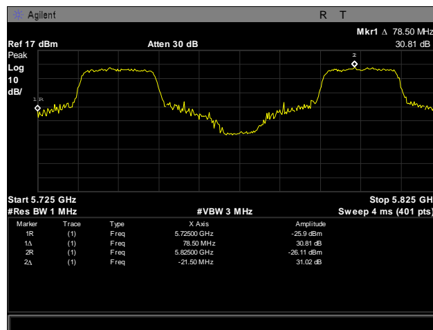
Plot 368. Frequency Stability, 5725 – 5825 MHz, 0°C, 120 V
