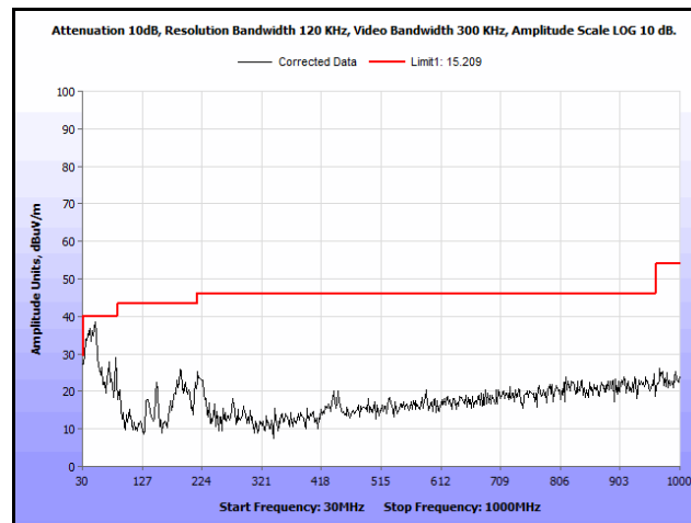
Plot 280. Radiated Spurs, Co-Location, 802.11n 20 MHz, 5200 MHz & 5300 MHz, 30 MHz – 1 GHz, Peak, Omni
