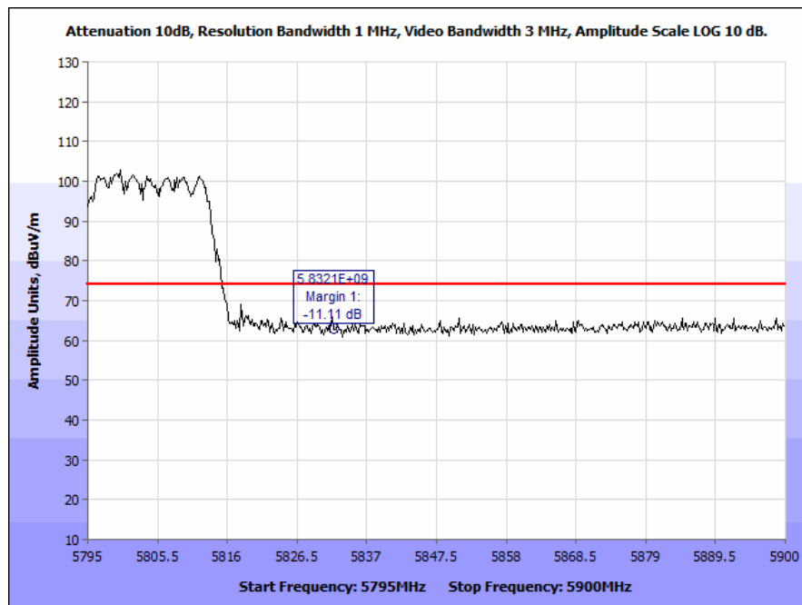
Plot 167. Radiated Band Edge, 802.11n 40 MHz, High Channel, Ceiling Antenna (5832 & 5835 MHz), Peak
