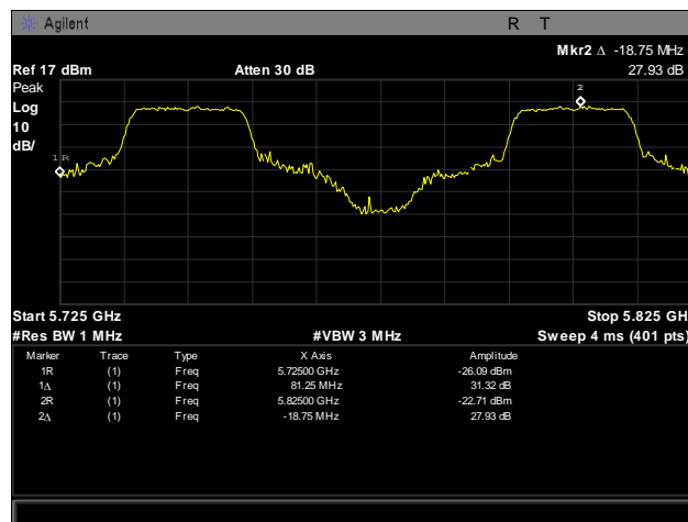
Plot 372. Frequency Stability, 5725 – 5825 MHz, 40°C, 120 V
