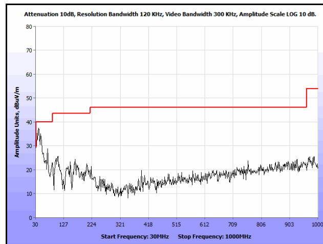
Plot 304. Radiated Spurs, Co-Location, 802.11n 20 MHz, 5580 MHz & 5580 MHz, 30 MHz – 1 GHz, Peak, Omni
