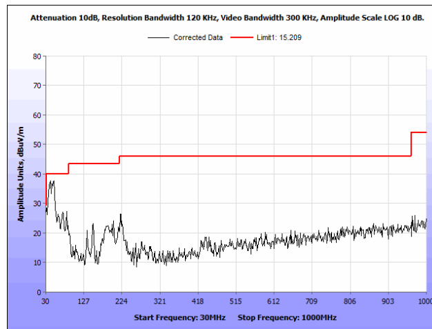
Plot 148. Radiated Spurious Emissions, 802.11n 40 MHz, High Channel, 30 MHz – 1 GHz, Patch Antenna
