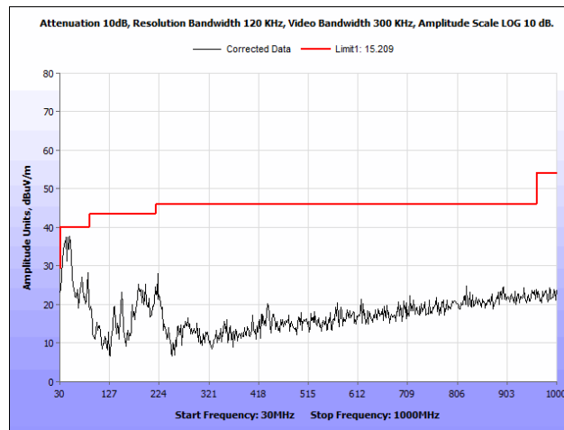
Plot 128. Radiated Spurious Emissions, 802.11a 40 MHz, High Channel, 30 MHz – 1 GHz, Patch Antenna
