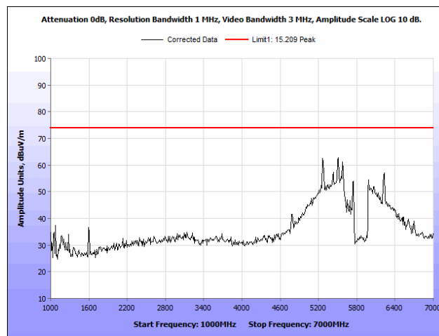
Plot 59. Radiated Spurious Emissions, 802.11n 20 MHz, Mid Channel, 1 GHz – 7 GHz, Peak, Ceiling Antenna
