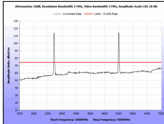
Plot 350. Radiated Spurs, Co-Location, 802.11n 20 MHz, 2462 MHz & 5200 MHz, 1 GHz – 7 GHz, Peak, Patch
