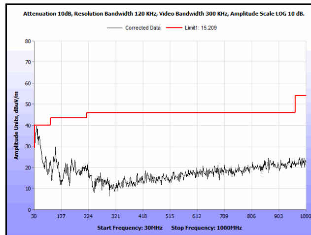
Plot 332. Radiated Spurs, Co-Location, 802.11n 20 MHz, 2437 MHz & 5200 MHz, 30 MHz – 1 GHz, Peak, Patch
