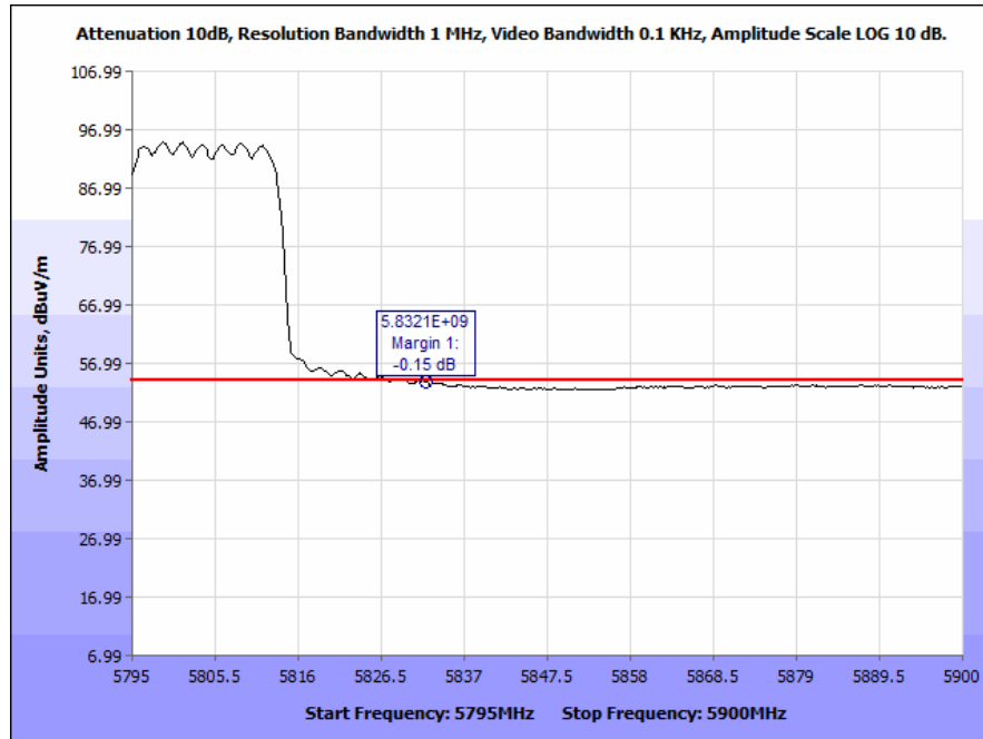
Plot 182. Radiated Band Edge, 802.11n 40 MHz, High Channel, Omni Antenna (5832 & 5835 MHz), Average
