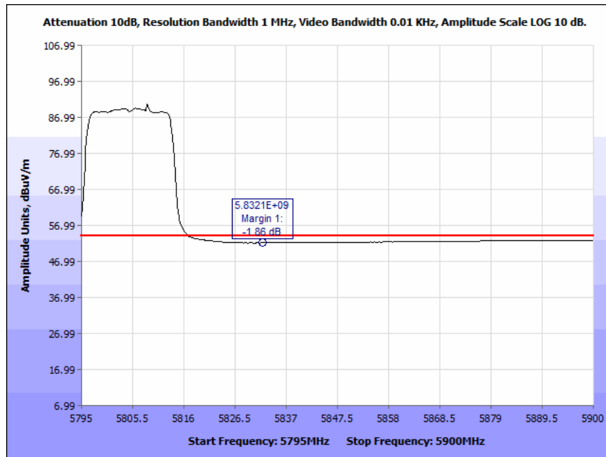
Plot 166. Radiated Band Edge, 802.11n 40 MHz, High Channel, Ceiling Antenna (5832 & 5835 MHz), Average
