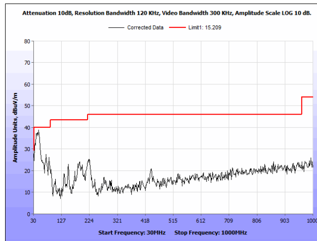
Plot 34. Radiated Spurious Emissions, 802.11a 40 MHz, Low Channel, 30 MHz – 1 GHz, Ceiling Antenna
