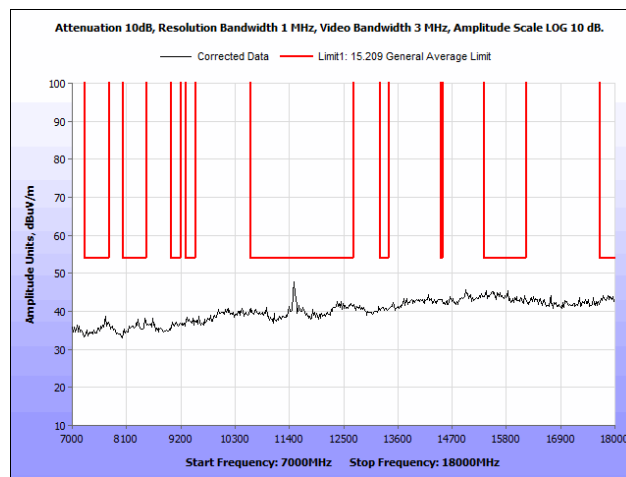
Plot 119. Radiated Spurious Emissions, 802.11a 40 MHz, Low Channel, 7 GHz – 18 GHz, Patch Antenna
