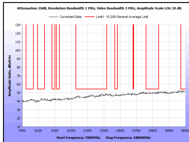
Plot 211. Radiated Spurs, Co-Location, 802.11n 20 MHz, 2412 MHz & 2437 MHz, 7 GHz – 18 GHz, Peak, Omni
