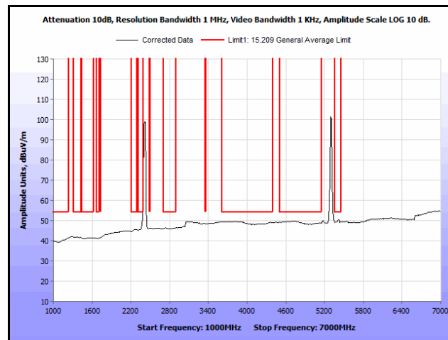
Plot 233. Radiated Spurs, Co-Location, 802.11n 20 MHz, 2412 MHz & 5300 MHz, 1 GHz – 7 GHz, Avg., Omni
