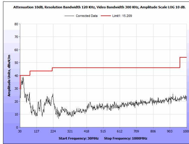
Plot 42. Radiated Spurious Emissions, 802.11a 20 MHz, High Channel, 30 MHz – 1 GHz, Ceiling Antenna
