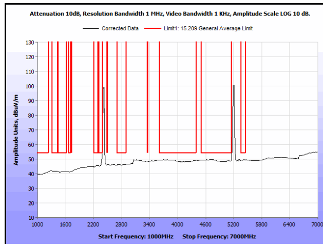
Plot 229. Radiated Spurs, Co-Location, 802.11n 20 MHz, 2412 MHz & 5200 MHz, 1 GHz – 7 GHz, Avg., Omni
