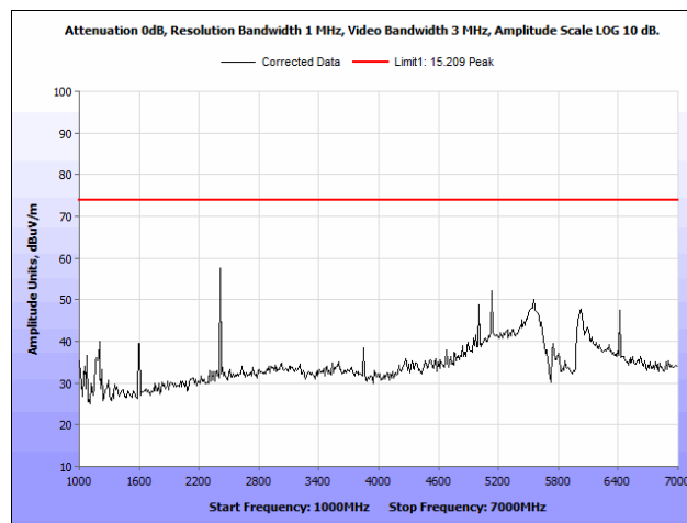
Plot 71. Radiated Spurious Emissions, 802.11ac 80 MHz, 1 GHz – 7 GHz, Peak, Ceiling Antenna
