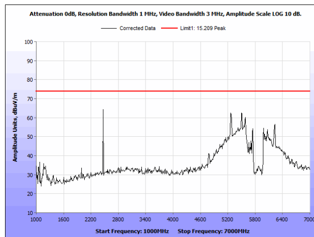
Plot 32. Radiated Spurious Emissions, 802.11a 20 MHz, Low Channel, 1 GHz – 7 GHz, Peak, Ceiling Antenna
