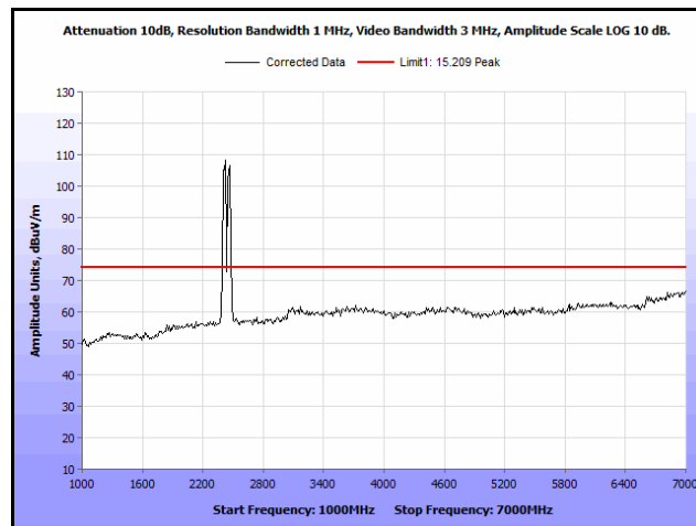
Plot 214. Radiated Spurs, Co-Location, 802.11n 20 MHz, 2412 MHz & 2462 MHz, 1 GHz – 7 GHz, Peak, Omni
