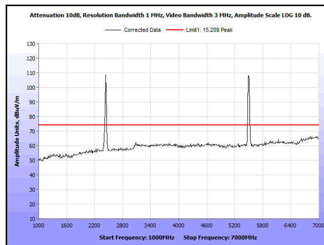
Plot 254. Radiated Spurs, Co-Location, 802.11n 20 MHz, 2437 MHz & 5580 MHz, 1 GHz – 7 GHz, Peak, Omni
