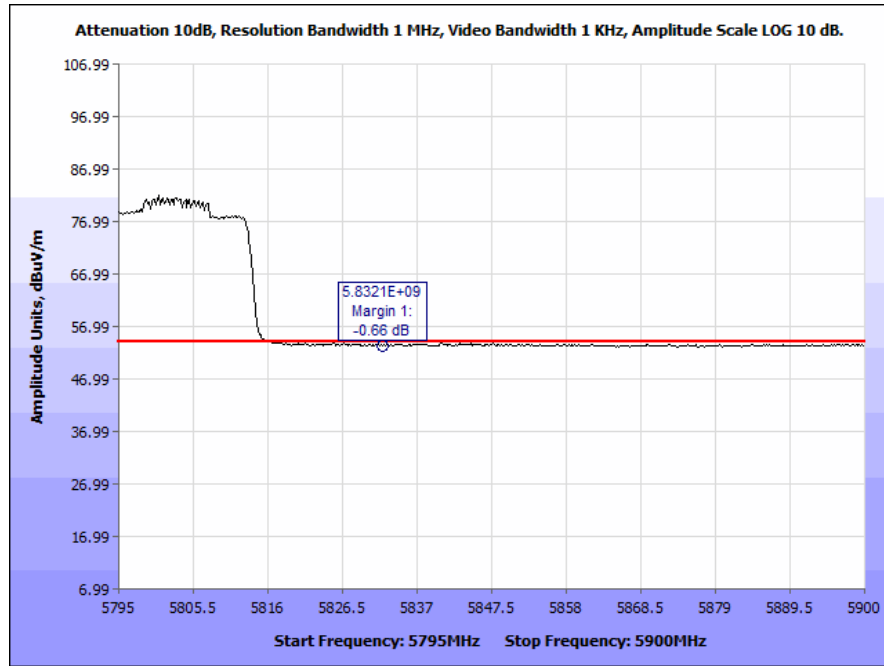
Plot 202. Radiated Band Edge, 802.11n 80 MHz, Patch Antenna (5832 & 5835 MHz), Average
