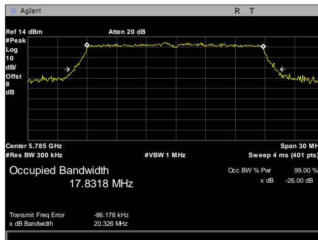
Plot 25. 26 dB Occupied Bandwidth, 802.11n, 5785 MHz, Port 2
