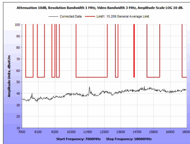
Plot 68. Radiated Spurious Emissions, 802.11n 40 MHz, High Channel, 7 GHz – 18 GHz, Peak, Ceiling Antenna
