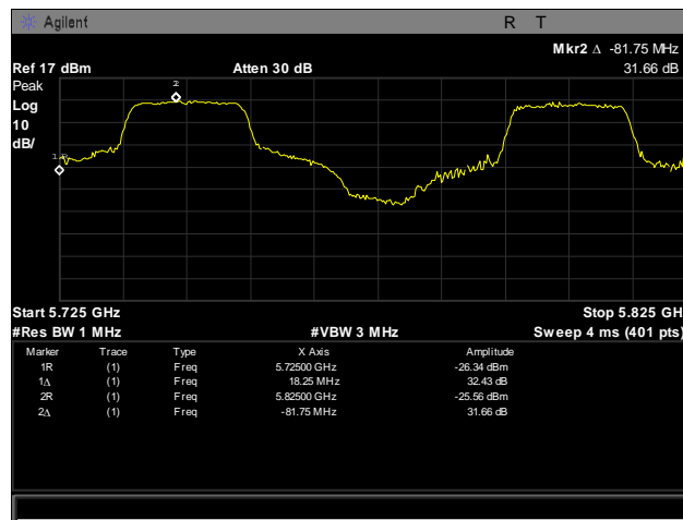
Plot 365. Frequency Stability, 5725 – 5825 MHz, -30°C, 120 V
