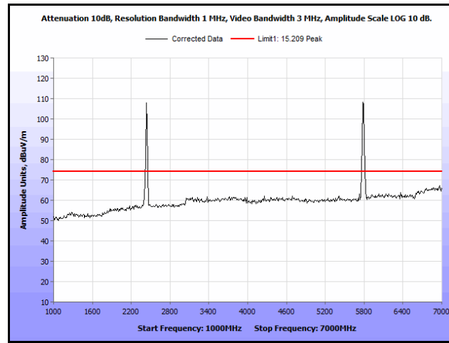
Plot 258. Radiated Spurs, Co-Location, 802.11n 20 MHz, 2437 MHz & 5785 MHz, 1 GHz – 7 GHz, Peak, Omni
