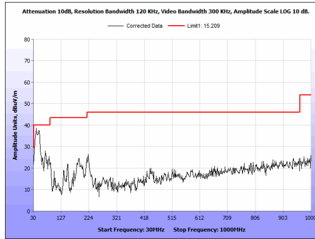
Plot 112. Radiated Spurious Emissions, 802.11a 20 MHz, Low Channel, 30 MHz – 1 GHz, Patch Antenna
