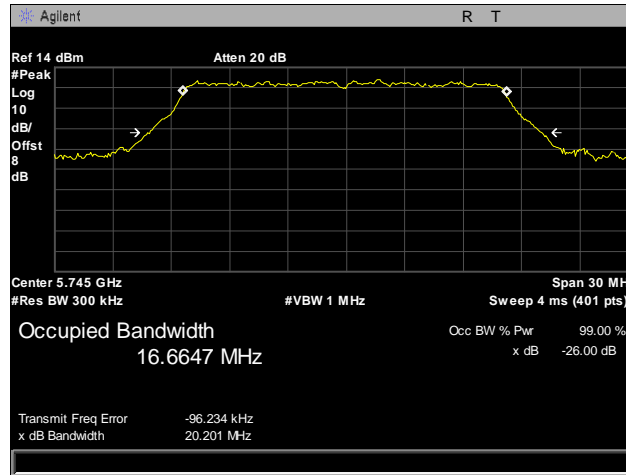
Plot 13. 26 dB Occupied Bandwidth, 802.11a, 5745 MHz
