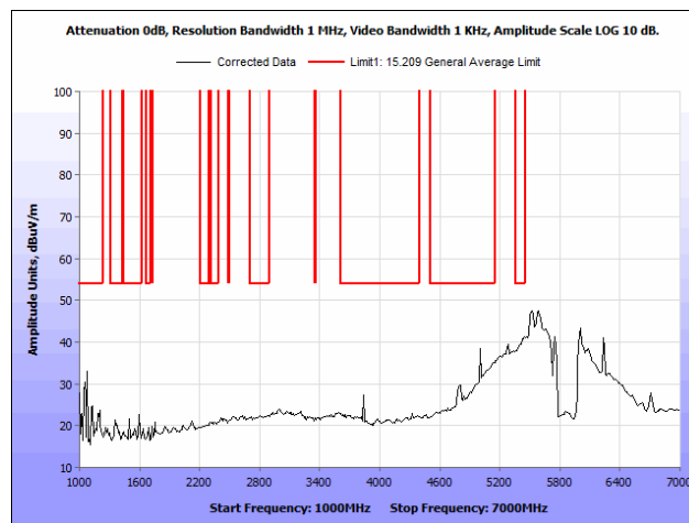
Plot 149. Radiated Spurious Emissions, 802.11n 40 MHz, High Channel, 1 GHz – 7 GHz, Average, Patch Antenna
