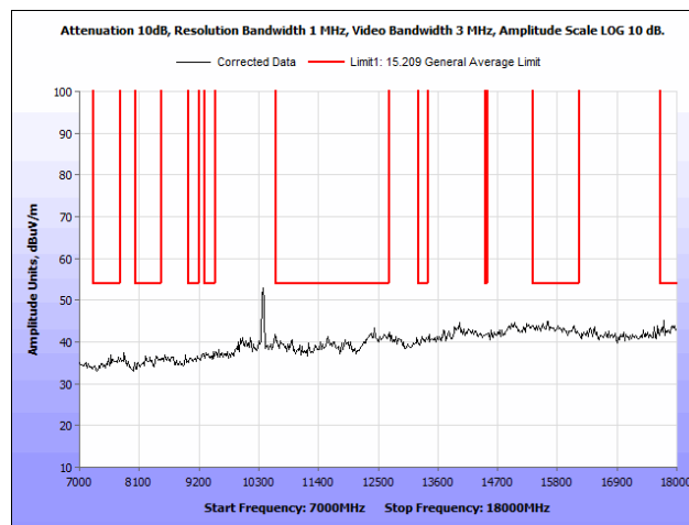
Plot 103. Radiated Spurious Emissions, 802.11n, 40 MHz, High Channel, 7 GHz – 18 GHz, Omni Antenna
