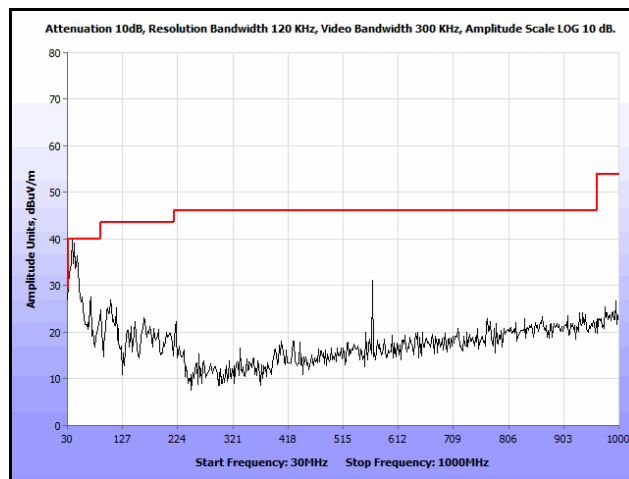
Plot 263. Radiated Spurs, Co-Location, 802.11n 20 MHz, 2437 MHz & 5785 MHz, 30 MHz – 1 GHz, Peak, Omni
