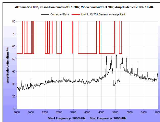
Plot 96. Radiated Spurious Emissions, 802.11n, 20 MHz, Mid Channel, 1 GHz – 7 GHz, Average, Omni Antenna
