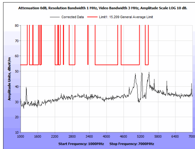
Plot 87. Radiated Spurious Emissions, 802.11a, 40 MHz, High Channel, 1 GHz – 7 GHz, Average, Omni Antenna
