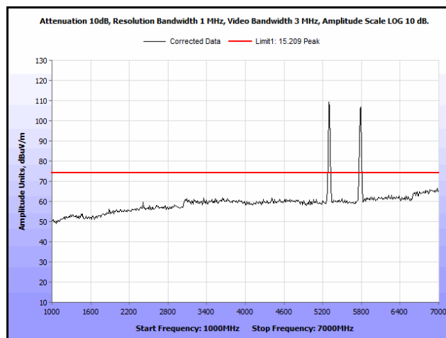
Plot 309. Radiated Spurs, Co-Location, 802.11n 20 MHz, 5300 MHz & 5785 MHz, 1 GHz – 7 GHz, Peak, Omni
