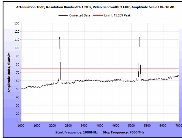
Plot 365. Radiated Spurs, Co-Location, 802.11n 20 MHz, 2462 MHz & 5580 MHz, 1 GHz – 7 GHz, Peak, Patch
