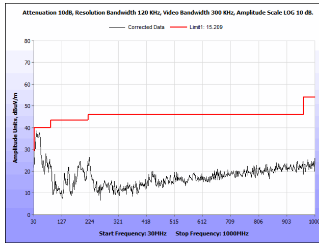
Plot 107. Radiated Spurious Emissions, 802.11a, 20 MHz, Low Channel, 30 MHz – 1 GHz, Patch Antenna
