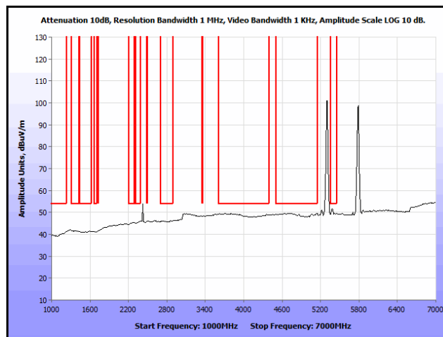
Plot 308. Radiated Spurs, Co-Location, 802.11n 20 MHz, 5300 MHz & 5785 MHz, 1 GHz – 7 GHz, Avg., Omni
