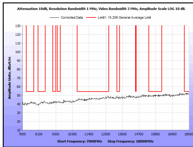
Plot 314. Radiated Spurs, Co-Location, 802.11n 20 MHz, 5580 MHz & 5580 MHz, 7 GHz – 18 GHz, Peak, Omni
