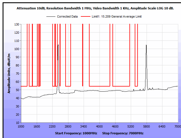
Plot 336. Radiated Spurs, Co-Location, 802.11n 20 MHz, 2412 MHz & 5785 MHz, 1 GHz – 7 GHz, Avg., Patch
