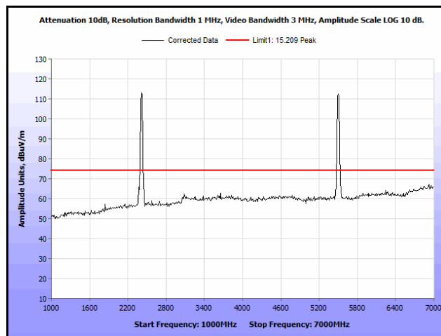
Plot 333. Radiated Spurs, Co-Location, 802.11n 20 MHz, 2412 MHz & 5580 MHz, 1 GHz – 7 GHz, Peak, Patch
