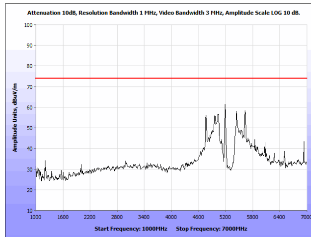
Plot 137. Radiated Spurious Emissions, 802.11n, 20 MHz, Mid Channel, 1 GHz – 7 GHz, Patch Antenna
