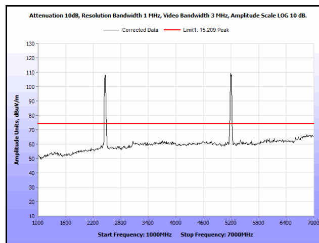
Plot 269. Radiated Spurs, Co-Location, 802.11n 20 MHz, 2462 MHz & 5200 MHz, 1 GHz – 7 GHz, Peak, Omni
