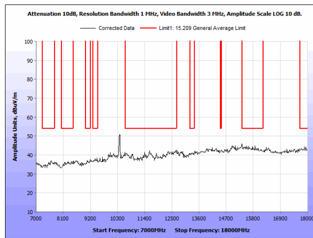
Plot 94. Radiated Spurious Emissions, 802.11n, 40 MHz, Low Channel, 7 GHz – 18 GHz, Omni Antenna
