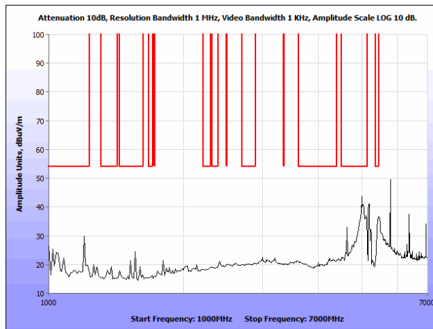
Plot 72. Radiated Spurious Emissions, 802.11ac, 1 GHz – 7 GHz, Peak, Ceiling Antenna
