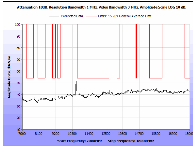
Plot 146. Radiated Spurious Emissions, 802.11n, 40 MHz, High Channel, 7 GHz – 18 GHz, Peak, Patch Antenna
