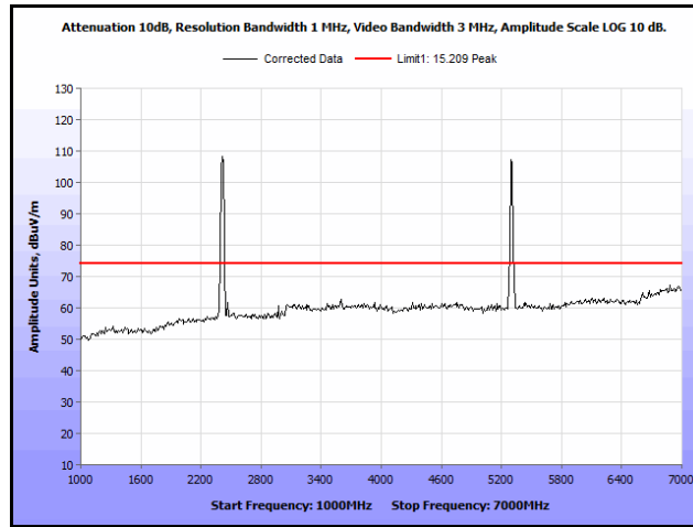
Plot 241. Radiated Spurs, Co-Location, 802.11n 20 MHz, 2412 MHz & 5300 MHz, 1 GHz – 7 GHz, Peak, Omni
