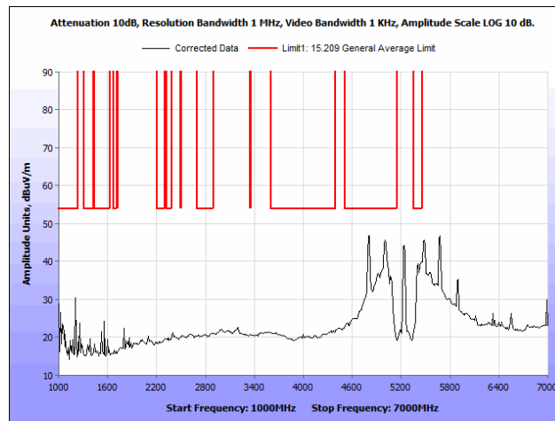
Plot 120. Radiated Spurious Emissions, 802.11a, 20 MHz, High Channel, 1 GHz – 7 GHz, Average, Patch Antenna
