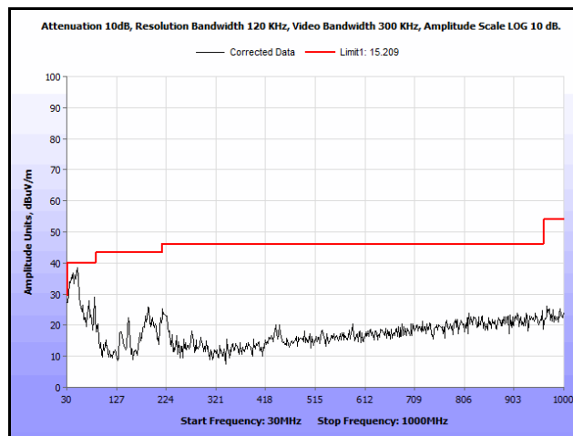
Plot 287. Radiated Spurs, Co-Location, 802.11n 20 MHz, 5200 MHz & 5300 MHz, 30 MHz – 1 GHz, Peak, Omni
