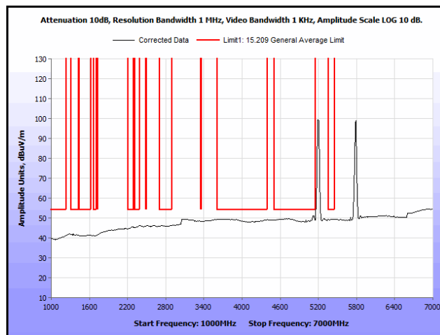
Plot 296. Radiated Spurs, Co-Location, 802.11n 20 MHz, 5200 MHz & 5785 MHz, 1 GHz – 7 GHz, Avg., Omni
