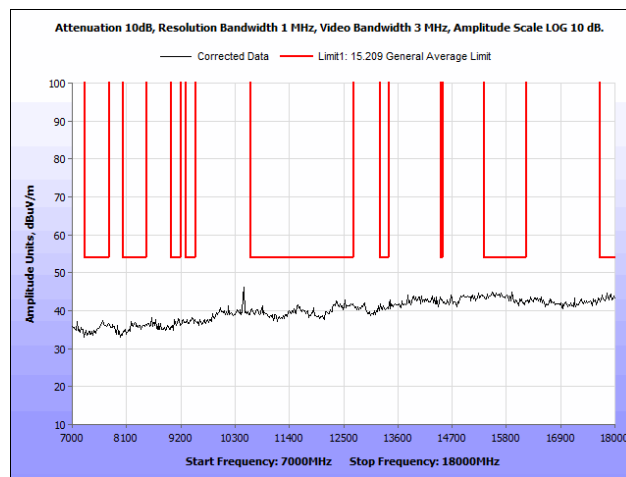
Plot 85. Radiated Spurious Emissions, 802.11a, 20 MHz, High Channel, 7 GHz – 18 GHz, Omni Antenna
