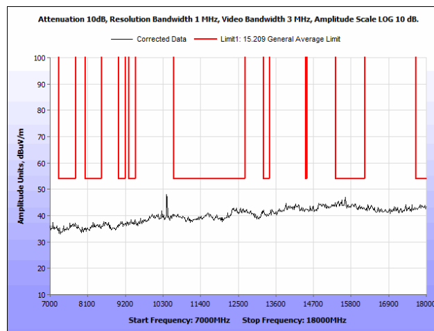
Plot 82. Radiated Spurious Emissions, 802.11a, 20 MHz, Mid Channel, 7 GHz – 18 GHz, Omni Antenna
