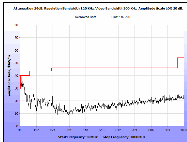
Plot 363. Radiated Spurs, Co-Location, 802.11n 20 MHz, 2462 MHz & 5580 MHz, 30 MHz – 1 GHz, Peak, Patch
