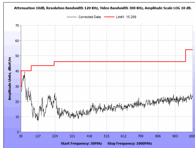
Plot 54. Radiated Spurious Emissions, 802.11n, 40 MHz, Low Channel, 30 MHz – 1 GHz, Ceiling Antenna
