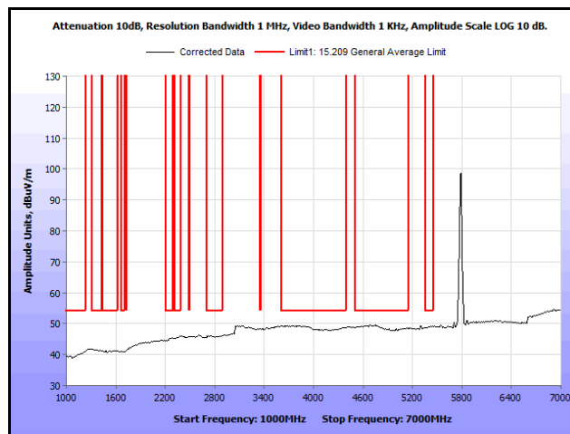
Plot 320. Radiated Spurs, Co-Location, 802.11n 20 MHz, 5785 MHz & 5785 MHz, 1 GHz – 7 GHz, Avg., Omni
