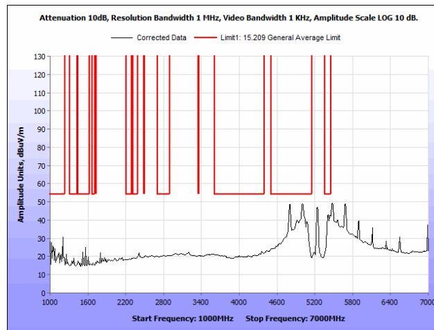
Plot 63. Radiated Spurious Emissions, 802.11n, High Channel, 1 GHz – 7 GHz, Average, Ceiling Antenna
