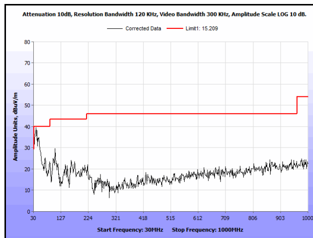
Plot 251. Radiated Spurs, Co-Location, 802.11n 20 MHz, 2437 MHz & 5200 MHz, 30 MHz – 1 GHz, Peak, Omni
