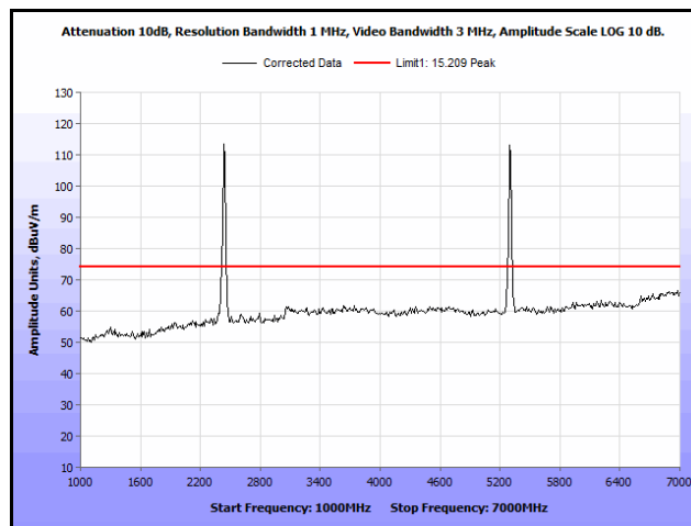
Plot 345. Radiated Spurs, Co-Location, 802.11n 20 MHz, 2437 MHz & 5300 MHz, 1 GHz – 7 GHz, Peak, Patch
