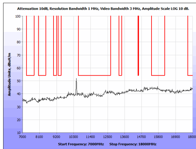
Plot 100. Radiated Spurious Emissions, 802.11n, 20 MHz, High Channel, 7 GHz – 18 GHz, Omni Antenna
