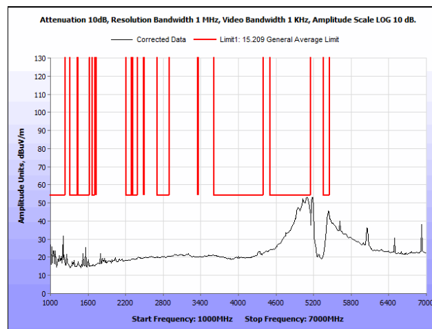
Plot 55. Radiated Spurious Emissions, 802.11n, 40 MHz, Low Channel, 1 GHz – 7 GHz, Average, Ceiling Antenna
