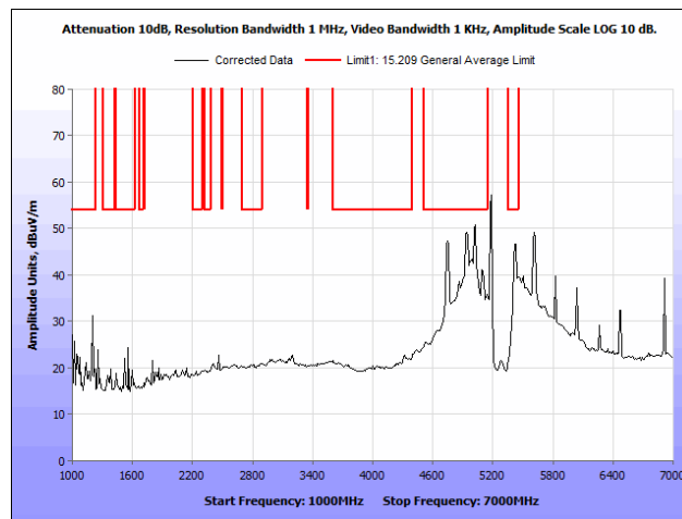
Plot 128. Radiated Spurious Emissions, 802.11n, 20 MHz, Low Channel, 1 GHz – 7 GHz, Average, Patch Antenna
