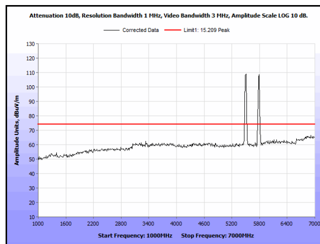
Plot 317. Radiated Spurs, Co-Location, 802.11n 20 MHz, 5580 MHz & 5785 MHz, 1 GHz – 7 GHz, Peak, Omni
