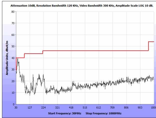
Plot 70. Radiated Spurious Emissions, 802.11ac, 80 MHz, 30 MHz – 1 GHz, Ceiling Antenna
