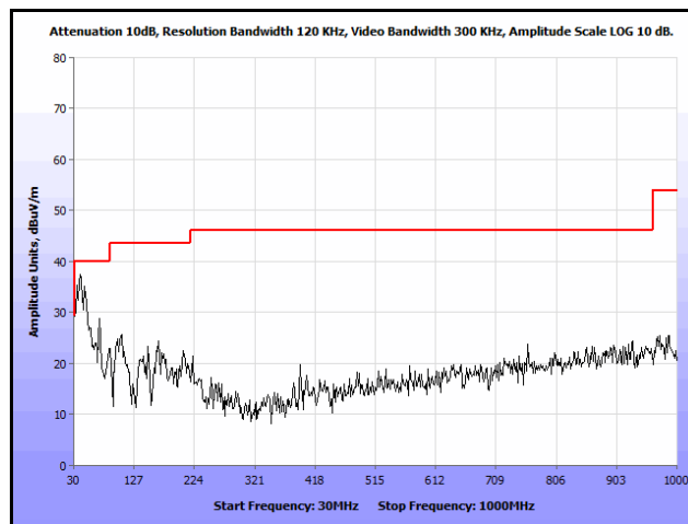
Plot 311. Radiated Spurs, Co-Location, 802.11n 20 MHz, 5580 MHz & 5580 MHz, 30 MHz – 1 GHz, Peak, Omni
