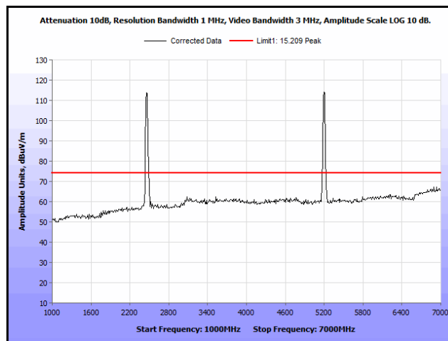
Plot 357. Radiated Spurs, Co-Location, 802.11n 20 MHz, 2462 MHz & 5200 MHz, 1 GHz – 7 GHz, Peak, Patch
