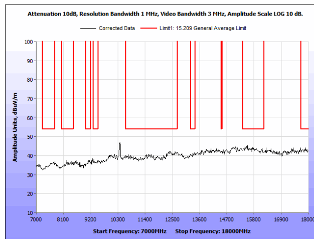
Plot 88. Radiated Spurious Emissions, 802.11a, 40 MHz, High Channel, 7 GHz – 18 GHz, Omni Antenna
