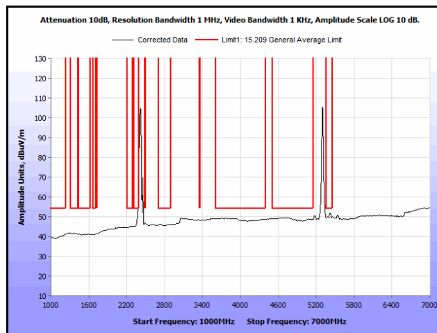
Plot 360. Radiated Spurs, Co-Location, 802.11n 20 MHz, 2462 MHz & 5300 MHz, 1 GHz – 7 GHz, Avg., Patch
