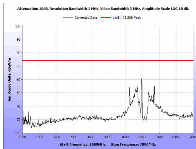
Plot 117. Radiated Spurious Emissions, 802.11a, 20 MHz, Mid Channel, 1 GHz – 7 GHz, Peak, Patch Antenna
