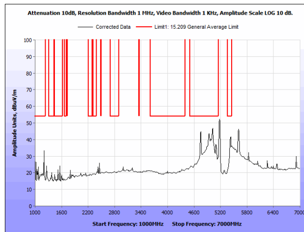
Plot 108. Radiated Spurious Emissions, 802.11a, 20 MHz, Low Channel, 1 GHz – 7 GHz, Average, Patch Antenna
