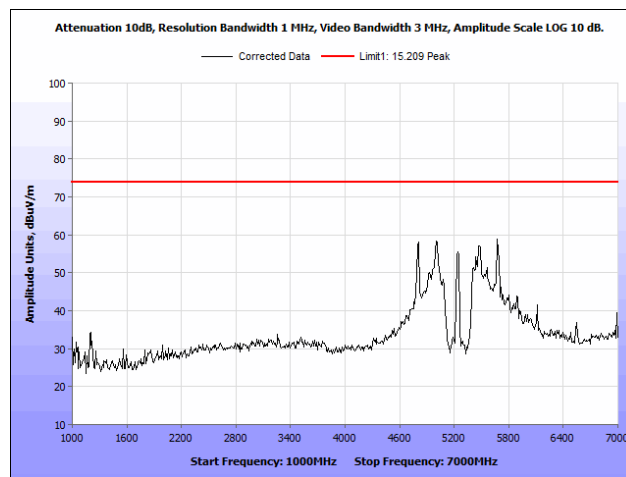
Plot 141. Radiated Spurious Emissions, 802.11n, 20 MHz, High Channel, 1 GHz – 7 GHz, Peak, Patch Antenna
