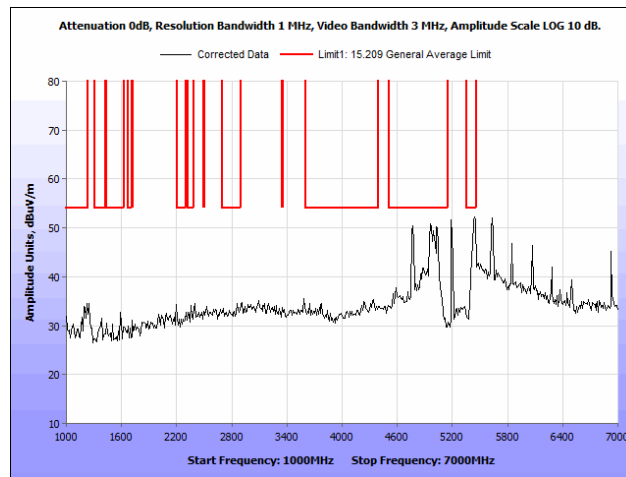
Plot 81. Radiated Spurious Emissions, 802.11a, 20 MHz, Mid Channel, 1 GHz – 7 GHz, Average, Omni Antenna
