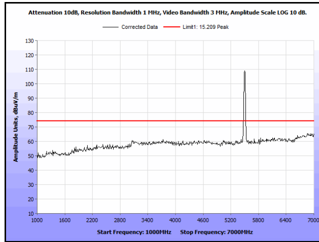
Plot 313. Radiated Spurs, Co-Location, 802.11n 20 MHz, 5580 MHz & 5580 MHz, 1 GHz – 7 GHz, Peak, Omni
