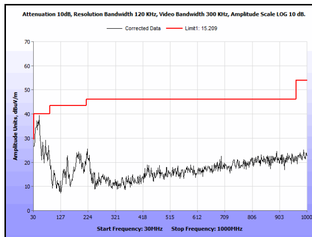
Plot 239. Radiated Spurs, Co-Location, 802.11n 20 MHz, 2412 MHz & 5300 MHz, 30 MHz – 1 GHz, Peak, Omni
