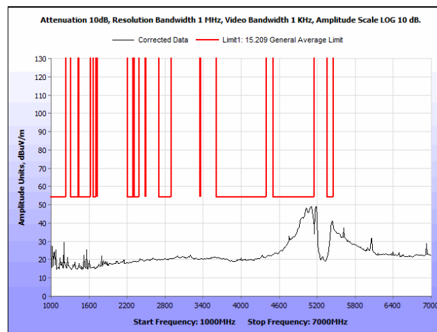
Plot 112. Radiated Spurious Emissions, 802.11a, 40 MHz, Low Channel, 1 GHz – 7 GHz, Average, Patch Antenna
