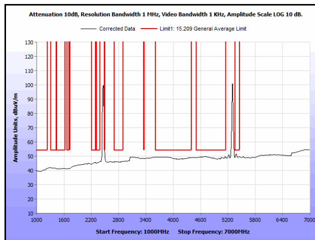
Plot 272. Radiated Spurs, Co-Location, 802.11n 20 MHz, 2462 MHz & 5300 MHz, 1 GHz – 7 GHz, Avg., Omni
