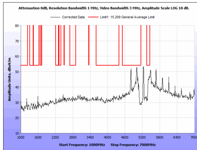
Plot 99. Radiated Spurious Emissions, 802.11n, 20 MHz, High Channel, 1 GHz – 7 GHz, Average, Omni Antenna
