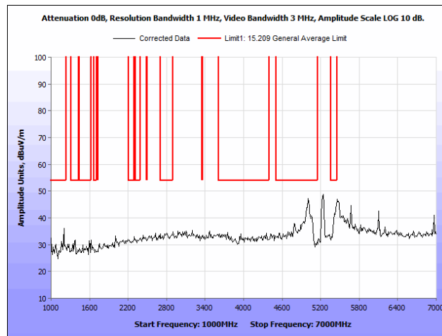
Plot 78. Radiated Spurious Emissions, 802.11a, 40 MHz, Low Channel, 1 GHz – 7 GHz, Average, Omni Antenna
