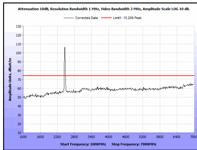
Plot 233. Radiated Spurs, Co-Location, 802.11n 20 MHz, 2462 MHz & 2462 MHz, 1 GHz – 7 GHz, Peak, Omni
