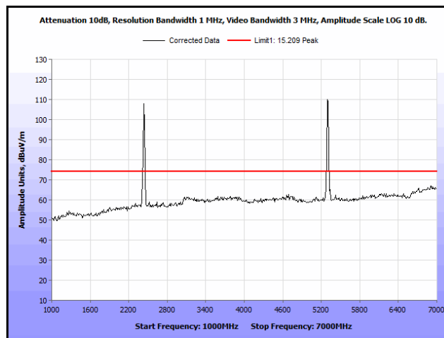
Plot 257. Radiated Spurs, Co-Location, 802.11n 20 MHz, 2437 MHz & 5300 MHz, 1 GHz – 7 GHz, Peak, Omni
