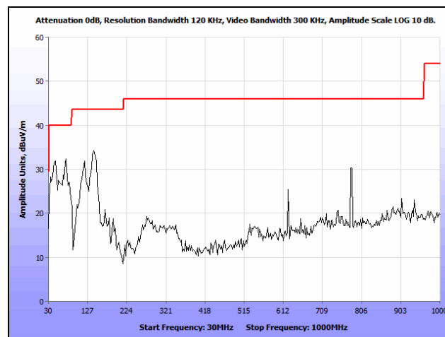
Plot 215. Radiated Spurious Emissions, 802.11a, High Channel, 30 MHz – 1 GHz, Patch, 5320 MHz
