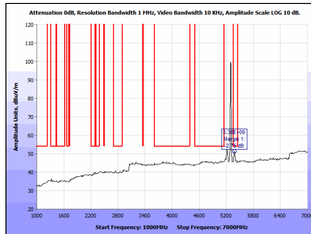
Plot 212. Radiated Spurious Emissions, 802.11a, Mid Channel, 1 GHz – 7 GHz, Avg., Patch, 5300 MHz
