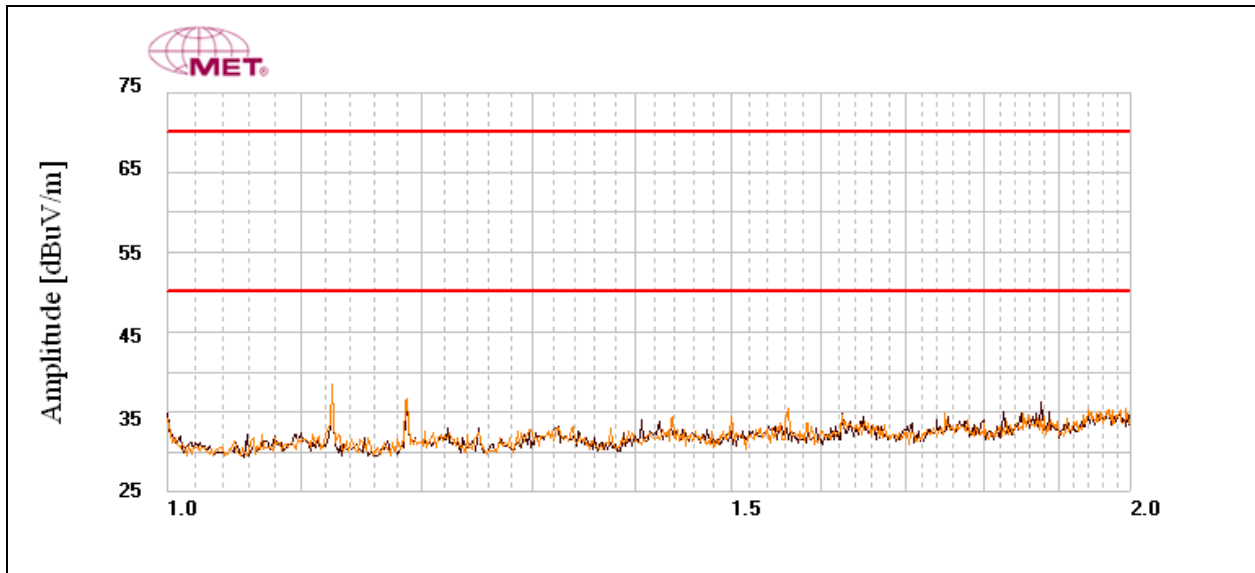
Plot 10. Radiated Emissions, ICES-003 Limits, Above 1 GHz
