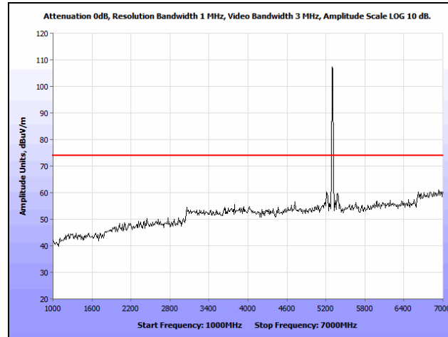
Plot 213. Radiated Spurious Emissions, 802.11a, Mid Channel, 1 GHz – 7 GHz, Peak, Patch, 5300 MHz
