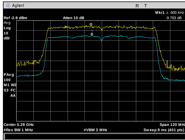
Plot 178. Peak Excursion Ratio, 802.11n 80 MHz, Port 2, 5290 MHz
