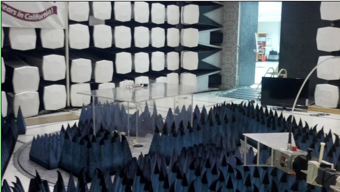
Photograph 8. Radiated Emissions, Test Setup, Above 1 GHz
