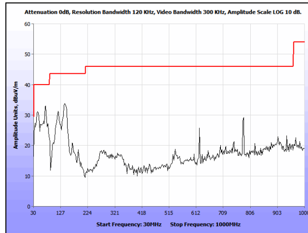
Plot 207. Radiated Spurious Emissions, 802.11a, Low Channel, 30 MHz – 1 GHz, Patch, 5260 MHz
