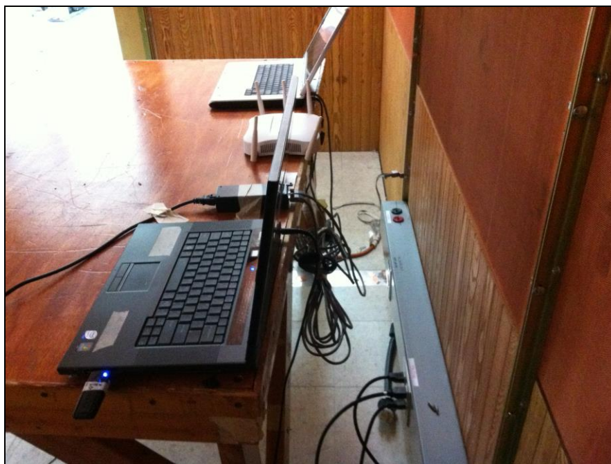
Photograph 5. Conducted Emissions, Test Setup, PoE, 2
