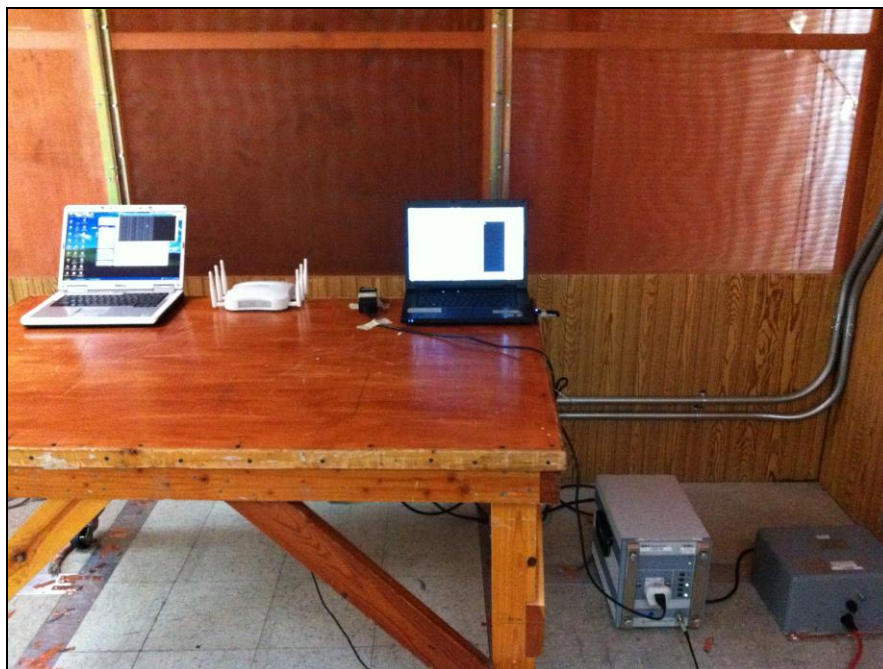
Photograph 4. Conducted Emissions, Test Setup, PoE, 1
