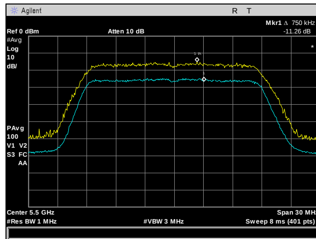
Plot 189. Peak Excursion Ratio, Low Channel, 802.11n 20 MHz, Port 3, 5500 MHz
