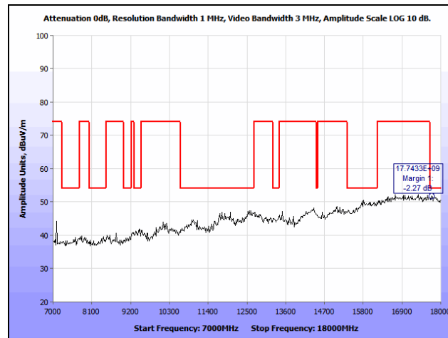
Plot 218. Radiated Spurious Emissions, 802.11a, High Channel, 7 GHz – 18 GHz, Patch, 5320 MHz
