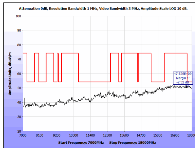
Plot 214. Radiated Spurious Emissions, 802.11a, Mid Channel, 7 GHz – 18 GHz, Patch, 5300 MHz
