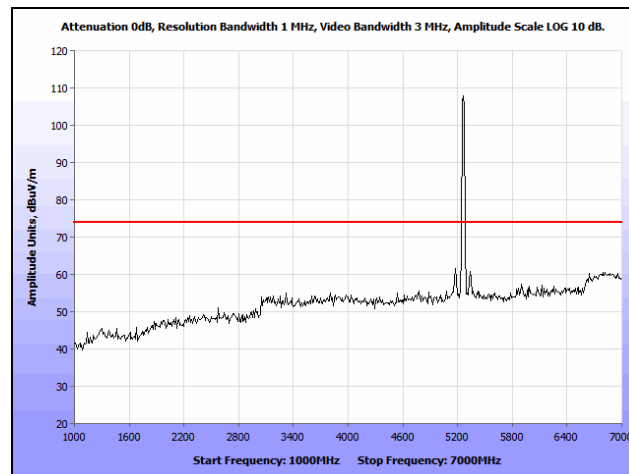
Plot 209. Radiated Spurious Emissions, 802.11a, Low Channel, 1 GHz – 7 GHz, Peak, Patch, 5260 MHz
