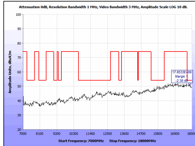
Plot 210. Radiated Spurious Emissions, 802.11a, Low Channel, 7 GHz – 18 GHz, Patch, 5260 MHz
