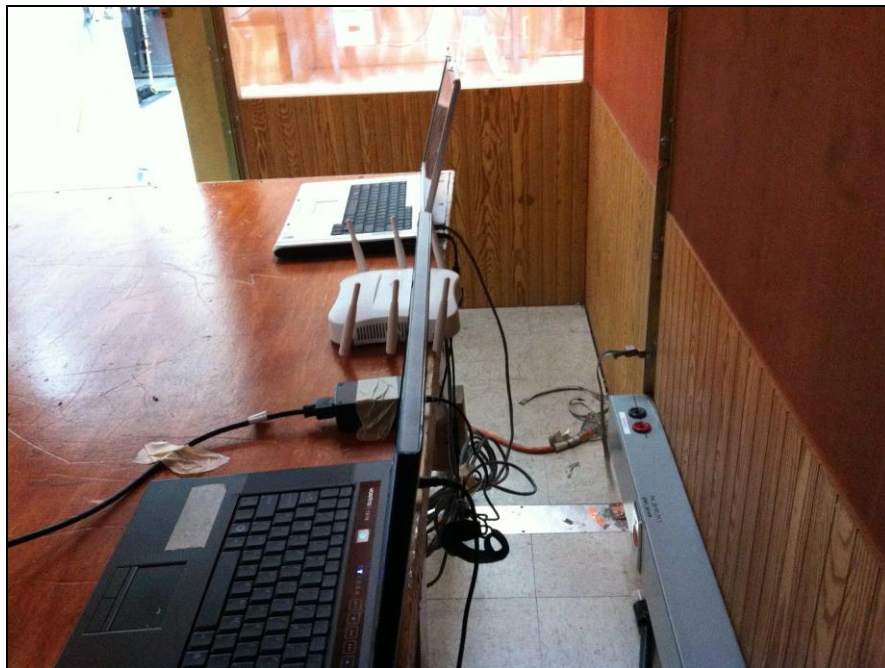
Photograph 3. Conducted Emissions, Test Setup, AC-DC Power Supply, 2
