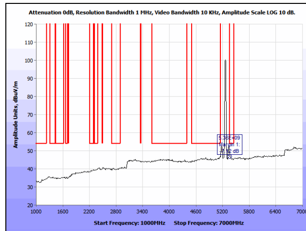
Plot 208. Radiated Spurious Emissions, 802.11a, Low Channel, 1 GHz – 7 GHz, Avg., Patch, 5260 MHz
