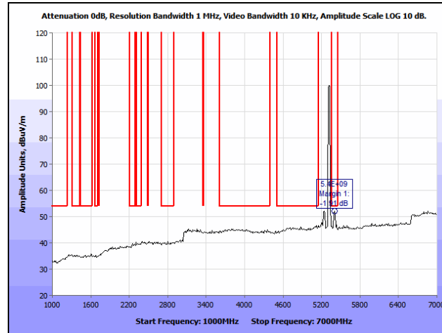
Plot 216. Radiated Spurious Emissions, 802.11a, High Channel, 1 GHz – 7 GHz, Avg., Patch, 5320 MHz
