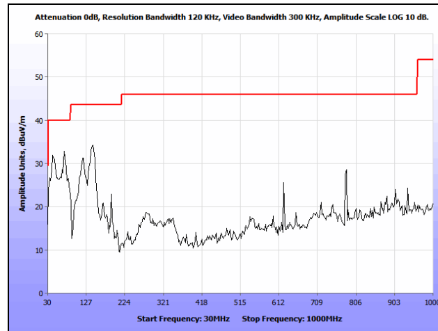
Plot 211. Radiated Spurious Emissions, 802.11a, Mid Channel, 30 MHz – 1 GHz, Patch, 5300 MHz
