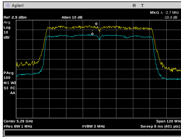
Plot 177. Peak Excursion Ratio, 802.11n 80 MHz, Port 1, 5290 MHz
