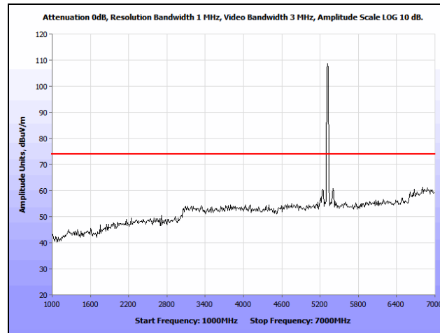
Plot 217. Radiated Spurious Emissions, 802.11a, High Channel, 1 GHz – 7 GHz, Peak, Patch, 5320 MHz
