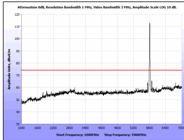
Plot 153. Radiated Spurious Emissions, 802.11n 20 MHz, High Channel, 1 GHz – 7 GHz, Peak, Ceiling
