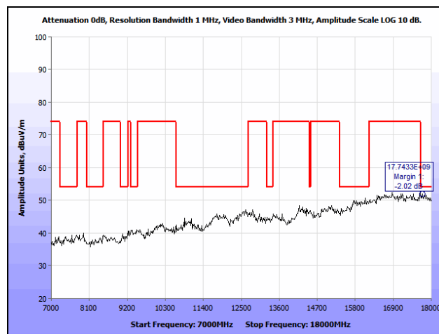
Plot 106. Radiated Spurious Emissions, 802.11a, High Channel, 7 GHz – 18 GHz, 7 dBi Patch
