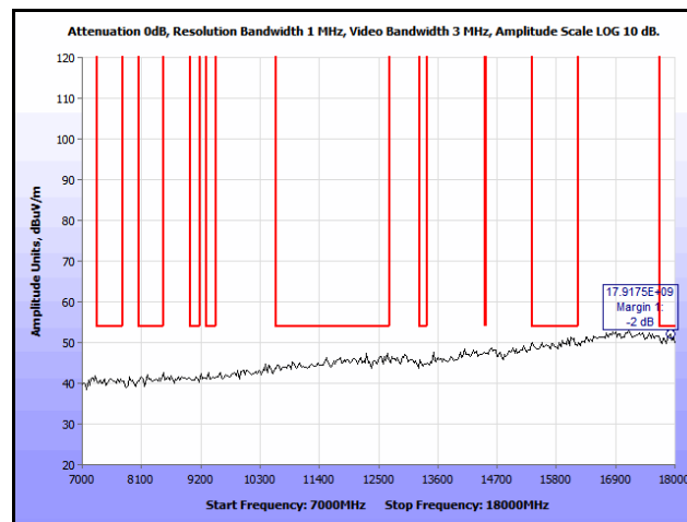
Plot 262. Co-location, Radiated Spurious Emissions, Patch, 802.11n 20 MHz, 2437 & 5785 MHz, 7 GHz – 18 GHz, Peak
