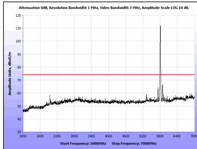
Plot 177. Radiated Spurious Emissions, 802.11a, High Channel, 1 GHz – 7 GHz, Peak, Omni
