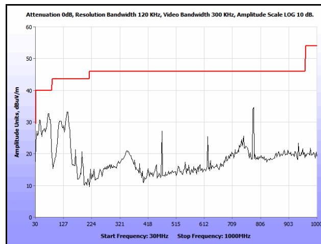
Plot 259. Co-location, Radiated Spurious Emissions, Patch, 802.11n 20 MHz, 2437 & 5785 MHz, 30 MHz – 1 GHz
