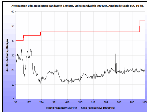
Plot 195. Radiated Spurious Emissions, 802.11n 40 MHz, High Channel, 30 MHz – 1 GHz, Omni
