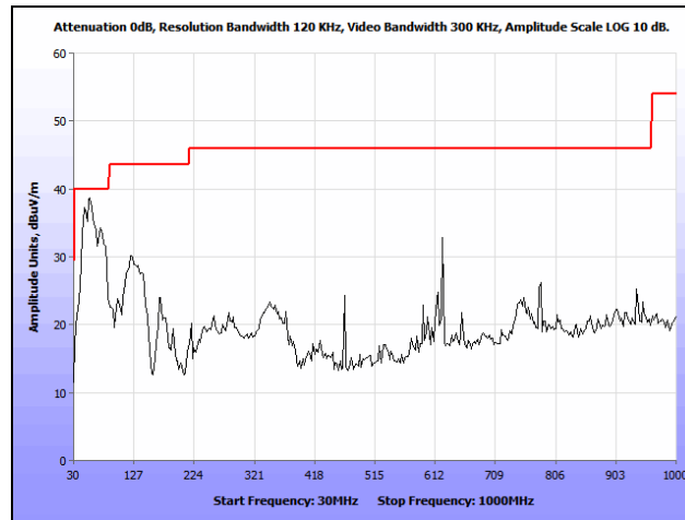
Plot 147. Radiated Spurious Emissions, 802.11n 20 MHz, Mid Channel, 30 MHz – 1 GHz, Ceiling
