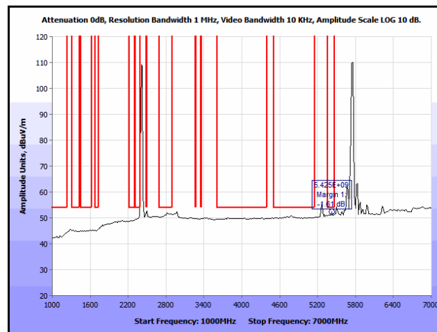
Plot 256. Co-location, Radiated Spurious Emissions, Patch, 802.11n 20 MHz, 2412 & 5785 MHz, 1 GHz – 7 GHz, Average
