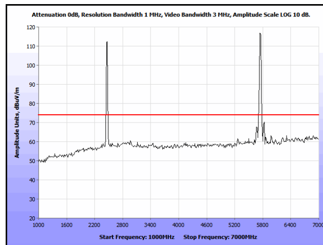
Plot 265. Co-location, Radiated Spurious Emissions, Patch, 802.11n 20 MHz, 2462 & 5785 MHz, 1 GHz – 7 GHz, Peak
