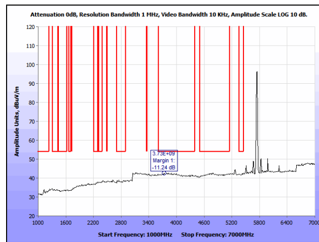
Plot 108. Radiated Spurious Emissions, 802.11n 20 MHz, Low Channel, 1 GHz – 7 GHz, Average, 7 dBi Patch
