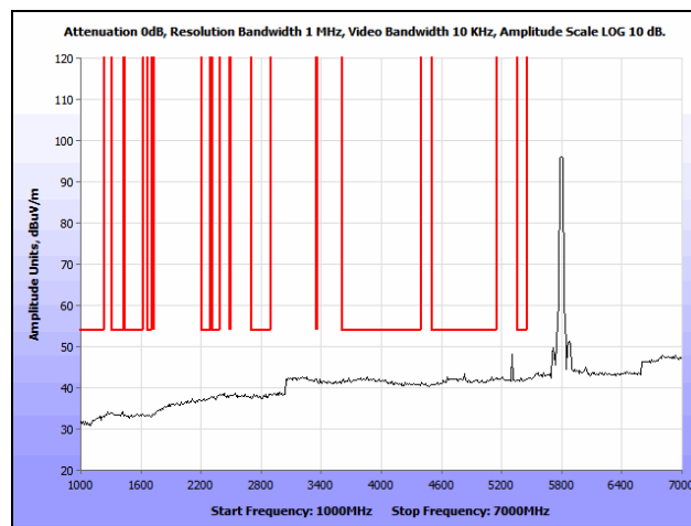
Plot 124. Radiated Spurious Emissions, 802.11n 40 MHz, High Channel, 1 GHz – 7 GHz, Average, 7 dBi Patch
