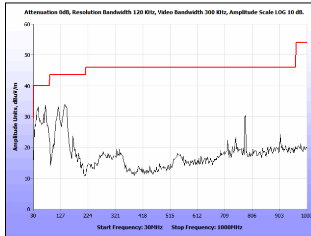
Plot 171. Radiated Spurious Emissions, 802.11a, Mid Channel, 30 MHz – 1 GHz, Omni
