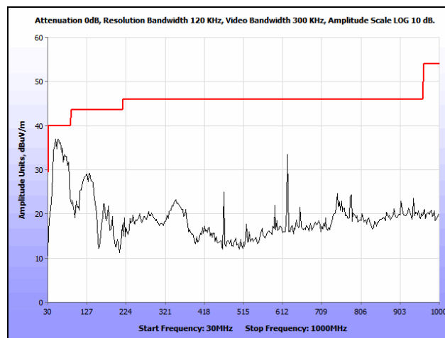
Plot 139. Radiated Spurious Emissions, 802.11a, High Channel, 30 MHz – 1 GHz, Ceiling
