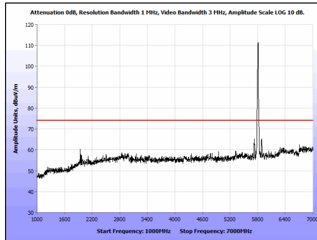
Plot 141. Radiated Spurious Emissions, 802.11a, High Channel, 1 GHz – 7 GHz, Peak, Ceiling
