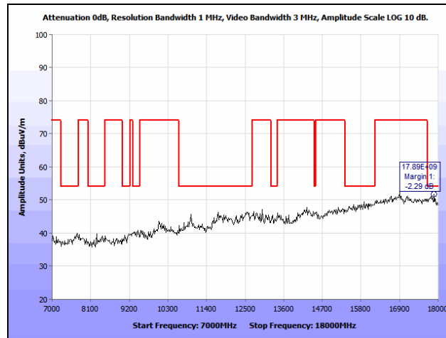
Plot 114. Radiated Spurious Emissions, 802.11n 20 MHz, Mid Channel, 7 GHz – 18 GHz, 7 dBi Patch
