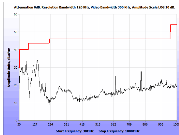
Plot 115. Radiated Spurious Emissions, 802.11n 20 MHz, High Channel, 30 MHz – 1 GHz, 7 dBi Patch
