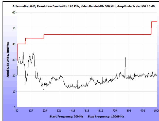
Plot 183. Radiated Spurious Emissions, 802.11n 20 MHz, Mid Channel, 30 MHz – 1 GHz, Omni
