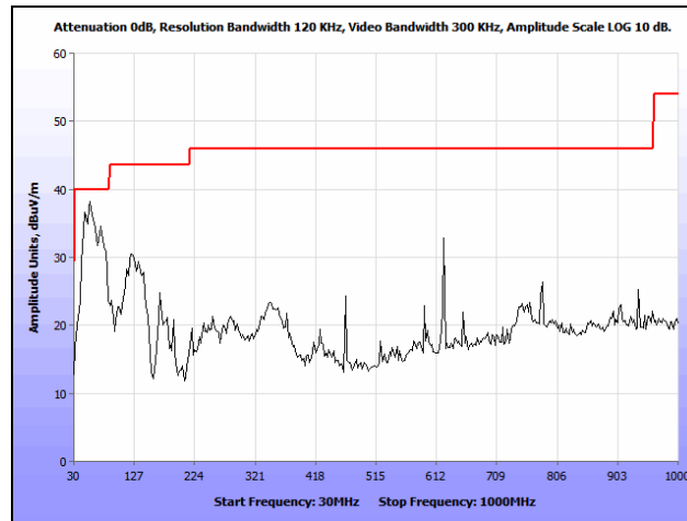
Plot 159. Radiated Spurious Emissions, 802.11n 40 MHz, High Channel, 30 MHz – 1 GHz, Ceiling
