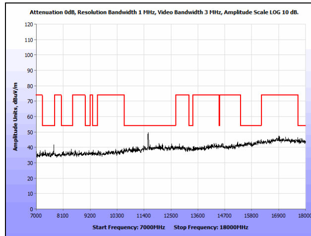
Plot 150. Radiated Spurious Emissions, 802.11n 20 MHz, Mid Channel, 7 GHz – 18 GHz, Ceiling
