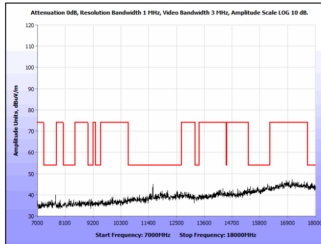
Plot 186. Radiated Spurious Emissions, 802.11n 20 MHz, Mid Channel, 7 GHz – 18 GHz, Omni
