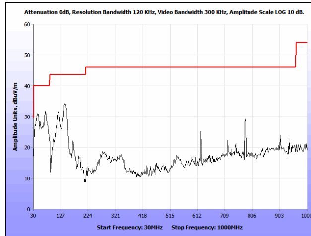
Plot 99. Radiated Spurious Emissions, 802.11a, Mid Channel, 30 MHz – 1 GHz, 7 dBi Patch
