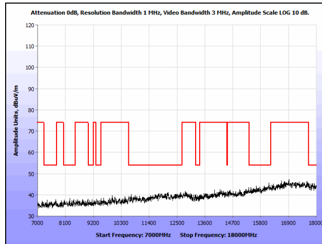
Plot 174. Radiated Spurious Emissions, 802.11a, Mid Channel, 7 GHz – 18 GHz, Omni
