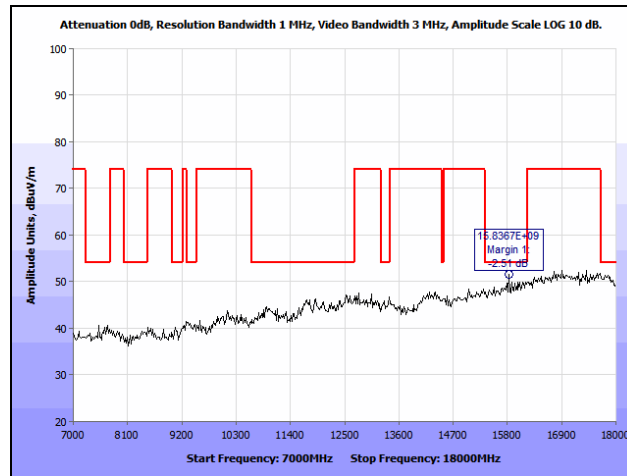
Plot 126. Radiated Spurious Emissions, 802.11n 40 MHz, High Channel, 7 GHz – 18 GHz, 7 dBi Patch
