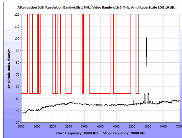
Plot 180. Radiated Spurious Emissions, 802.11n 20 MHz, Low Channel, 1 GHz – 7 GHz, Average, Omni
