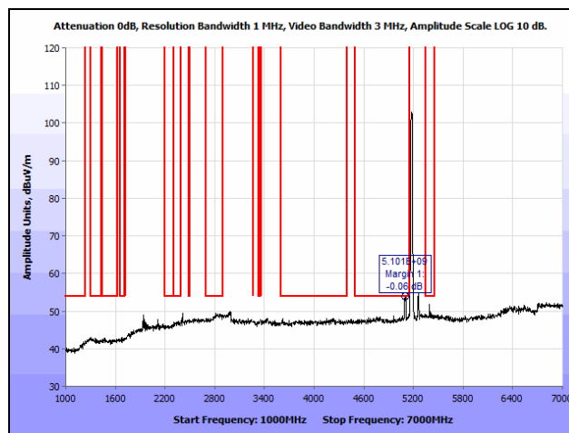
Plot 147. Radiated Spurious Emissions, 802.11n 20 MHz, Low Channel, 1 GHz – 7 GHz, Average, Ceiling
