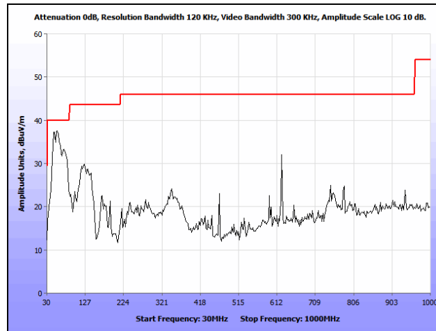
Plot 162. Radiated Spurious Emissions, 802.11n 40 MHz, High Channel, 30 MHz – 1 GHz, Ceiling
