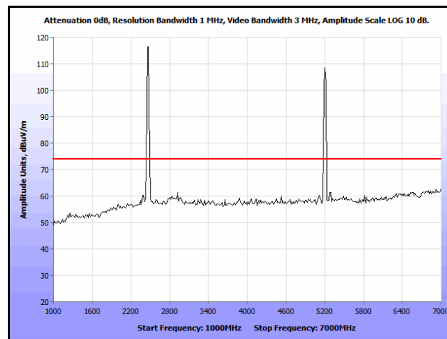
Plot 292. Co-location, Radiated Spurious Emissions, Patch, 802.11n 20 MHz, 2462 & 5200 MHz, 1 GHz – 7 GHz, Peak
