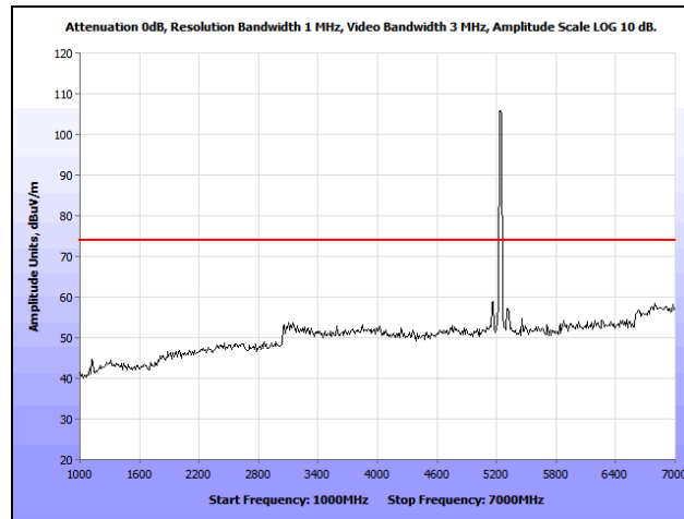
Plot 120. Radiated Spurious Emissions, 802.11n 20 MHz, High Channel, 1 GHz – 7 GHz, Peak, 7 dBi Patch
