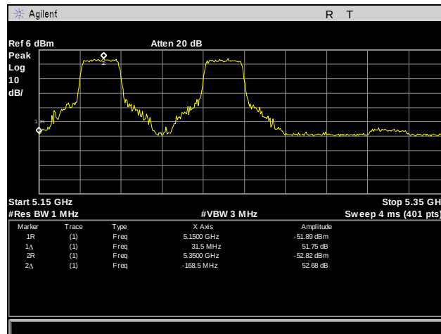
Plot 305. Frequency Stability, 5150 – 5250 MHz, 55°C, 120 V
