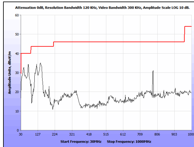
Plot 198. Radiated Spurious Emissions, 802.11n 40 MHz, High Channel, 30 MHz – 1 GHz, Omni
