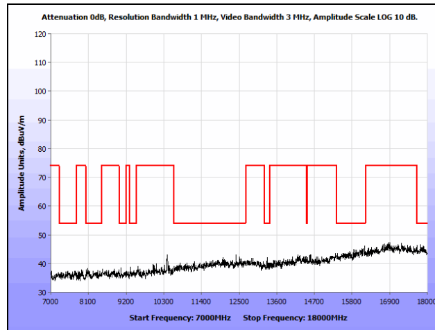
Plot 141. Radiated Spurious Emissions, 802.11a, Mid Channel, 7 GHz – 18 GHz, Ceiling
