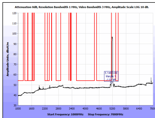
Plot 159. Radiated Spurious Emissions, 802.11n 40 MHz, Low Channel, 1 GHz – 7 GHz, Average, Ceiling
