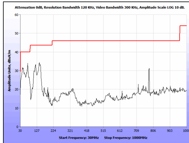
Plot 186. Radiated Spurious Emissions, 802.11n 20 MHz, Mid Channel, 30 MHz – 1 GHz, Omni
