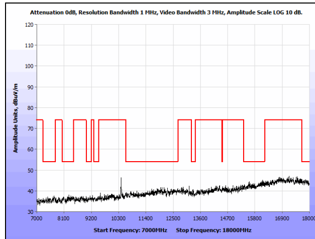
Plot 189. Radiated Spurious Emissions, 802.11n 20 MHz, Mid Channel, 7 GHz – 18 GHz, Omni
