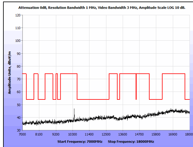
Plot 177. Radiated Spurious Emissions, 802.11a, Mid Channel, 7 GHz – 18 GHz, Omni
