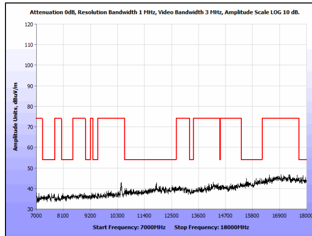
Plot 201. Radiated Spurious Emissions, 802.11n 40 MHz, High Channel, 7 GHz – 18 GHz, Omni
