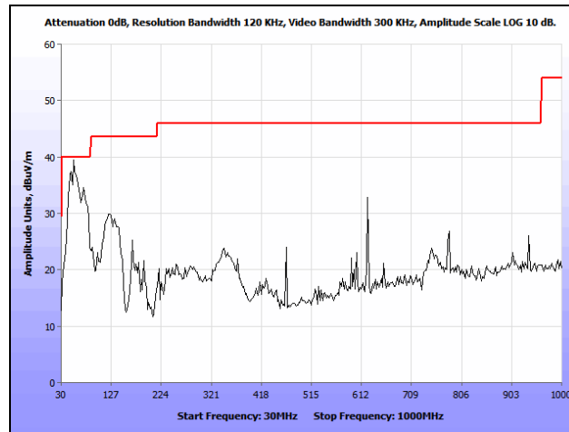
Plot 138. Radiated Spurious Emissions, 802.11a, Mid Channel, 30 MHz – 1 GHz, Ceiling
