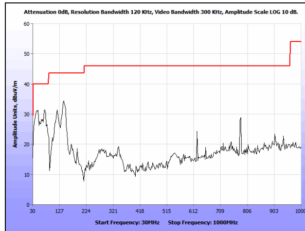
Plot 102. Radiated Spurious Emissions, 802.11a, Mid Channel, 30 MHz – 1 GHz, 7 dBi Patch
