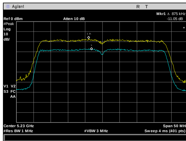
Plot 92. Peak Excursion Ratio, High Channel, 802.11n 40 MHz, Port 2
