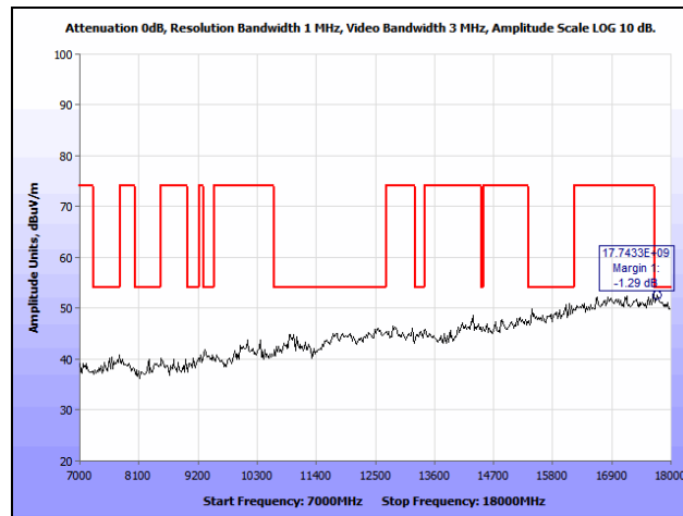
Plot 121. Radiated Spurious Emissions, 802.11n 20 MHz, High Channel, 7 GHz – 18 GHz, 7 dBi Patch
