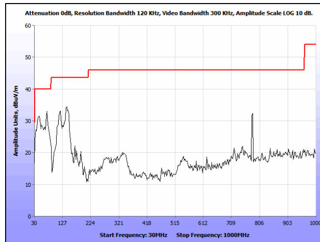
Plot 190. Radiated Spurious Emissions, 802.11n 20 MHz, High Channel, 30 MHz – 1 GHz, Omni
