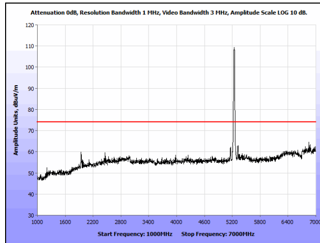
Plot 144. Radiated Spurious Emissions, 802.11a, High Channel, 1 GHz – 7 GHz, Peak, Ceiling
