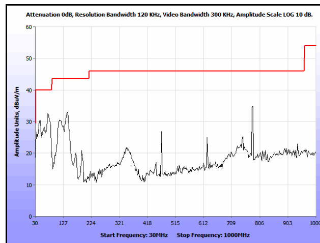
Plot 286. Co-location, Radiated Spurious Emissions, Patch, 802.11n 20 MHz, 2437 & 5200 MHz, 30 MHz – 1 GHz
