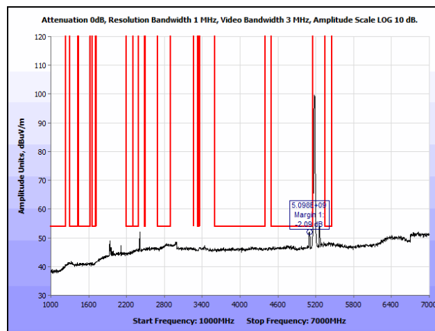
Plot 135. Radiated Spurious Emissions, 802.11a, Low Channel, 1 GHz – 7 GHz, Average, Ceiling
