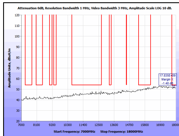
Plot 289. Co-location, Radiated Spurious Emissions, Patch, 802.11n 20 MHz, 2437 & 5200 MHz, 7 GHz – 18 GHz, Peak
