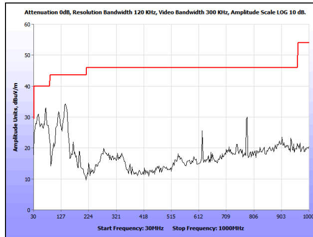
Plot 126. Radiated Spurious Emissions, 802.11n 40 MHz, High Channel, 30 MHz – 1 GHz, 7 dBi Patch
