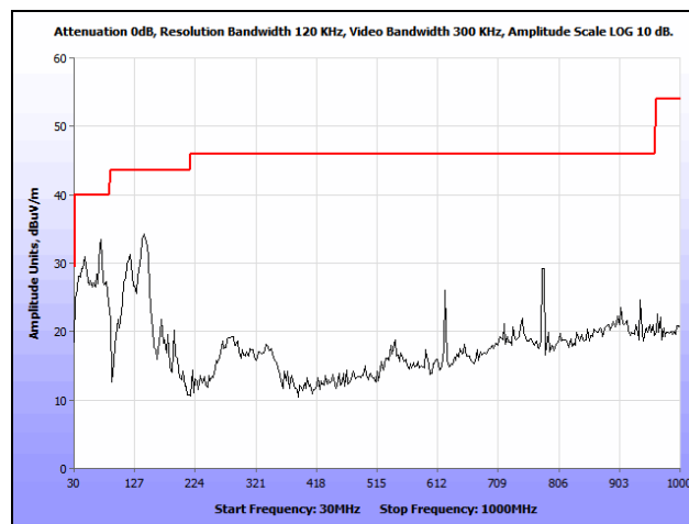
Plot 118. Radiated Spurious Emissions, 802.11n 20 MHz, High Channel, 30 MHz – 1 GHz, 7 dBi Patch
