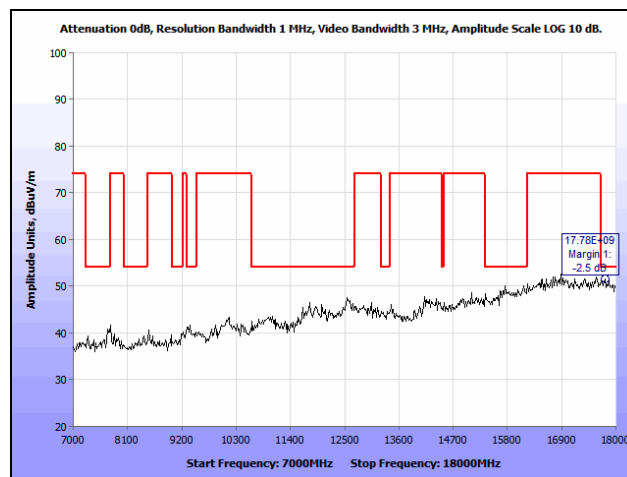
Plot 109. Radiated Spurious Emissions, 802.11a, High Channel, 7 GHz – 18 GHz, 7 dBi Patch
