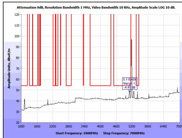
Plot 111. Radiated Spurious Emissions, 802.11n 20 MHz, Low Channel, 1 GHz – 7 GHz, Average, 7 dBi Patch
