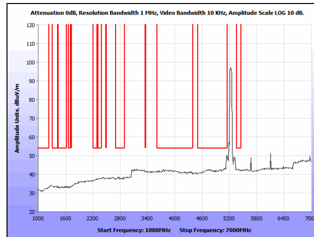
Plot 127. Radiated Spurious Emissions, 802.11n 40 MHz, High Channel, 1 GHz – 7 GHz, Average, 7 dBi Patch
