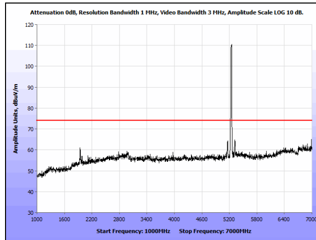
Plot 156. Radiated Spurious Emissions, 802.11n 20 MHz, High Channel, 1 GHz – 7 GHz, Peak, Ceiling
