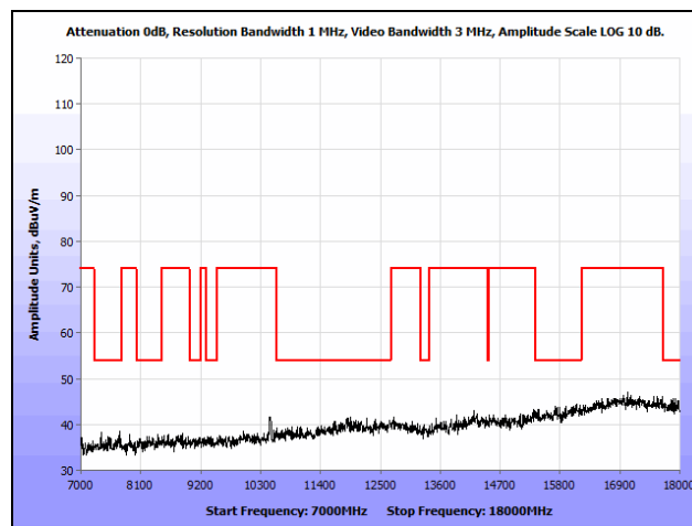
Plot 193. Radiated Spurious Emissions, 802.11n 20 MHz, High Channel, 7 GHz – 18 GHz, Omni
