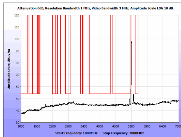
Plot 175. Radiated Spurious Emissions, 802.11a, Mid Channel, 1 GHz – 7 GHz, Average, Omni
