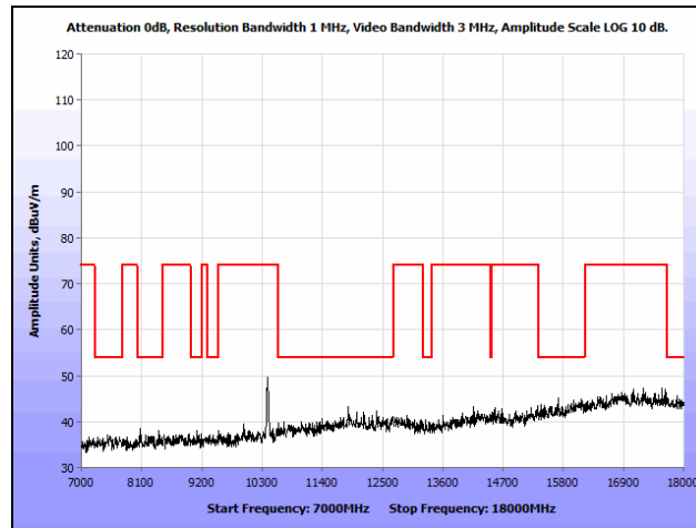
Plot 153. Radiated Spurious Emissions, 802.11n 20 MHz, Mid Channel, 7 GHz – 18 GHz, Ceiling
