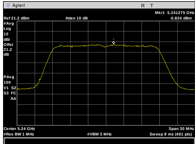
Plot 58. Power Spectral Density, High Channel, 802.11a
