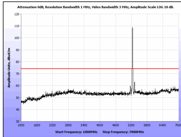
Plot 180. Radiated Spurious Emissions, 802.11a, High Channel, 1 GHz – 7 GHz, Peak, Omni
