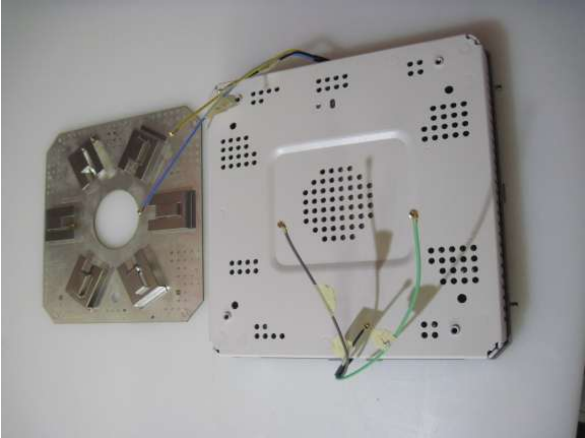
Photograph 1. Antenna Removed
