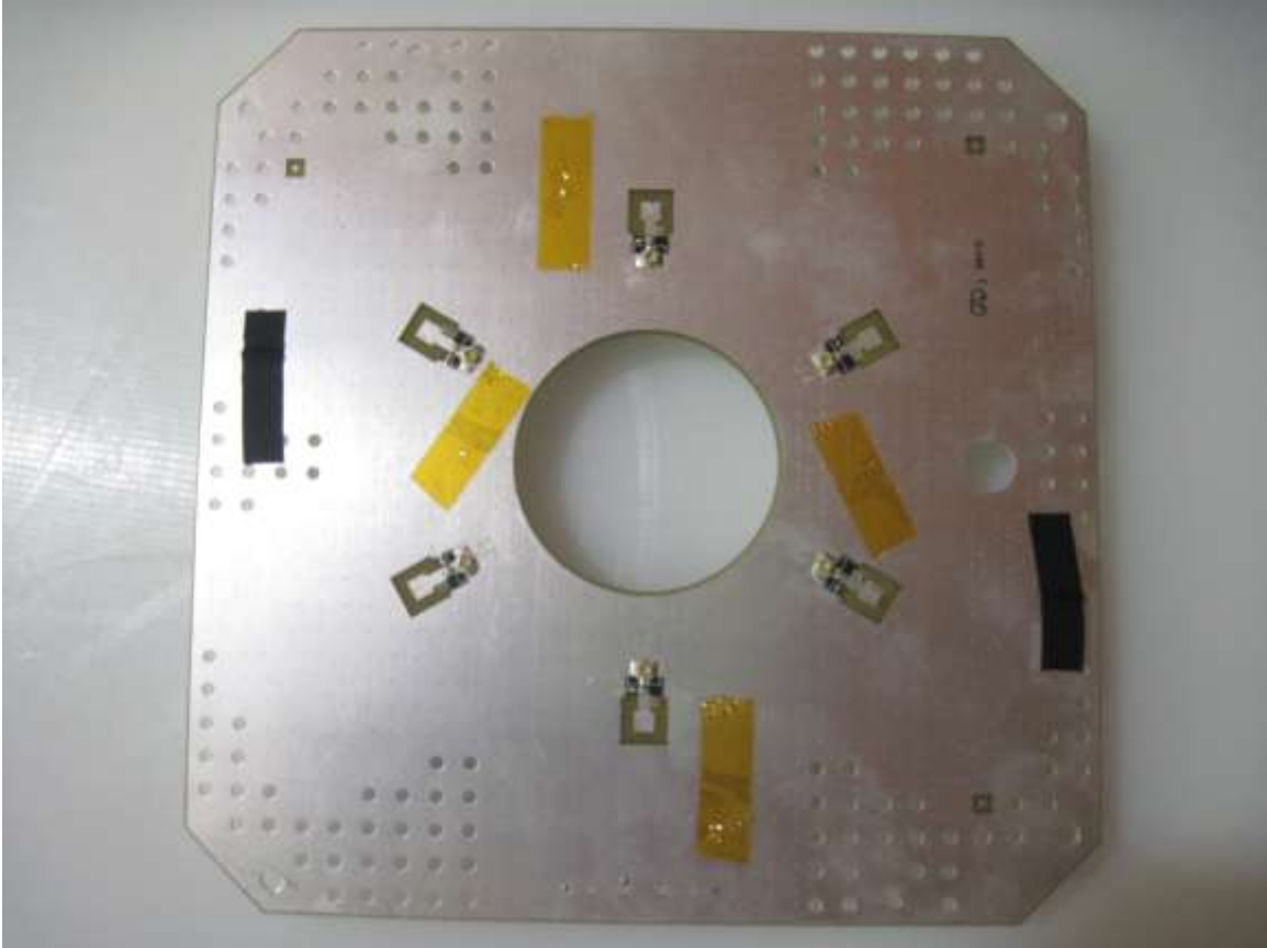
Photograph 11. PIFA Antenna Bottom
