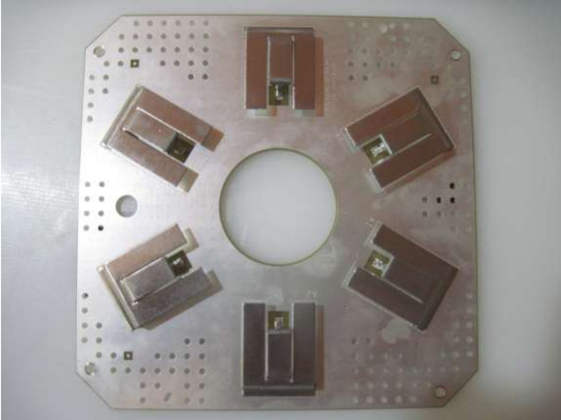
Photograph 12. PIFA Antenna Top
