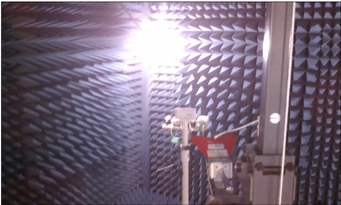
Photograph 12. Radiated Spurious Emissions, Test Setup, HF Ceiling Mount Antenna
