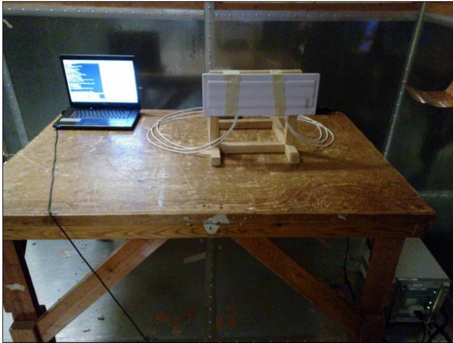
Photograph 3. Conducted Emissions, 15.207(a), Test Setup
