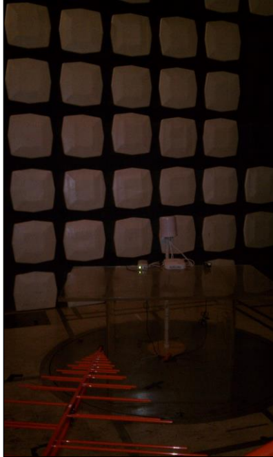
Photograph 9. Radiated Spurious Emissions, Test Setup, LF Dome Antenna
