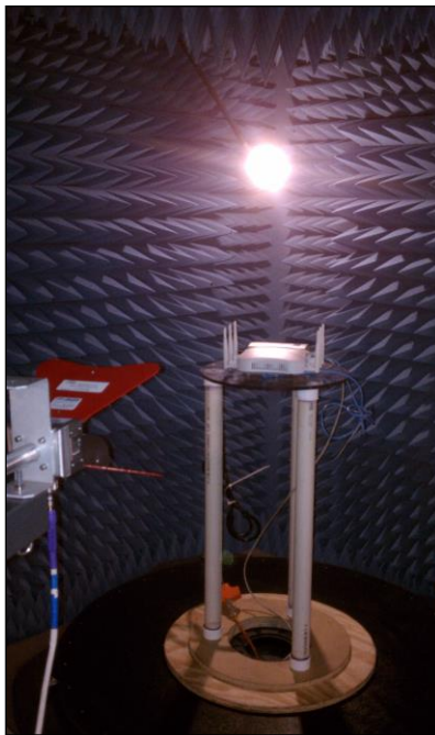
Photograph 6. Radiated Spurious Emissions, Test Setup, HF Dipole Antenna
