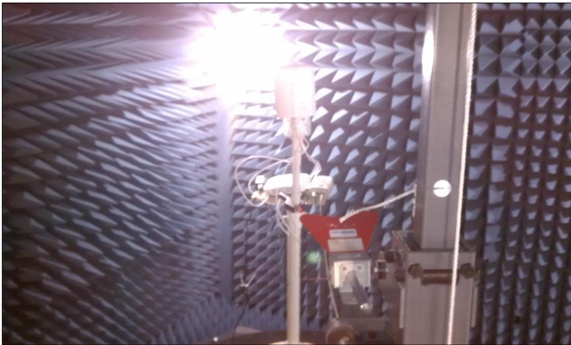
Photograph 10. Radiated Spurious Emissions, Test Setup, HF Dome Antenna
