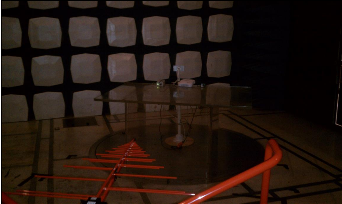
Photograph 11. Radiated Spurious Emissions, Test Setup, LF Ceiling Mount Antenna
