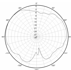
E-Plane Pattern
