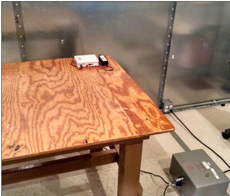
Photograph 2. Conducted Emissions, Test Setup, AC/DC
