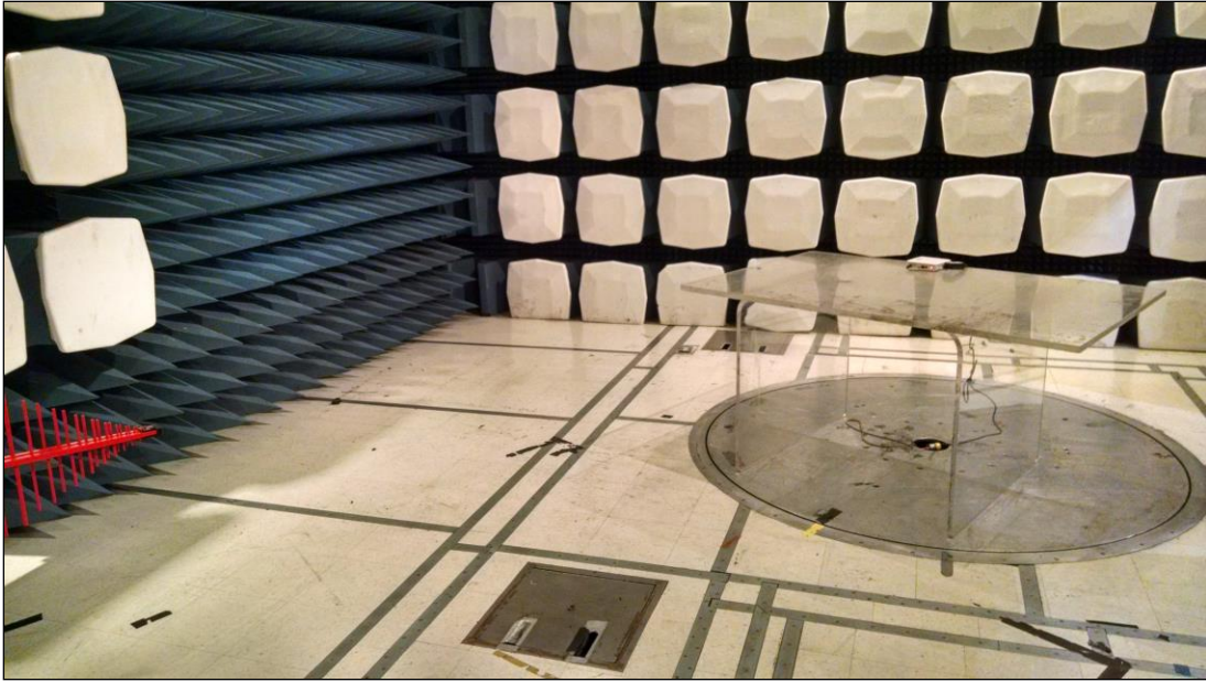
Photograph 3. Radiated Emissions, Test Setup, 30 MHz – 1 GHz
