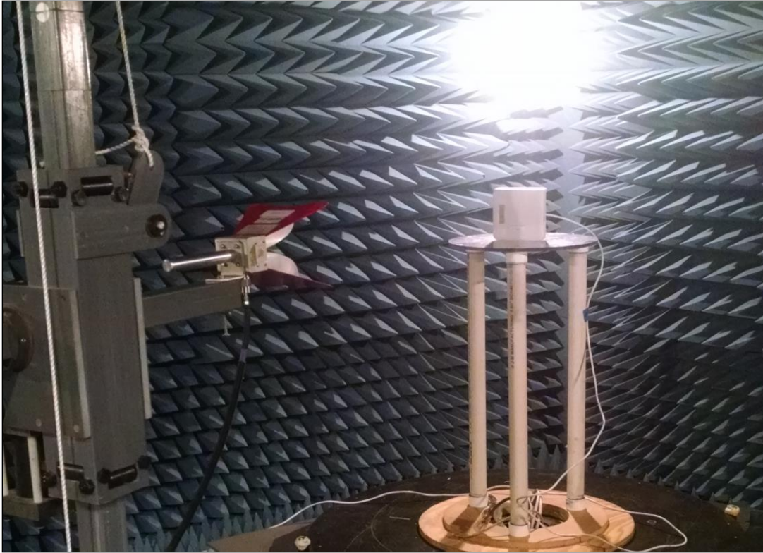
Photograph 5. Radiated Spurious Emissions, Test Setup, Above 1-18 GHz,
