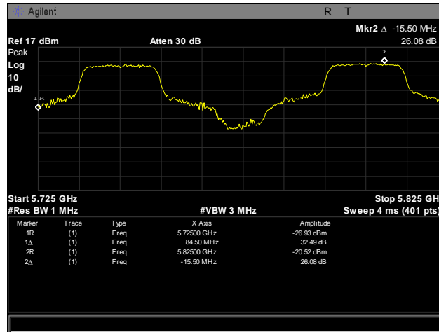
Plot 186. Frequency Stability, 5725 – 5825 MHz, 50°C, 120 V
