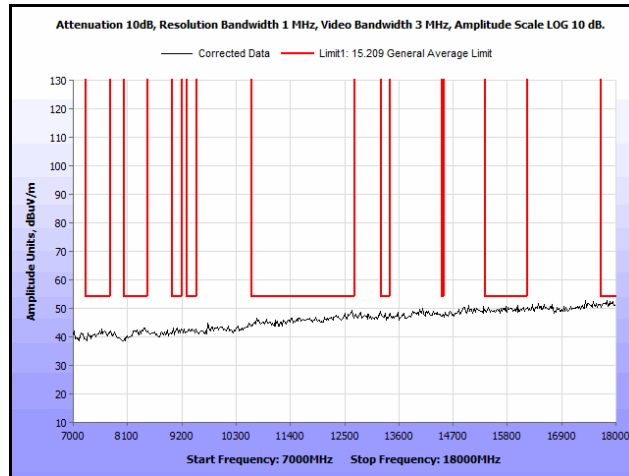
Plot 168. Radiated Spurs, Co-Location, 802.11n 20 MHz, 5580 MHz & 5580 MHz, 7 GHz – 18 GHz, Peak
