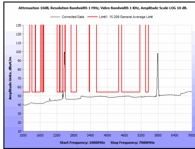
Plot 134. Radiated Spurs, Co-Location, 802.11n 20 MHz, 2462 MHz & 5785 MHz, 1 GHz – 7 GHz, Avg.
