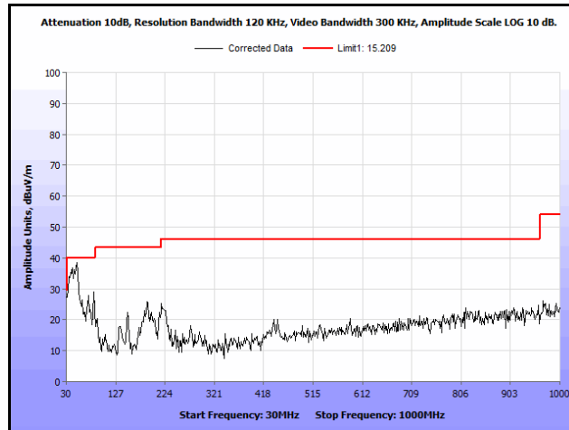
Plot 141. Radiated Spurs, Co-Location, 802.11n 20 MHz, 5200 MHz & 5300 MHz, 30 MHz – 1 GHz, Peak
