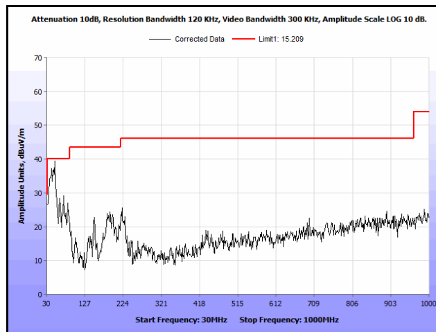
Plot 97. Radiated Spurs, Co-Location, 802.11n 20 MHz, 2412 MHz & 5580 MHz, 30 MHz – 1 GHz, Peak
