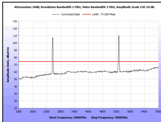
Plot 127. Radiated Spurs, Co-Location, 802.11n 20 MHz, 2462 MHz & 5300 MHz, 1 GHz – 7 GHz, Peak
