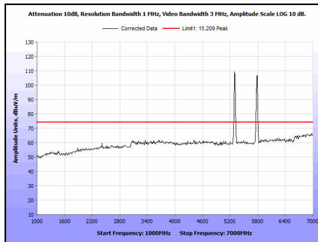
Plot 163. Radiated Spurs, Co-Location, 802.11n 20 MHz, 5300 MHz & 5785 MHz, 1 GHz – 7 GHz, Peak
