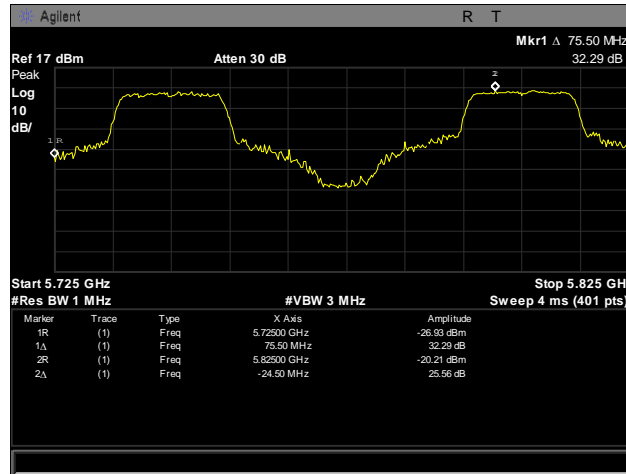
Plot 183. Frequency Stability, 5725 – 5825 MHz, 20°C, 120 V
