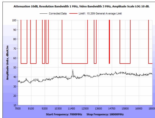
Plot 37. Radiated Spurious Emissions, 802.11a 40 MHz, Low Channel, 7 GHz – 18 GHz
