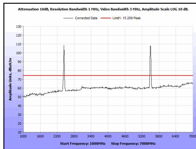
Plot 115. Radiated Spurs, Co-Location, 802.11n 20 MHz, 2437 MHz & 5580 MHz, 1 GHz – 7 GHz, Peak
