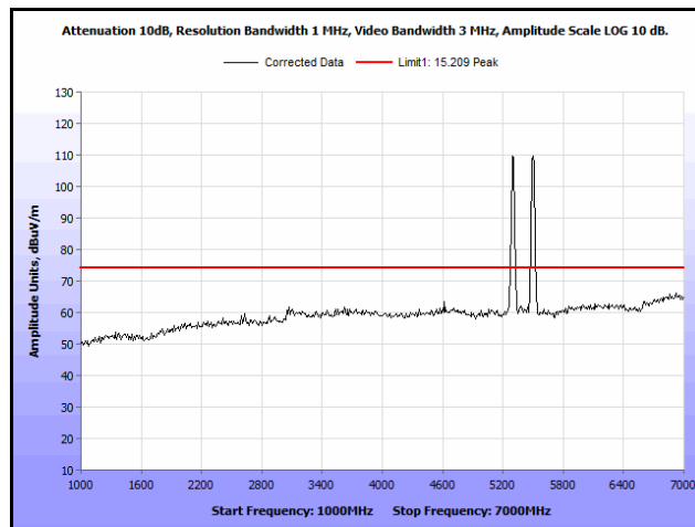
Plot 159. Radiated Spurs, Co-Location, 802.11n 20 MHz, 5300 MHz & 5580 MHz, 1 GHz – 7 GHz, Peak
