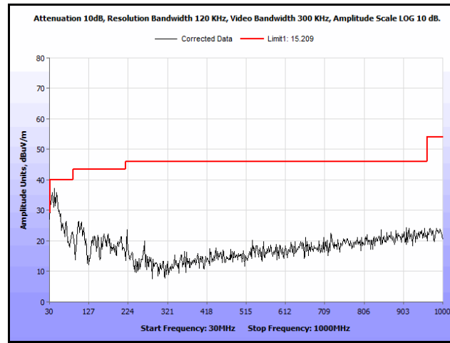
Plot 113. Radiated Spurs, Co-Location, 802.11n 20 MHz, 2437 MHz & 5580 MHz, 30 MHz – 1 GHz, Peak
