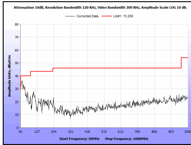
Plot 137. Radiated Spurs, Co-Location, 802.11n 20 MHz, 5200 MHz & 5200 MHz, 30 MHz – 1 GHz, Peak
