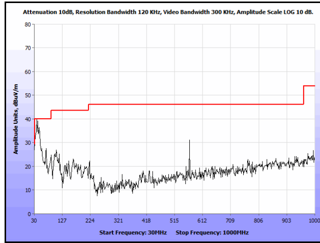
Plot 173. Radiated Spurs, Co-Location, 802.11n 20 MHz, 5785 MHz & 5785 MHz, 30 MHz – 1 GHz, Peak
