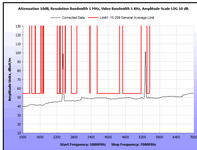
Plot 94. Radiated Spurs, Co-Location, 802.11n 20 MHz, 2412 MHz & 5300 MHz, 1 GHz – 7 GHz, Avg.
