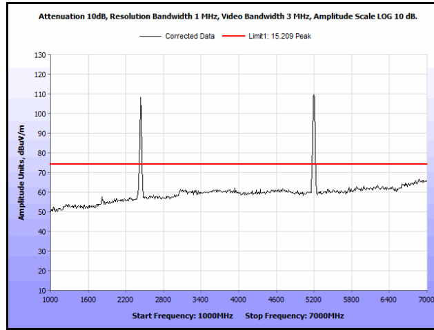
Plot 107. Radiated Spurs, Co-Location, 802.11n 20 MHz, 2437 MHz & 5200 MHz, 1 GHz – 7 GHz, Peak
