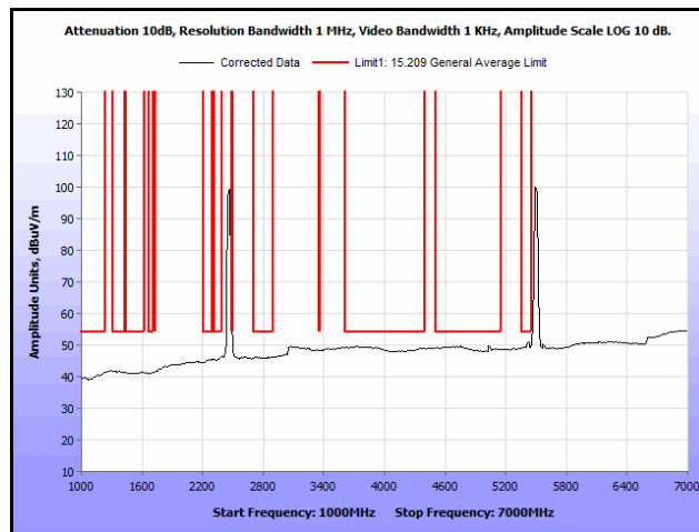
Plot 130. Radiated Spurs, Co-Location, 802.11n 20 MHz, 2462 MHz & 5580 MHz, 1 GHz – 7 GHz, Avg.
