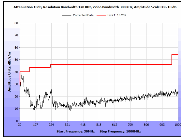
Plot 89. Radiated Spurs, Co-Location, 802.11n 20 MHz, 2412 MHz & 5200 MHz, 30 MHz – 1 GHz, Peak, Omni
