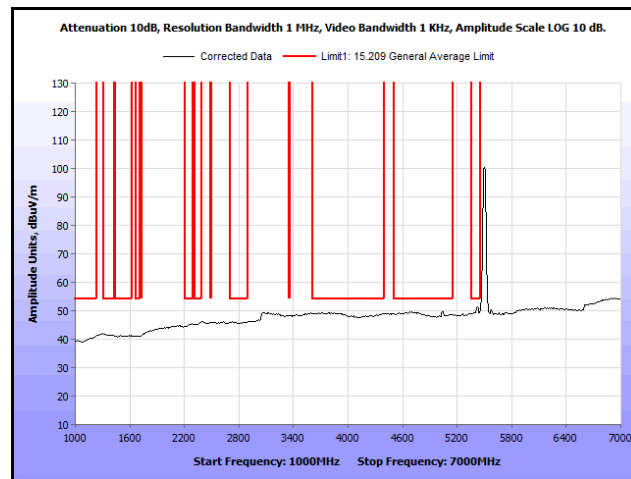
Plot 166. Radiated Spurs, Co-Location, 802.11n 20 MHz, 5580 MHz & 5580 MHz, 1 GHz – 7 GHz, Avg.
