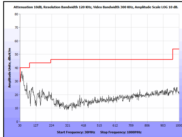
Plot 165. Radiated Spurs, Co-Location, 802.11n 20 MHz, 5580 MHz & 5580 MHz, 30 MHz – 1 GHz, Peak
