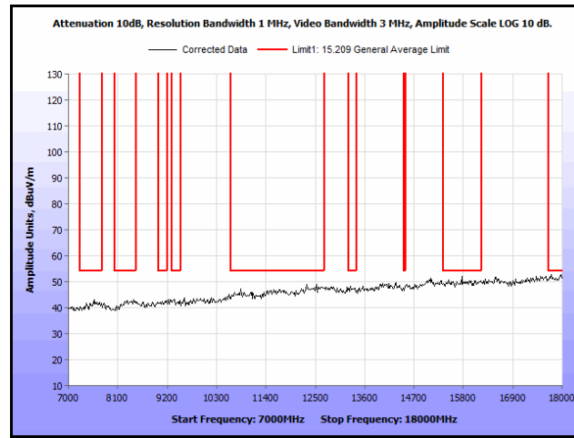
Plot 164. Radiated Spurs, Co-Location, 802.11n 20 MHz, 5300 MHz & 5785 MHz, 7 GHz – 18 GHz, Peak
