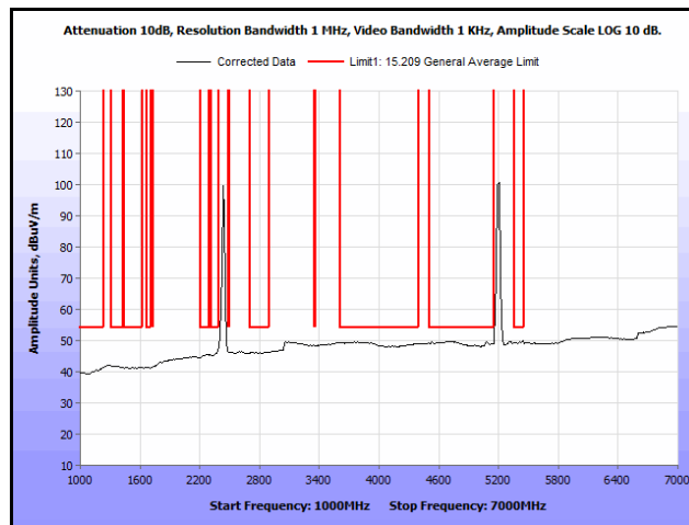
Plot 106. Radiated Spurs, Co-Location, 802.11n 20 MHz, 2437 MHz & 5200 MHz, 1 GHz – 7 GHz, Avg.
