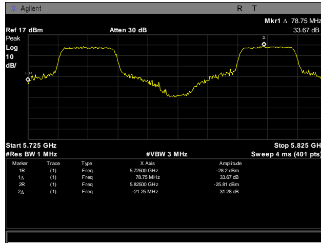
Plot 180. Frequency Stability, 5725 – 5825 MHz, -10°C, 120 V
