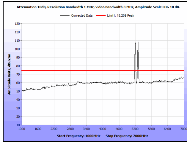
Plot 143. Radiated Spurs, Co-Location, 802.11n 20 MHz, 5200 MHz & 5300 MHz, 1 GHz – 7 GHz, Peak
