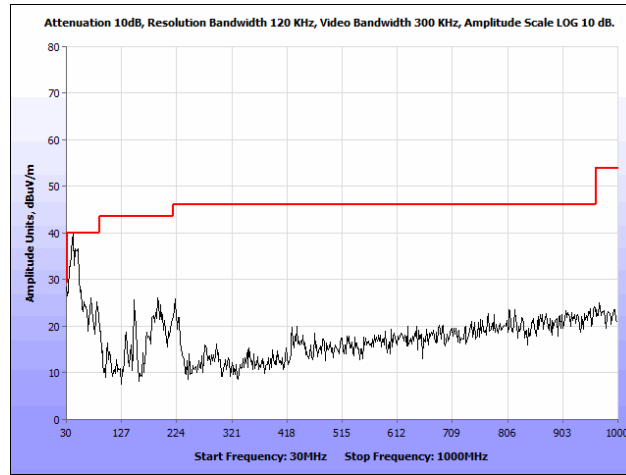
Plot 69. Radiated Spurious Emissions, 802.11ac 80 MHz, 30 MHz – 1 GHz
