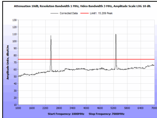
Plot 111. Radiated Spurs, Co-Location, 802.11n 20 MHz, 2437 MHz & 5300 MHz, 1 GHz – 7 GHz, Peak
