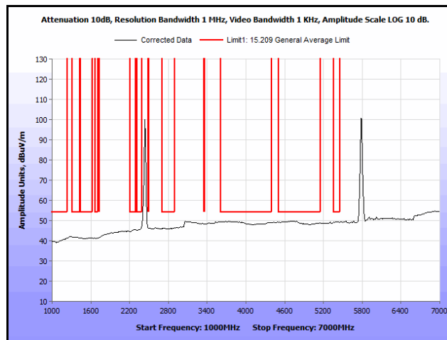
Plot 118. Radiated Spurs, Co-Location, 802.11n 20 MHz, 2437 MHz & 5785 MHz, 1 GHz – 7 GHz, Avg.
