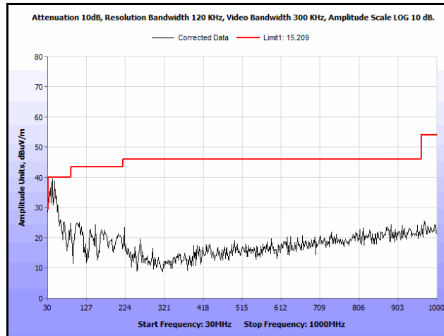
Plot 129. Radiated Spurs, Co-Location, 802.11n 20 MHz, 2462 MHz & 5580 MHz, 30 MHz – 1 GHz, Peak
