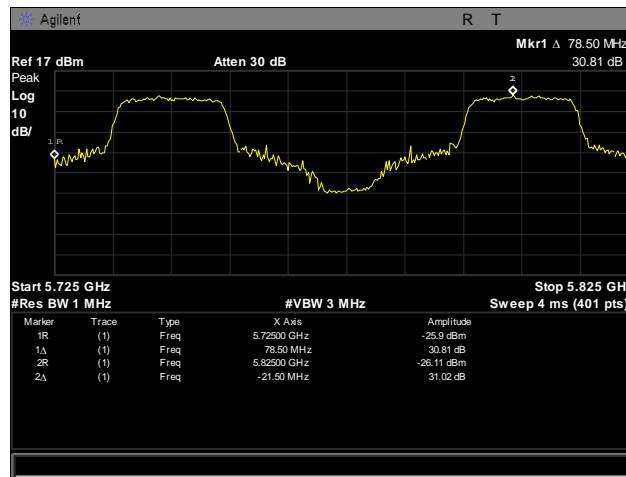
Plot 181. Frequency Stability, 5725 – 5825 MHz, 0°C, 120 V
