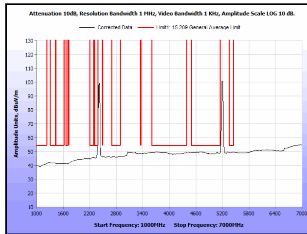
Plot 90. Radiated Spurs, Co-Location, 802.11n 20 MHz, 2412 MHz & 5200 MHz, 1 GHz – 7 GHz, Avg.
