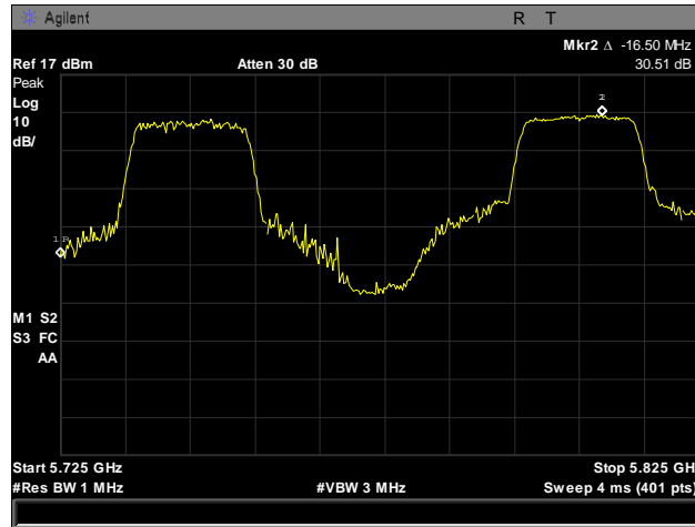
Plot 177. Frequency Stability, 5725 – 5825 MHz, -40°C, 120 V
