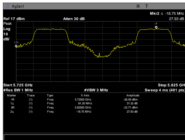
Plot 185. Frequency Stability, 5725 – 5825 MHz, 40°C, 120 V
