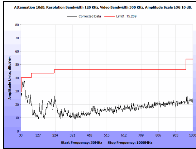
Plot 101. Radiated Spurs, Co-Location, 802.11n 20 MHz, 2412 MHz & 5785 MHz, 30 MHz – 1 GHz, Peak
