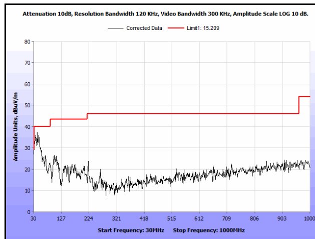
Plot 169. Radiated Spurs, Co-Location, 802.11n 20 MHz, 5580 MHz & 5785 MHz, 30 MHz – 1 GHz, Peak
