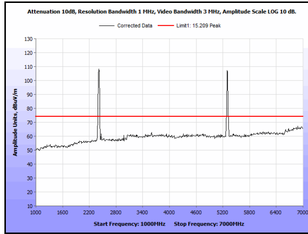
Plot 95. Radiated Spurs, Co-Location, 802.11n 20 MHz, 2412 MHz & 5300 MHz, 1 GHz – 7 GHz, Peak
