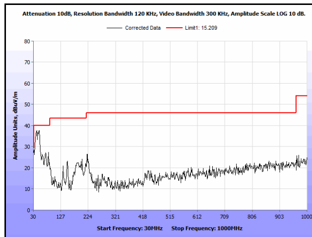
Plot 157. Radiated Spurs, Co-Location, 802.11n 20 MHz, 5300 MHz & 5580 MHz, 30 MHz – 1 GHz, Peak
