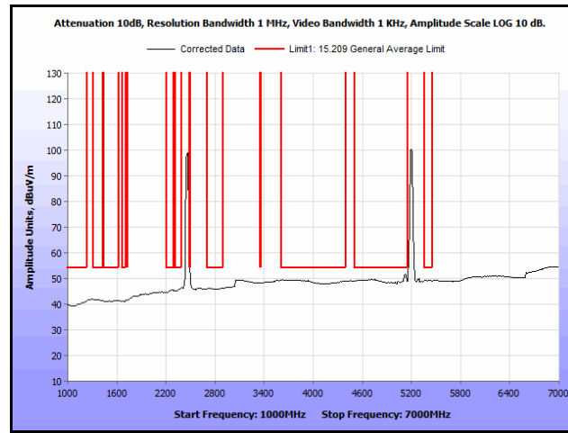
Plot 122. Radiated Spurs, Co-Location, 802.11n 20 MHz, 2462 MHz & 5200 MHz, 1 GHz – 7 GHz, Avg.
