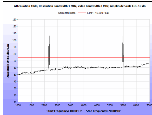
Plot 135. Radiated Spurs, Co-Location, 802.11n 20 MHz, 2462 MHz & 5785 MHz, 1 GHz – 7 GHz, Peak
