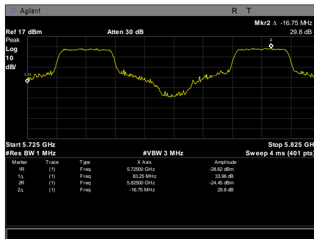
Plot 184. Frequency Stability, 5725 – 5825 MHz, 30°C, 120 V
