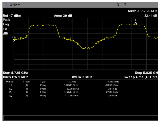
Plot 187. Frequency Stability, 5725 – 5825 MHz, 55°C, 120 V
