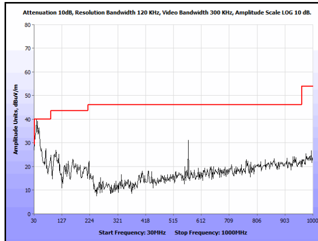
Plot 117. Radiated Spurs, Co-Location, 802.11n 20 MHz, 2437 MHz & 5785 MHz, 30 MHz – 1 GHz, Peak
