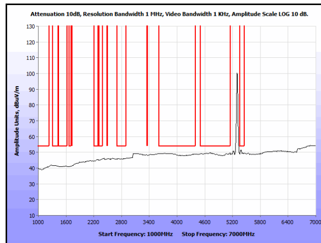
Plot 154. Radiated Spurs, Co-Location, 802.11n 20 MHz, 5300 MHz & 5300 MHz, 1 GHz – 7 GHz, Avg.
