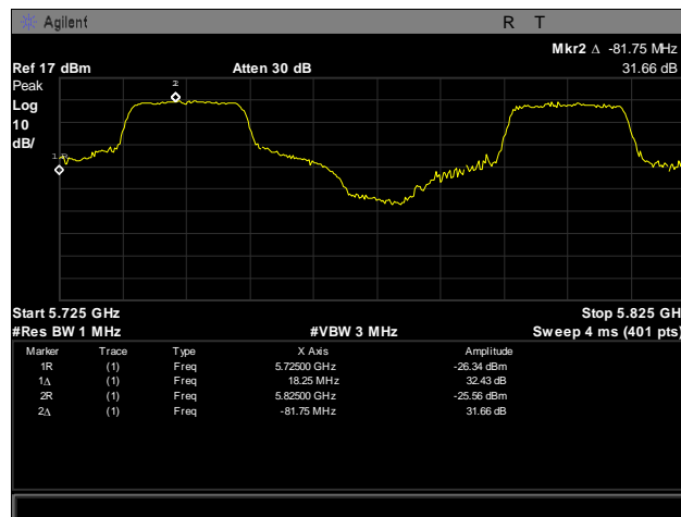
Plot 178. Frequency Stability, 5725 – 5825 MHz, -30°C, 120 V
