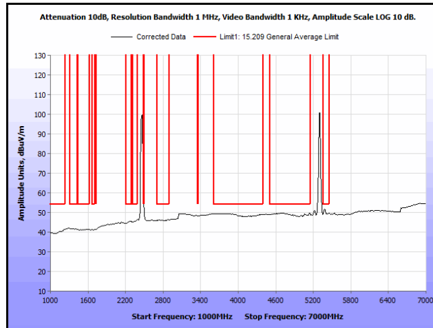
Plot 126. Radiated Spurs, Co-Location, 802.11n 20 MHz, 2462 MHz & 5300 MHz, 1 GHz – 7 GHz, Avg.
