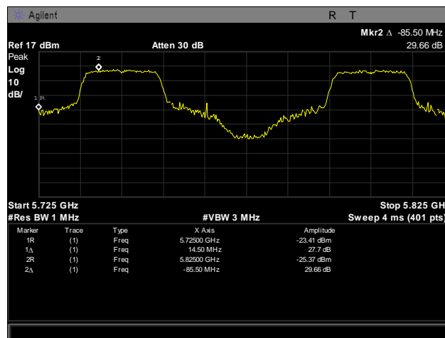
Plot 182. Frequency Stability, 5725 – 5825 MHz, 10°C, 120 V
