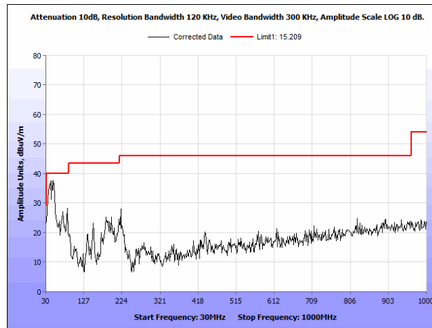
Plot 45. Radiated Spurious Emissions, 802.11a 40 MHz, High Channel, 30 MHz – 1 GHz
