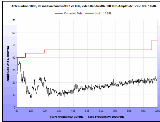
Plot 149. Radiated Spurs, Co-Location, 802.11n 20 MHz, 5200 MHz & 5785 MHz, 30 MHz – 1 GHz, Peak
