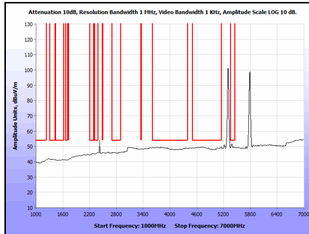
Plot 162. Radiated Spurs, Co-Location, 802.11n 20 MHz, 5300 MHz & 5785 MHz, 1 GHz – 7 GHz, Avg.
