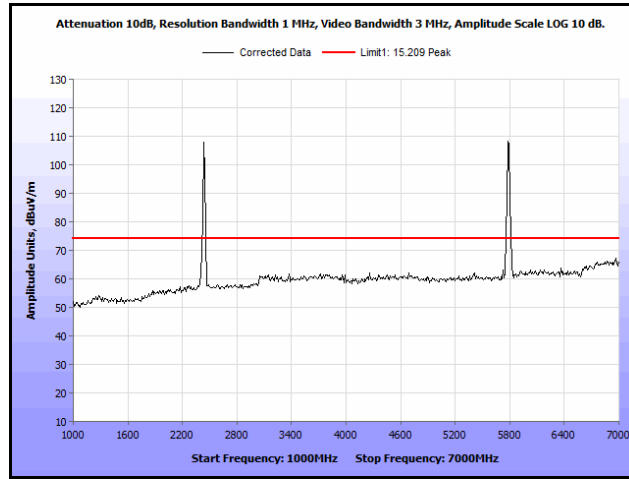
Plot 119. Radiated Spurs, Co-Location, 802.11n 20 MHz, 2437 MHz & 5785 MHz, 1 GHz – 7 GHz, Peak
