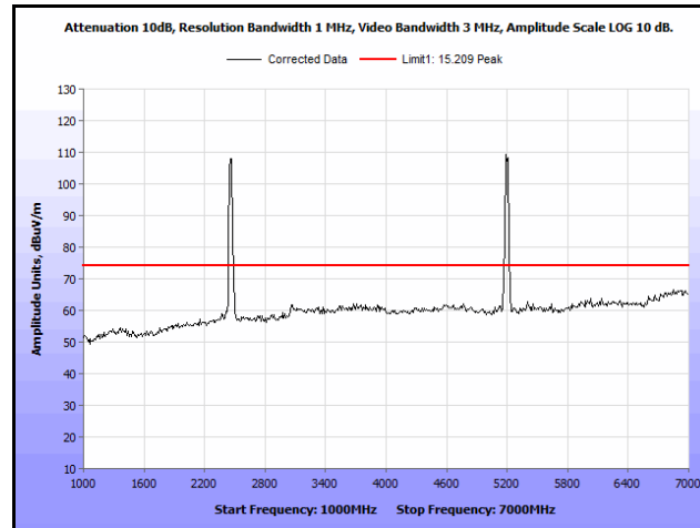
Plot 123. Radiated Spurs, Co-Location, 802.11n 20 MHz, 2462 MHz & 5200 MHz, 1 GHz – 7 GHz, Peak
