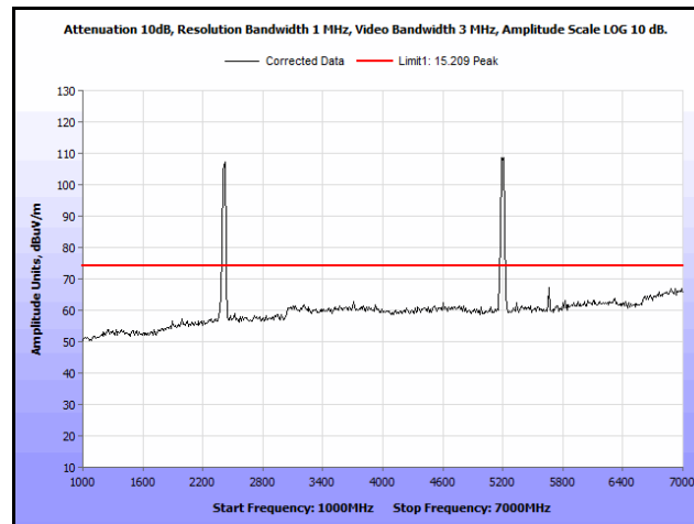
Plot 91. Radiated Spurs, Co-Location, 802.11n 20 MHz, 2412 MHz & 5200 MHz, 1 GHz – 7 GHz, Peak
