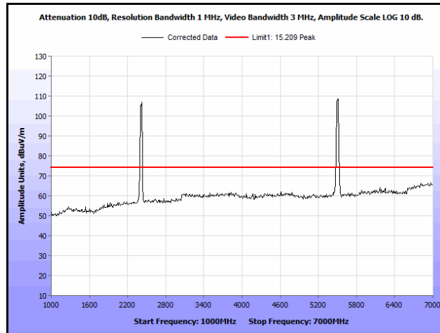
Plot 99. Radiated Spurs, Co-Location, 802.11n 20 MHz, 2412 MHz & 5580 MHz, 1 GHz – 7 GHz, Peak
