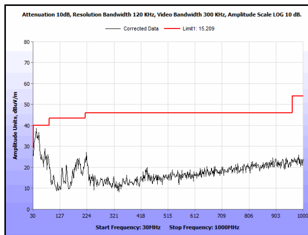
Plot 229. Radiated Spurs, Co-Location, 802.11n 20 MHz, 5200 MHz & 5580 MHz, 30 MHz – 1 GHz, Peak
