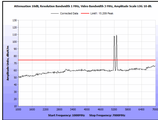
Plot 227. Radiated Spurs, Co-Location, 802.11n 20 MHz, 5200 MHz & 5300 MHz, 1 GHz – 7 GHz, Peak
