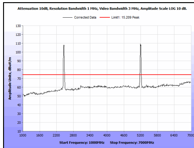
Plot 207. Radiated Spurs, Co-Location, 802.11n 20 MHz, 2462 MHz & 5200 MHz, 1 GHz – 7 GHz, Peak
