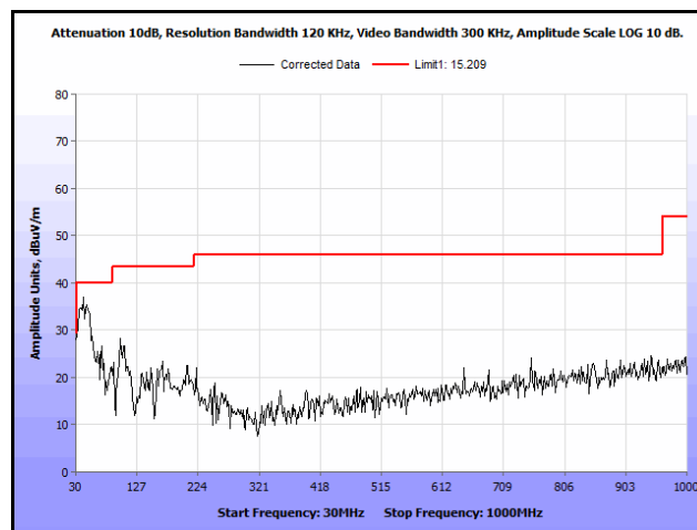
Plot 205. Radiated Spurs, Co-Location, 802.11n 20 MHz, 2462 MHz & 5200 MHz, 30 MHz – 1 GHz, Peak
