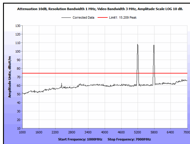
Plot 235. Radiated Spurs, Co-Location, 802.11n 20 MHz, 5200 MHz & 5785 MHz, 1 GHz – 7 GHz, Peak
