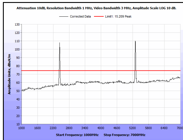
Plot 195. Radiated Spurs, Co-Location, 802.11n 20 MHz, 2437 MHz & 5300 MHz, 1 GHz – 7 GHz, Peak
