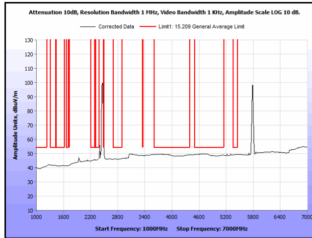
Plot 218. Radiated Spurs, Co-Location, 802.11n 20 MHz, 2462 MHz & 5785 MHz, 1 GHz – 7 GHz, Avg.
