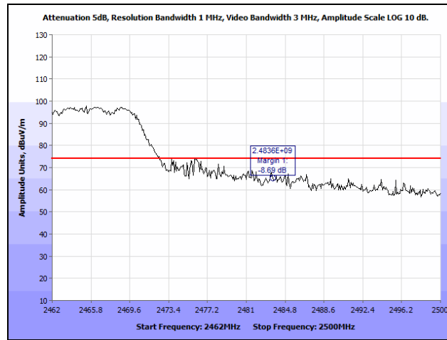
Plot 106. Radiated Restricted Band Edge, 802.11n 40 MHz, 2452 MHz @ 2483.5 MHz, Peak
