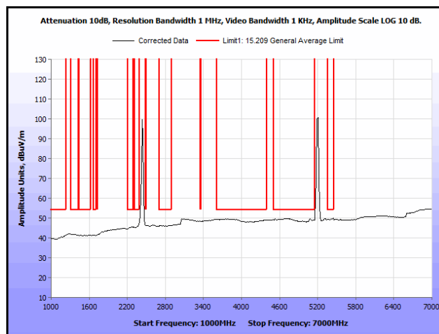
Plot 190. Radiated Spurs, Co-Location, 802.11n 20 MHz, 2437 MHz & 5200 MHz, 1 GHz – 7 GHz, Avg.
