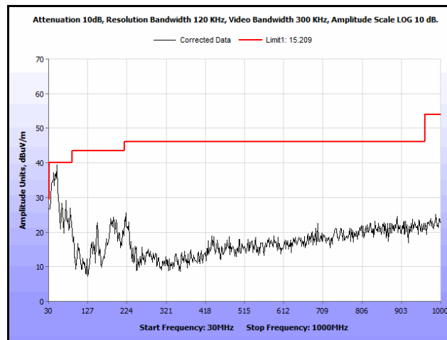
Plot 237. Radiated Spurs, Co-Location, 802.11n 20 MHz, 5300 MHz & 5300 MHz, 30 MHz – 1 GHz, Peak
