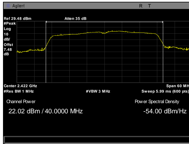
Plot 61. Peak Power Output, Low Channel, 2422 MHz, 802.11n 40 MHz, Port 1
