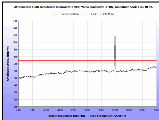
Plot 223. Radiated Spurs, Co-Location, 802.11n 20 MHz, 5200 MHz & 5200 MHz, 1 GHz – 7 GHz, Peak
