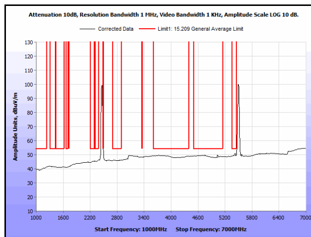
Plot 214. Radiated Spurs, Co-Location, 802.11n 20 MHz, 2462 MHz & 5580 MHz, 1 GHz – 7 GHz, Avg.
