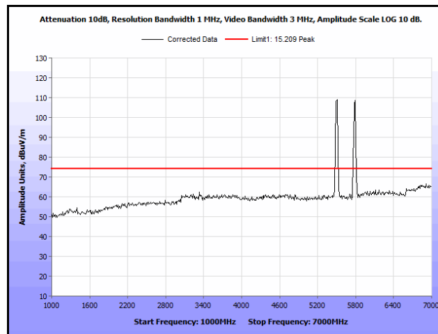
Plot 255. Radiated Spurs, Co-Location, 802.11n 20 MHz, 5580 MHz & 5785 MHz, 1 GHz – 7 GHz, Peak
