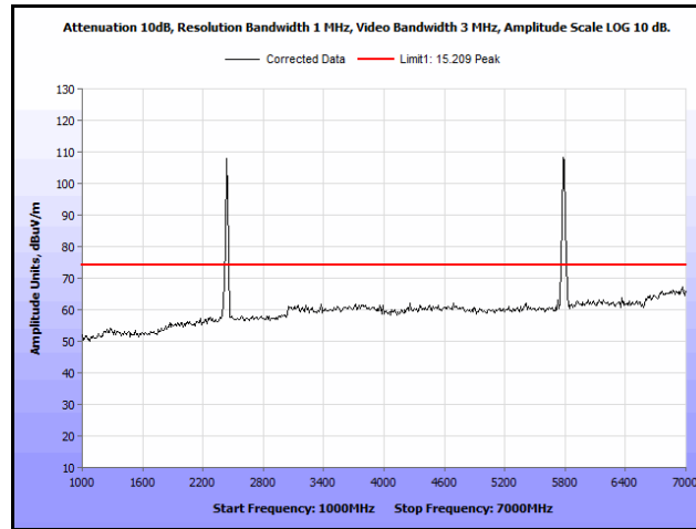
Plot 203. Radiated Spurs, Co-Location, 802.11n 20 MHz, 2437 MHz & 5785 MHz, 1 GHz – 7 GHz, Peak
