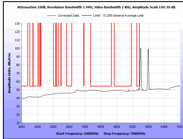
Plot 254. Radiated Spurs, Co-Location, 802.11n 20 MHz, 5580 MHz & 5785 MHz, 1 GHz – 7 GHz, Avg.
