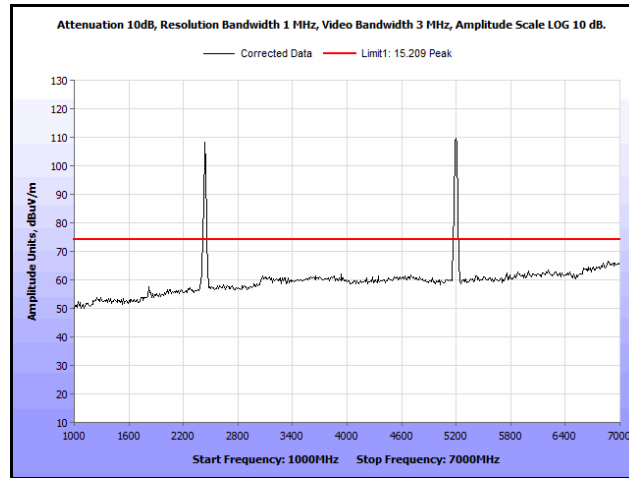
Plot 191. Radiated Spurs, Co-Location, 802.11n 20 MHz, 2437 MHz & 5200 MHz, 1 GHz – 7 GHz, Peak
