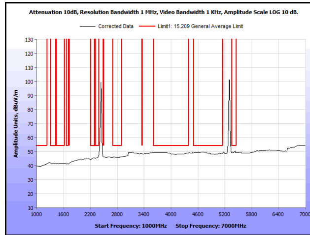
Plot 194. Radiated Spurs, Co-Location, 802.11n 20 MHz, 2437 MHz & 5300 MHz, 1 GHz – 7 GHz, Avg.
