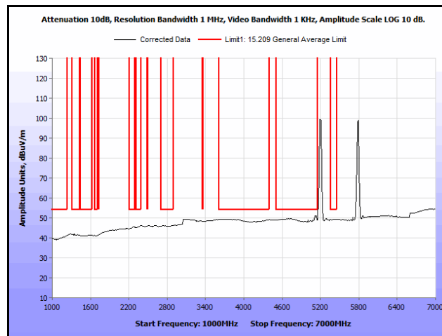
Plot 234. Radiated Spurs, Co-Location, 802.11n 20 MHz, 5200 MHz & 5785 MHz, 1 GHz – 7 GHz, Avg.
