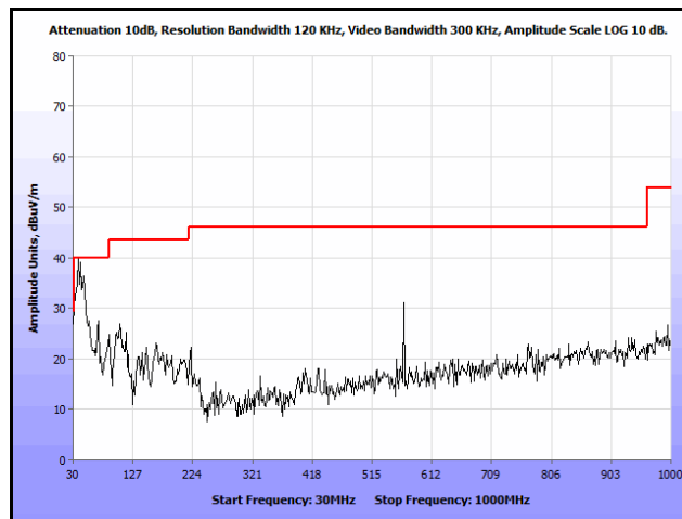
Plot 201. Radiated Spurs, Co-Location, 802.11n 20 MHz, 2437 MHz & 5785 MHz, 30 MHz – 1 GHz, Peak
