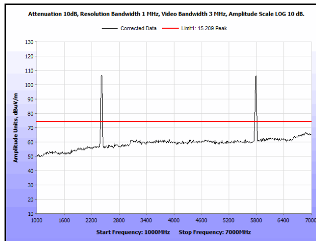
Plot 219. Radiated Spurs, Co-Location, 802.11n 20 MHz, 2462 MHz & 5785 MHz, 1 GHz – 7 GHz, Peak
