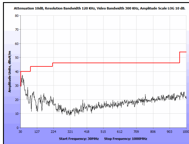
Plot 249. Radiated Spurs, Co-Location, 802.11n 20 MHz, 5580 MHz & 5580 MHz, 30 MHz – 1 GHz, Peak
