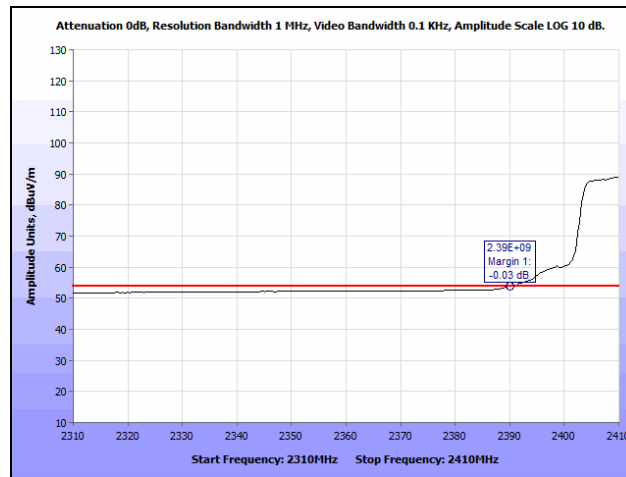
Plot 95. Radiated Restricted Band Edge, 802.11g, 2412 MHz @ 2390 MHz, Average
