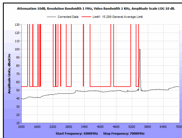
Plot 250. Radiated Spurs, Co-Location, 802.11n 20 MHz, 5580 MHz & 5580 MHz, 1 GHz – 7 GHz, Avg.
