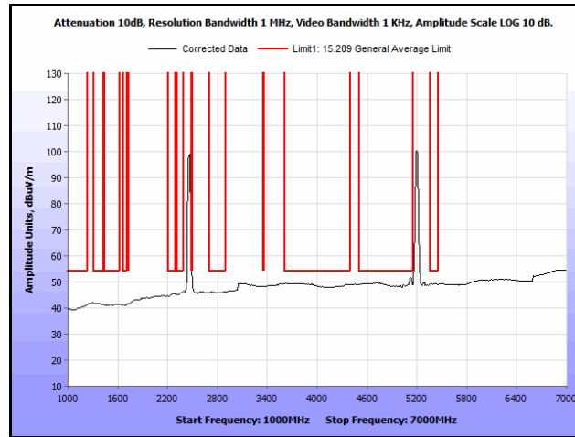
Plot 206. Radiated Spurs, Co-Location, 802.11n 20 MHz, 2462 MHz & 5200 MHz, 1 GHz – 7 GHz, Avg.
