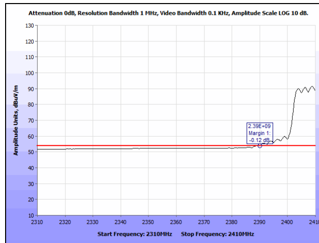
Plot 99. Radiated Restricted Band Edge, 802.11n 20 MHz, 2412 MHz @ 2390 MHz, Average
