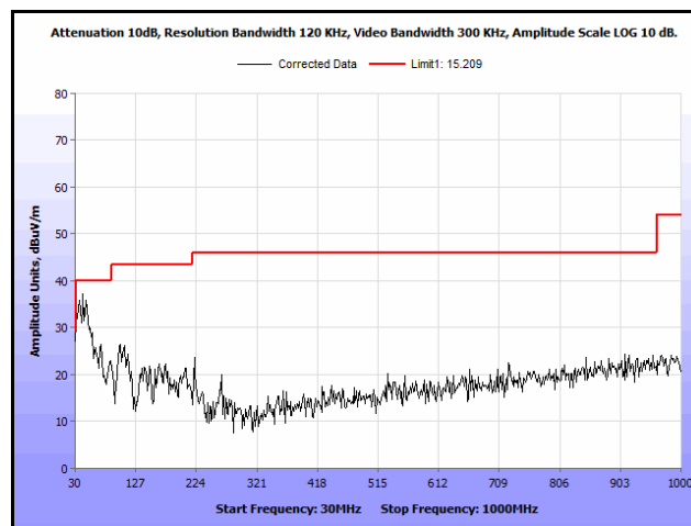
Plot 253. Radiated Spurs, Co-Location, 802.11n 20 MHz, 5580 MHz & 5785 MHz, 30 MHz – 1 GHz, Peak
