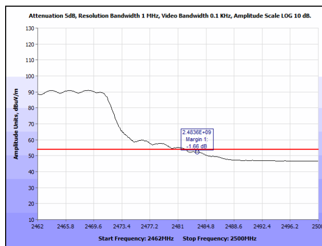
Plot 101. Radiated Restricted Band Edge, 802.11n 20 MHz, 2462 MHz @ 2483.5 MHz, Average
