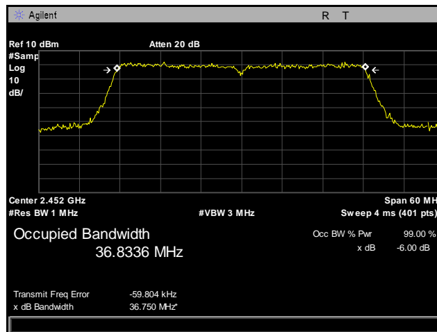
Plot 48. 99% Occupied Bandwidth, High Channel, 2452 MHz, 802.11n 40 MHz, Port 2
