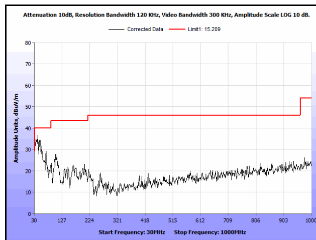
Plot 217. Radiated Spurs, Co-Location, 802.11n 20 MHz, 2462 MHz & 5785 MHz, 30 MHz – 1 GHz, Peak
