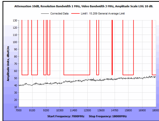
Plot 236. Radiated Spurs, Co-Location, 802.11n 20 MHz, 5200 MHz & 5785 MHz, 7 GHz – 18 GHz, Peak
