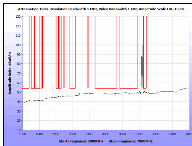
Plot 238. Radiated Spurs, Co-Location, 802.11n 20 MHz, 5300 MHz & 5300 MHz, 1 GHz – 7 GHz, Avg.
