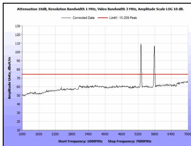
Plot 247. Radiated Spurs, Co-Location, 802.11n 20 MHz, 5300 MHz & 5785 MHz, 1 GHz – 7 GHz, Peak
