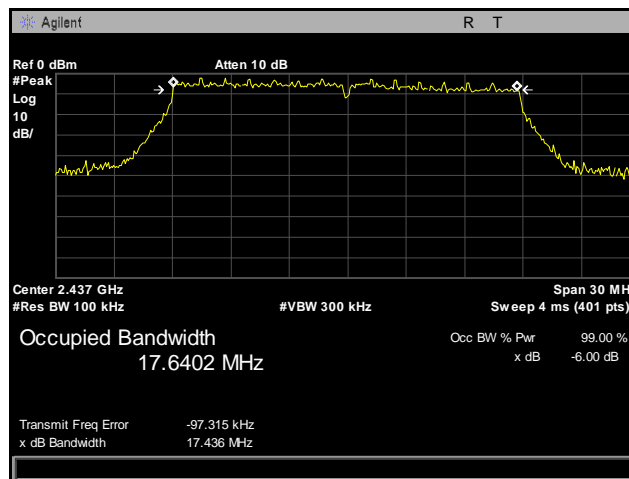
Plot 23. 6 dB Occupied Bandwidth, Mid Channel, 2437 MHz, 802.11n 20 MHz, Port 2
