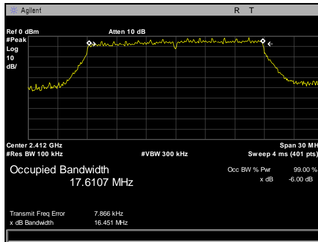
Plot 22. 6 dB Occupied Bandwidth, Low Channel, 2412 MHz, 802.11n 20 MHz, Port 2
