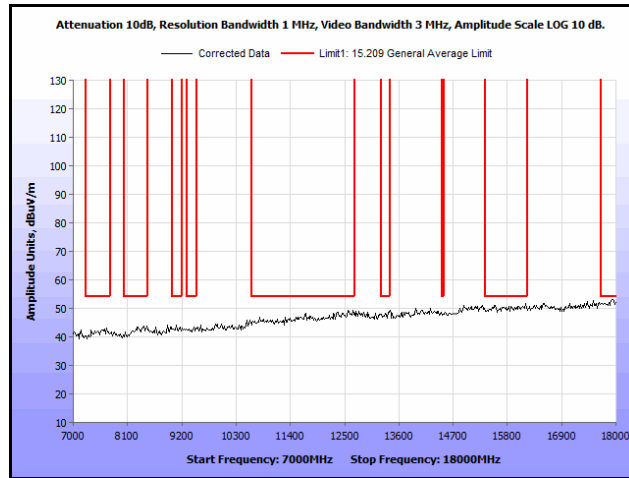
Plot 200. Radiated Spurs, Co-Location, 802.11n 20 MHz, 2437 MHz & 5580 MHz, 7 GHz – 18 GHz, Peak
