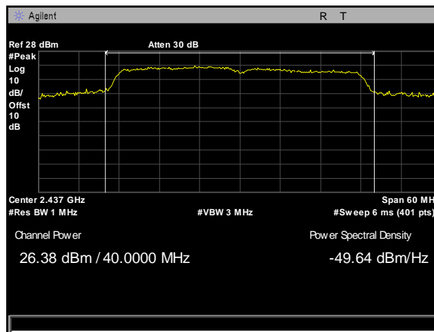
Plot 62. Peak Power Output, Mid Channel, 2437 MHz, 802.11n 40 MHz, Port 1
