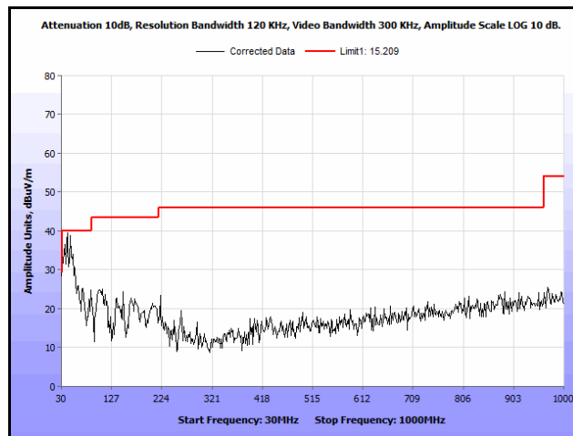
Plot 213. Radiated Spurs, Co-Location, 802.11n 20 MHz, 2462 MHz & 5580 MHz, 30 MHz – 1 GHz, Peak
