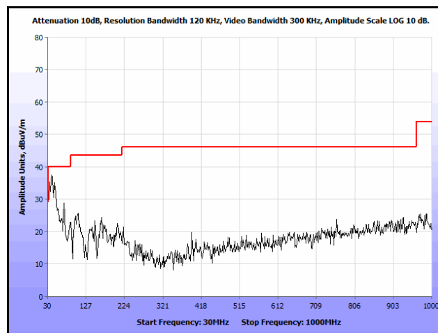
Plot 193. Radiated Spurs, Co-Location, 802.11n 20 MHz, 2437 MHz & 5300 MHz, 30 MHz – 1 GHz, Peak
