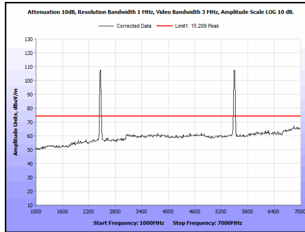
Plot 215. Radiated Spurs, Co-Location, 802.11n 20 MHz, 2462 MHz & 5580 MHz, 1 GHz – 7 GHz, Peak
