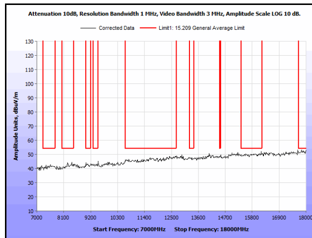
Plot 204. Radiated Spurs, Co-Location, 802.11n 20 MHz, 2437 MHz & 5785 MHz, 7 GHz – 18 GHz, Peak
