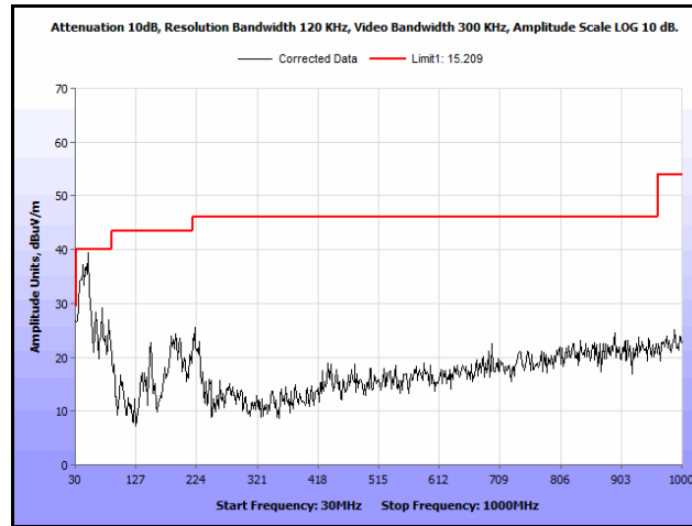
Plot 233. Radiated Spurs, Co-Location, 802.11n 20 MHz, 5200 MHz & 5785 MHz, 30 MHz – 1 GHz, Peak
