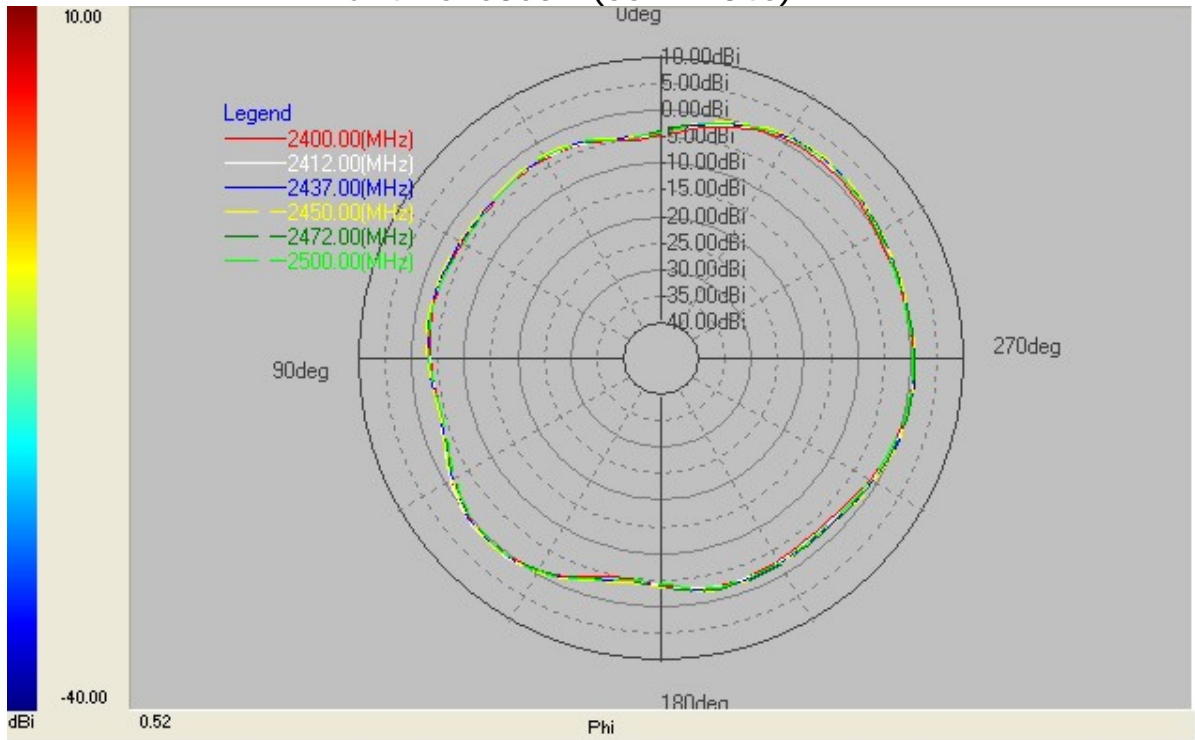
X-Y plane(theta=90)
