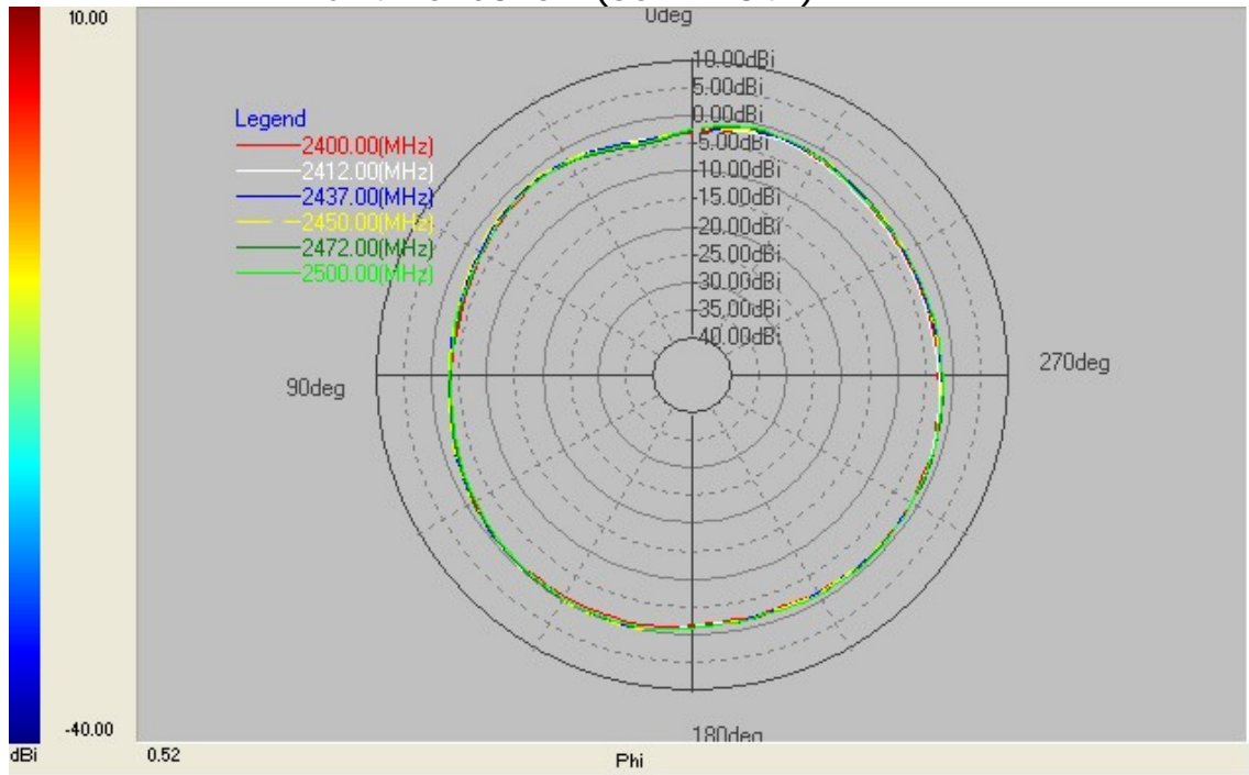
X-Y plane(theta=90)
