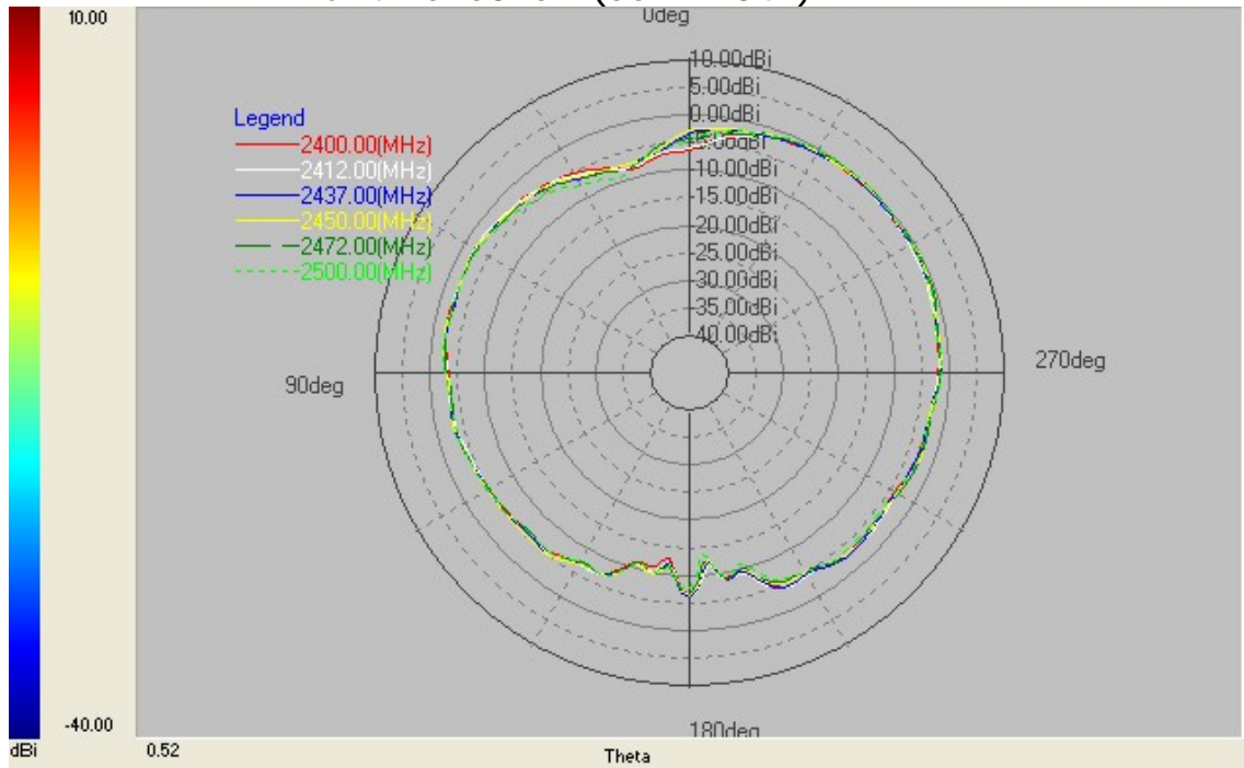
X-Z plane(Phi=0)
