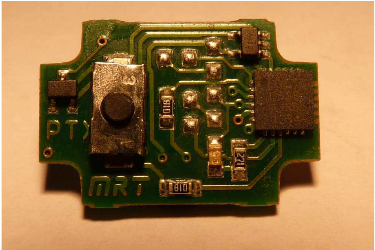
PTX Internal Photos
