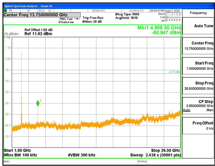
2DH1_Ant1_2480_1000~26500
