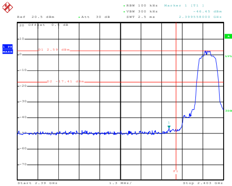
No-hopping mode
