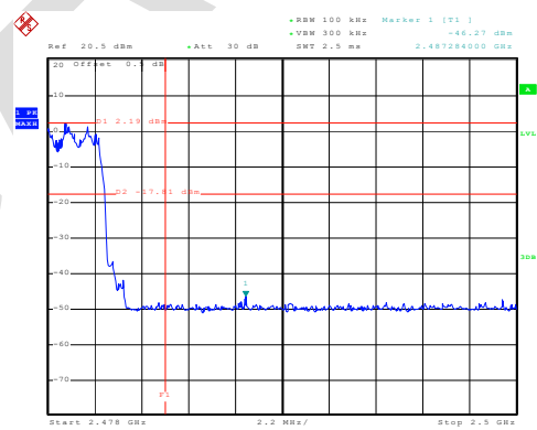
Hopping mode
