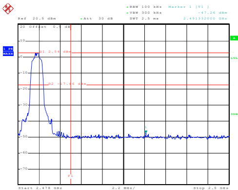
No-hopping mode
