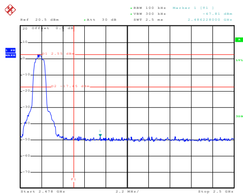
No-hopping mode
