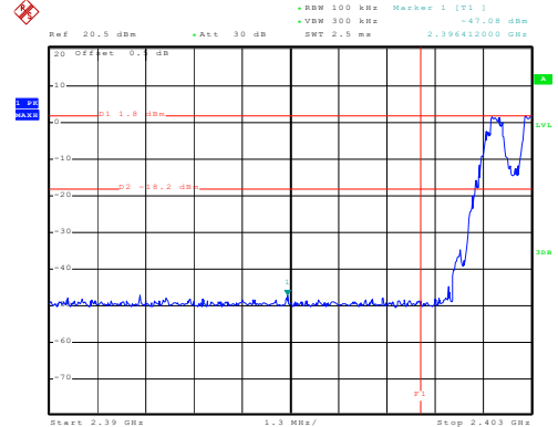
Hopping mode
