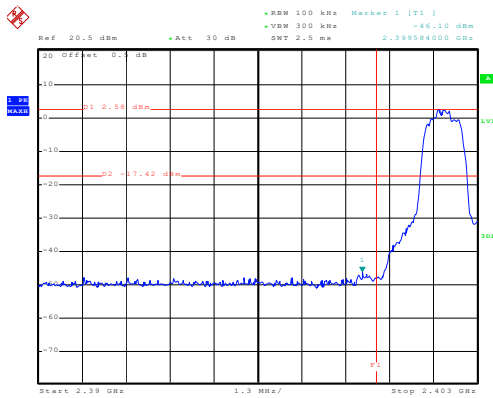
No-hopping mode
