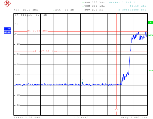
Hopping mode
