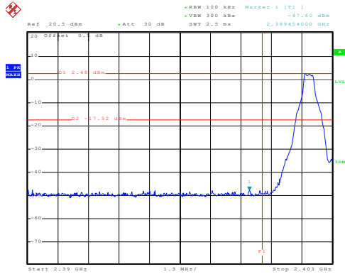
No-hopping mode
