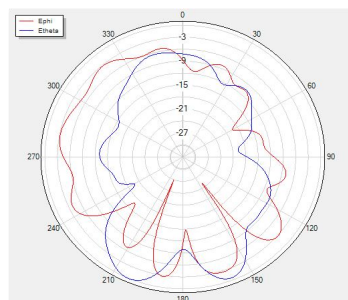
Phi=0 freq=2400MHz
